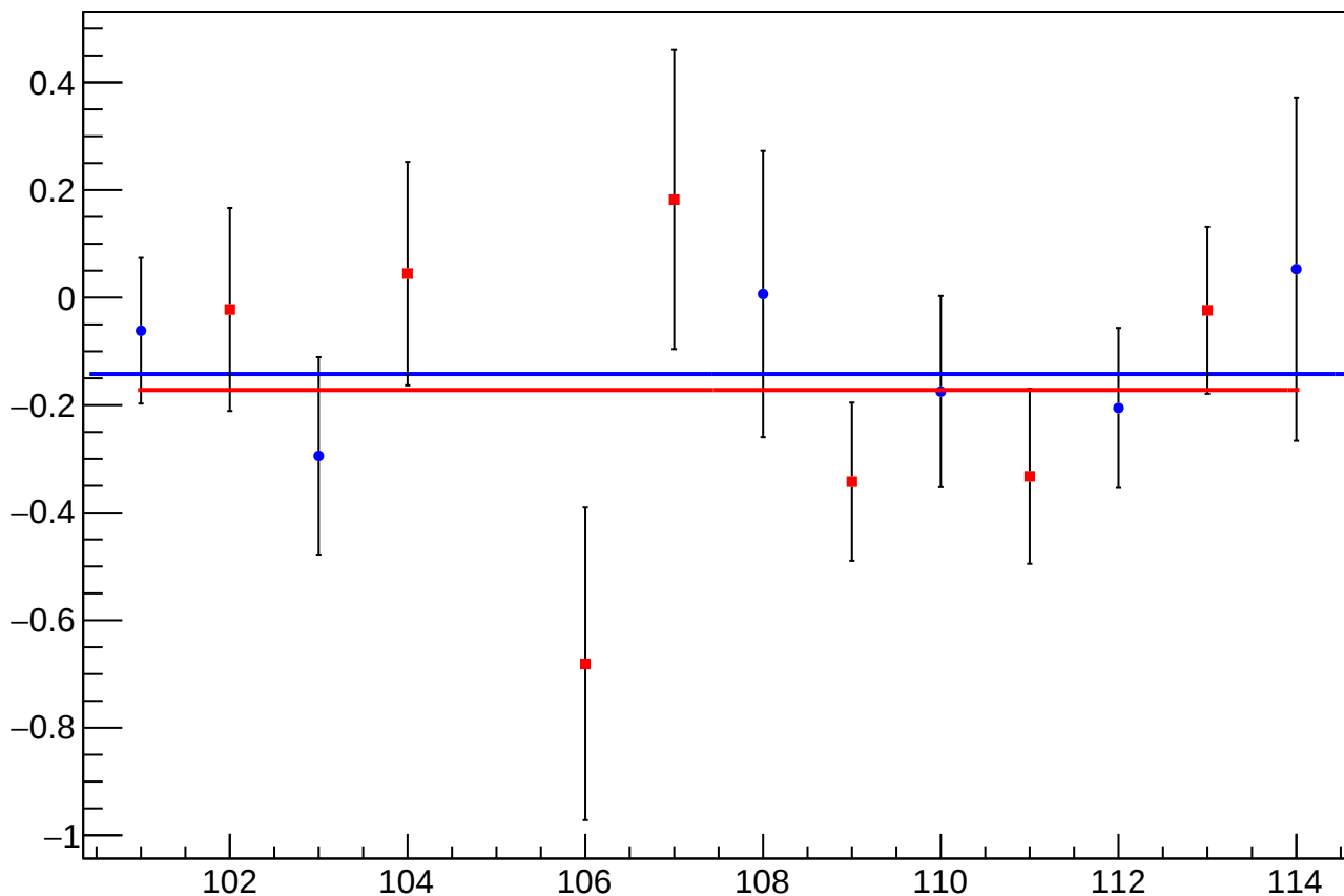
reg_asym_dsl_diff_bpm4aX_slope vs Slug
