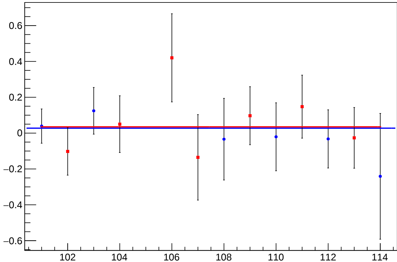
reg_asym_ds_avg_diff_bpm4eX_slope vs Slug
