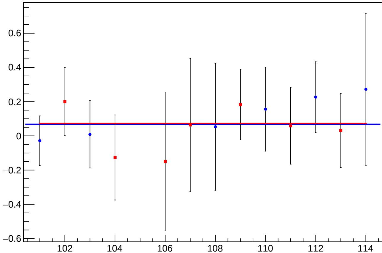
reg_asym_dsr_diff_bpm4aX_slope vs Slug
