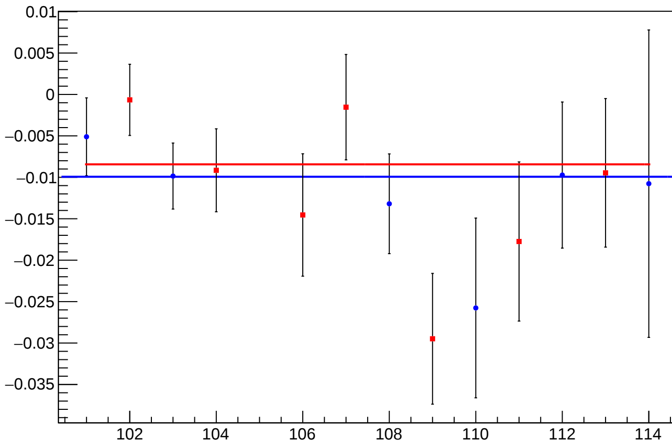
reg_asym_dsl_diff_bpm12X_slope vs Slug
