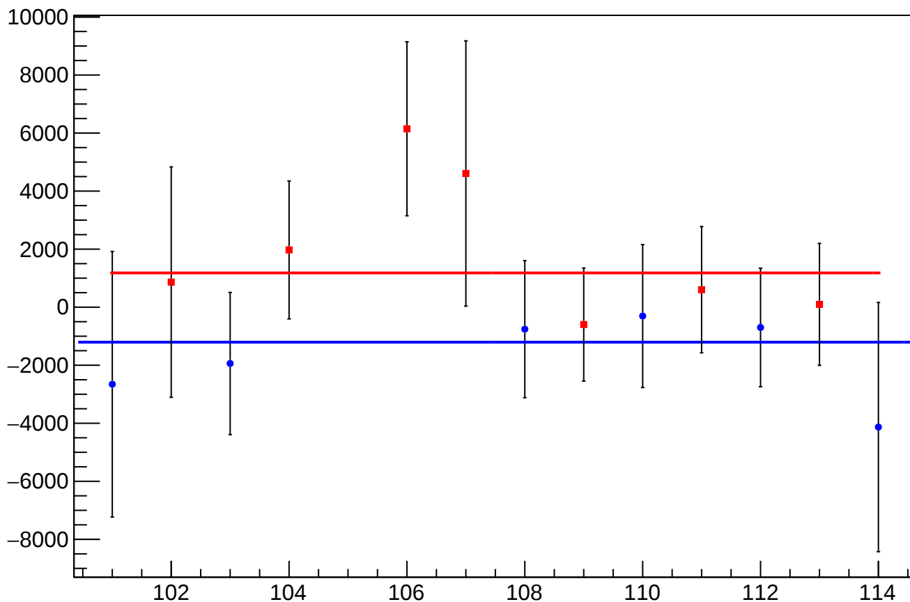
asym_atl_avg_atr_avg_dd_mean vs Slug
