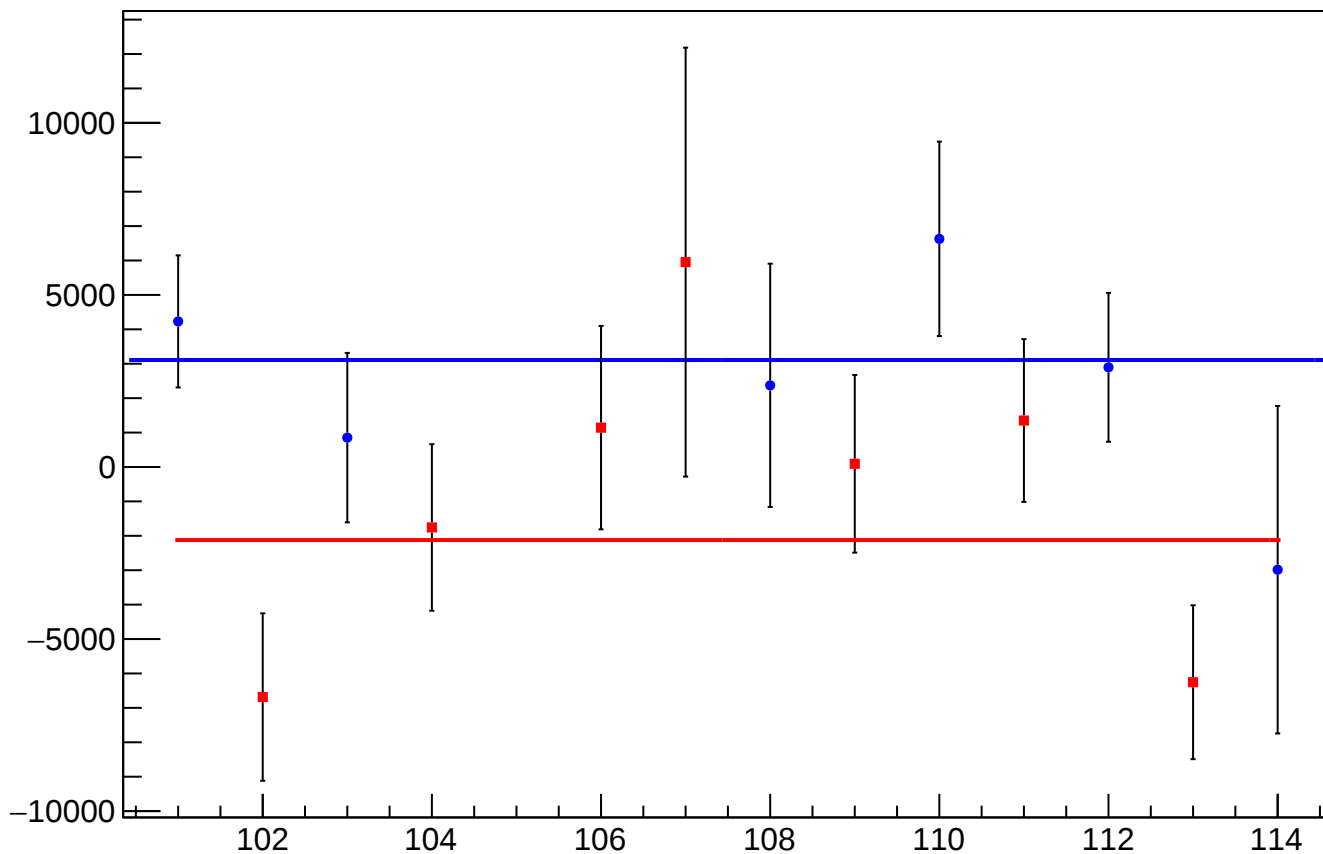
asym_usl_mean vs Slug
