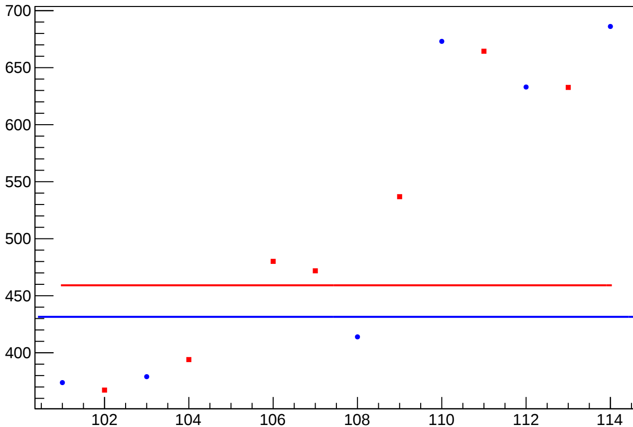
asym_sam6_correction_rms vs Slug
