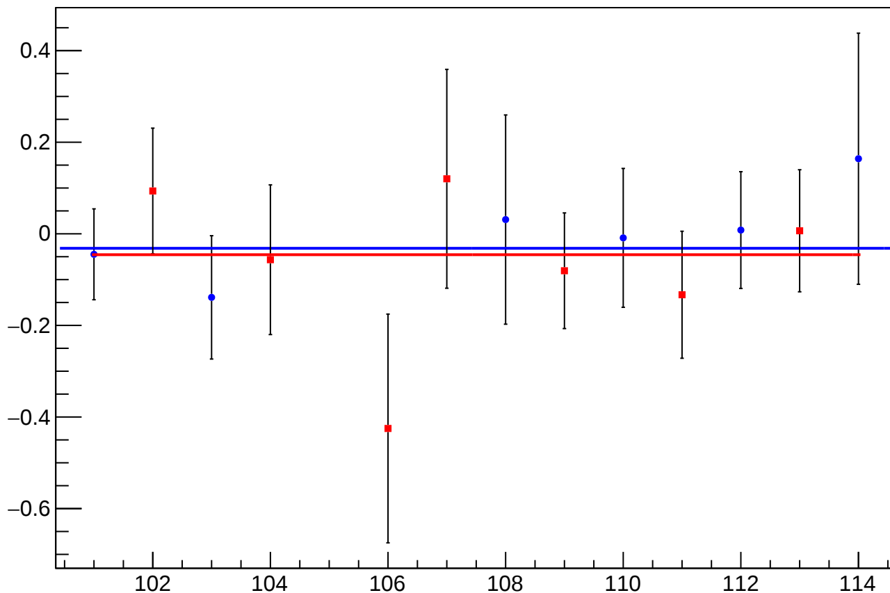
reg_asym_ds_avg_diff_bpm4aX_slope vs Slug
