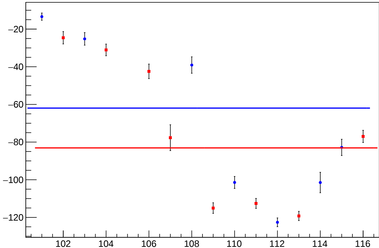
reg_asym_us_avg_diff_bpm4aX_slope vs Slug
