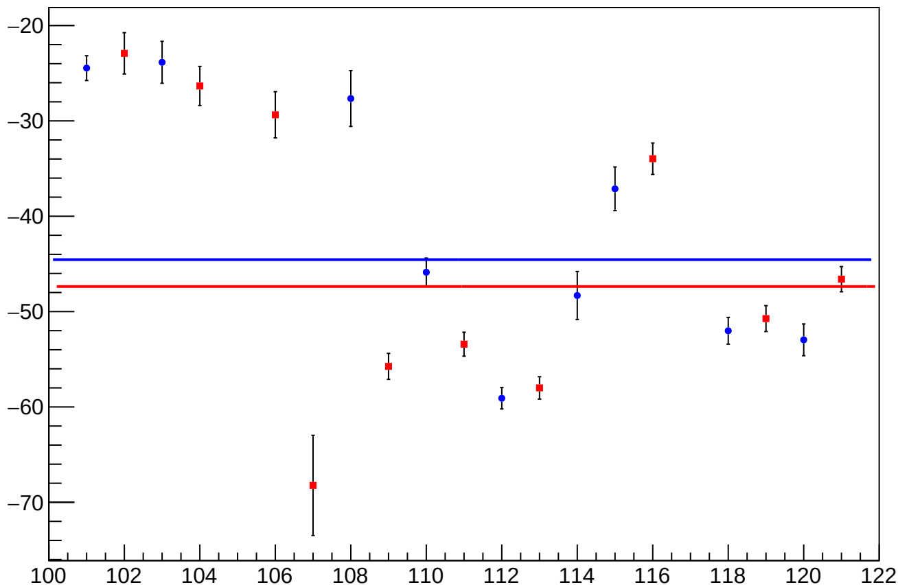
reg_asym_left_dd_diff_bpm4aX_slope vs Slug, Sign Corrected
