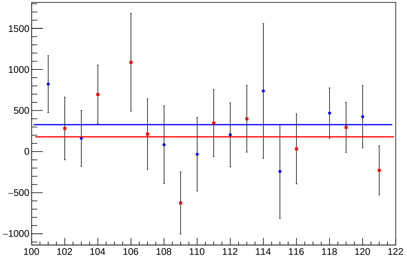
dit_asym_sam_26_dd_mean vs Slug, Sign Corrected
