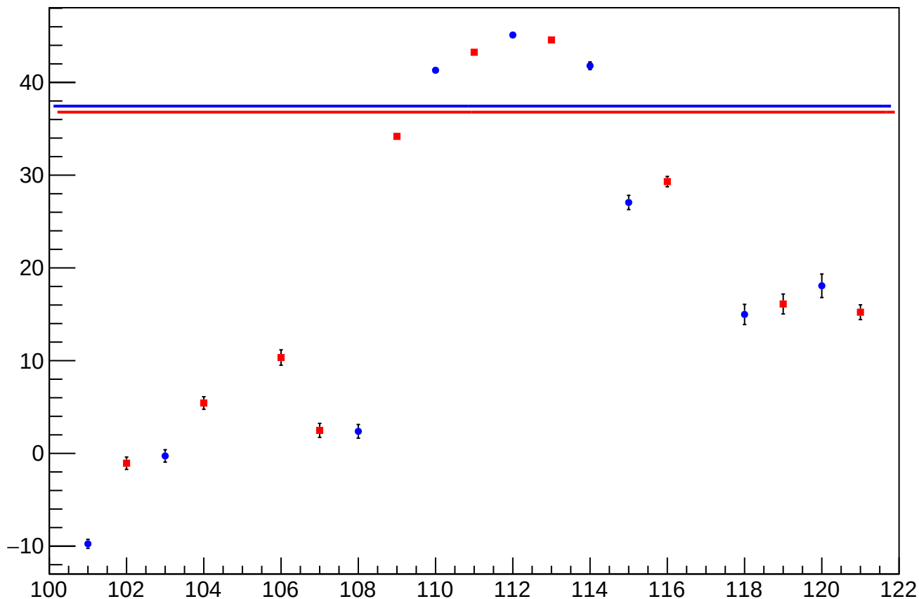
reg_asym_sam8_diff_bpm4aX_slope vs Slug, Sign Corrected
