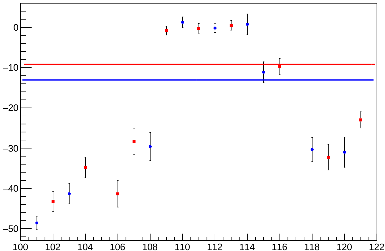
reg_asym_sam_37_avg_diff_bpm4aX_slope vs Slug, Sign Corrected
