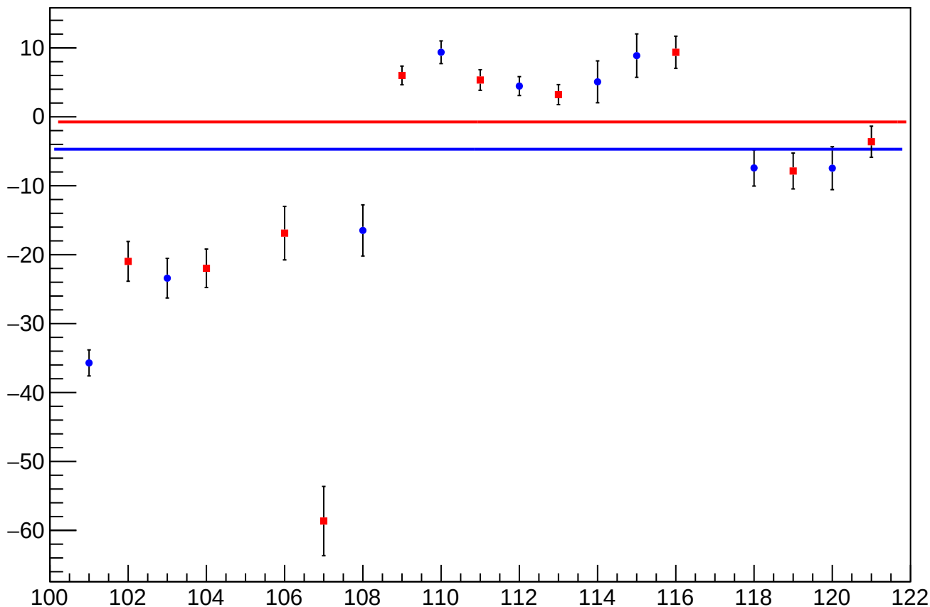
reg_asym_us_dd_diff_bpm4aX_slope vs Slug, Sign Corrected
