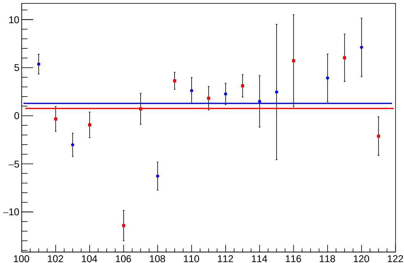
reg_asym_sam5_diff_bpm4aX_slope vs Slug, Sign Corrected
