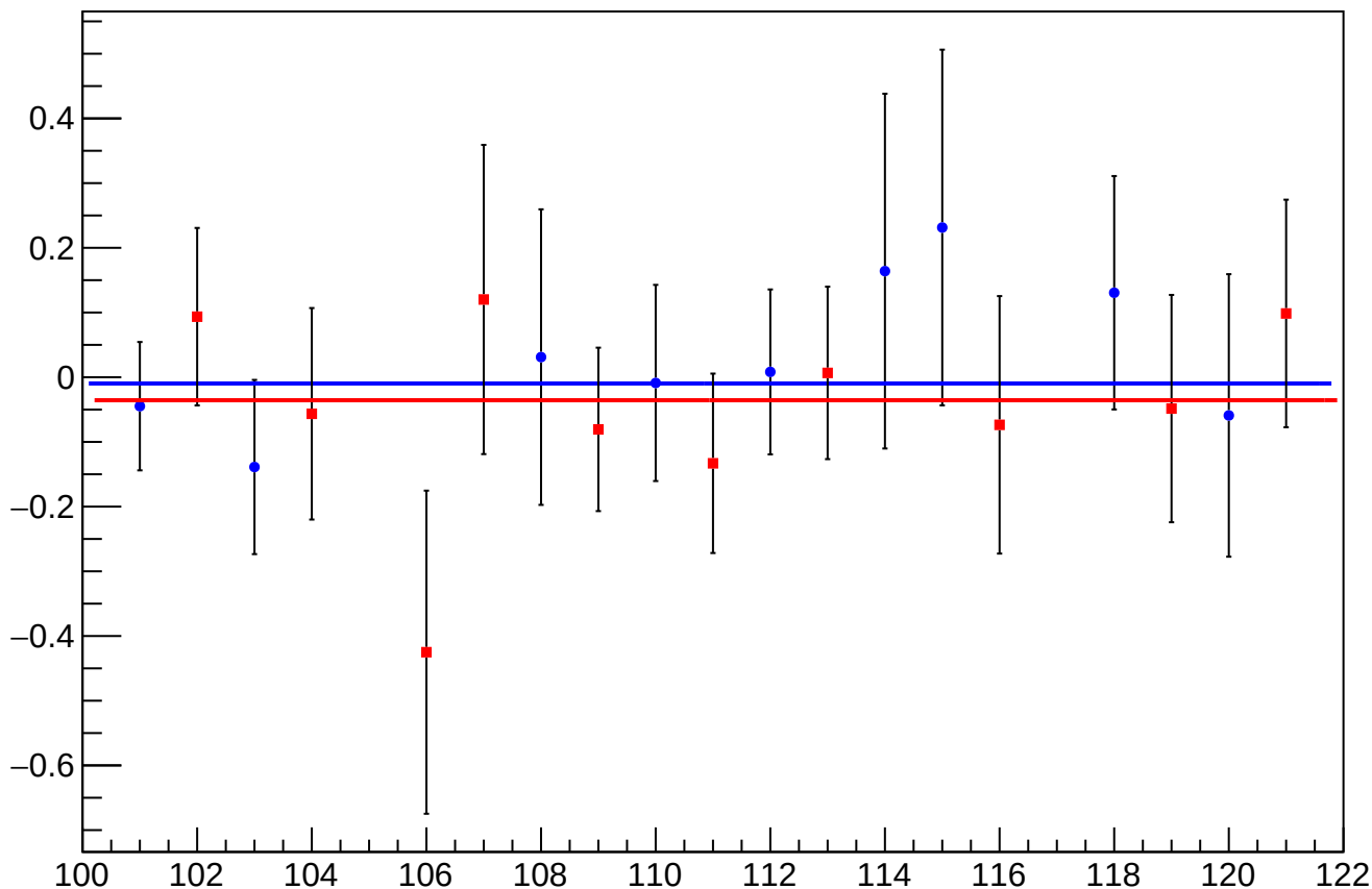
reg_asym_ds_avg_diff_bpm4aX_slope vs Slug, Sign Corrected
