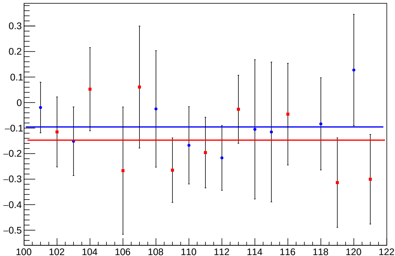
reg_asym_ds_dd_diff_bpm4aX_slope vs Slug, Sign Corrected
