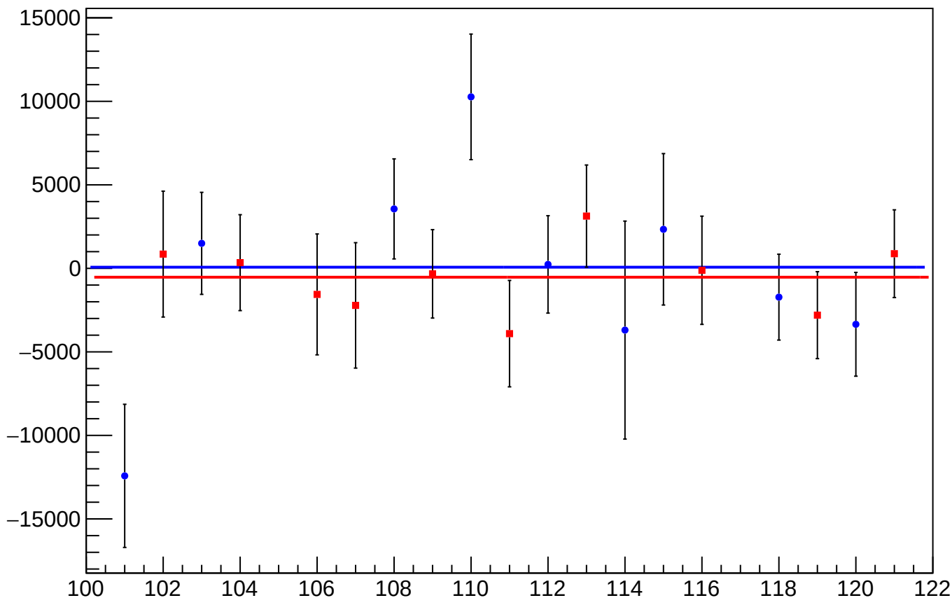
asym_atl_dd_atr_dd_dd_mean vs Slug, Sign Corrected
