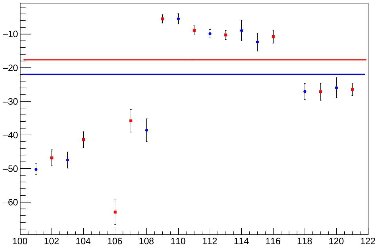
reg_asym_sam_12345678_avg_diff_bpm4aX_slope vs Slug, Sign Corrected
