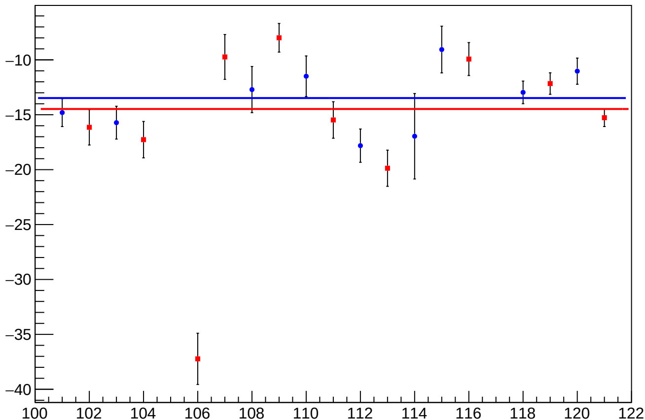
reg_asym_sam1_diff_bpm4aX_slope vs Slug, Sign Corrected
