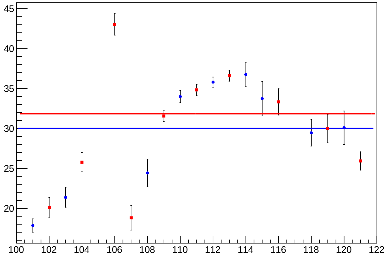
reg_asym_sam_15_37_dd_diff_bpm4eX_slope vs Slug, Sign Corrected
