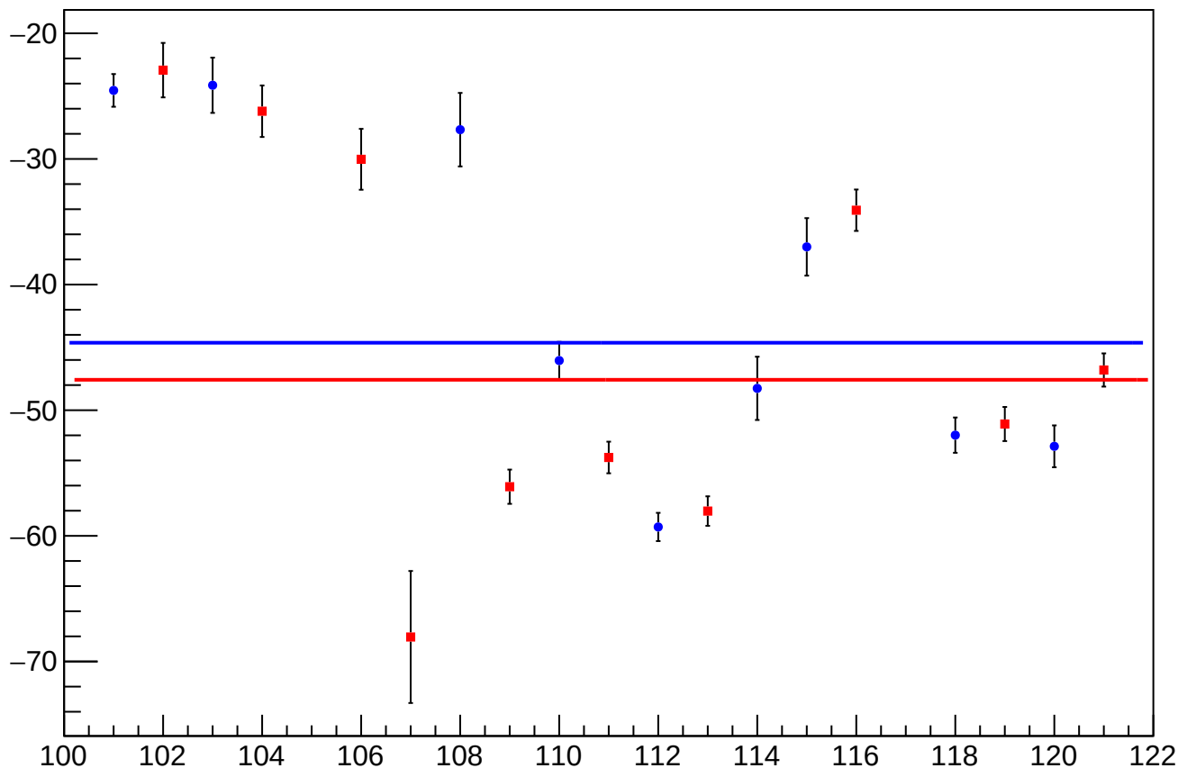
reg_asym_left_avg_diff_bpm4aX_slope vs Slug, Sign Corrected
