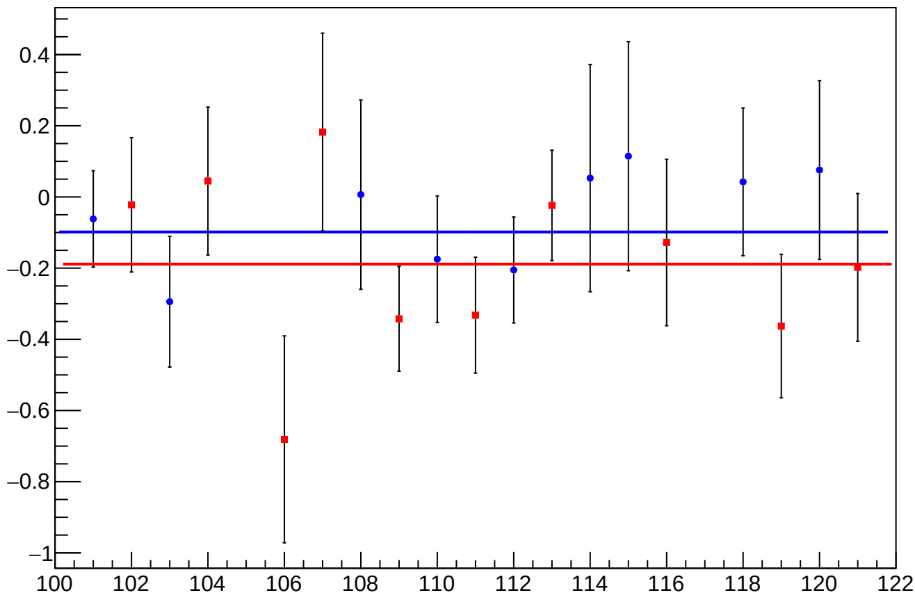
reg_asym_dsl_diff_bpm4aX_slope vs Slug, Sign Corrected
