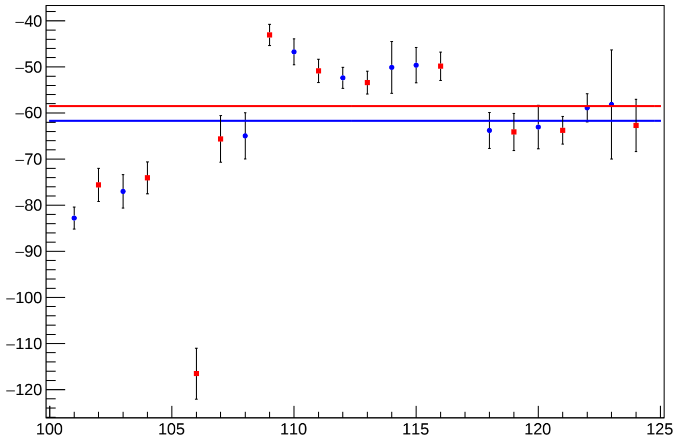
reg_asym_sam_24_68_dd_diff_bpm4aX_slope vs Slug, Sign Corrected
