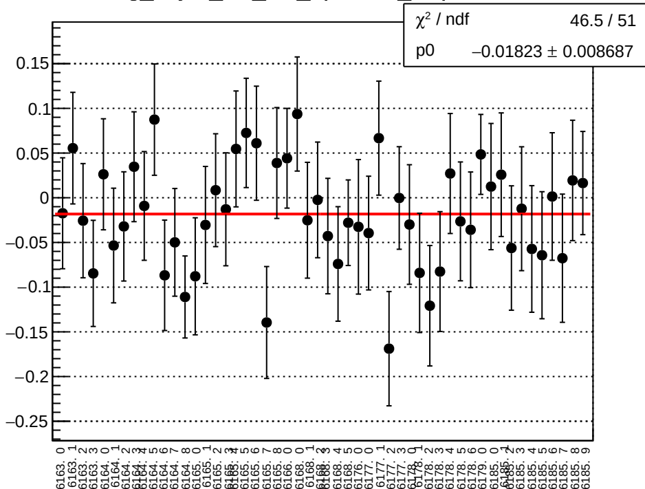
reg asym dsl diff bpm12X slope vs run
