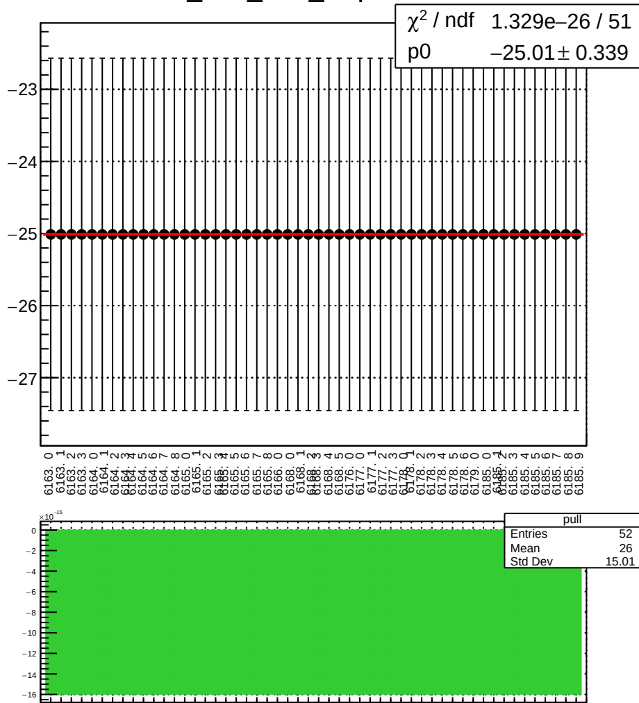
dit_atr1_4eY_slope vs run
