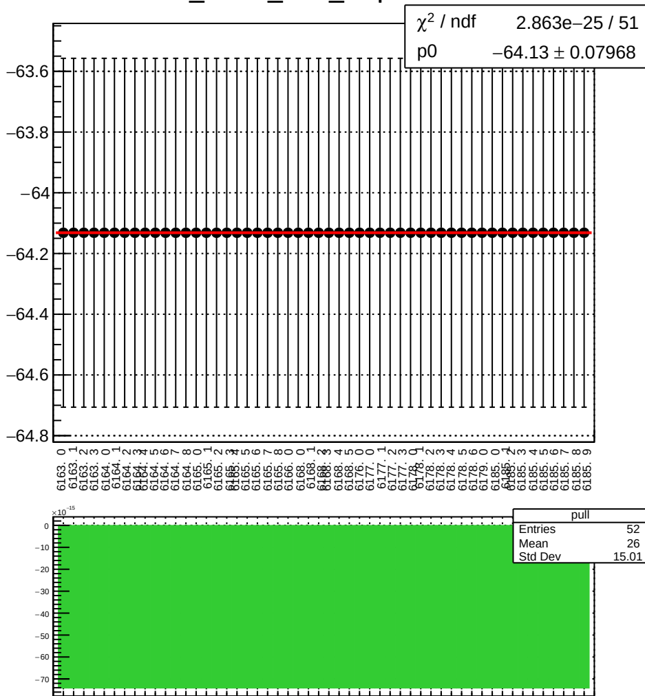
dit_sam8_4eX_slope vs run
