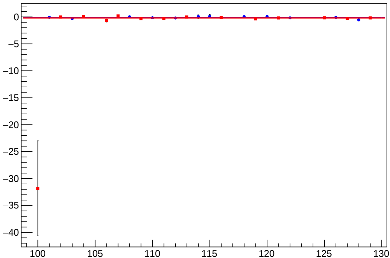
reg_asym_dsl_diff_bpm4aX_slope vs Slug, Sign Corrected
