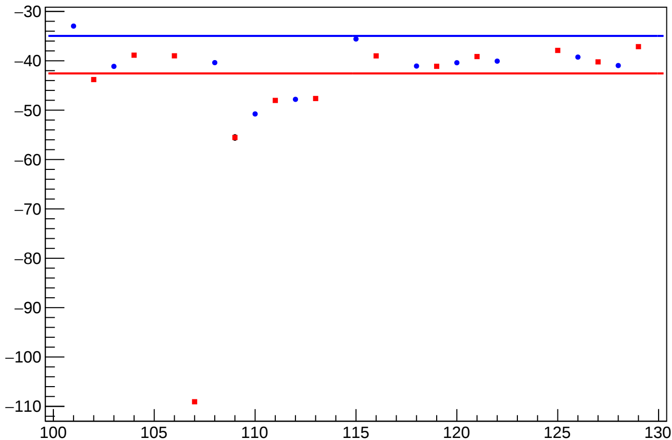
dit_usl_11X12X_slope vs Slug, Sign Corrected
