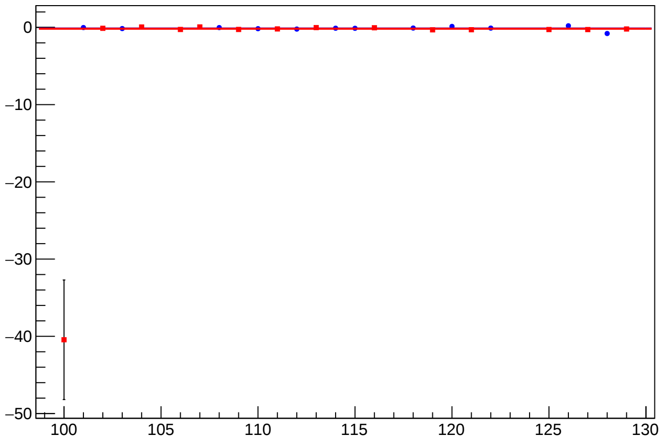
reg_asym_ds_dd_diff_bpm4aX_slope vs Slug, Sign Corrected
