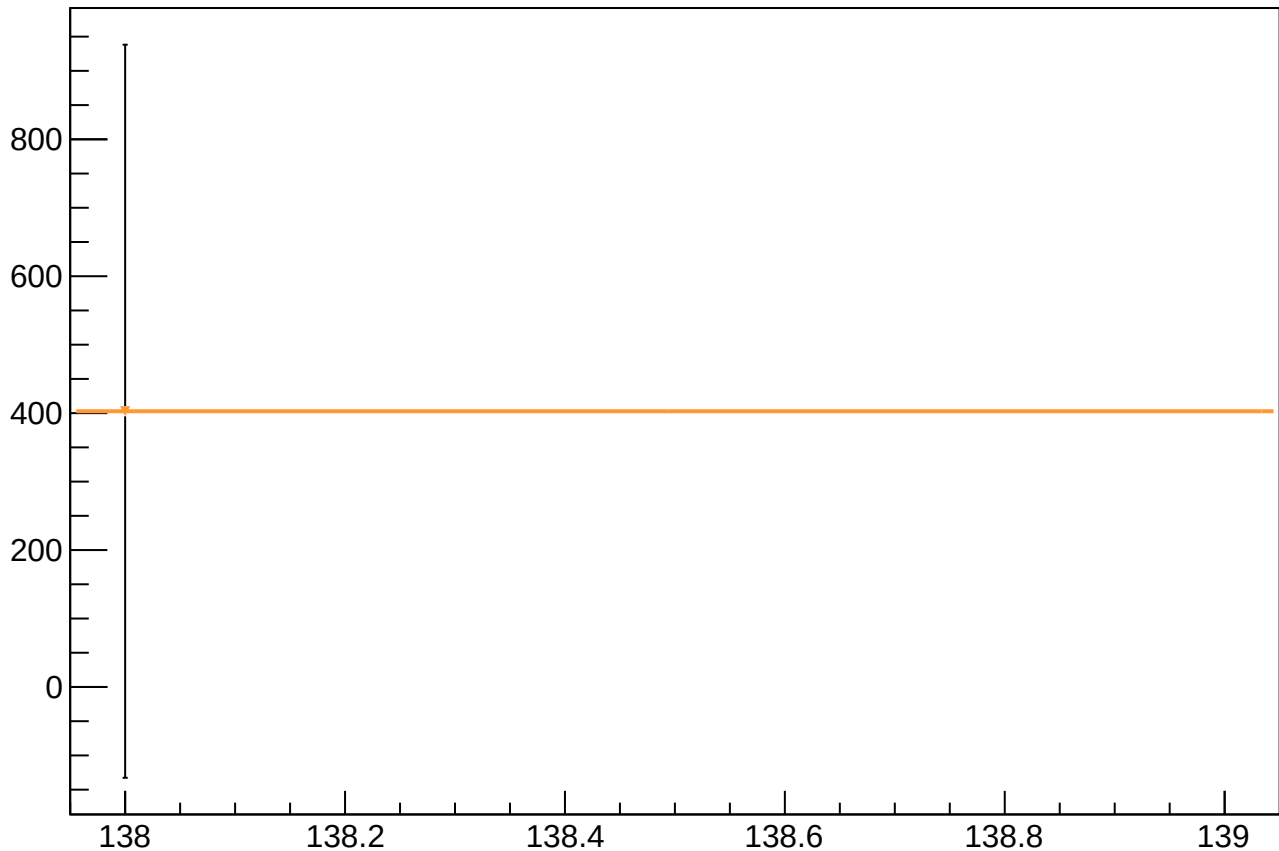
asym_sam_37_48_dd_correction_mean vs Slug
