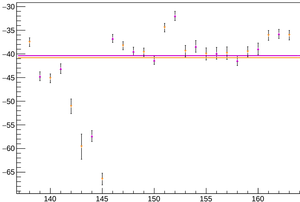
reg_asym_left_dd_diff_bpm1X_slope vs Slug
