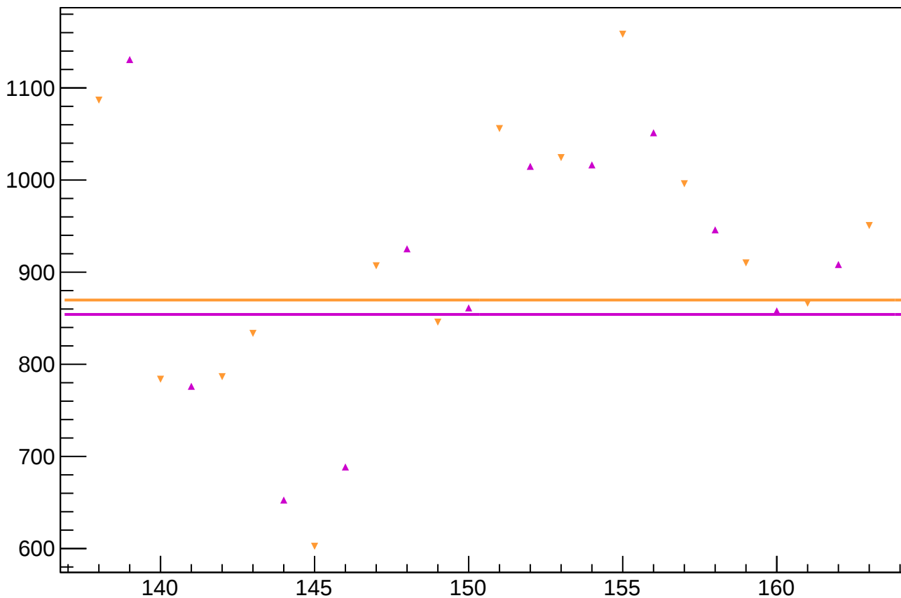
asym_sam_3748_avg_rms vs Slug
