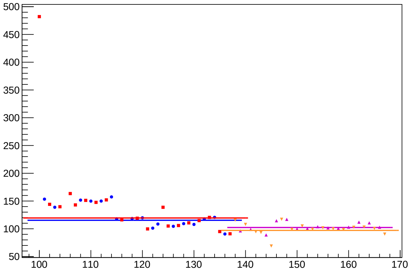
dit_asym_sam_26_48_dd_rms vs Slug
