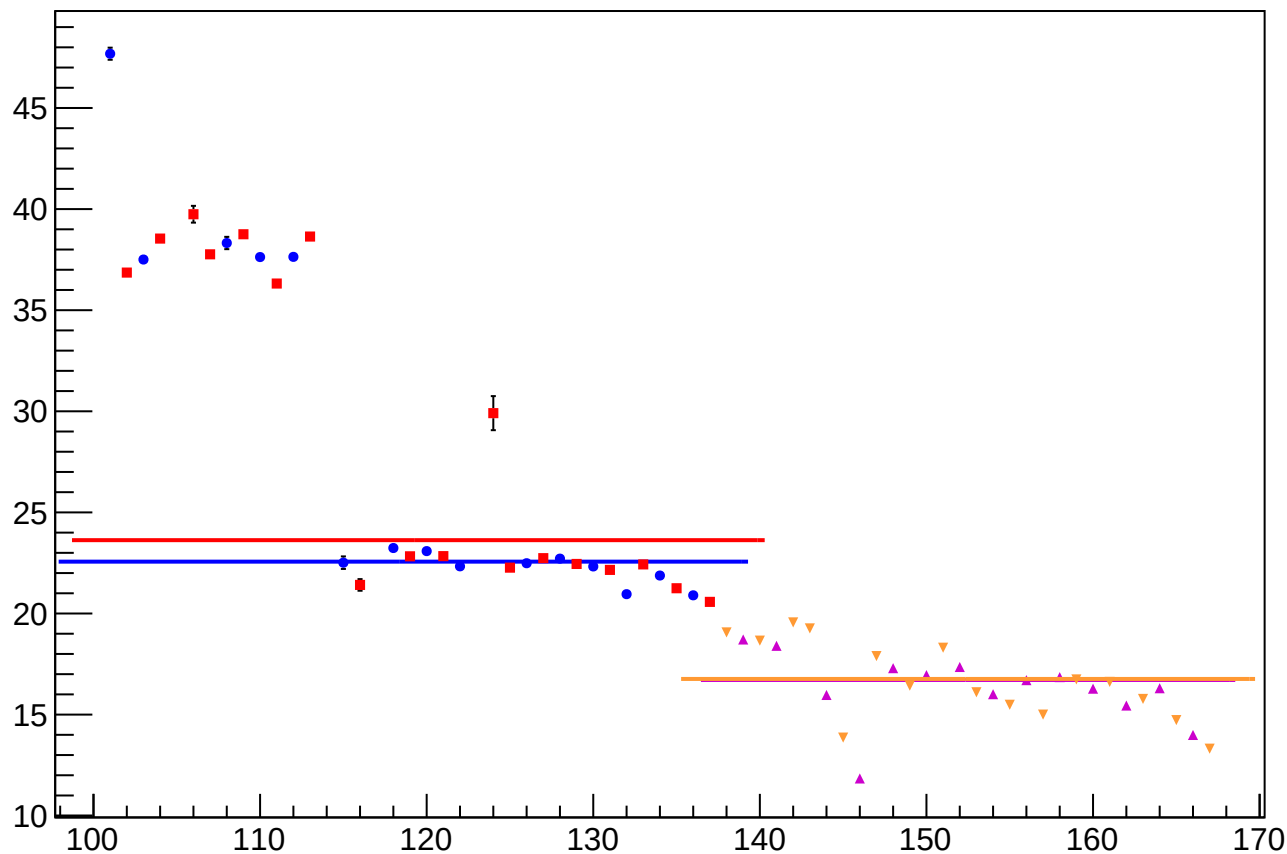
dit_sam6_4aY_slope vs Slug
