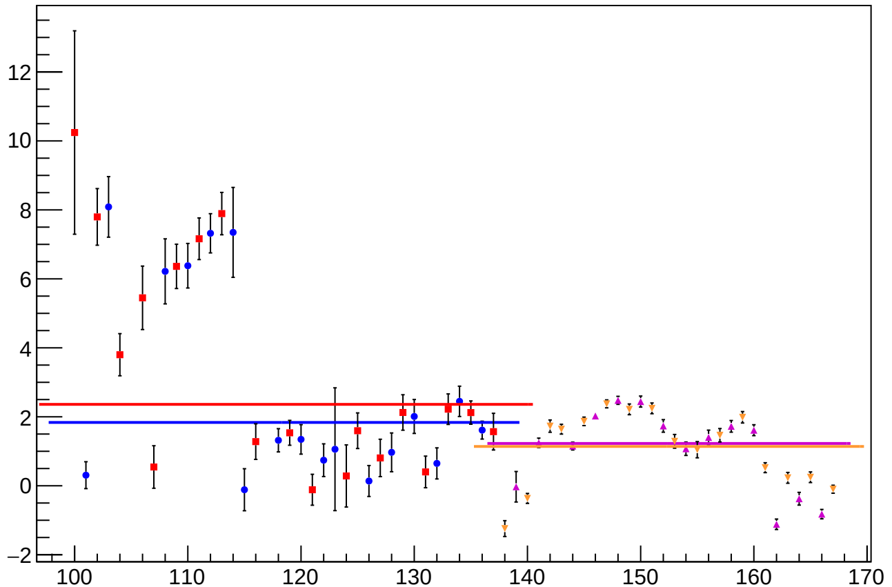
reg_asym_sam_1357_2468_dd_diff_bpm4aY_slope vs Slug
