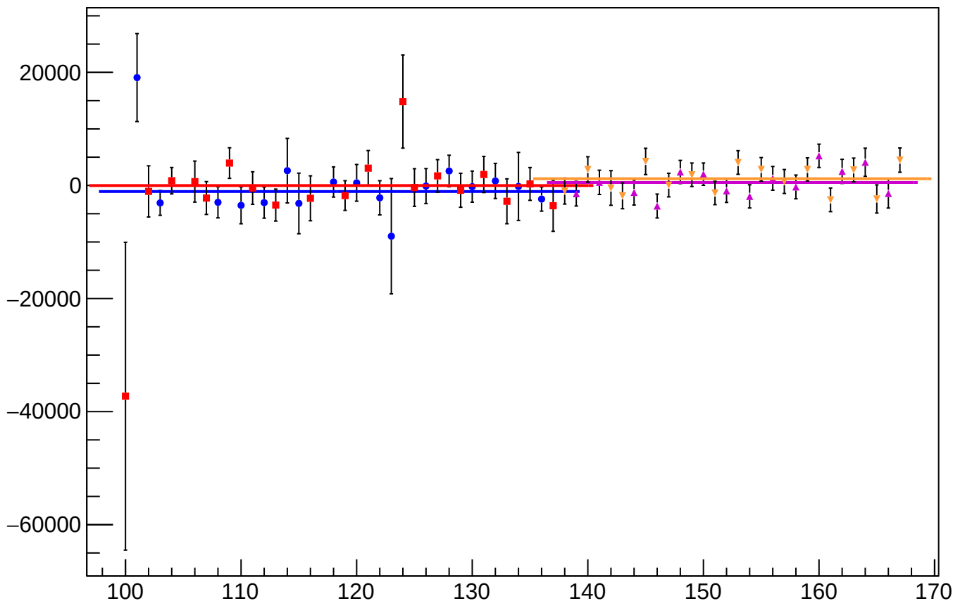
dit_asym_atr_dd_mean vs Slug
