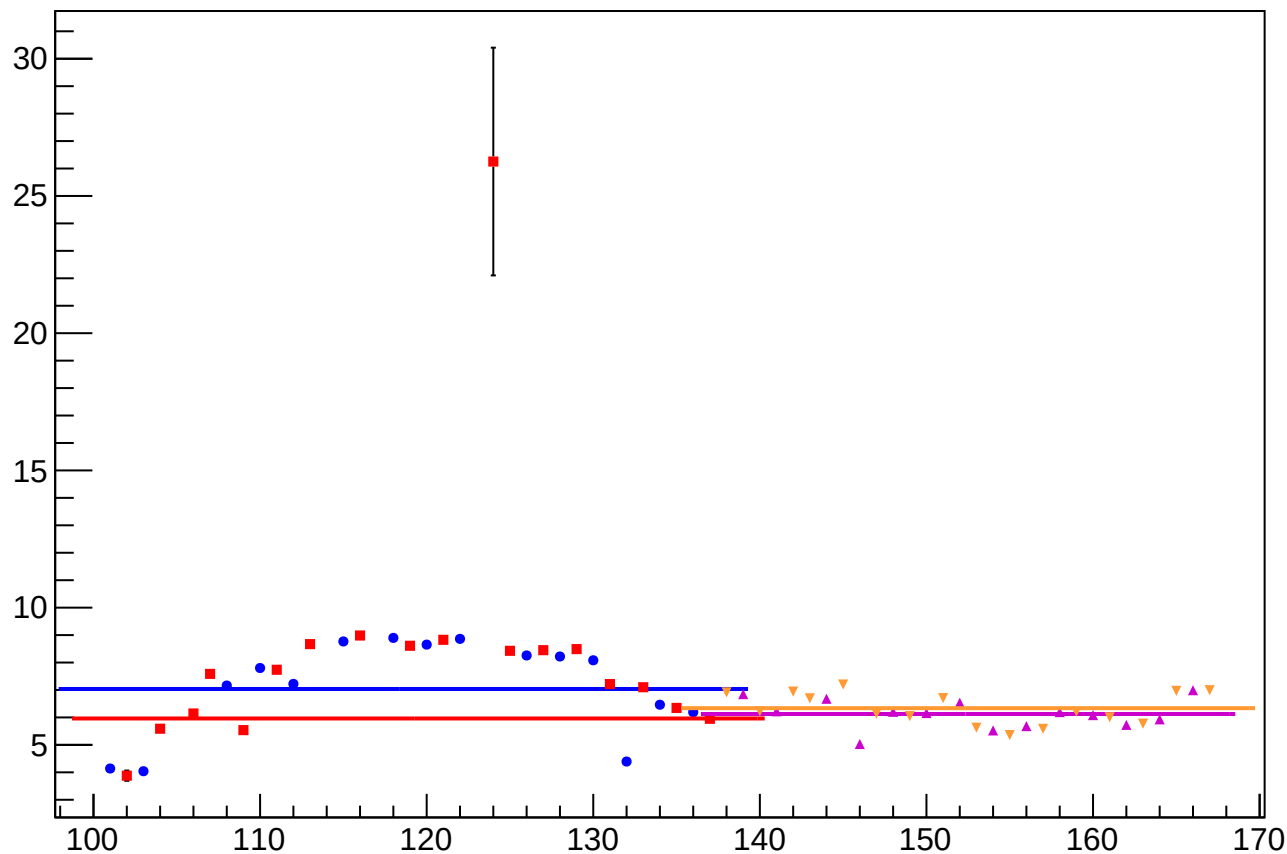
dit_sam7_4aY_slope vs Slug
