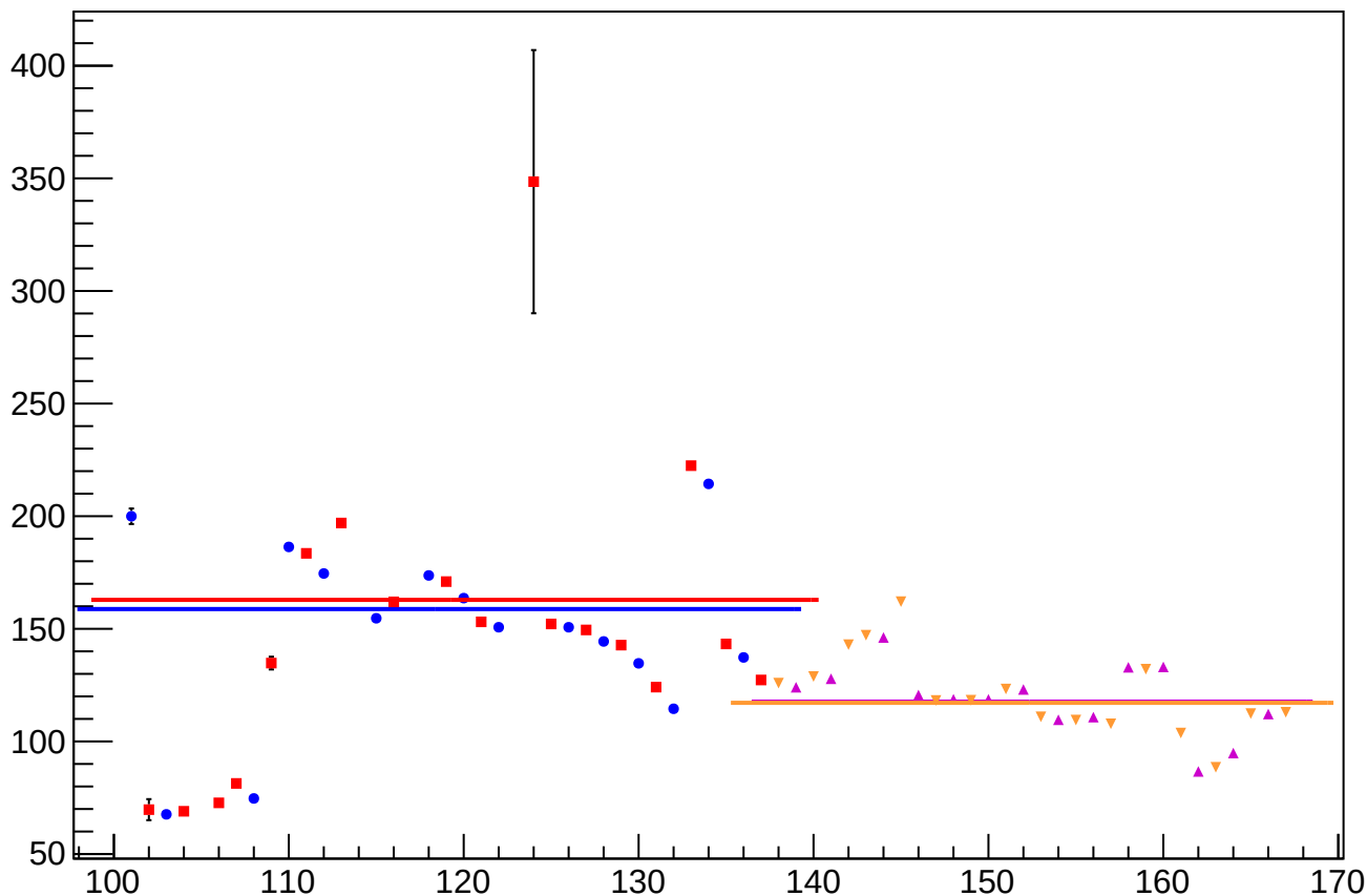
dit_atr2_4eY_slope vs Slug
