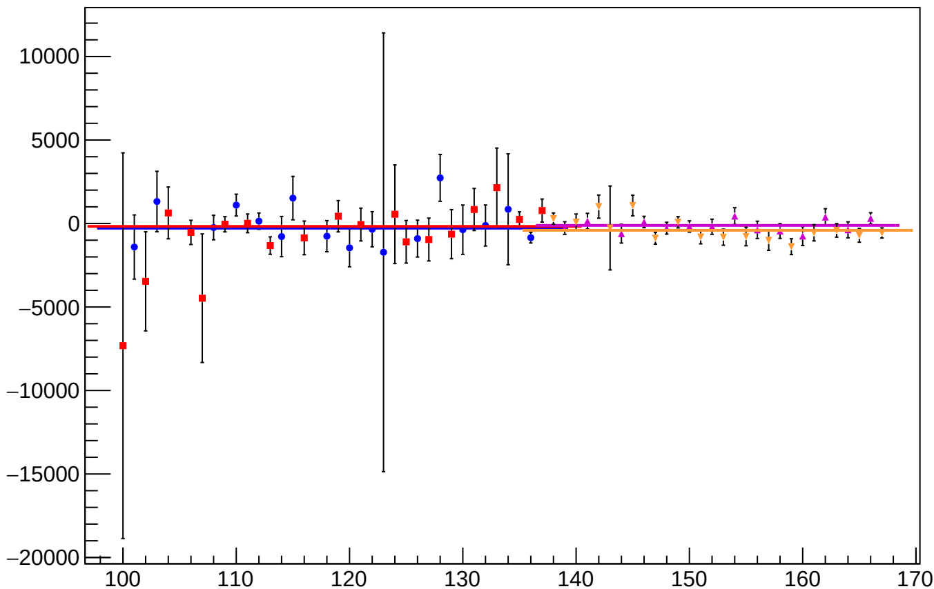
asym_atl_avg_atr_avg_dd_correction_mean vs Slug
