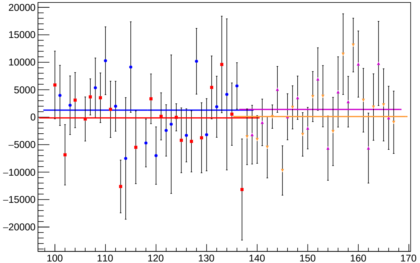
asym_atl_dd_atr_dd_avg_correction_mean vs Slug
