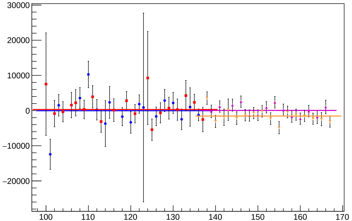
asym_atl_dd_atr_dd_dd_mean vs Slug
