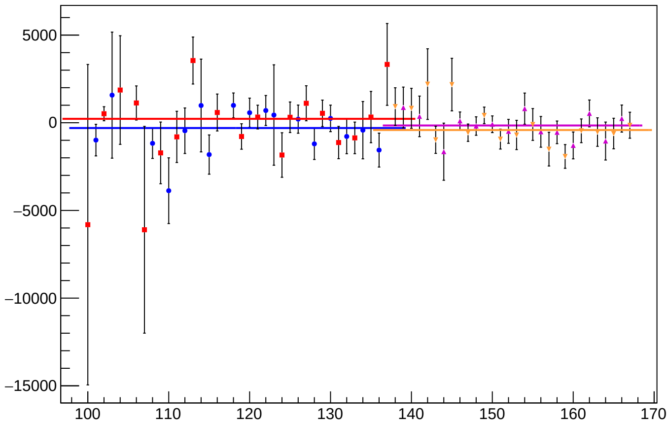
asym_at1_avg_correction_mean vs Slug
