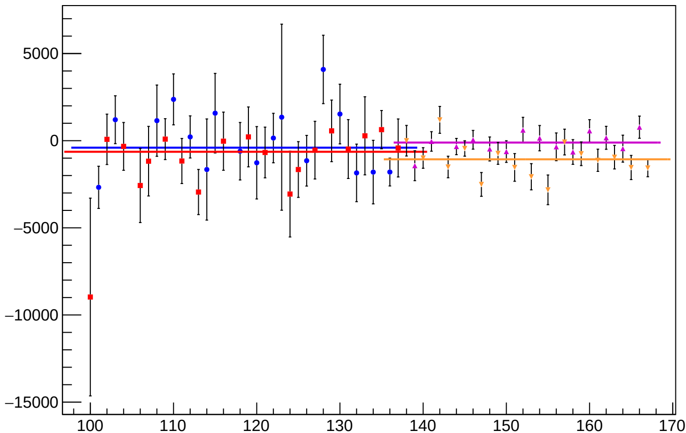
asym_sam_12345678_avg_correction_mean vs Slug
