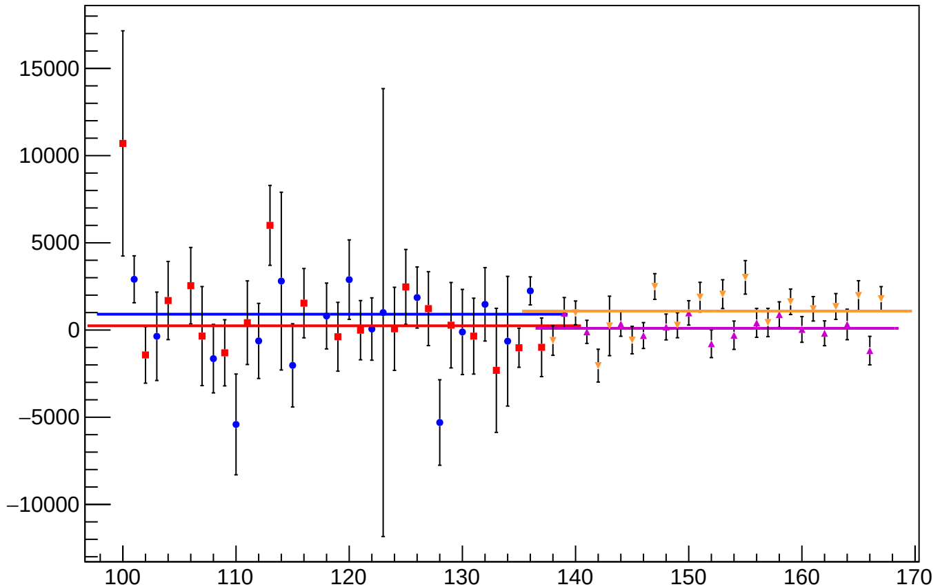
asym_atl_dd_atr_dd_dd_correction_mean vs Slug
