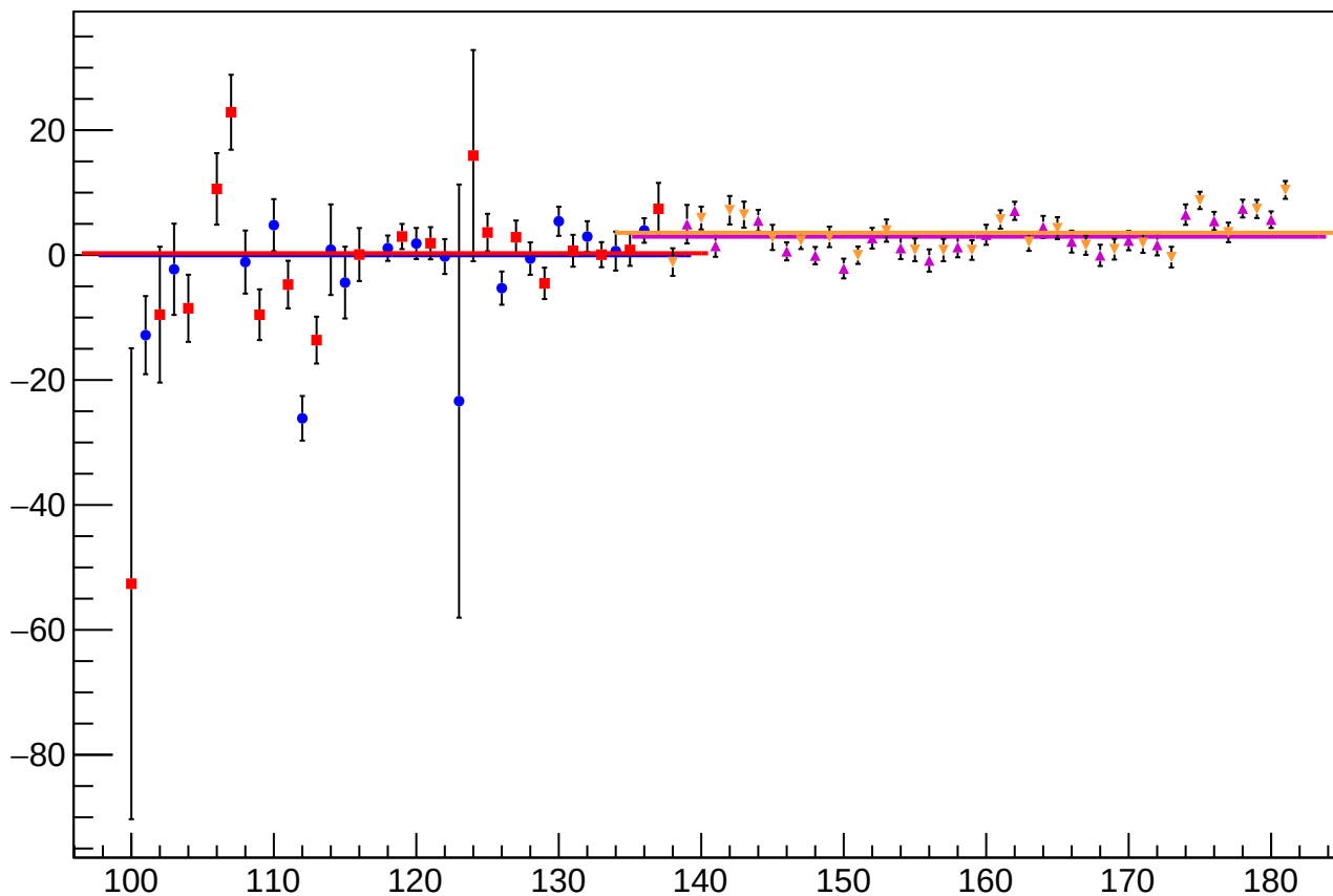
reg asym at1 dd diff bpm4eY slope vs Slug
