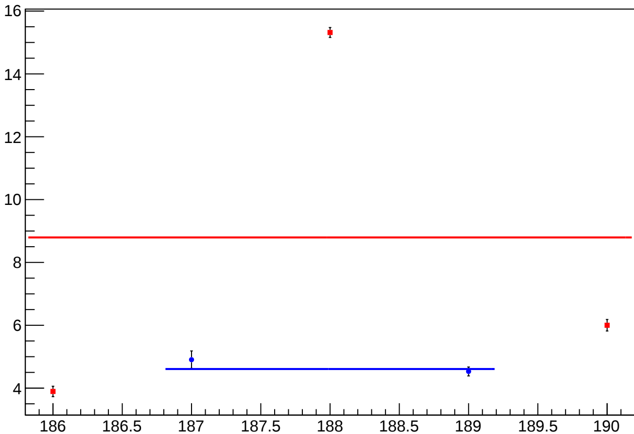
reg_asym_atl_dd_atr_dd_dd_diff_bpm12X_slope vs Slug
