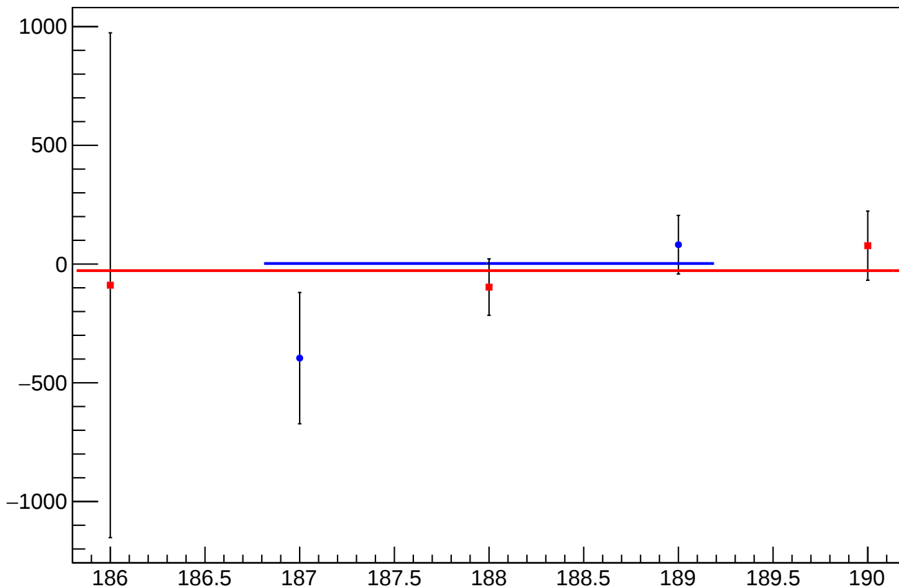
dit_asym_sam1_mean vs Slug
