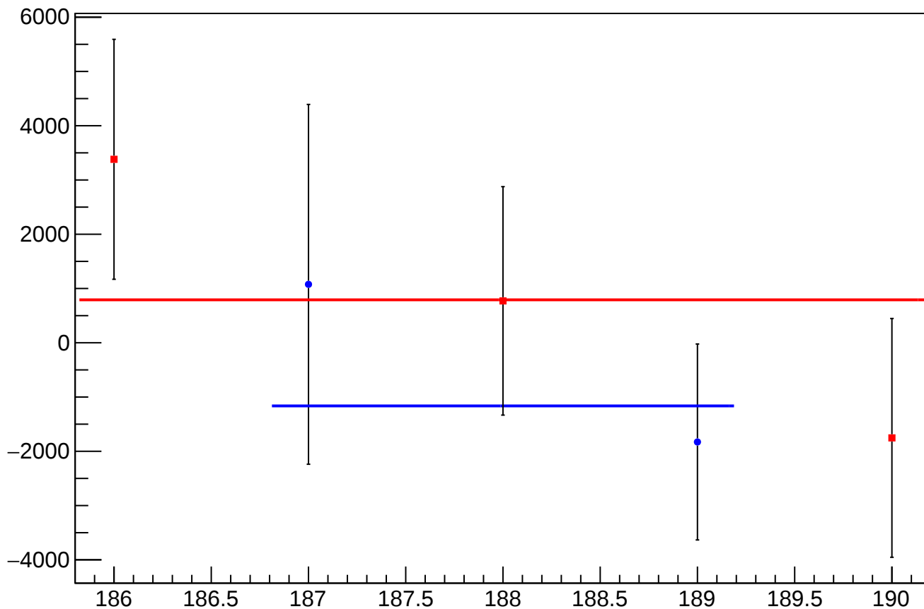
dit_asym_atl_dd_atr_dd_dd_mean vs Slug
