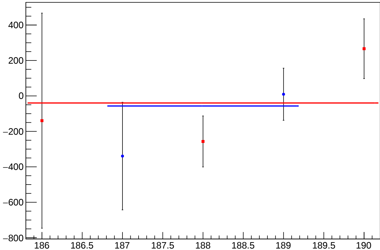
dit_asym_sam_15_dd_mean vs Slug
