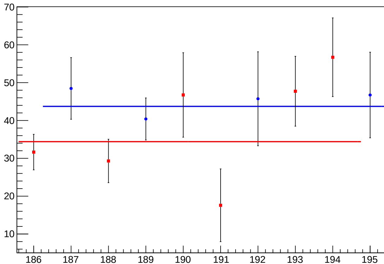
reg_asym_atl_avg_atr_avg_avg_diff_bpm4aY_slope vs Slug
