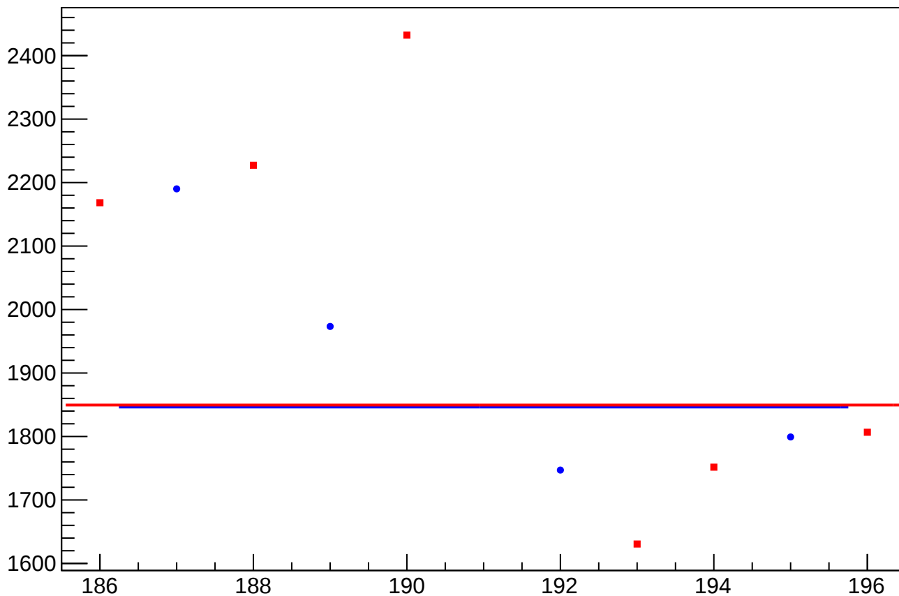
asym_us_dd_rms vs Slug, Sign Corrected
