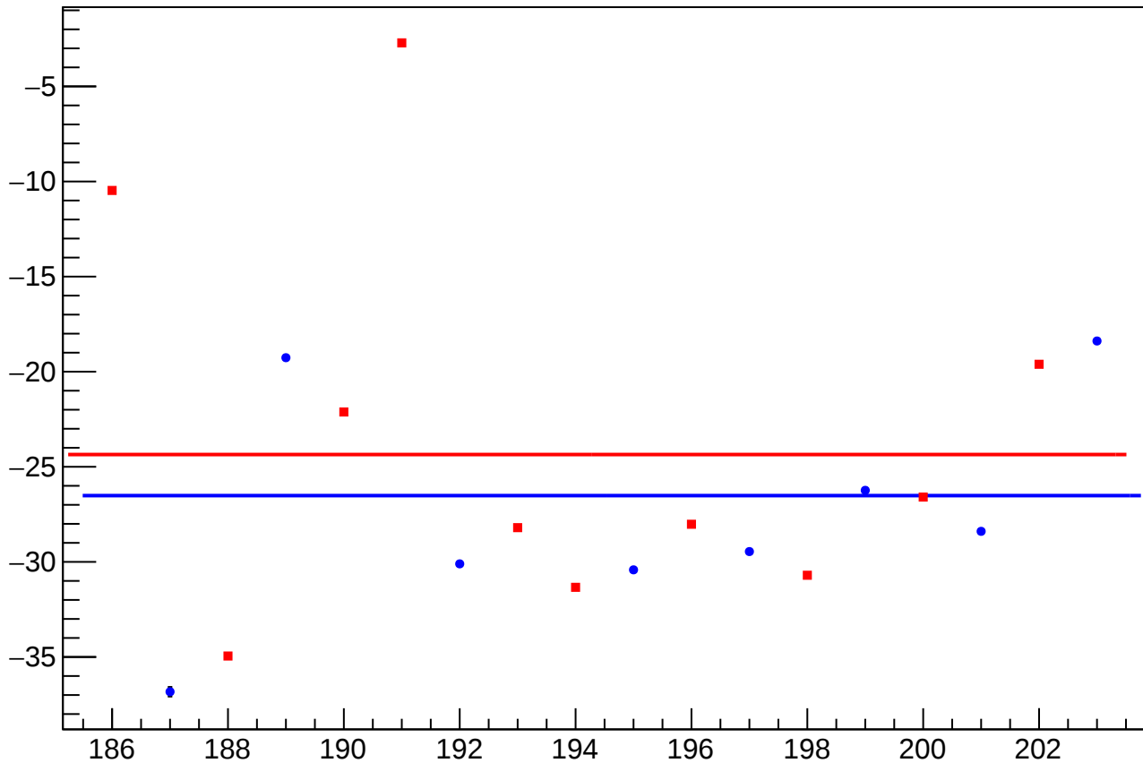
reg_asym_at1_avg_diff_bpm12X_slope vs Slug
