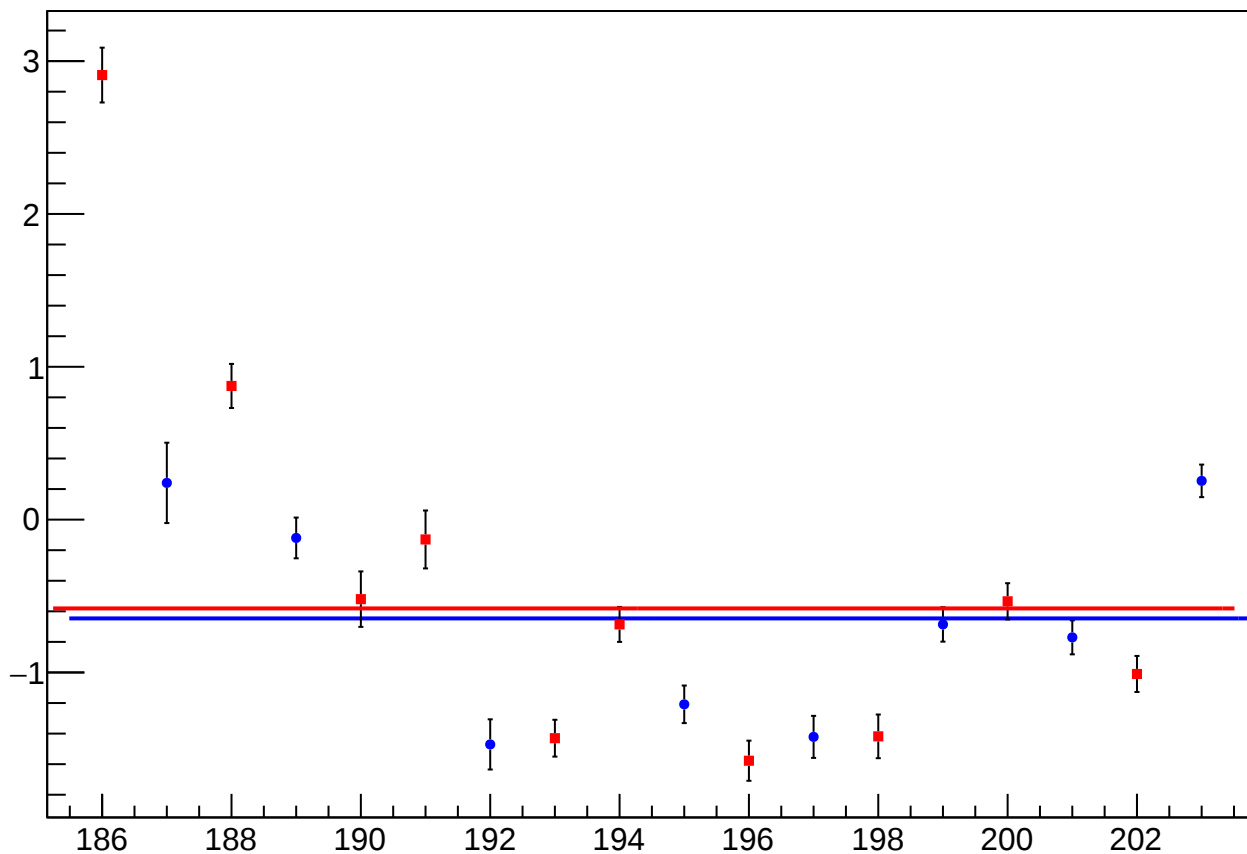
reg_asym_sam_37_avg_diff_bpm12X_slope vs Slug
