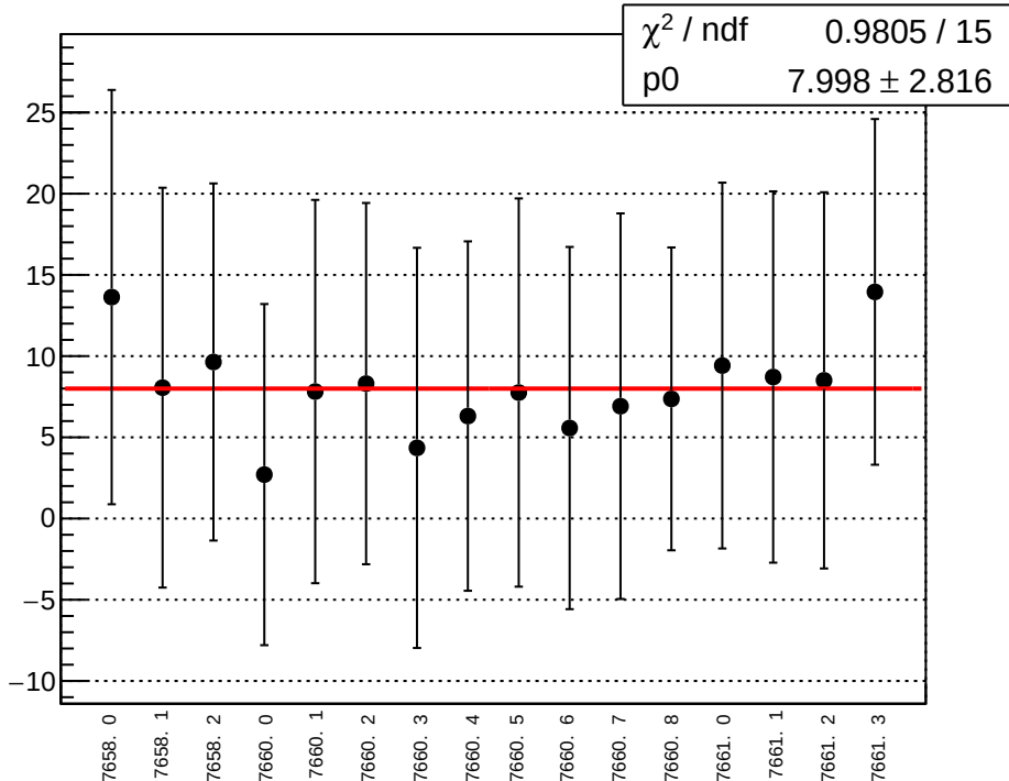
reg asym sam 12345678 avg diff bpm4aY slope vs run
