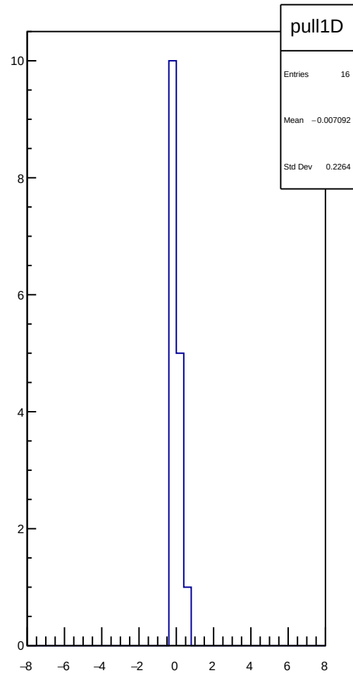
\chi^2 / \text{ndf} 0.8206 / 15 p0 13.77 \pm 11.88
