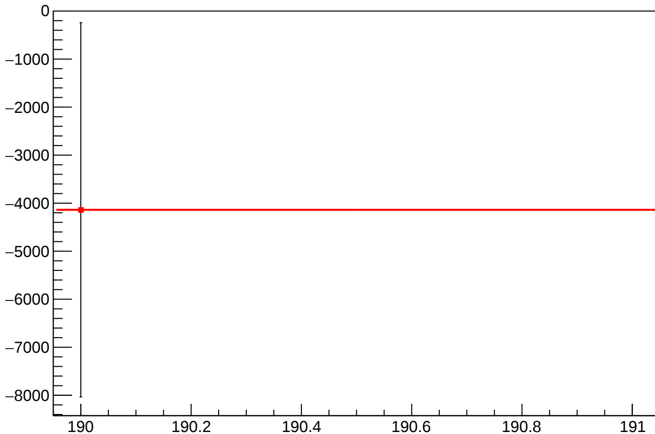
dit_asym_atr_dd_mean vs Slug, Sign Corrected
