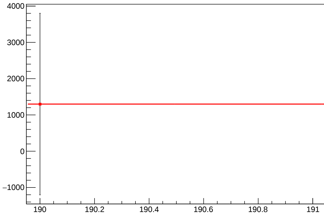
dit_asym_atl_dd_atr_dd_dd_mean vs Slug, Sign Corrected
