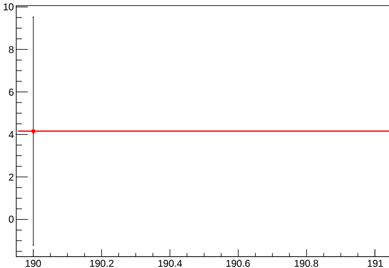
reg_asym_usl_diff_bpm4eY_slope vs Slug, Sign Corrected
