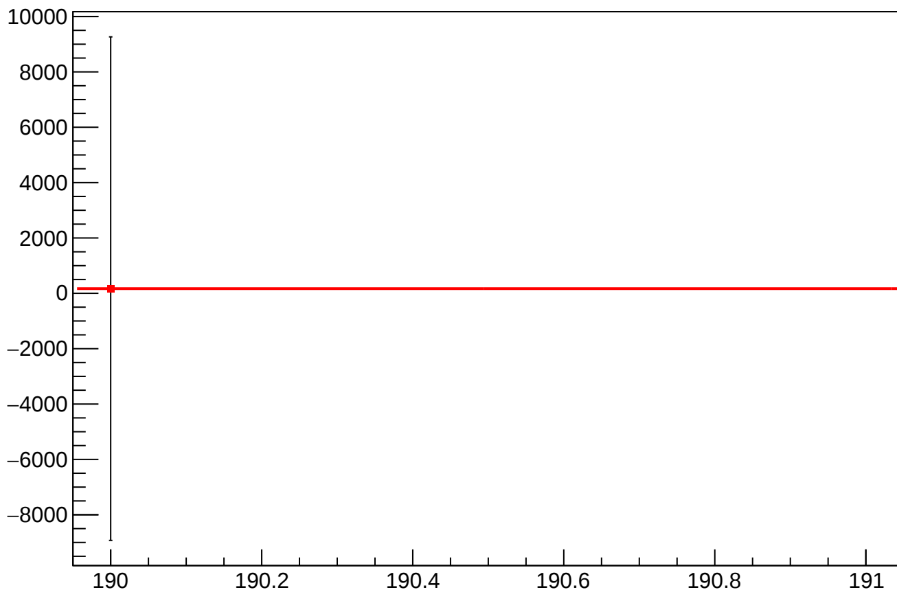
asym_usr_correction_mean vs Slug, Sign Corrected
