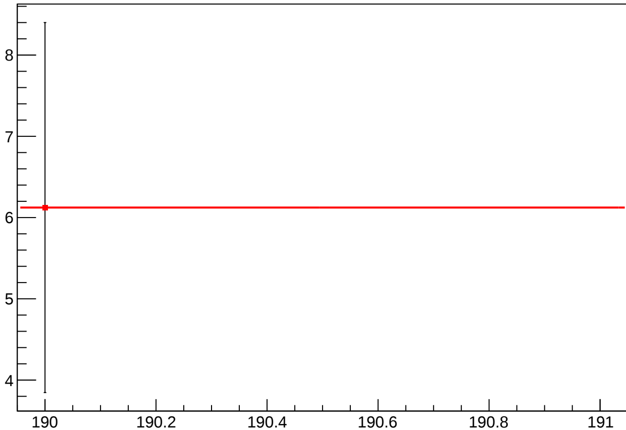
reg_asym_sam7_diff_bpm1X_slope vs Slug, Sign Corrected
