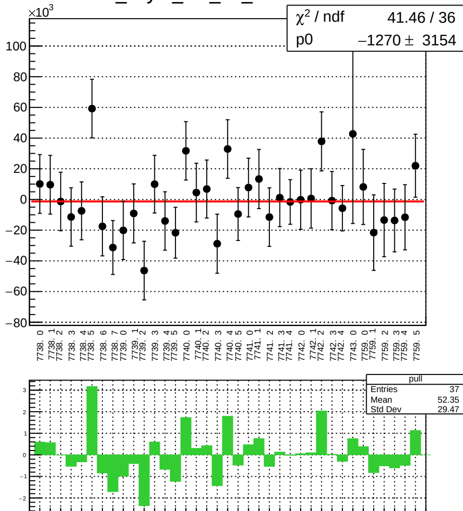
dit_asym_at1_dd_mean vs run
