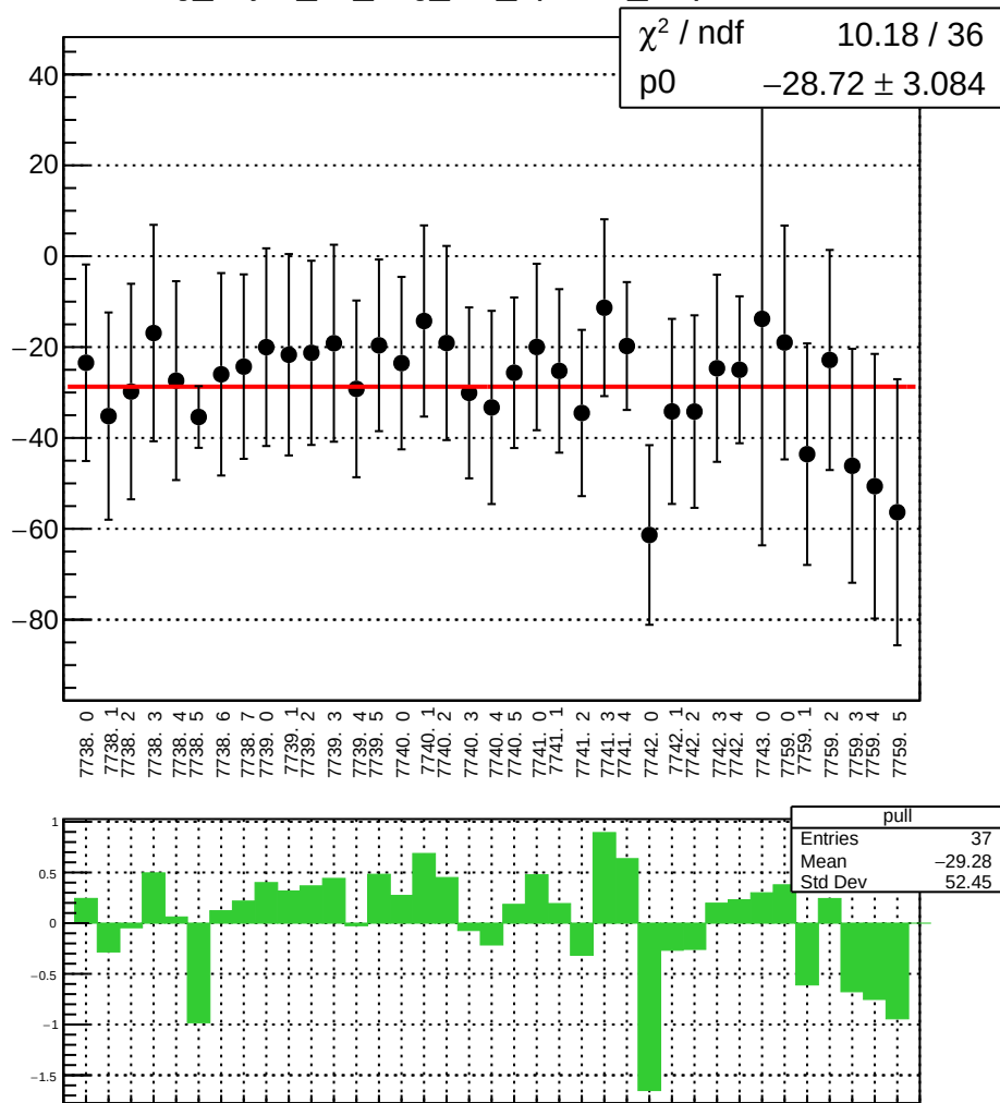
reg_asym_us_avg_diff_bpm1X_slope vs run
