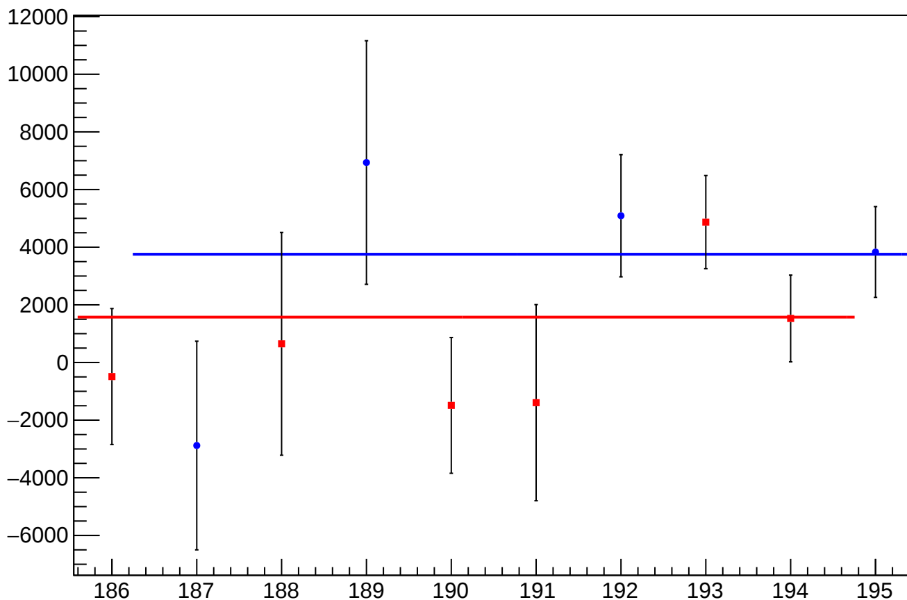
dit_asym_atl_avg_atr_avg_avg_mean vs Slug, Sign Corrected
