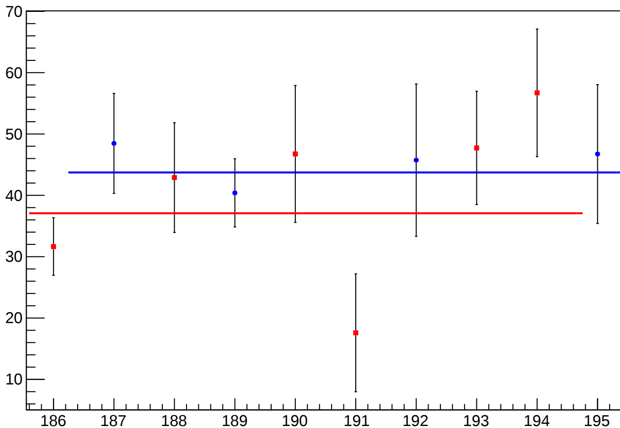
reg_asym_atl_avg_atr_avg_avg_diff_bpm4aY_slope vs Slug, Sign Corrected
