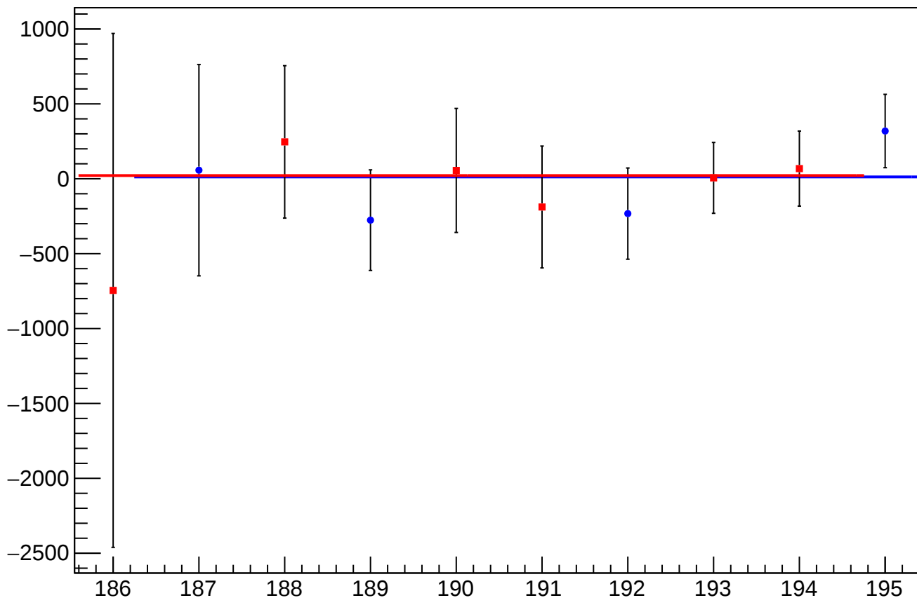
dit_asym_sam6_mean vs Slug, Sign Corrected
