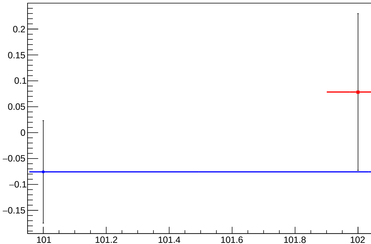
reg_asym_dsr_diff_bpm4aY_slope vs slug
