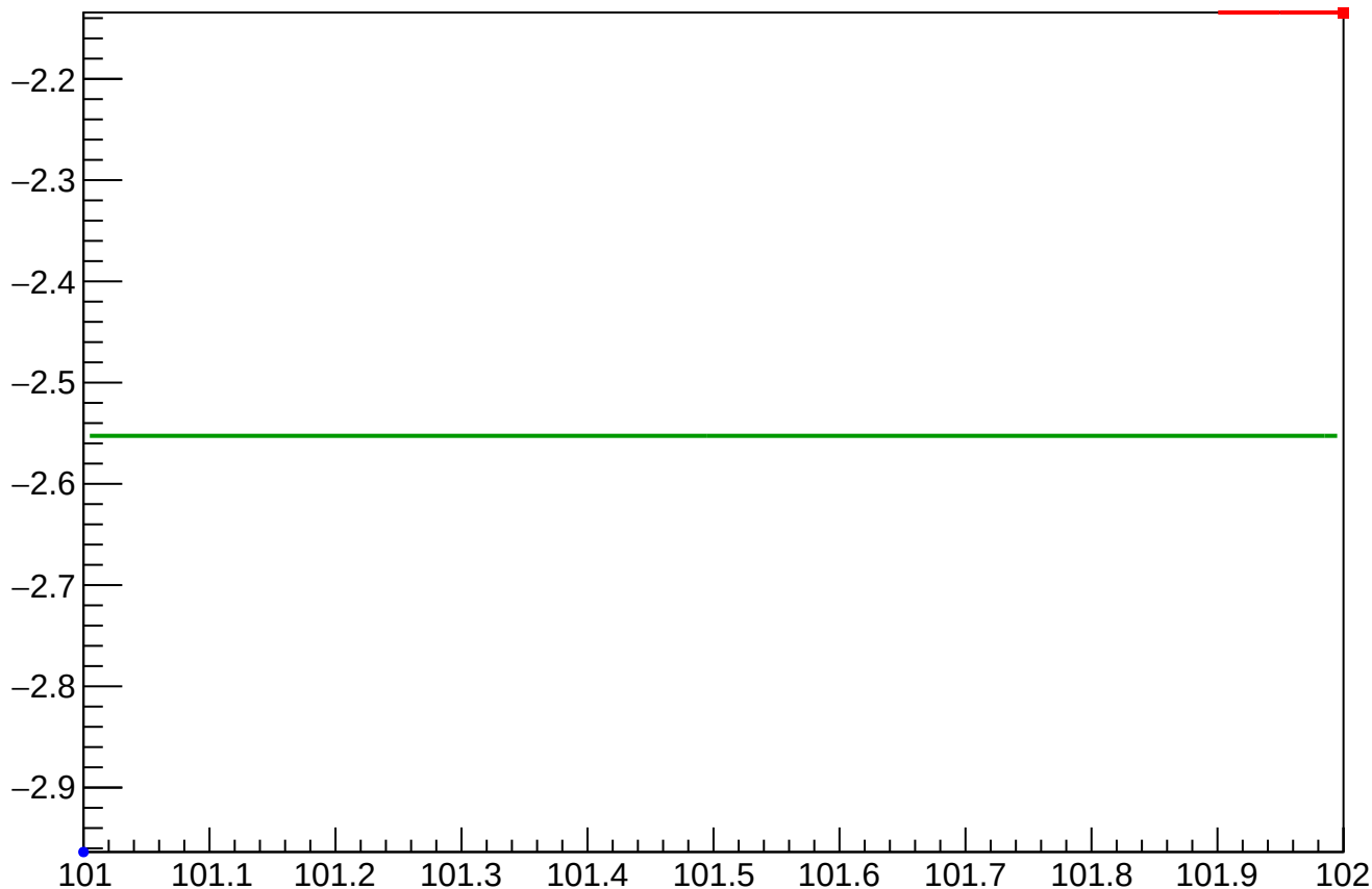
dit_4aX_coil6_mean vs Slug, Sign Corrected
