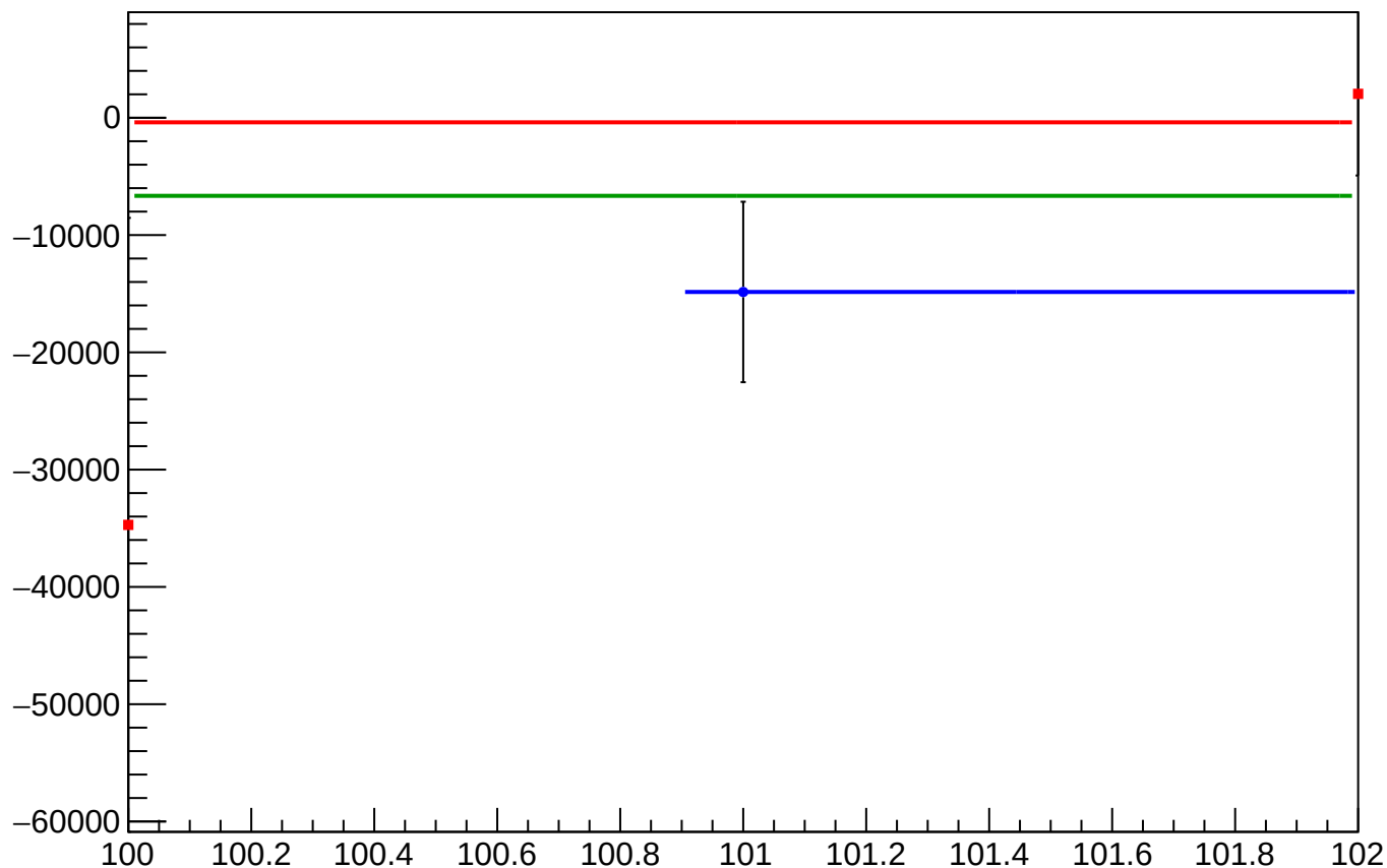
asym_at1_dd_mean vs Slug, Sign Corrected
