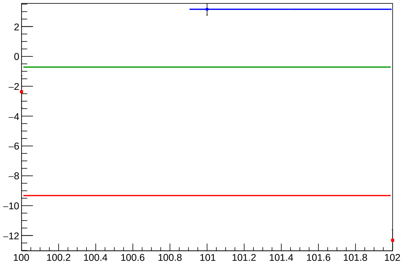
reg_asym_bcm_dg_ds_diff_bpm4aX_slope vs Slug, Sign Corrected
