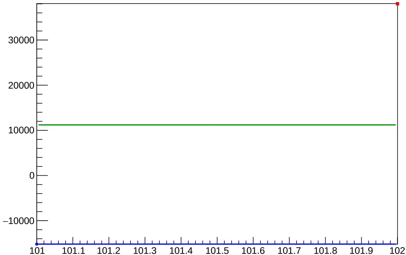
dit_atl1_coil7_mean vs Slug, Sign Corrected
