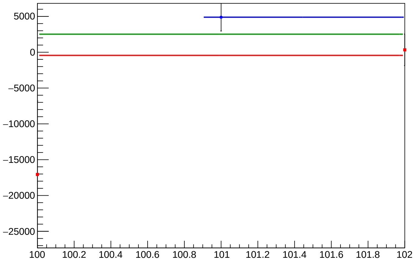
asym_sam3_mean vs Slug, Sign Corrected
