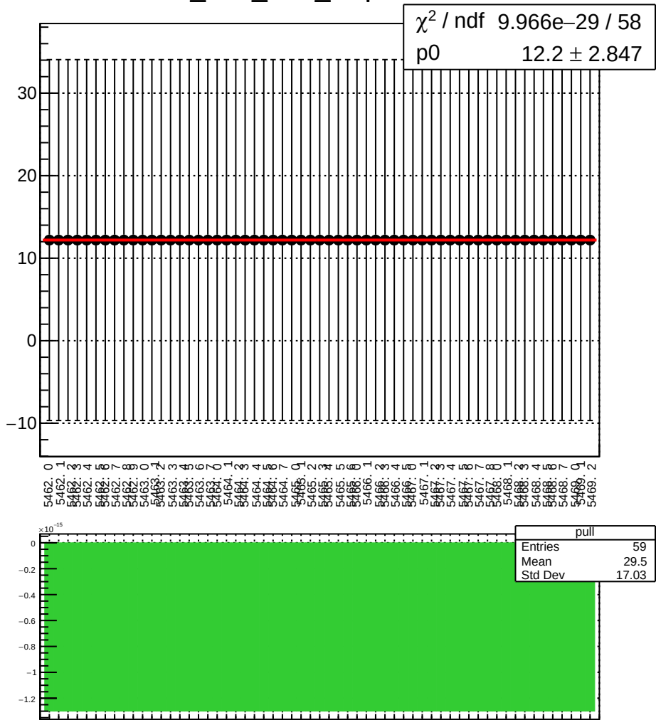
dit_atr1_4eX_slope vs run
