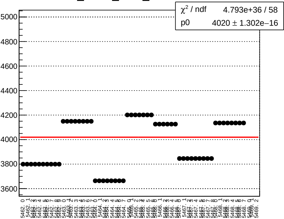
dit_sam3_coil3_mean vs run
