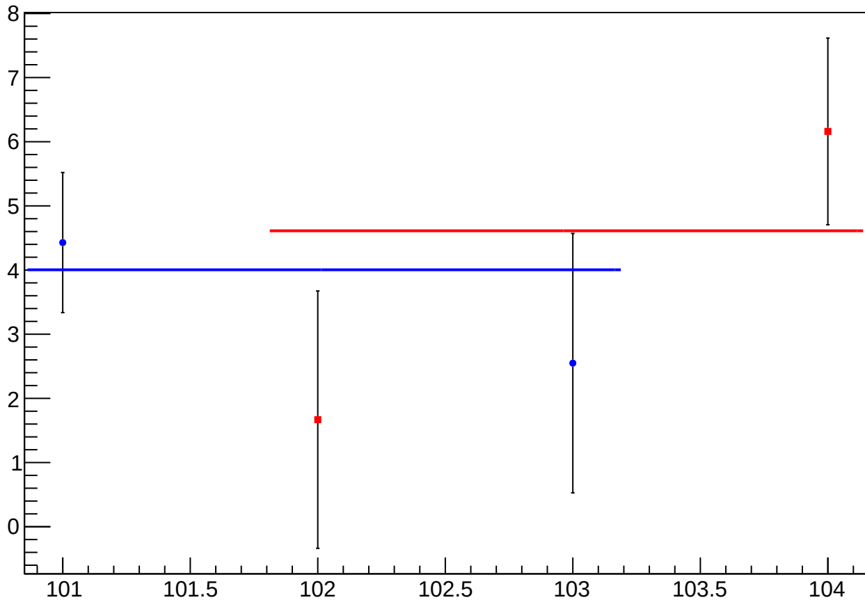
reg_asym_left_avg_diff_bpm4eY_slope vs slug
