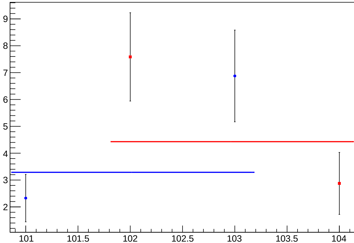
reg_asym_left_avg_diff_bpm4aY_slope vs slug
