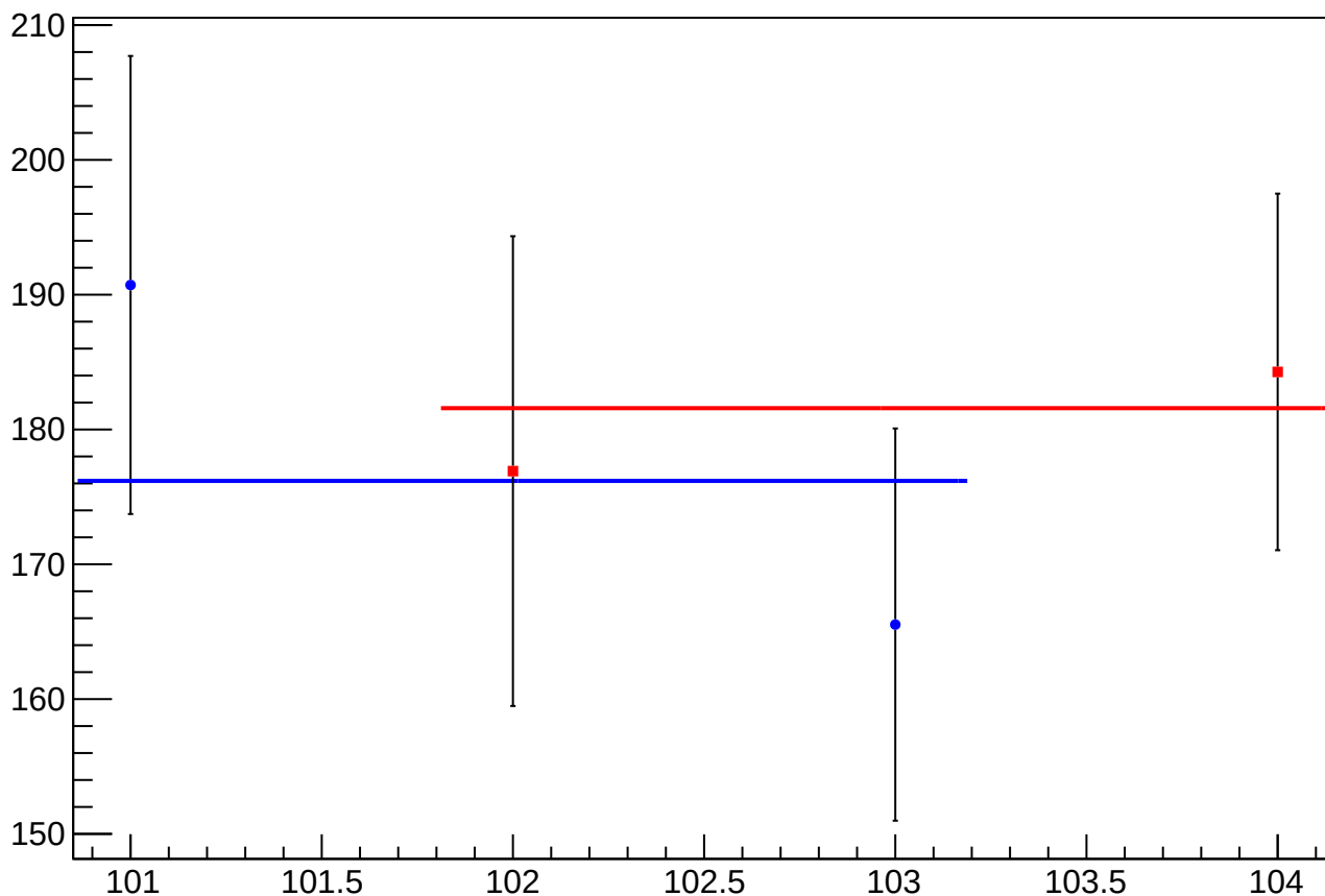
reg_asym_atl2_diff_bpm4eX_slope vs slug
