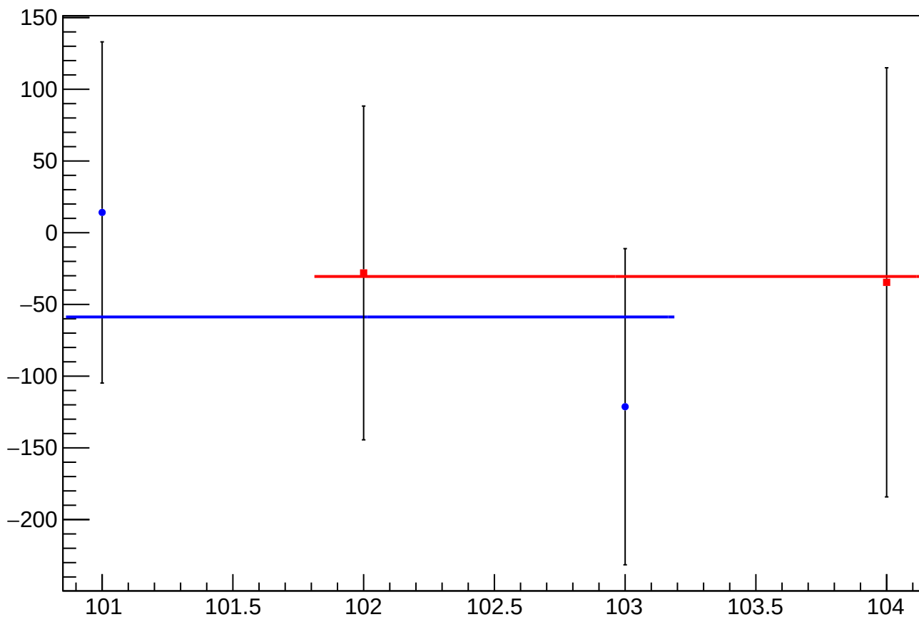
dit_asym_dsr_mean vs slug
