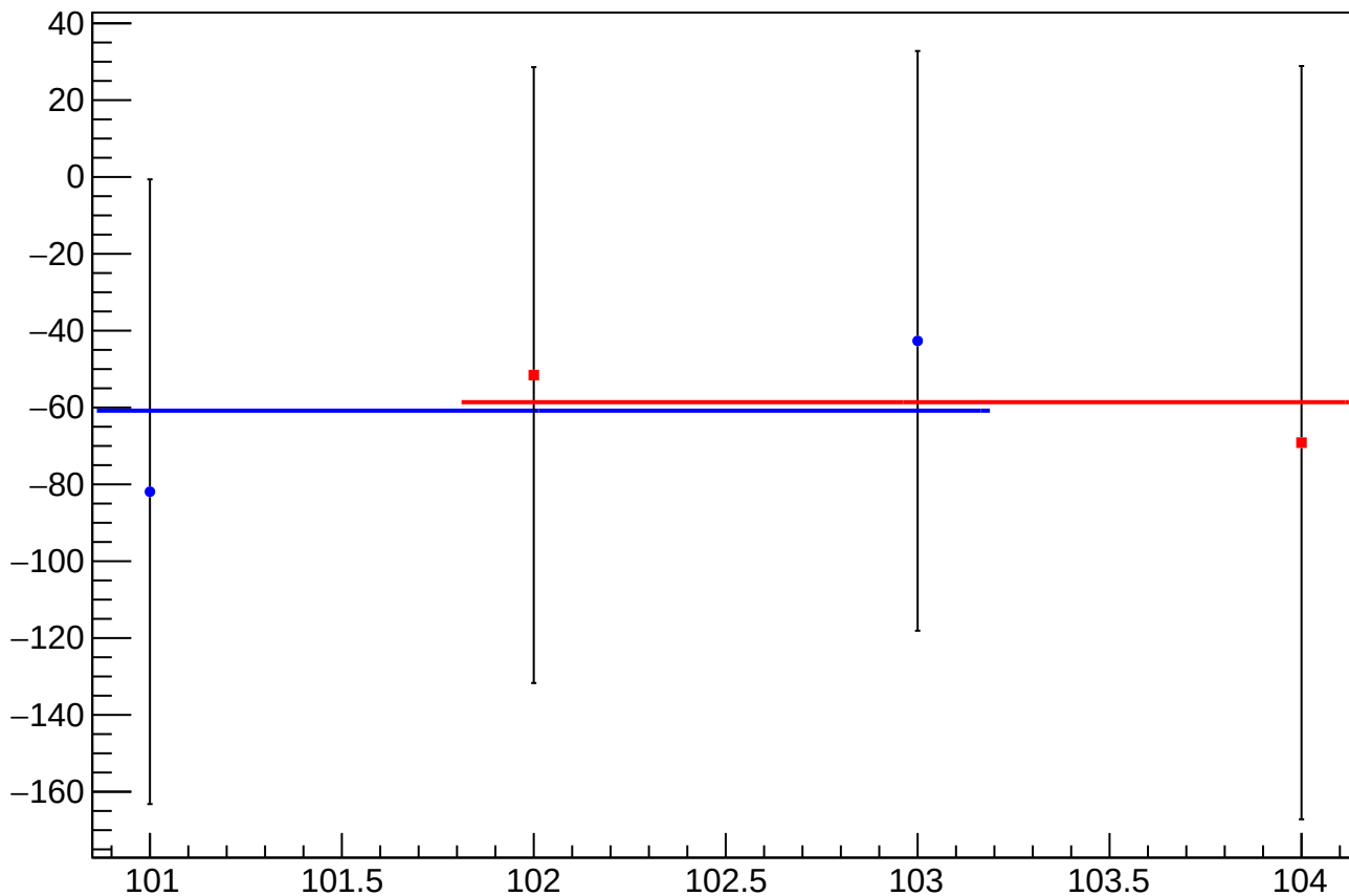
asym_ds_avg_mean vs slug
