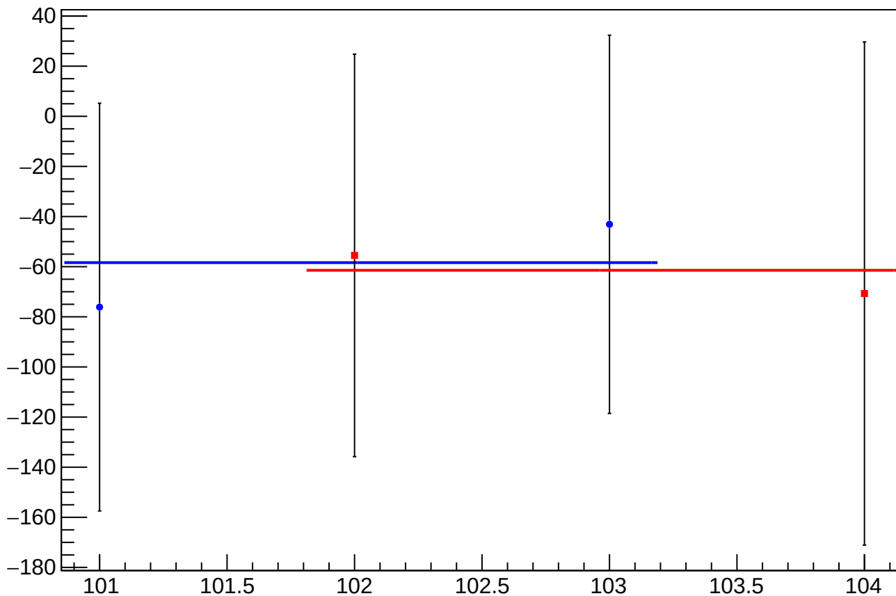
dit_asym_ds_avg_mean vs slug
