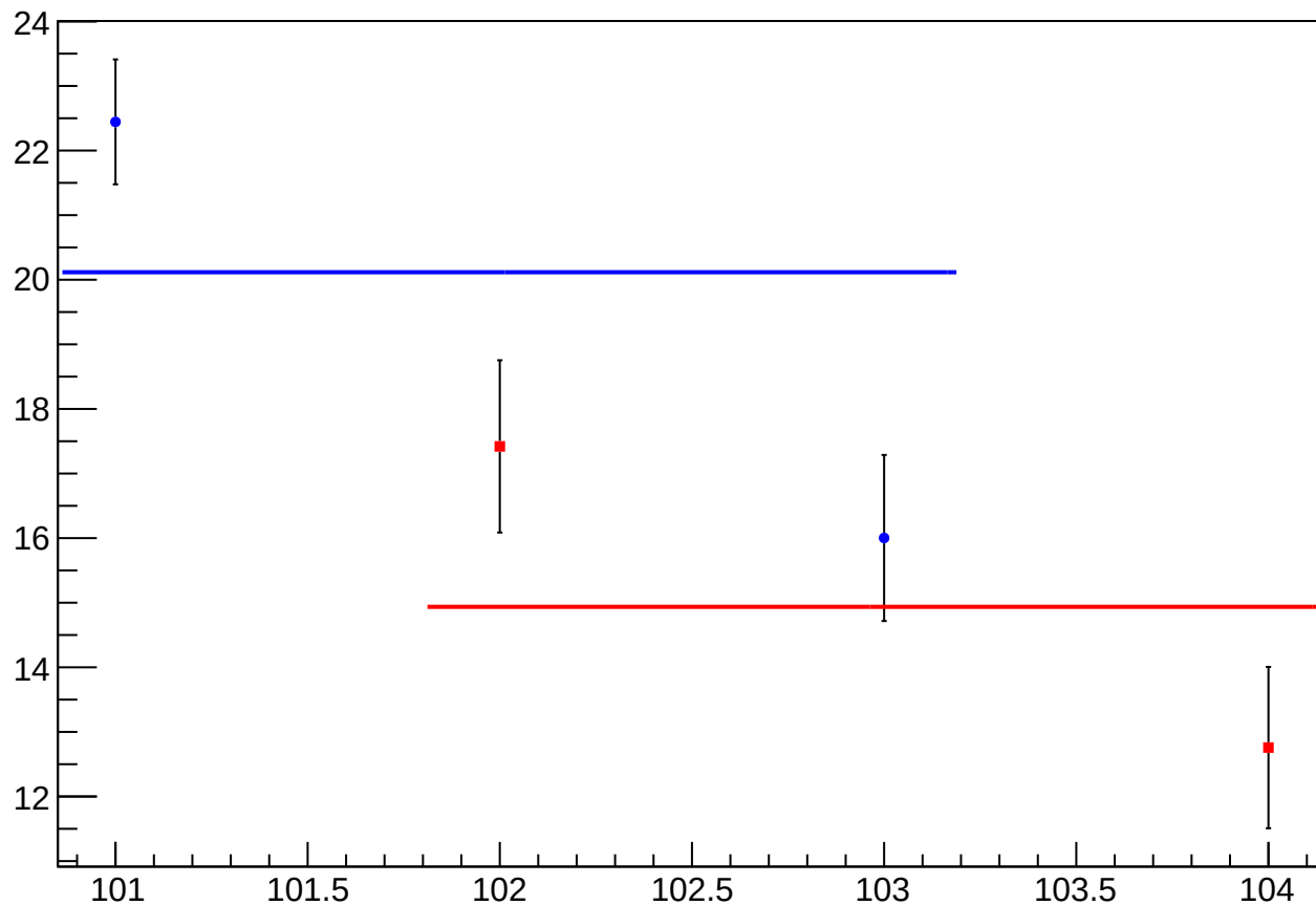
reg_asym_sam_15_37_dd_diff_bpm4aX_slope vs slug
