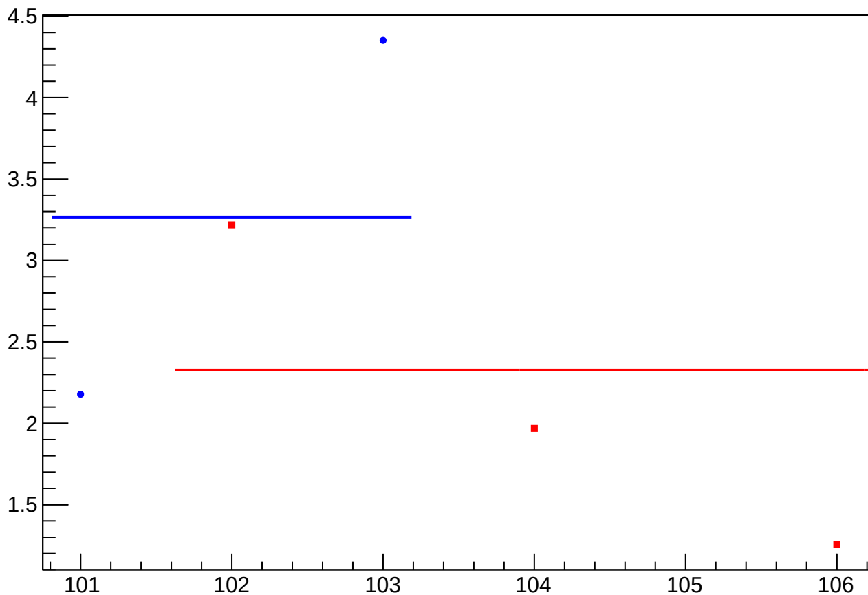
dit_4aY_coil1_err_mean vs Slug
