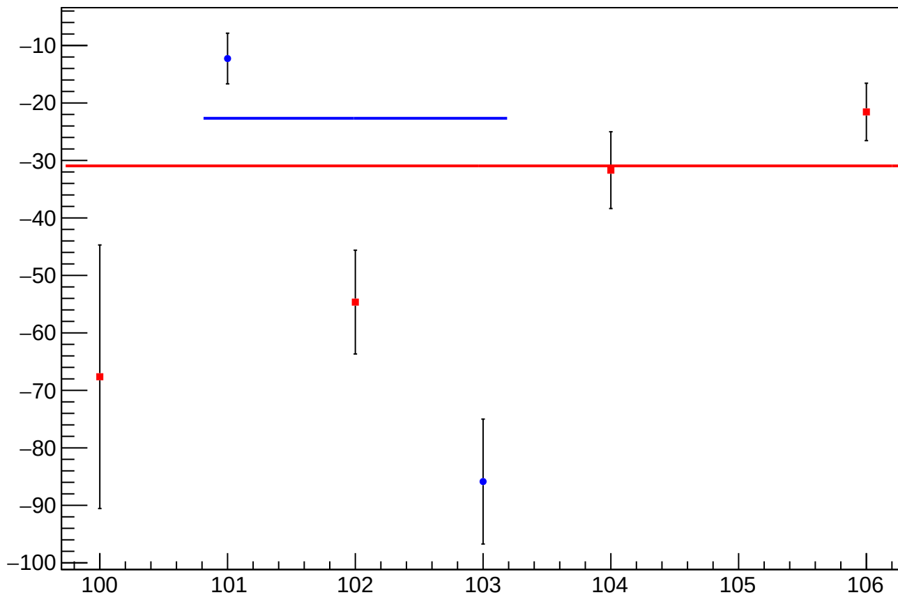
reg_asym_atl_dd_diff_bpm4aY_slope vs Slug
