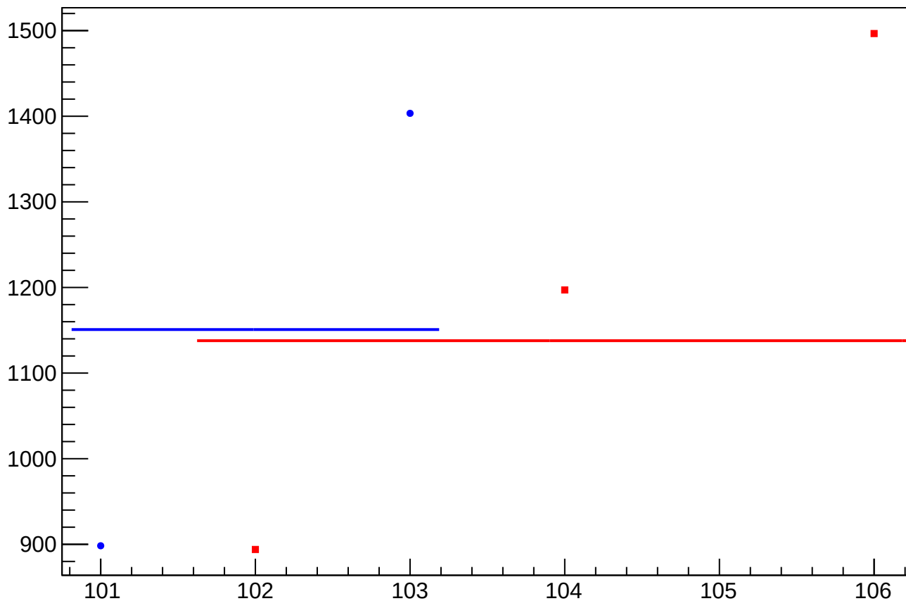
dit_sam7_coil4_Ndata_mean vs Slug
