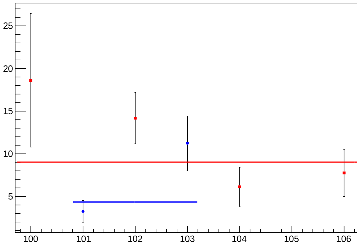
reg_asym_usl_diff_bpm4aY_slope vs Slug
