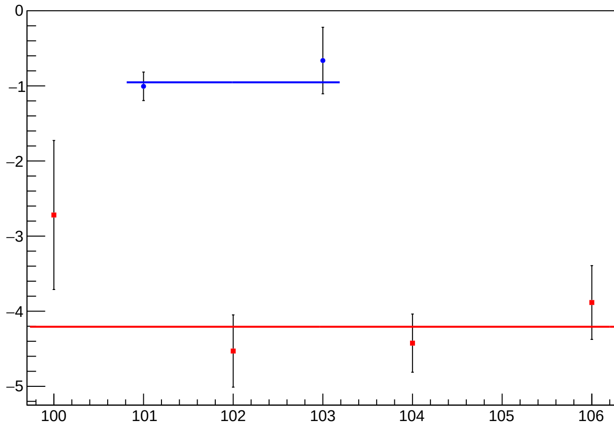
reg_asym_bcm_an_ds_diff_bpm4aY_slope vs Slug
