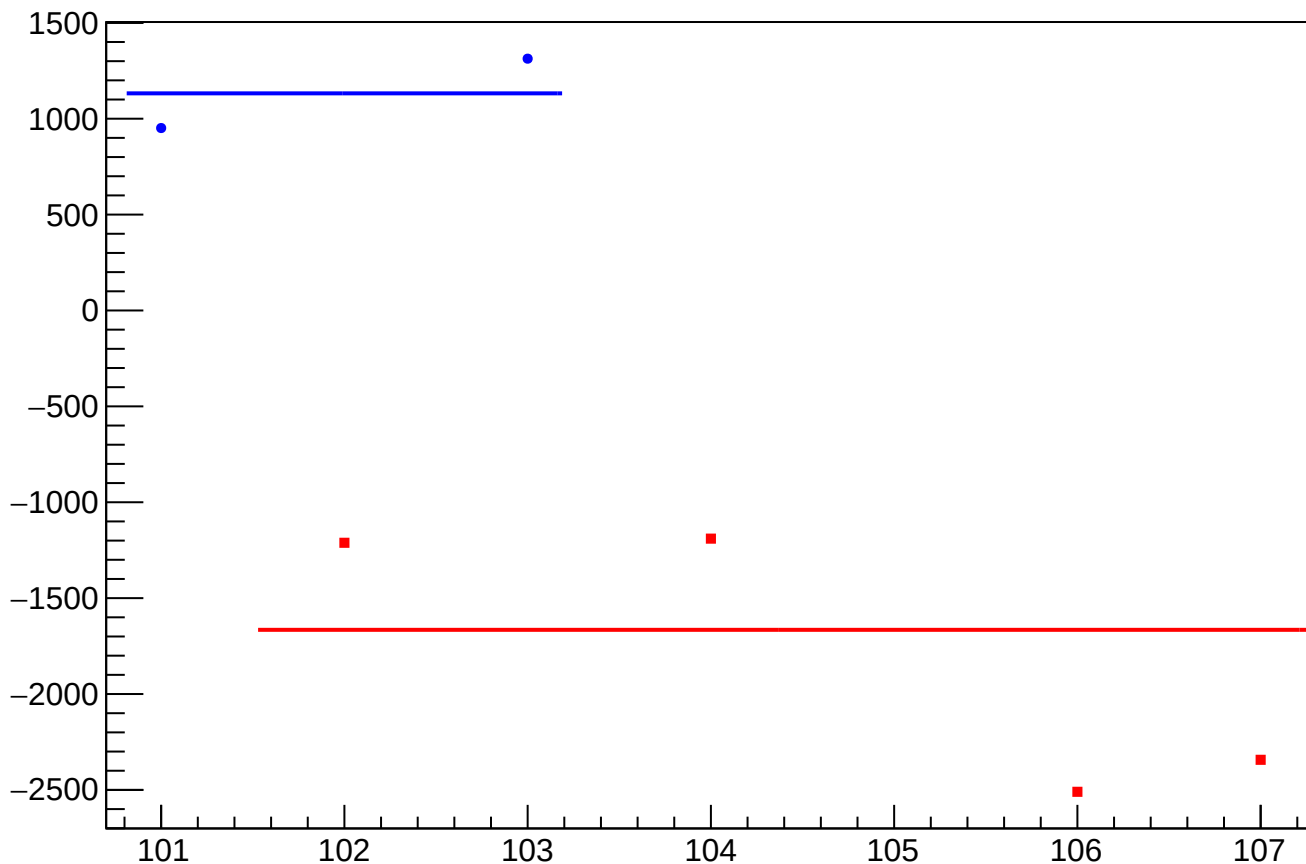
dit_sam3_coil4_mean vs Slug, Sign Corrected
