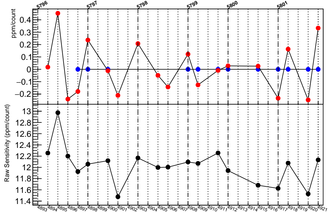
Residual Sensitivity in us1_coil1
