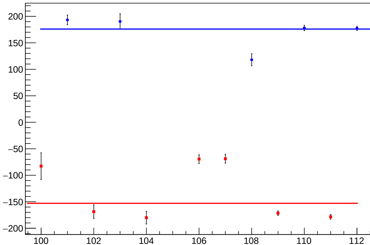
reg_asym_atl_dd_diff_bpm4aX_slope vs Slug, Sign Corrected
