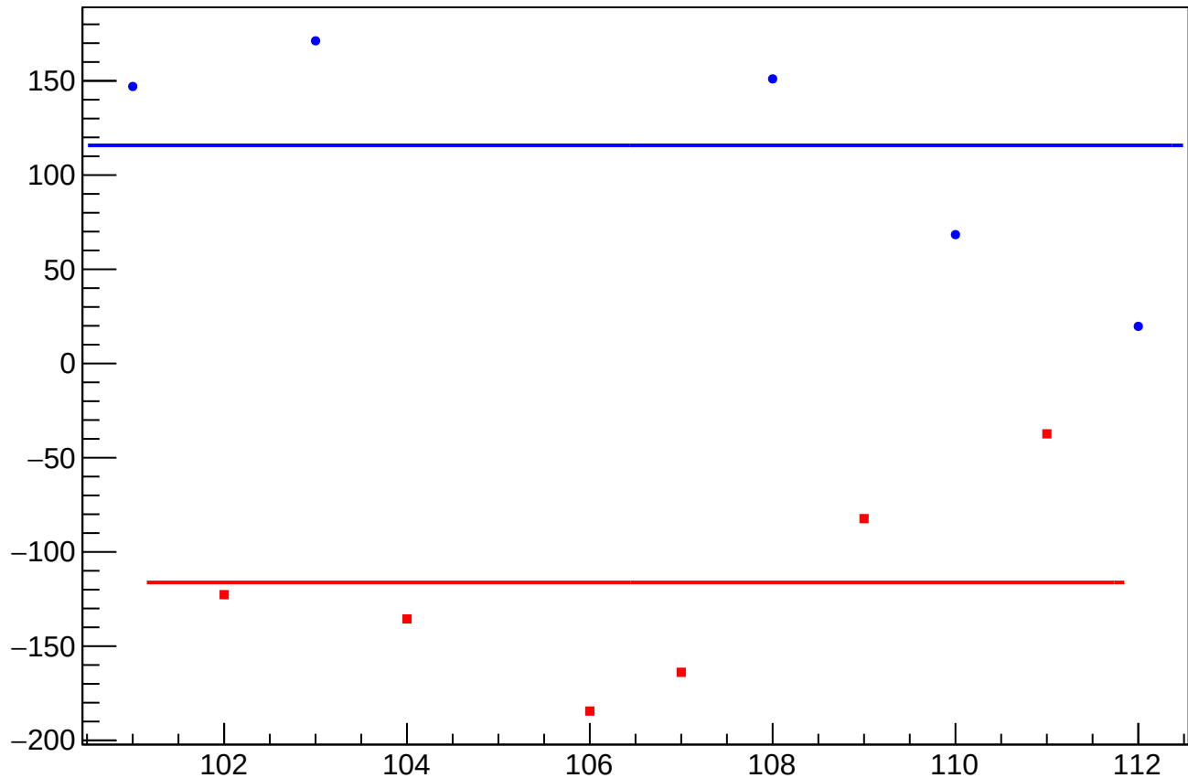
dit_sam8_coil4_err_mean vs Slug, Sign Corrected
