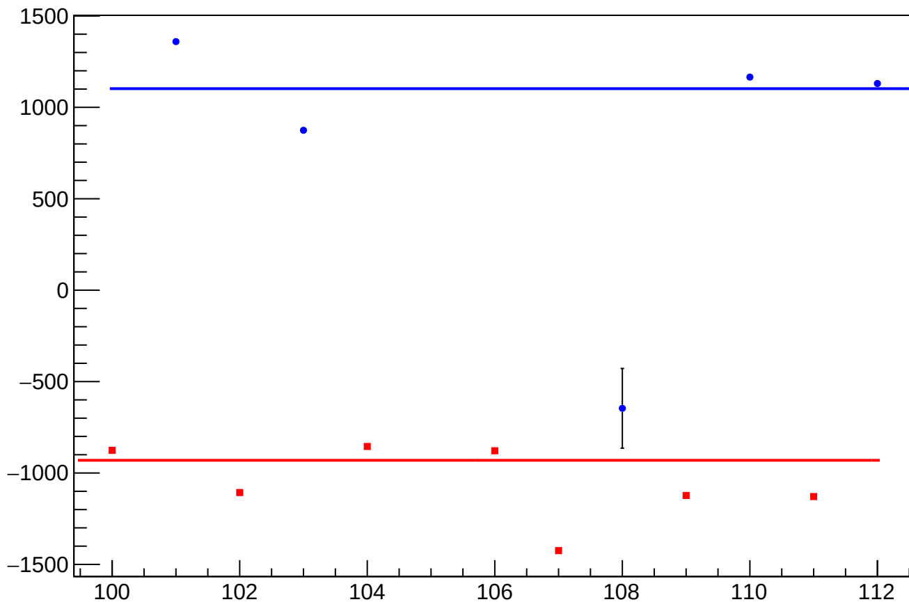
dit_atl2_4eX_slope vs Slug, Sign Corrected
