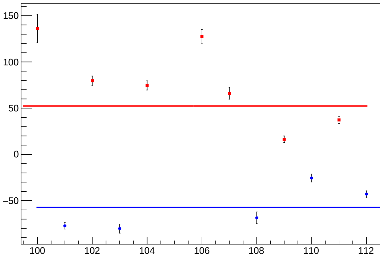
reg_asym_sam_26_avg_diff_bpm4aX_slope vs Slug, Sign Corrected
