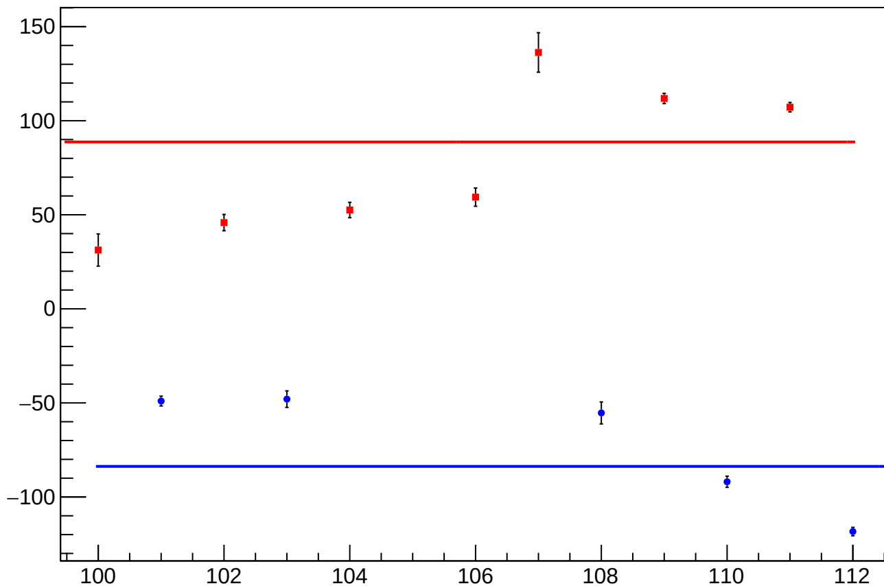
reg_asym_usl_diff_bpm4aX_slope vs Slug, Sign Corrected
