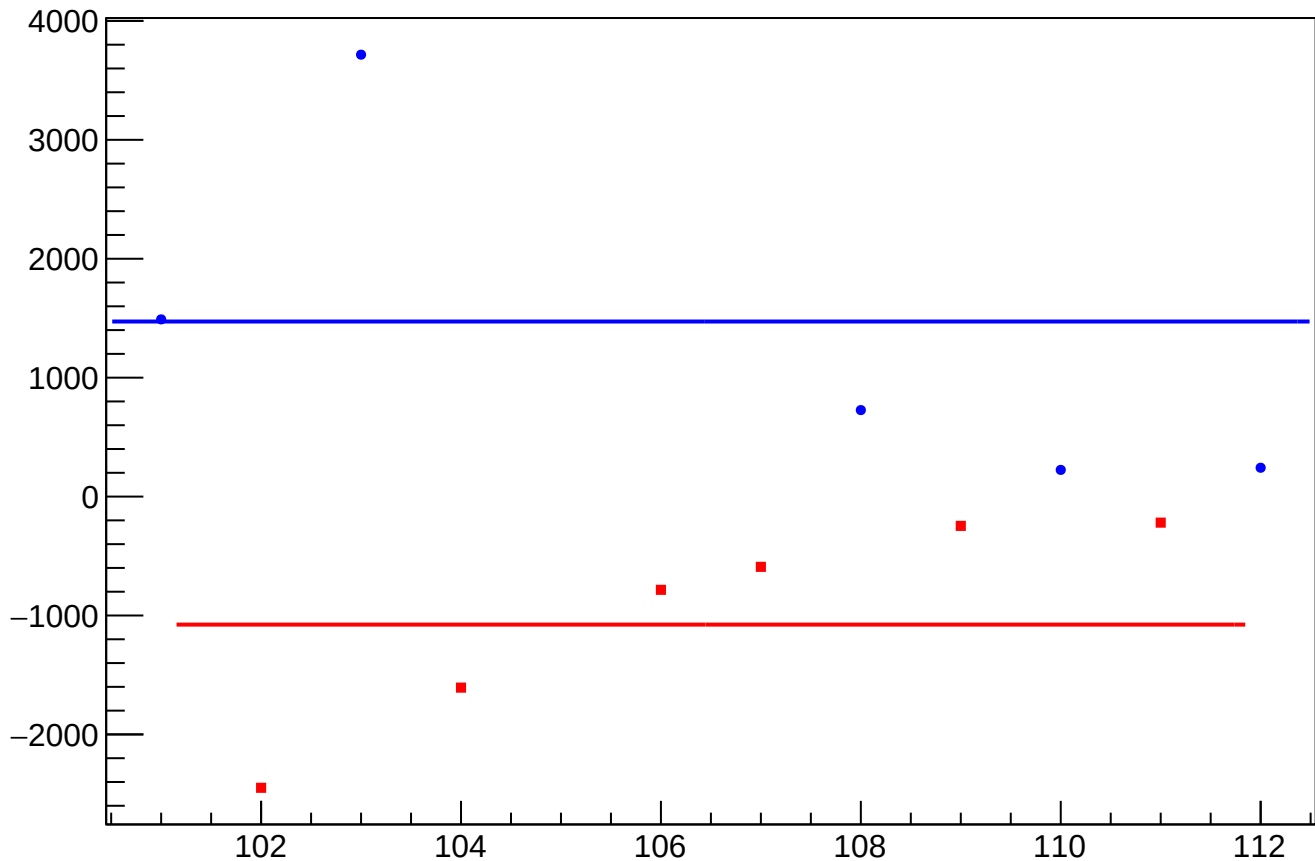
dit_sam4_coil6_err_mean vs Slug, Sign Corrected
