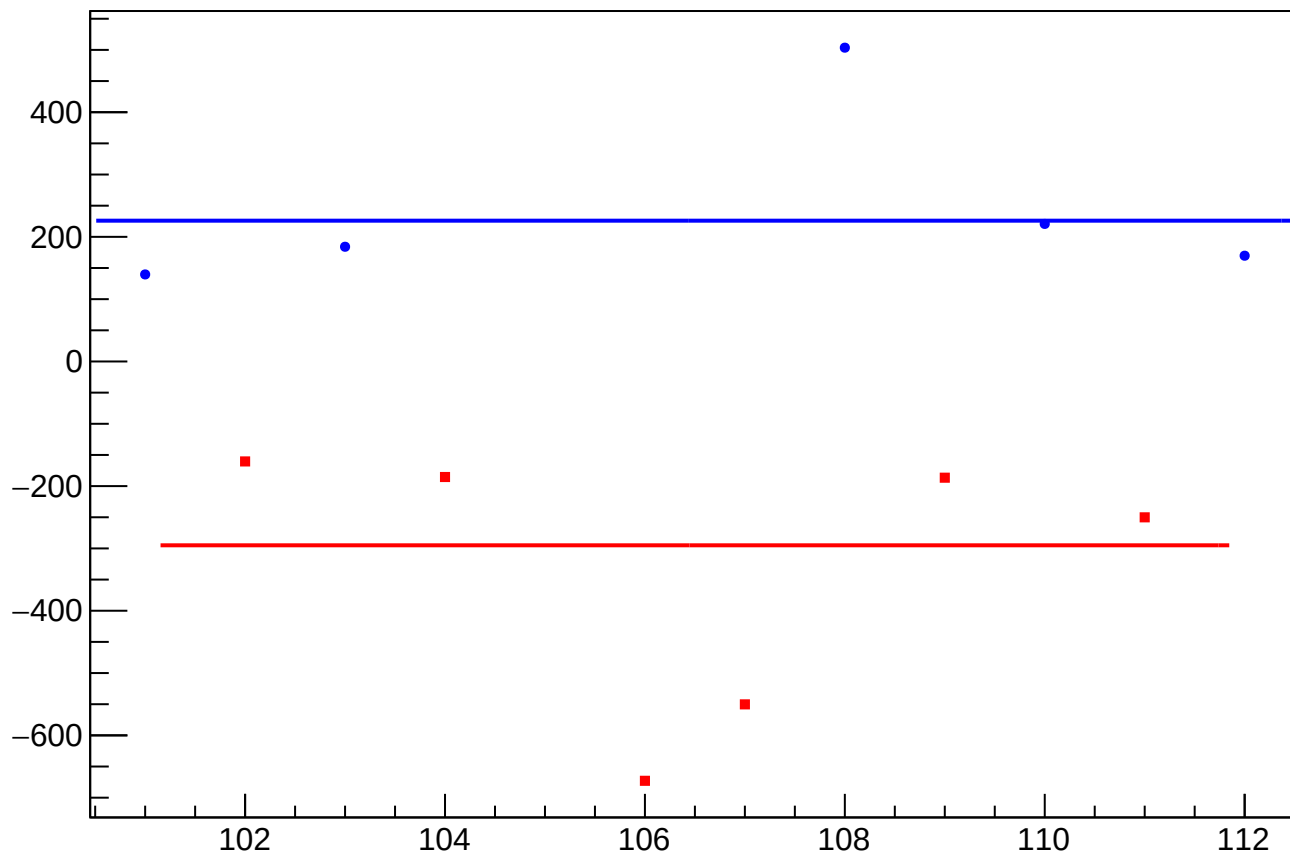
dit_sam5_coil3_mean vs Slug, Sign Corrected
