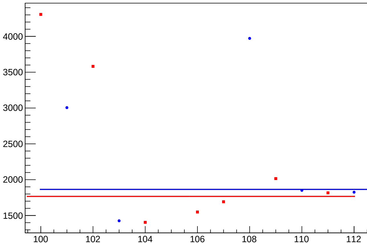
dit_asym_at2_avg_rms vs Slug, Sign Corrected
