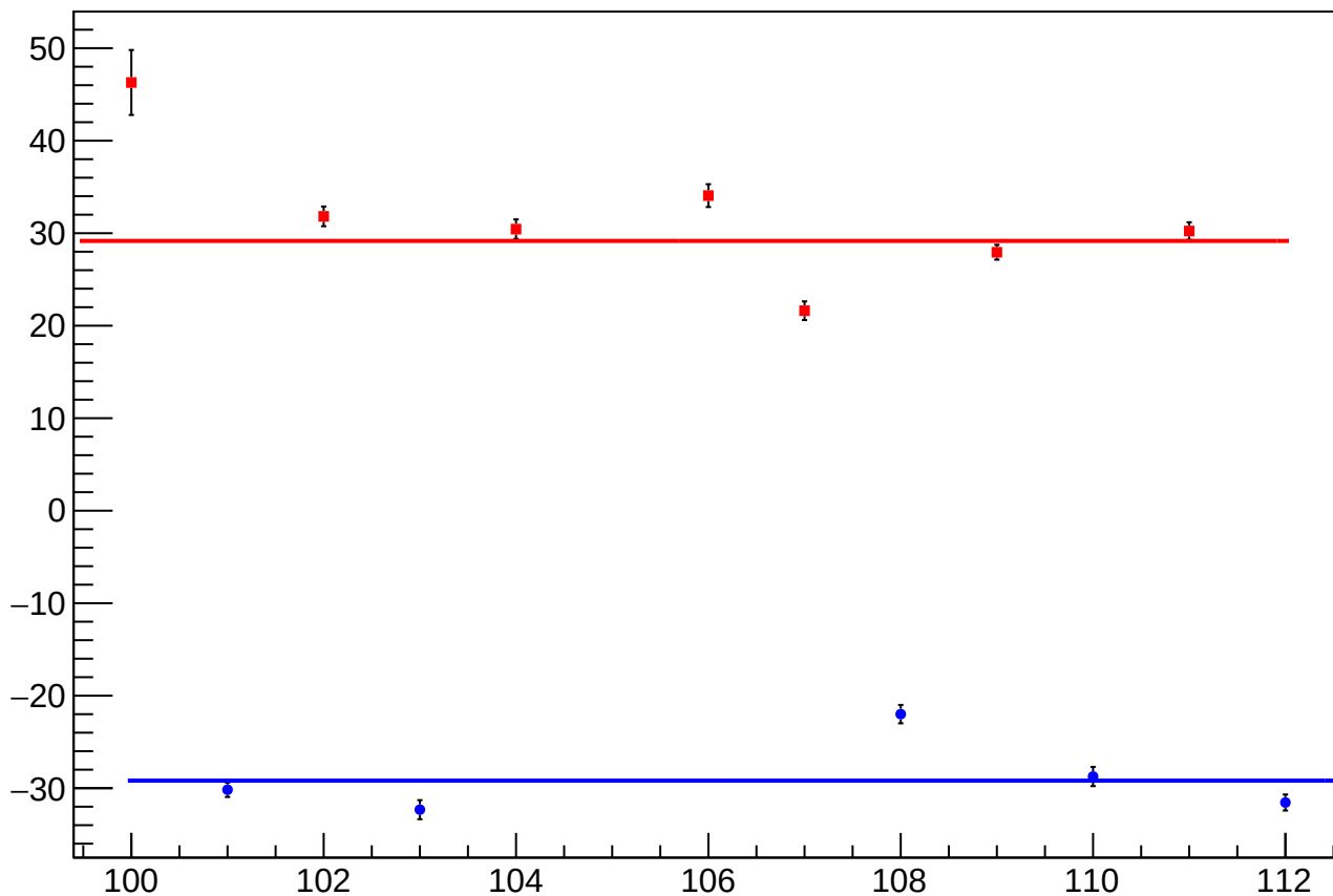
reg_asym_sam_13_57_dd_diff_bpm4aX_slope vs Slug, Sign Corrected
