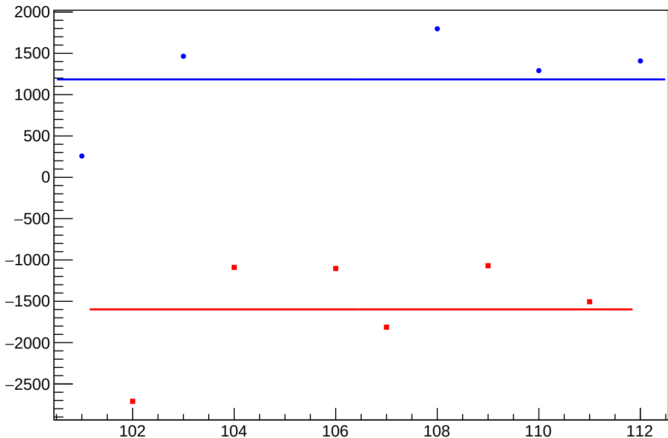
dit_atr1_coil3_mean vs Slug, Sign Corrected
