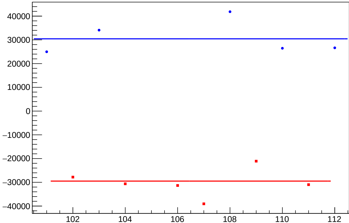
dit_sam4_coil1_mean vs Slug, Sign Corrected
