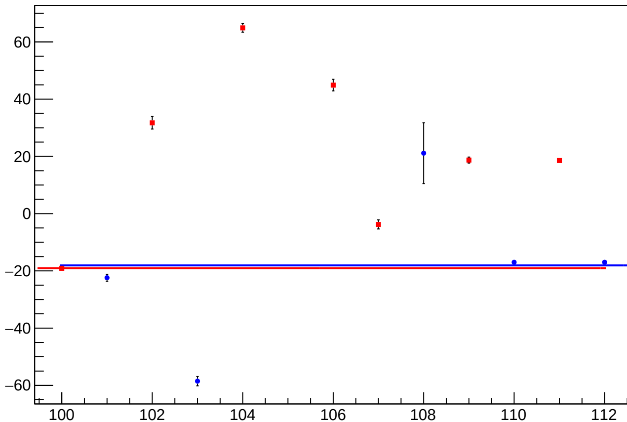
dit_atl1_4eY_slope vs Slug, Sign Corrected
