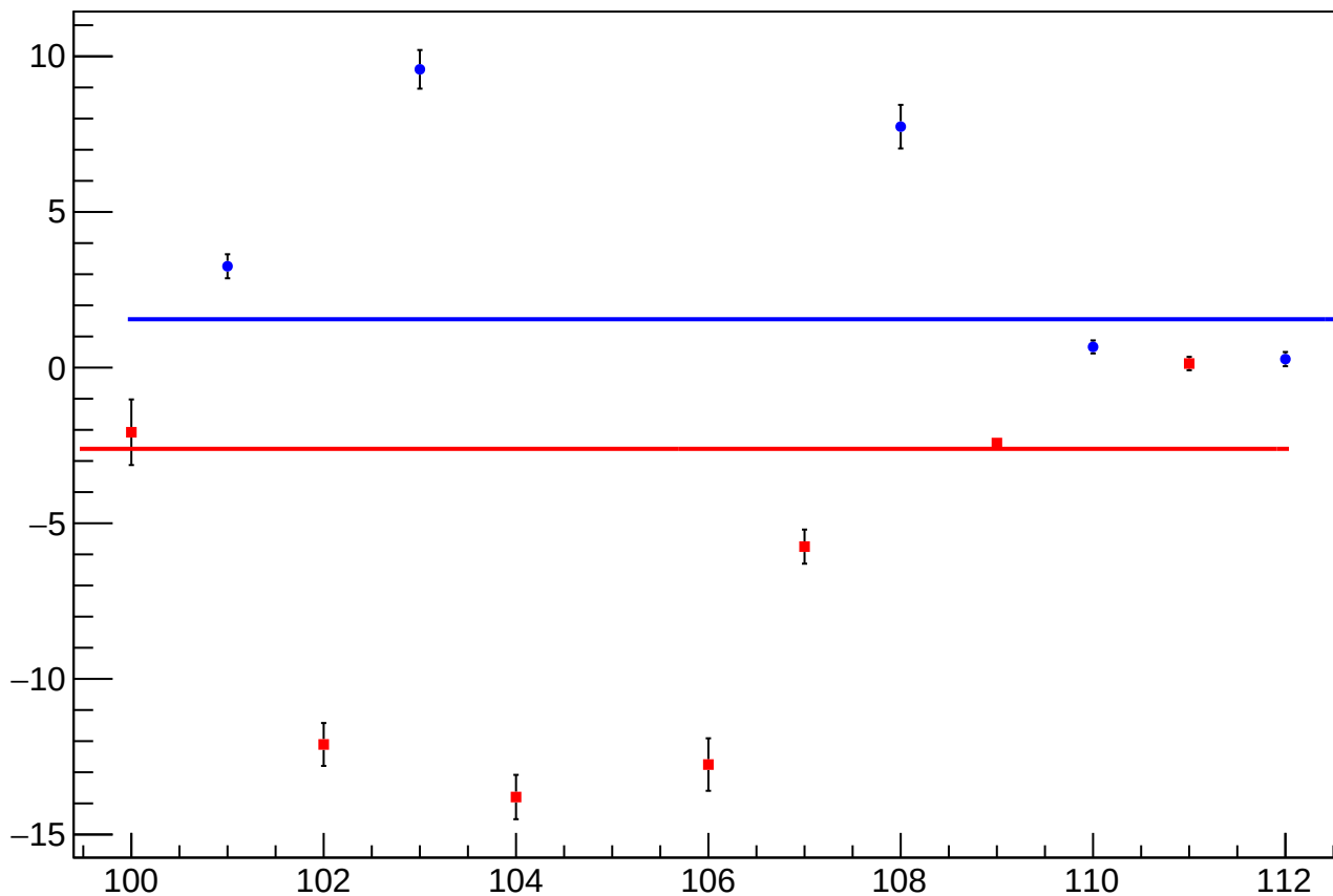
reg_asym_bcm_an_us_diff_bpm4aX_slope vs Slug, Sign Corrected
