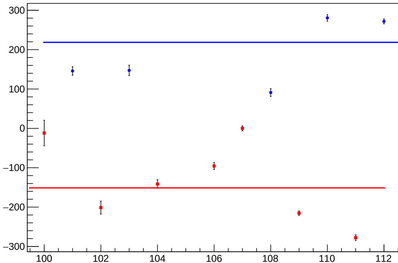
reg_asym_atl1r2_dd_diff_bpm4aX_slope vs Slug, Sign Corrected
