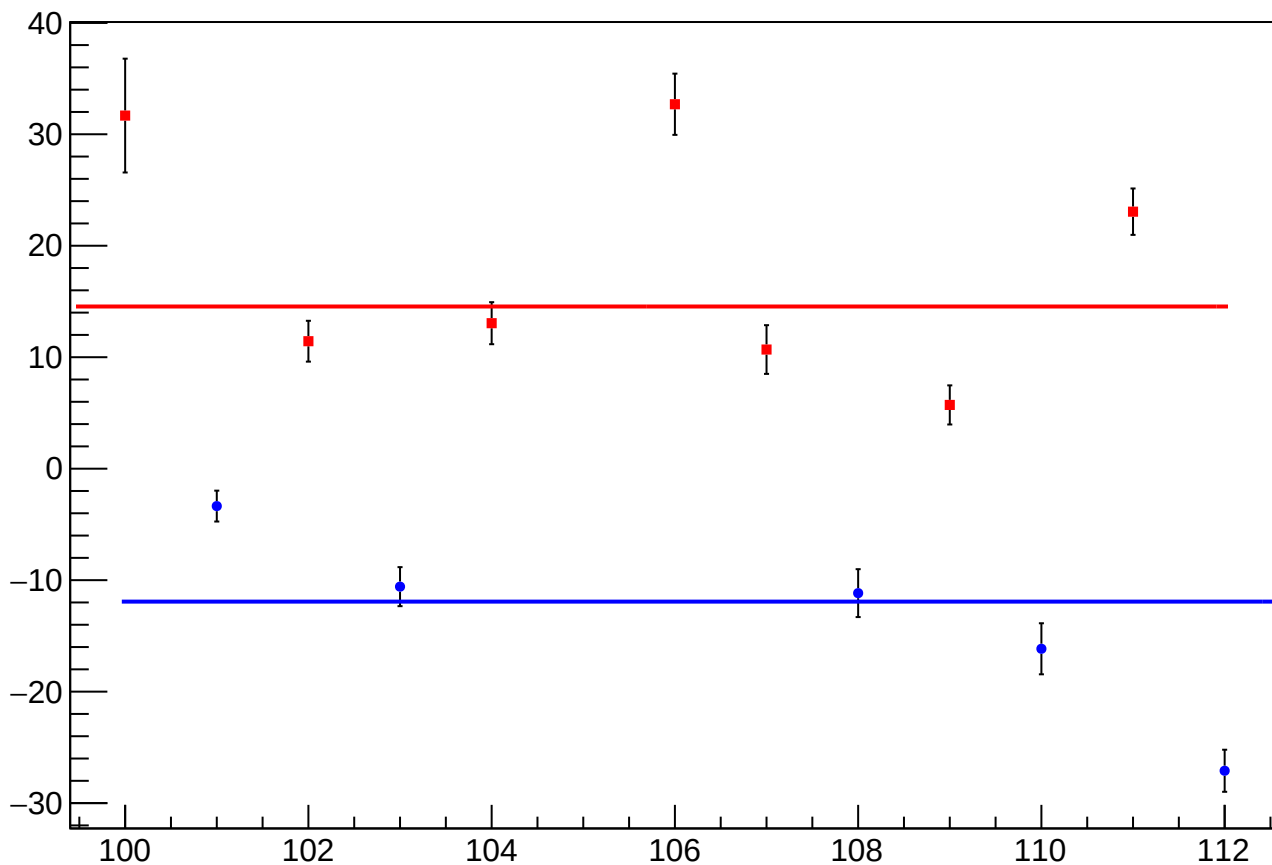
reg_asym_sam_26_48_dd_diff_bpm4aX_slope vs Slug, Sign Corrected
