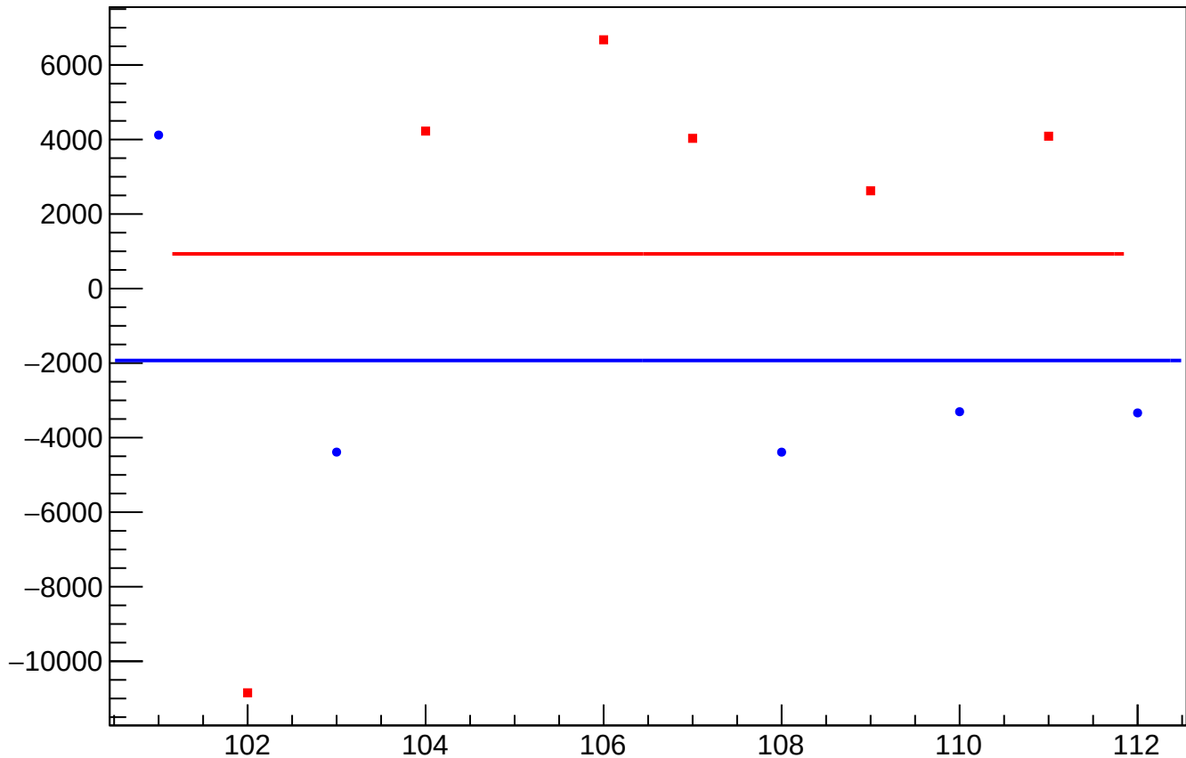
dit_atr1_coil4_mean vs Slug, Sign Corrected
