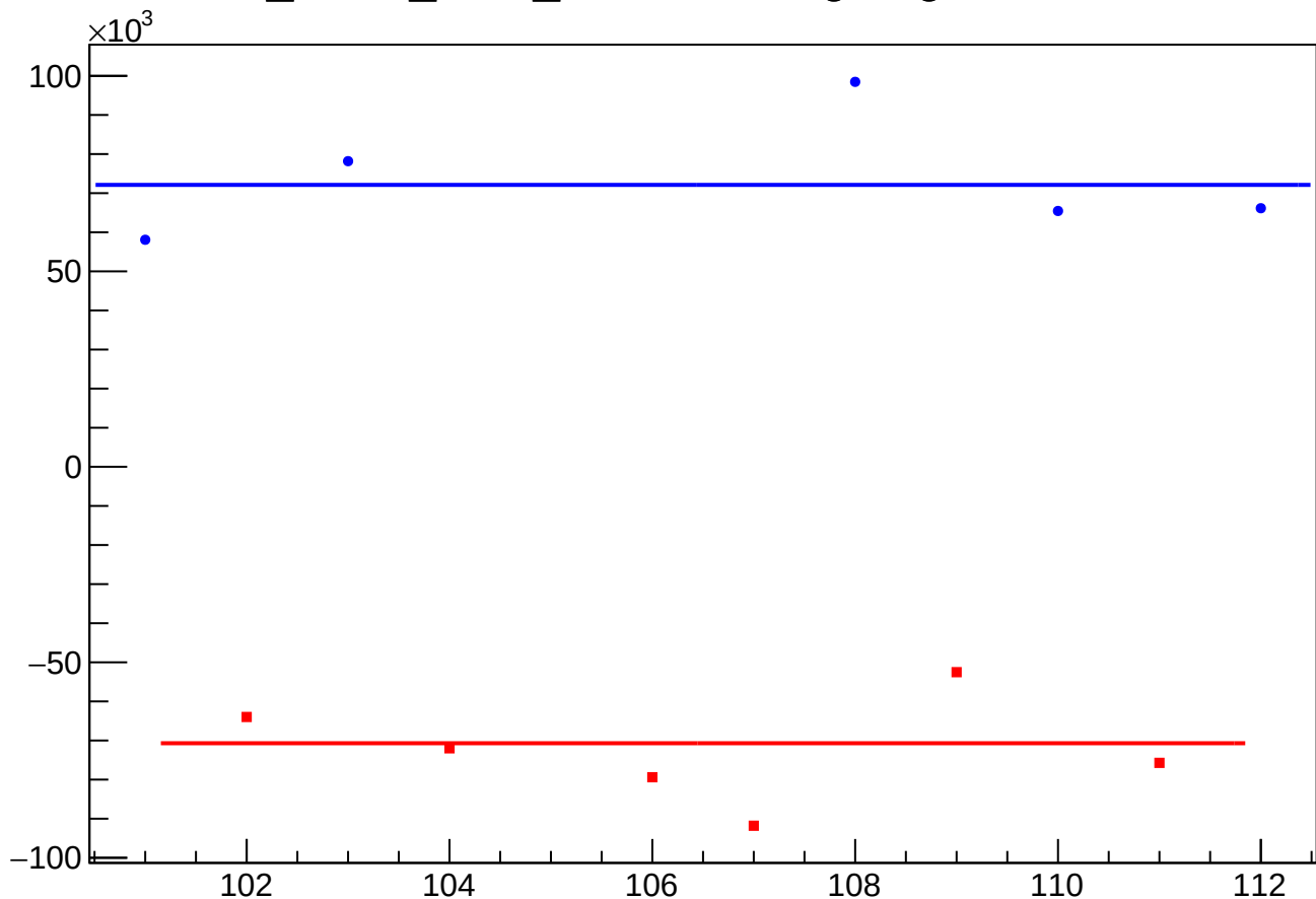
dit_sam2_coil1_mean vs Slug, Sign Corrected
