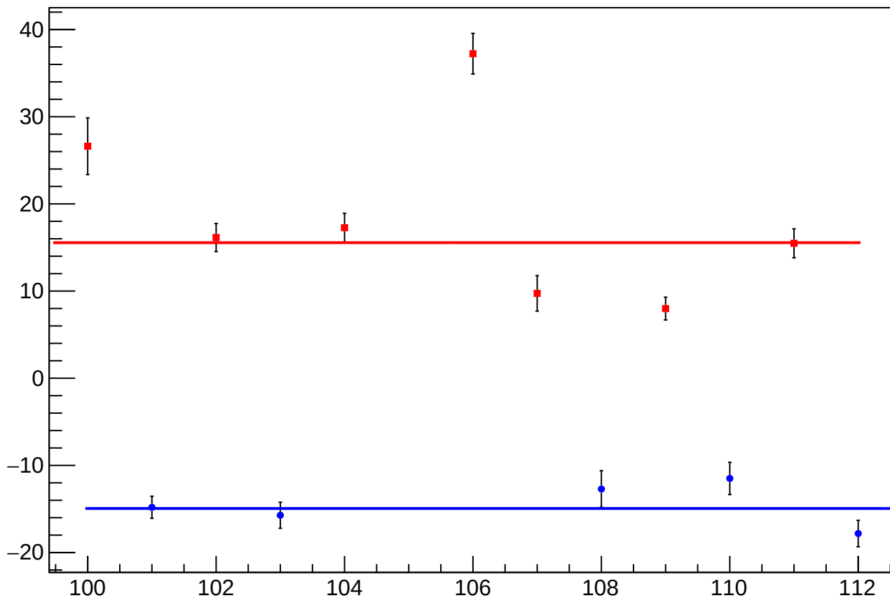
reg_asym_sam1_diff_bpm4aX_slope vs Slug, Sign Corrected
