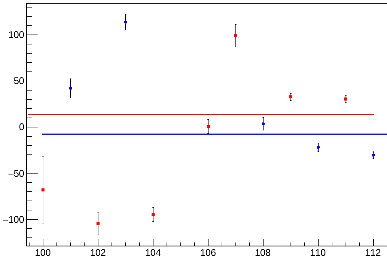
reg_asym_at1_dd_diff_bpm4aX_slope vs Slug, Sign Corrected
