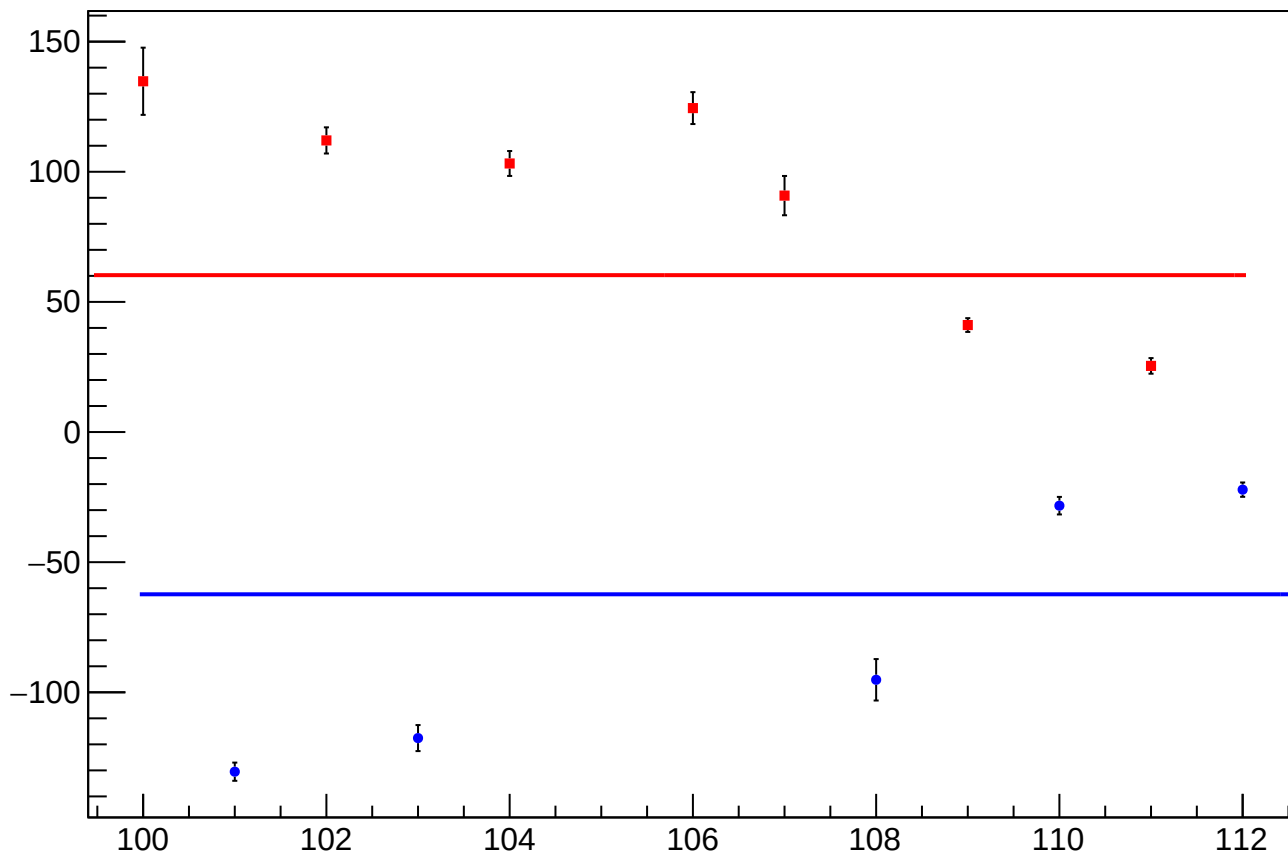
reg_asym_sam4_diff_bpm4aX_slope vs Slug, Sign Corrected
