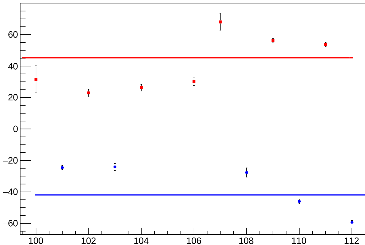
reg_asym_left_avg_diff_bpm4aX_slope vs Slug, Sign Corrected
