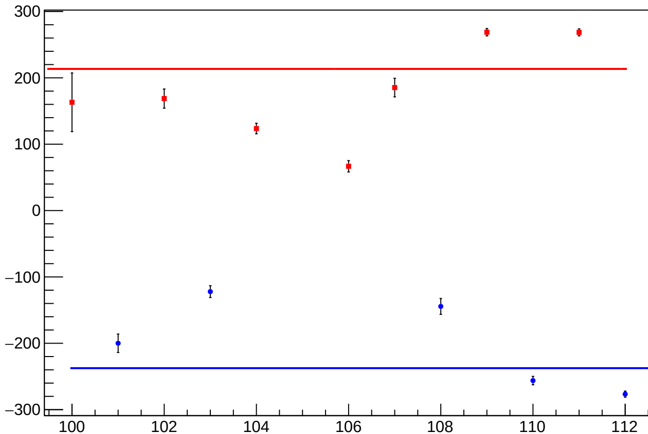
reg_asym_atr1l2_avg_diff_bpm4aX_slope vs Slug, Sign Corrected
