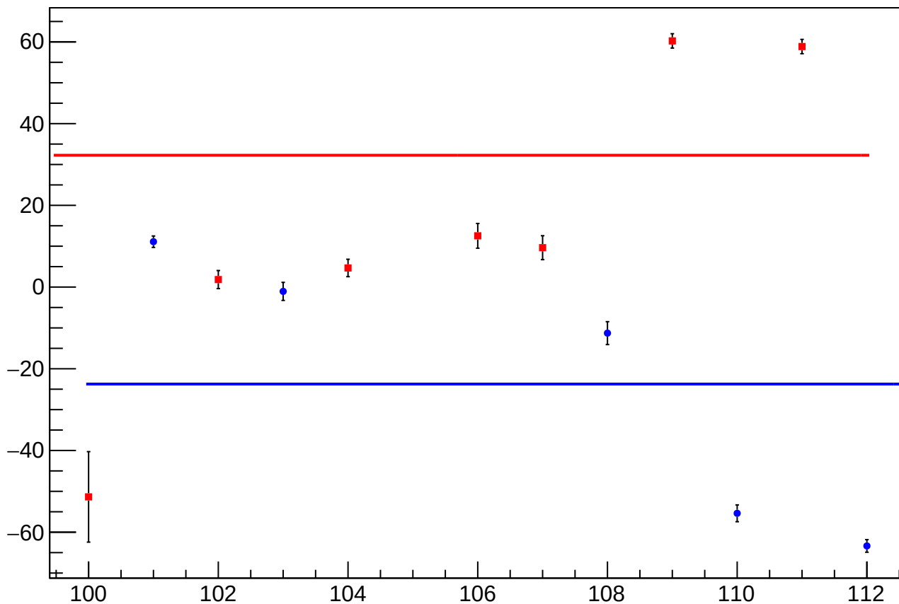
reg_asym_right_avg_diff_bpm4aX_slope vs Slug, Sign Corrected
