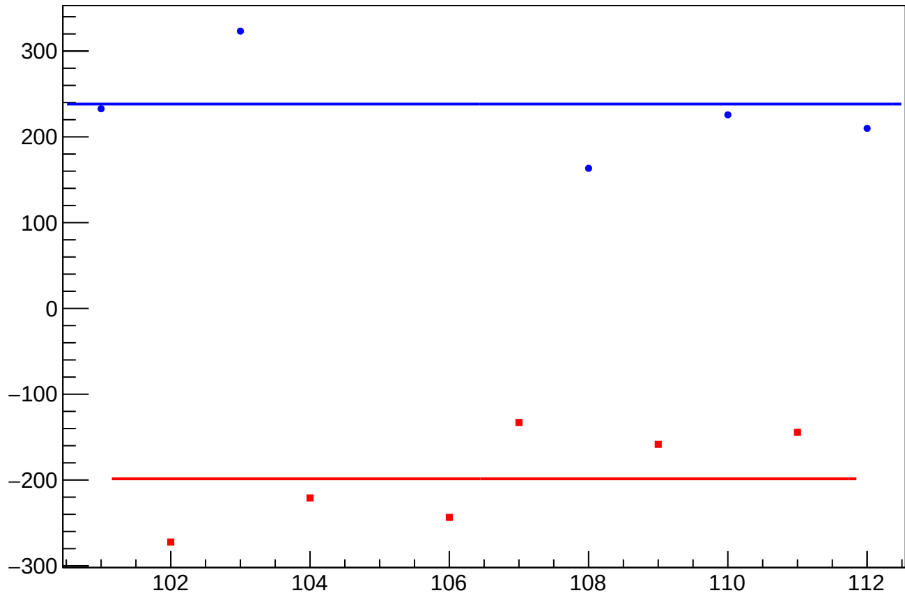
dit_sam5_coil7_err_mean vs Slug, Sign Corrected
