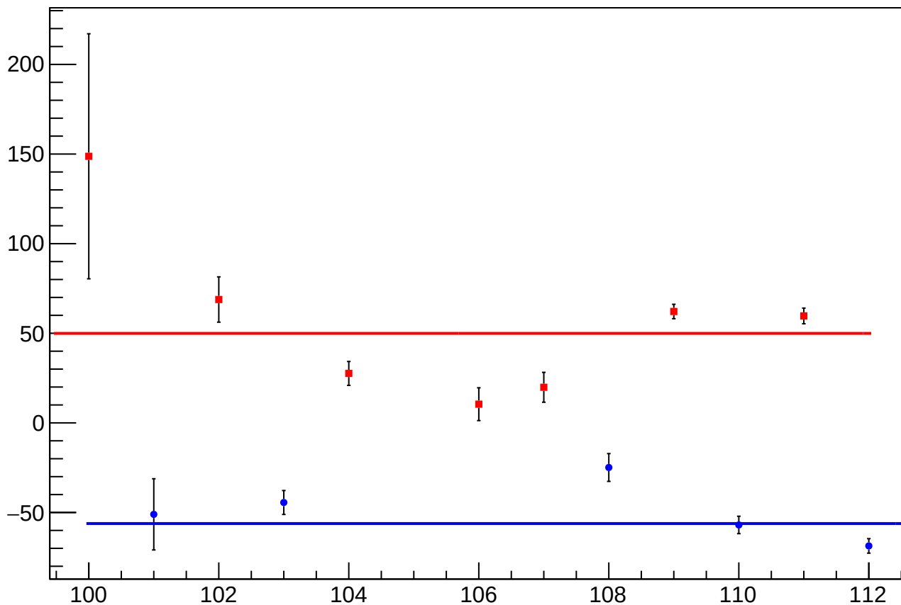
reg_asym_atr1_diff_bpm4aX_slope vs Slug, Sign Corrected
