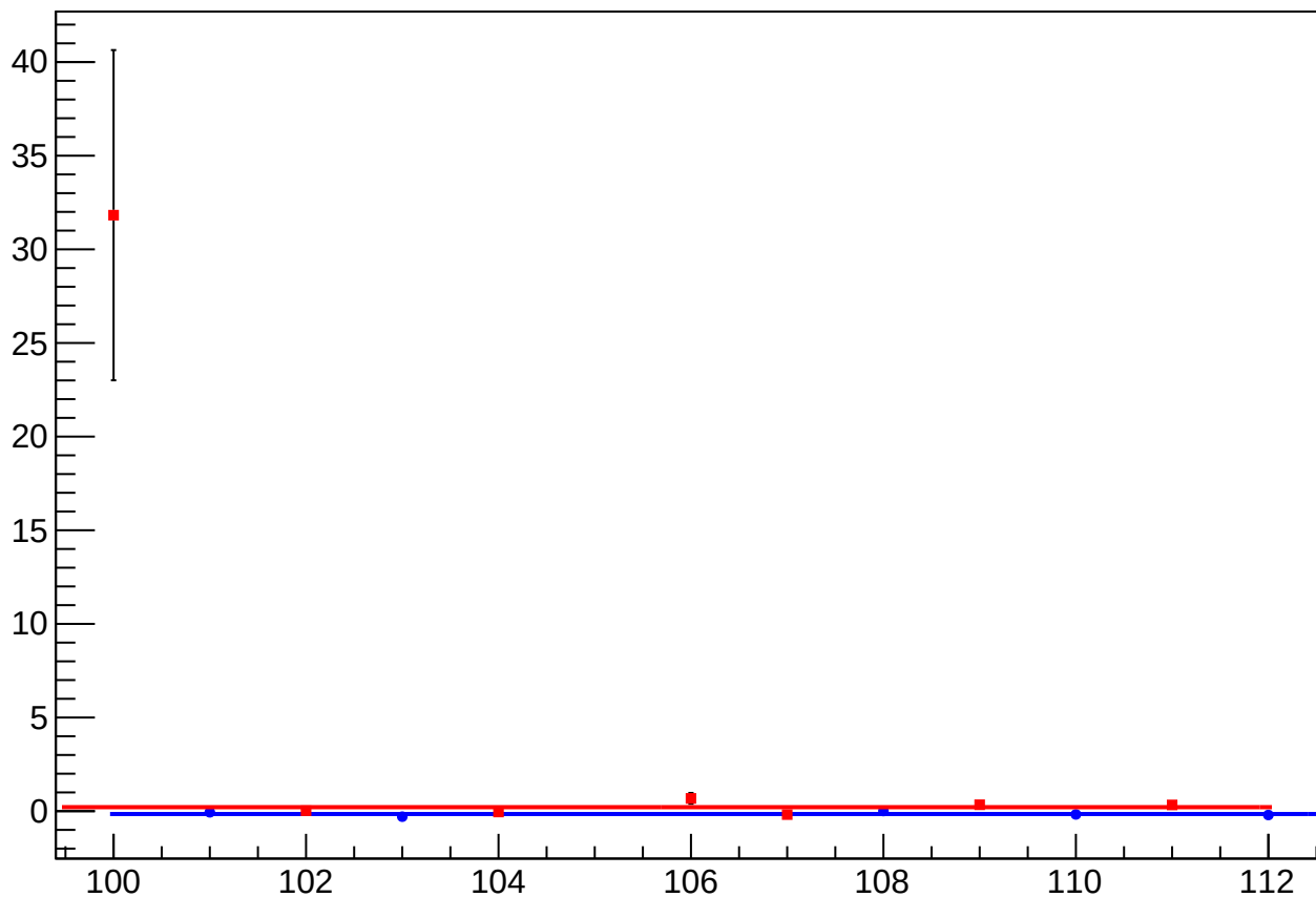
reg_asym_dsl_diff_bpm4aX_slope vs Slug, Sign Corrected
