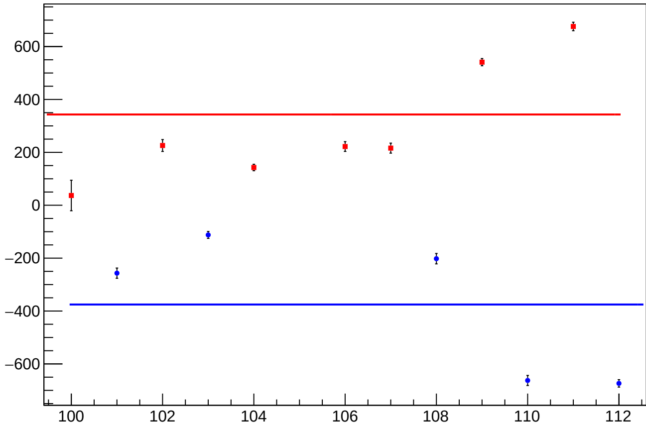
reg_asym_atr2_diff_bpm4aX_slope vs Slug, Sign Corrected
