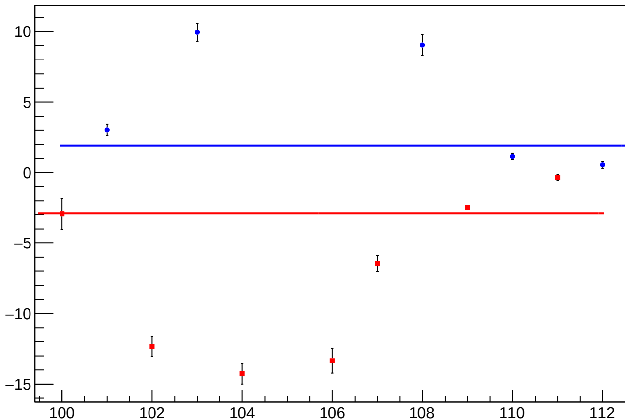
reg_asym_bcm_dg_us_diff_bpm4aX_slope vs Slug, Sign Corrected
