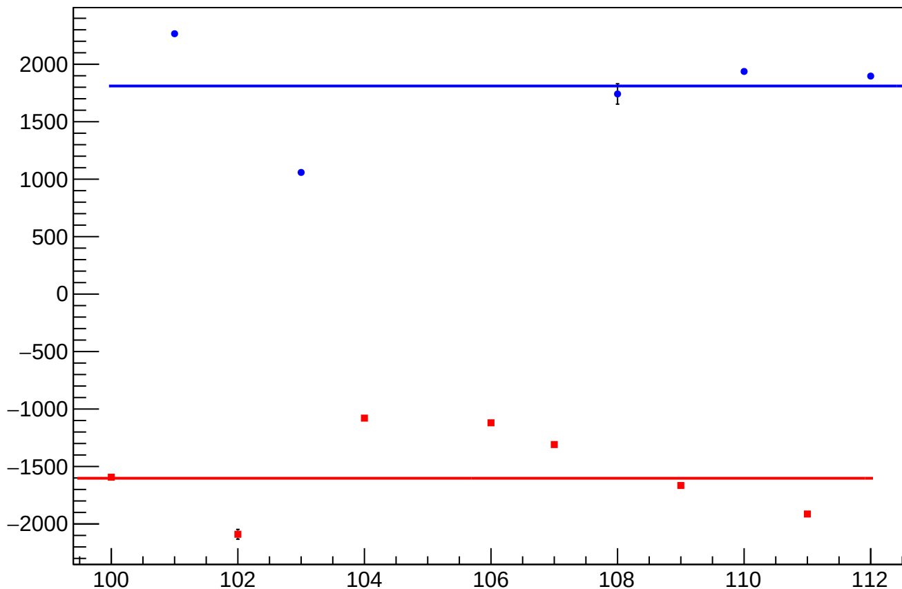
dit_atr2_4eX_slope vs Slug, Sign Corrected
