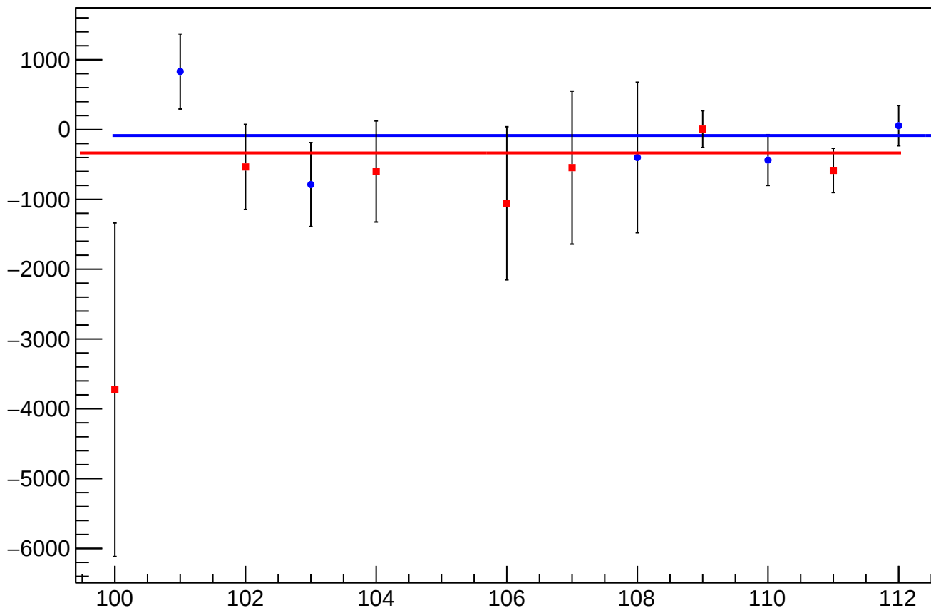
asym_sam7_mean vs Slug, Sign Corrected
