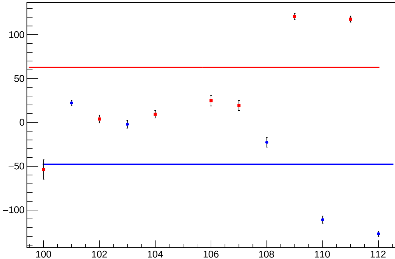
reg_asym_usr_diff_bpm4aX_slope vs Slug, Sign Corrected
