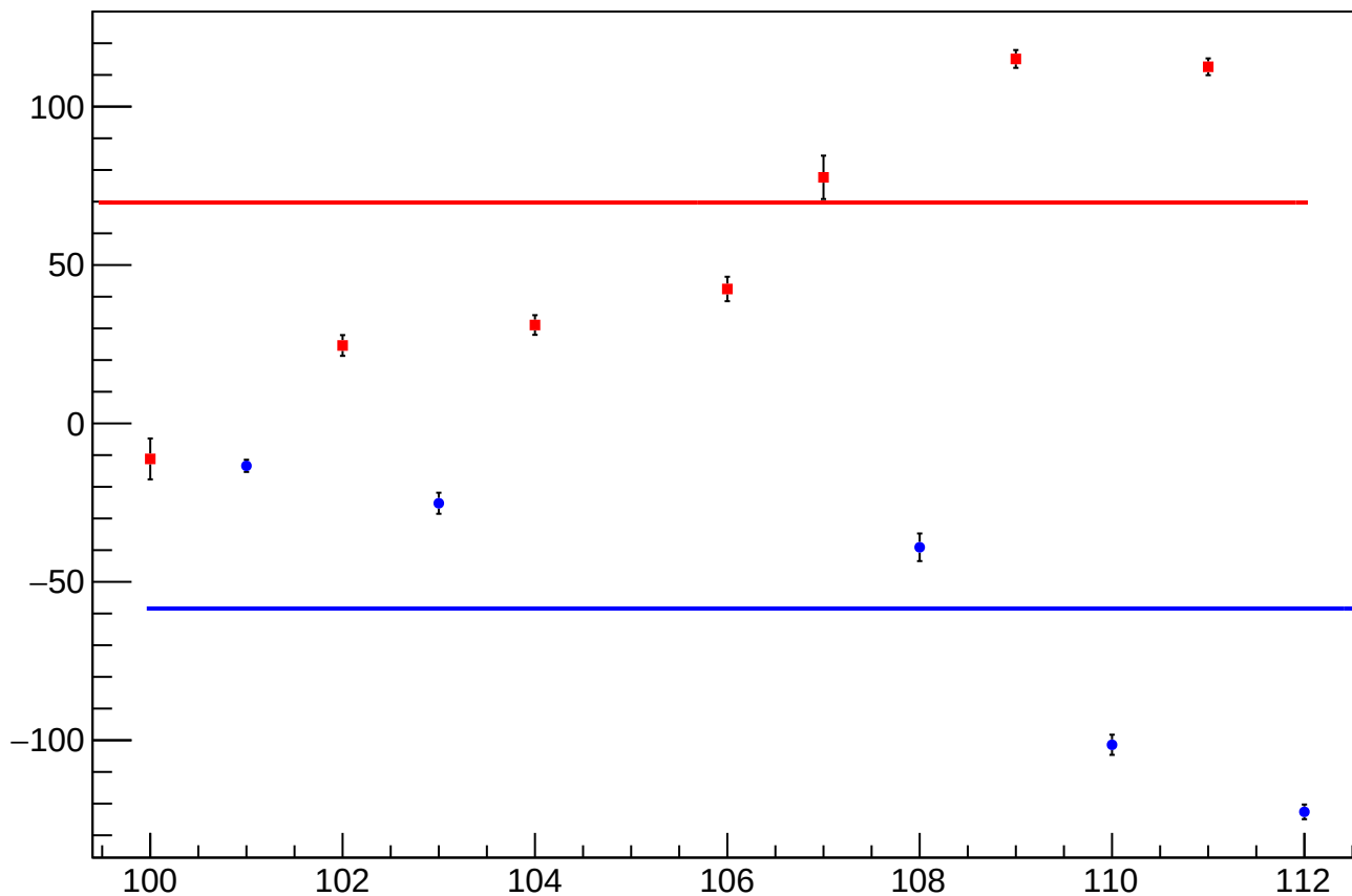
reg_asym_us_avg_diff_bpm4aX_slope vs Slug, Sign Corrected
