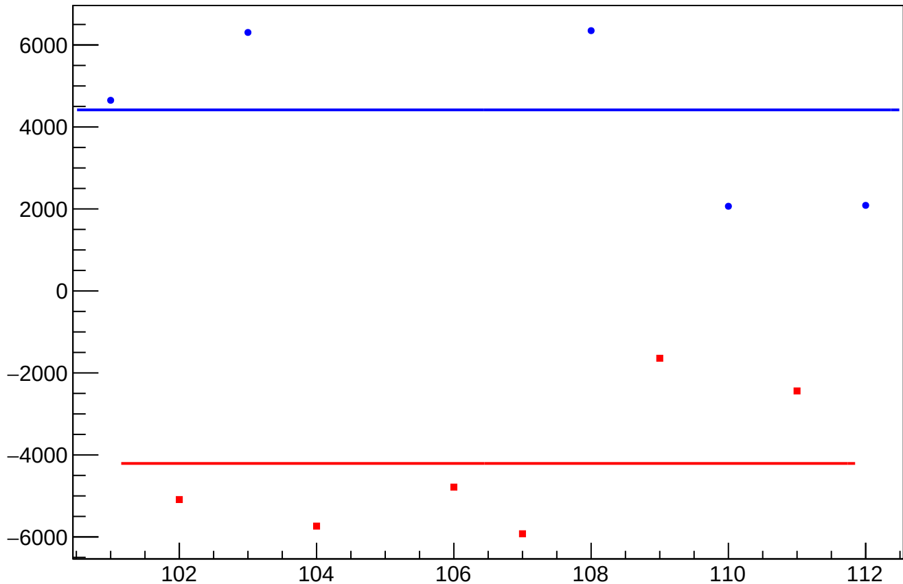
dit_sam8_coil1_mean vs Slug, Sign Corrected
