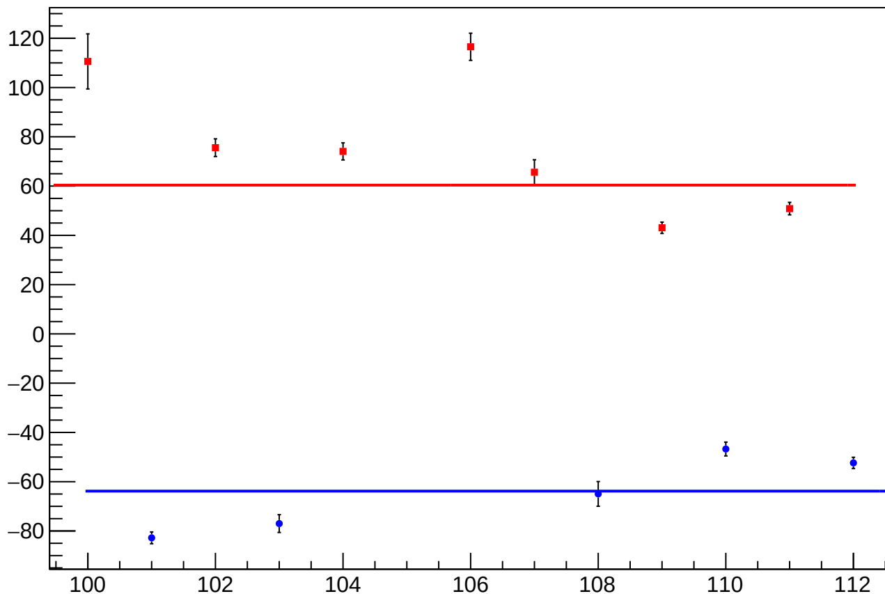
reg_asym_sam_24_68_dd_diff_bpm4aX_slope vs Slug, Sign Corrected
