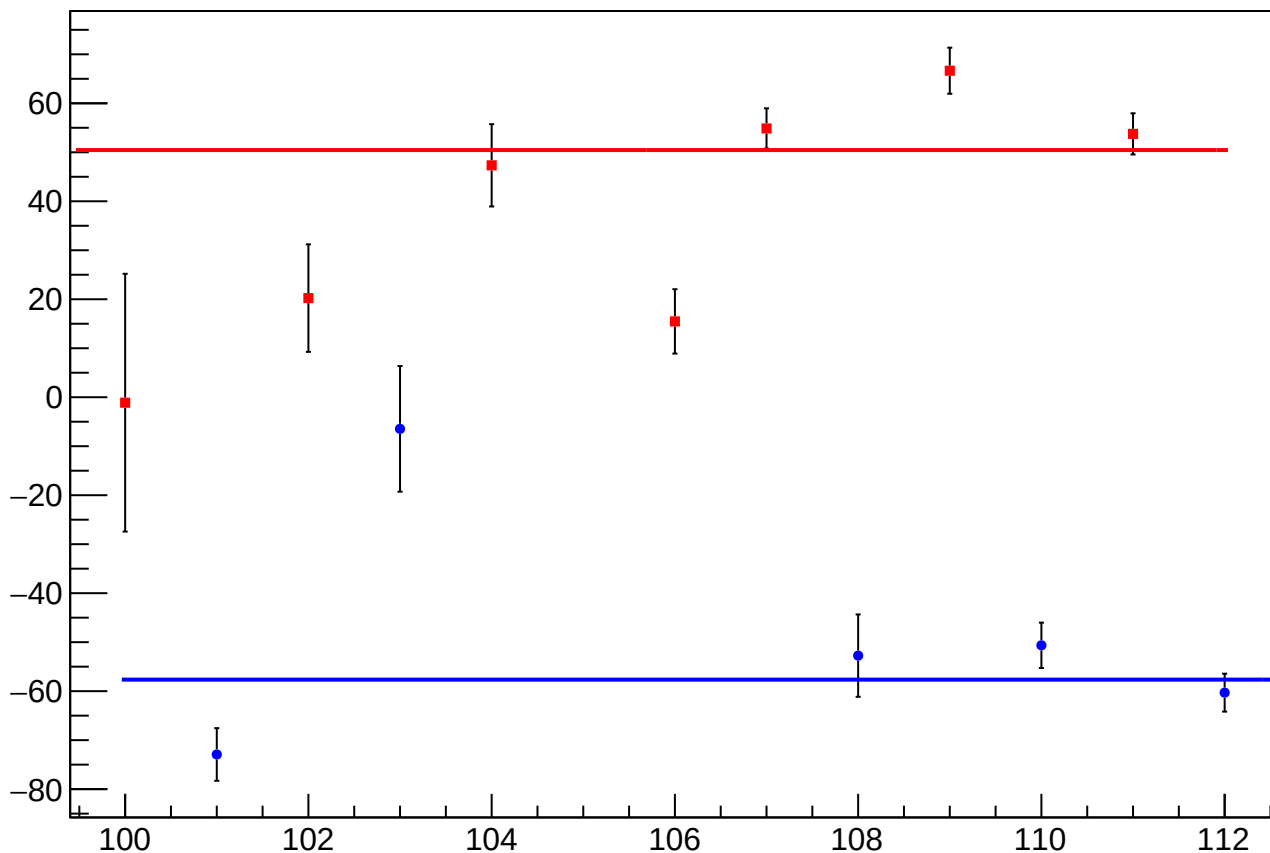
reg_asym_atl_dd_diff_bpm4eY_slope vs Slug, Sign Corrected
