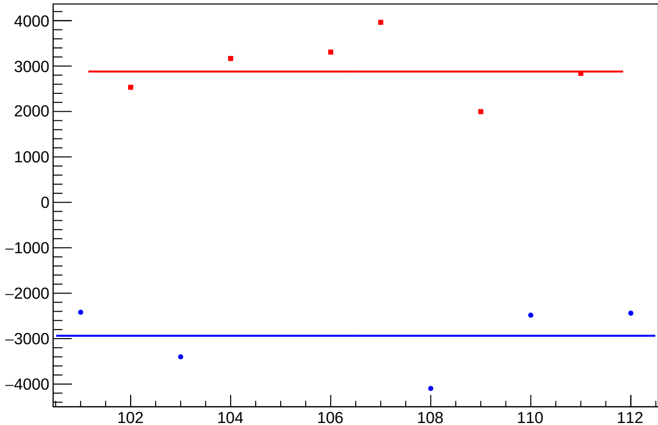
dit_usr_coil3_mean vs Slug, Sign Corrected
