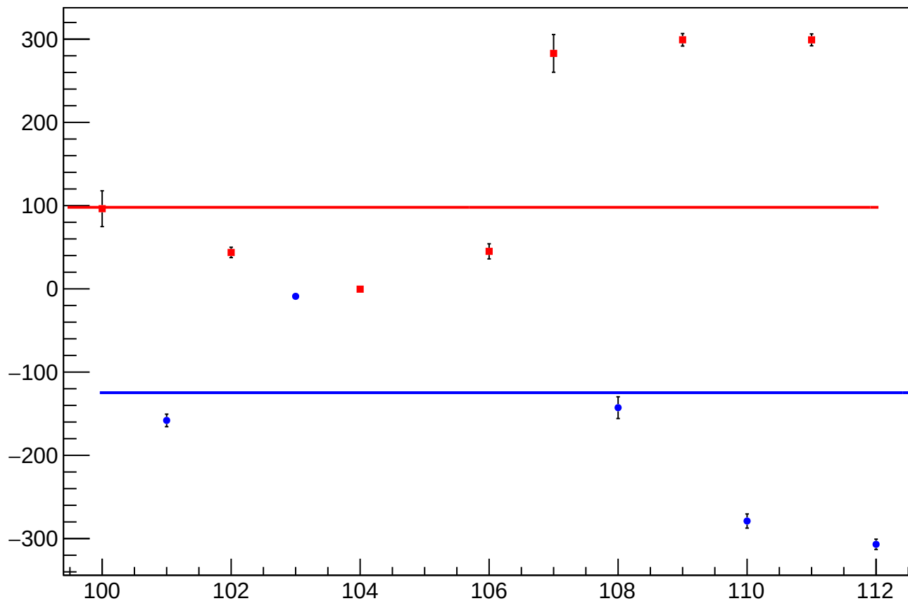
reg_asym_atl_avg_diff_bpm4aX_slope vs Slug, Sign Corrected
