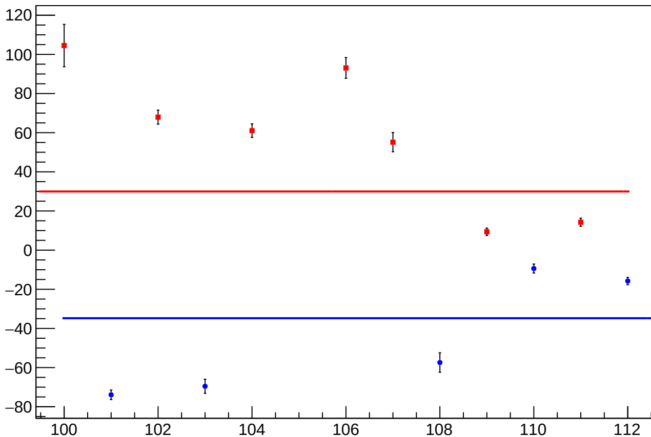
reg_asym_sam_2468_avg_diff_bpm4aX_slope vs Slug, Sign Corrected
