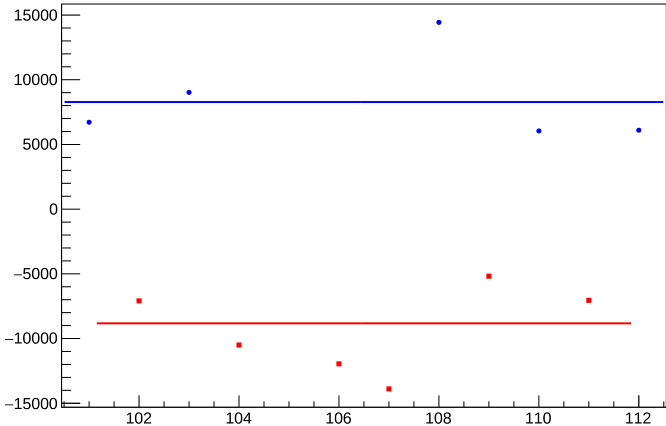
dit_sam7_coil1_mean vs Slug, Sign Corrected
