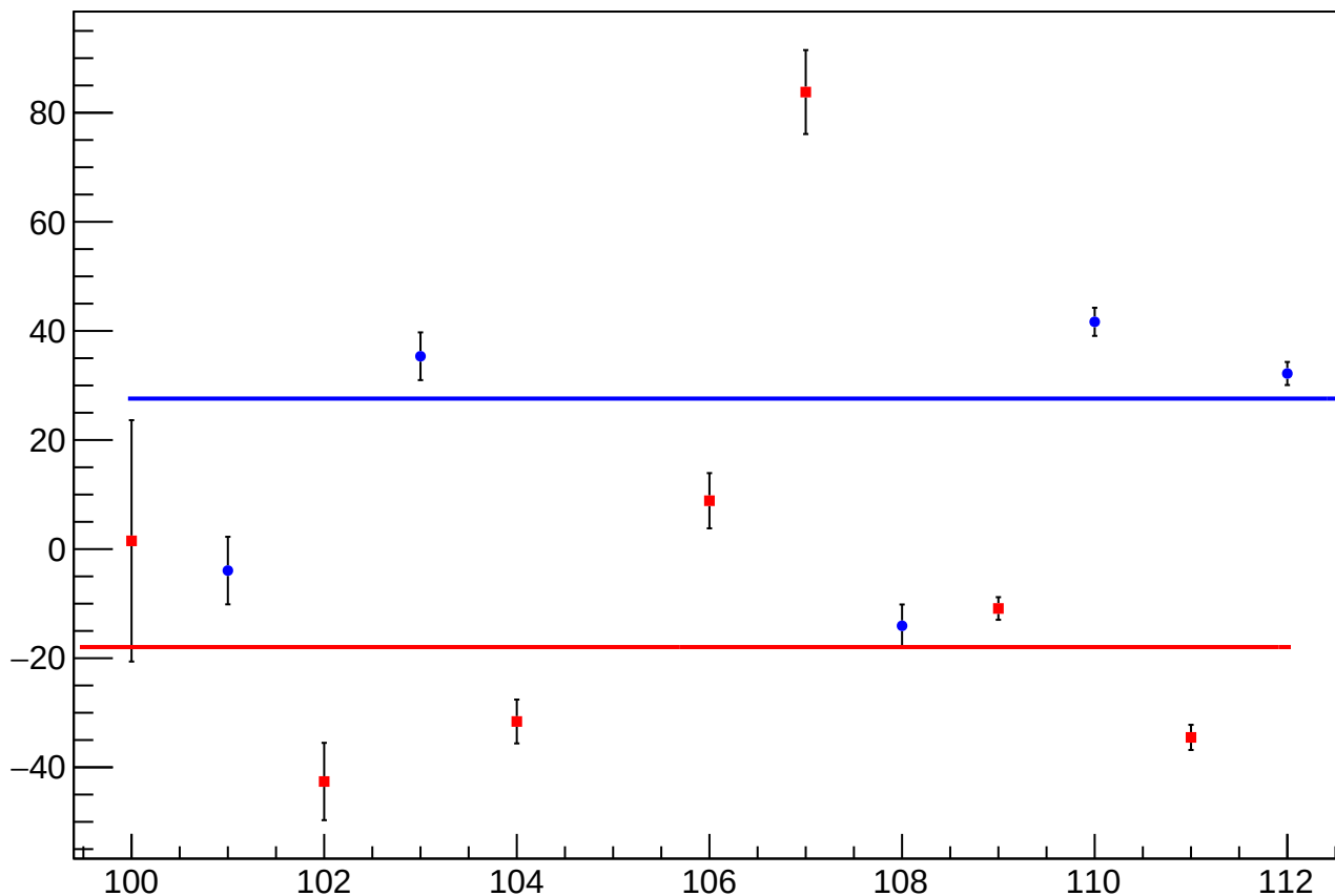
reg_asym_atl_avg_atr_avg_dd_diff_bpm4aX_slope vs Slug, Sign Corrected
