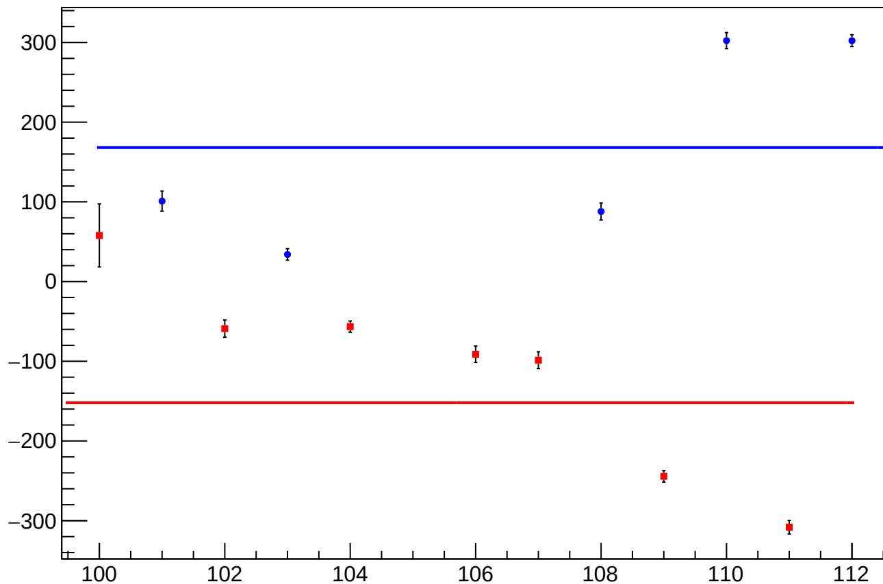
reg_asym_atr_dd_diff_bpm4aX_slope vs Slug, Sign Corrected
