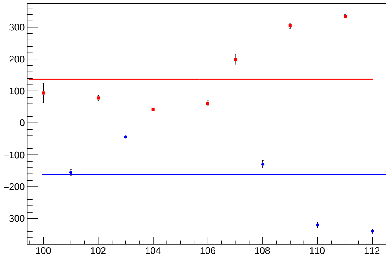
reg_asym_atl_avg_atr_avg_avg_diff_bpm4aX_slope vs Slug, Sign Corrected
