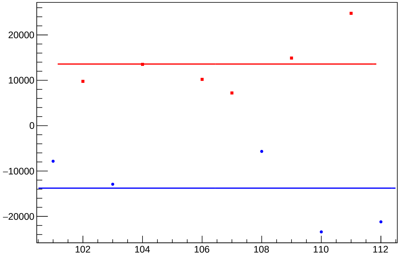
dit_sam4_coil7_mean vs Slug, Sign Corrected
