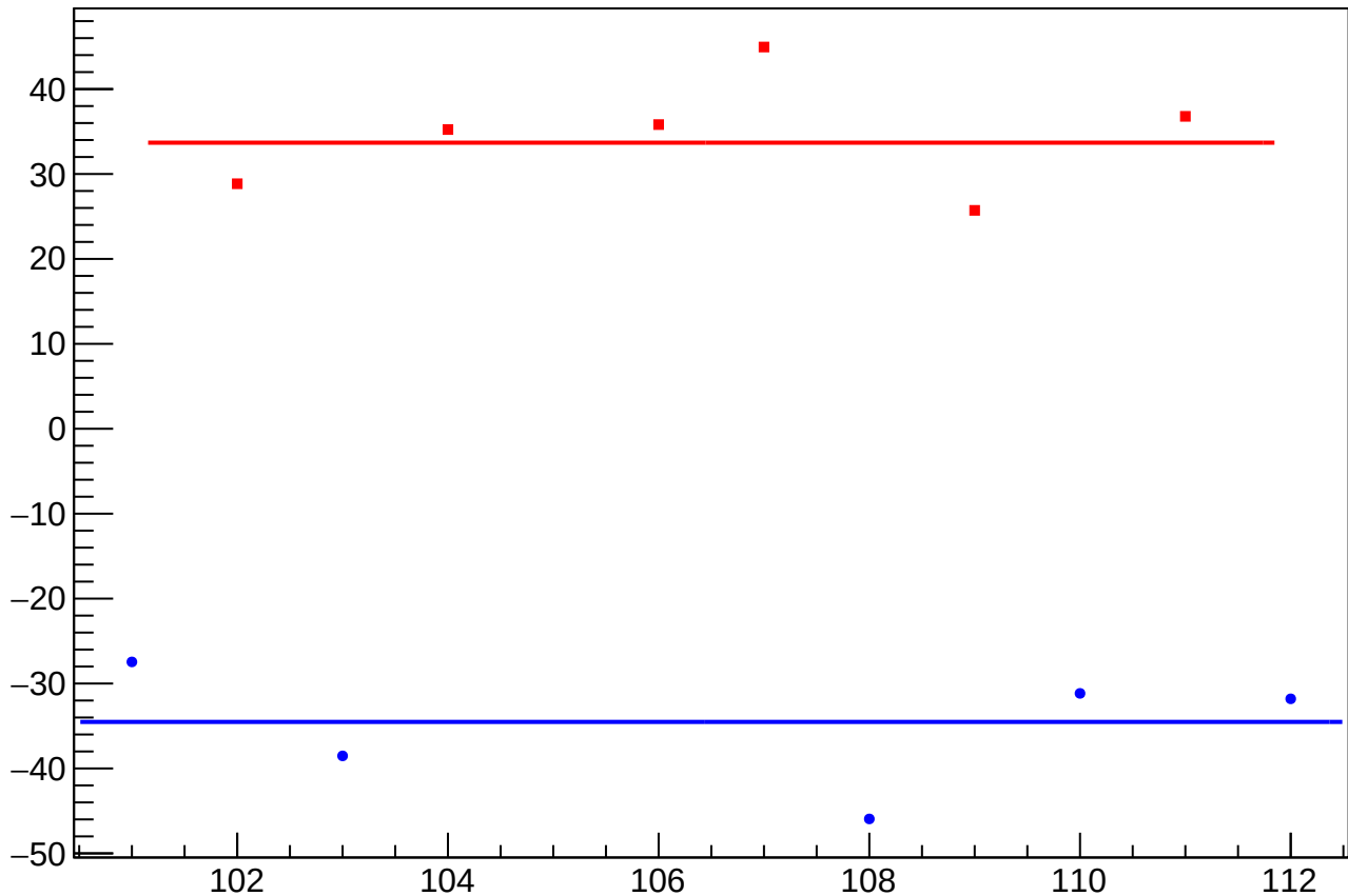
dit_4eX_coil3_mean vs Slug, Sign Corrected
