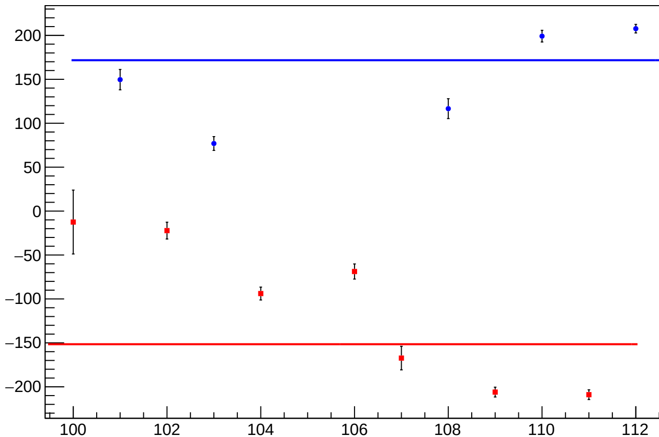
reg_asym_atr1l2_dd_diff_bpm4aX_slope vs Slug, Sign Corrected
