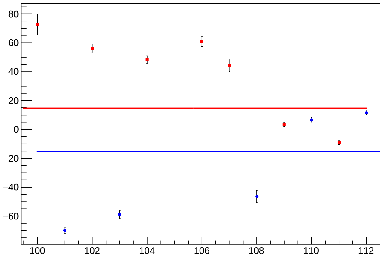
reg_asym_sam_48_avg_diff_bpm4aX_slope vs Slug, Sign Corrected
