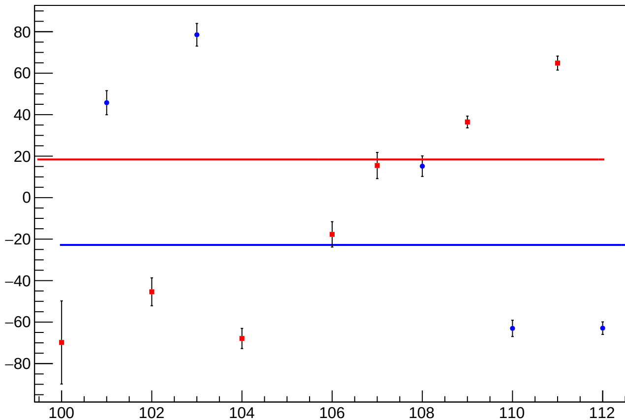
reg_asym_atl_dd_atr_dd_diff_bpm4aX_slope vs Slug, Sign Corrected
