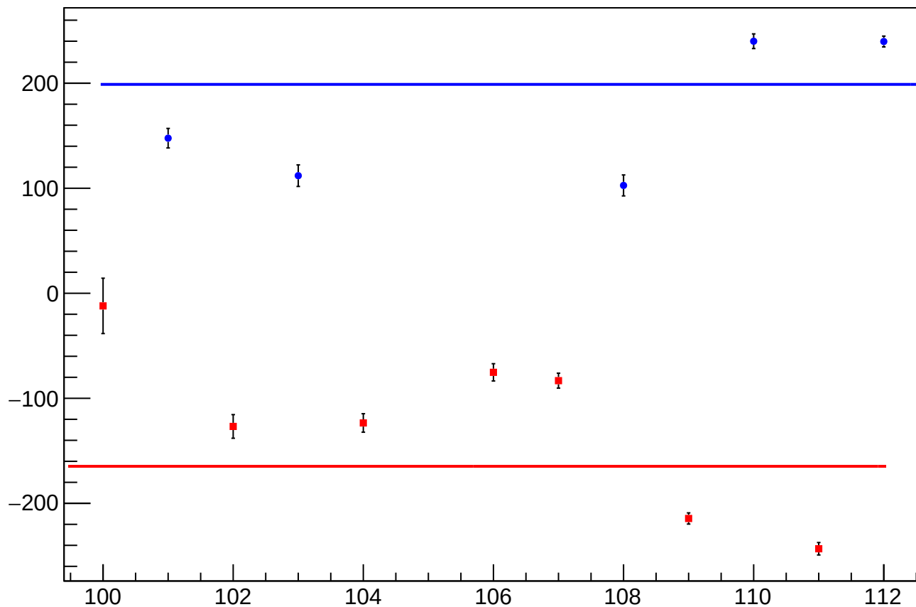
reg_asym_atl_dd_atr_dd_avg_diff_bpm4aX_slope vs Slug, Sign Corrected
