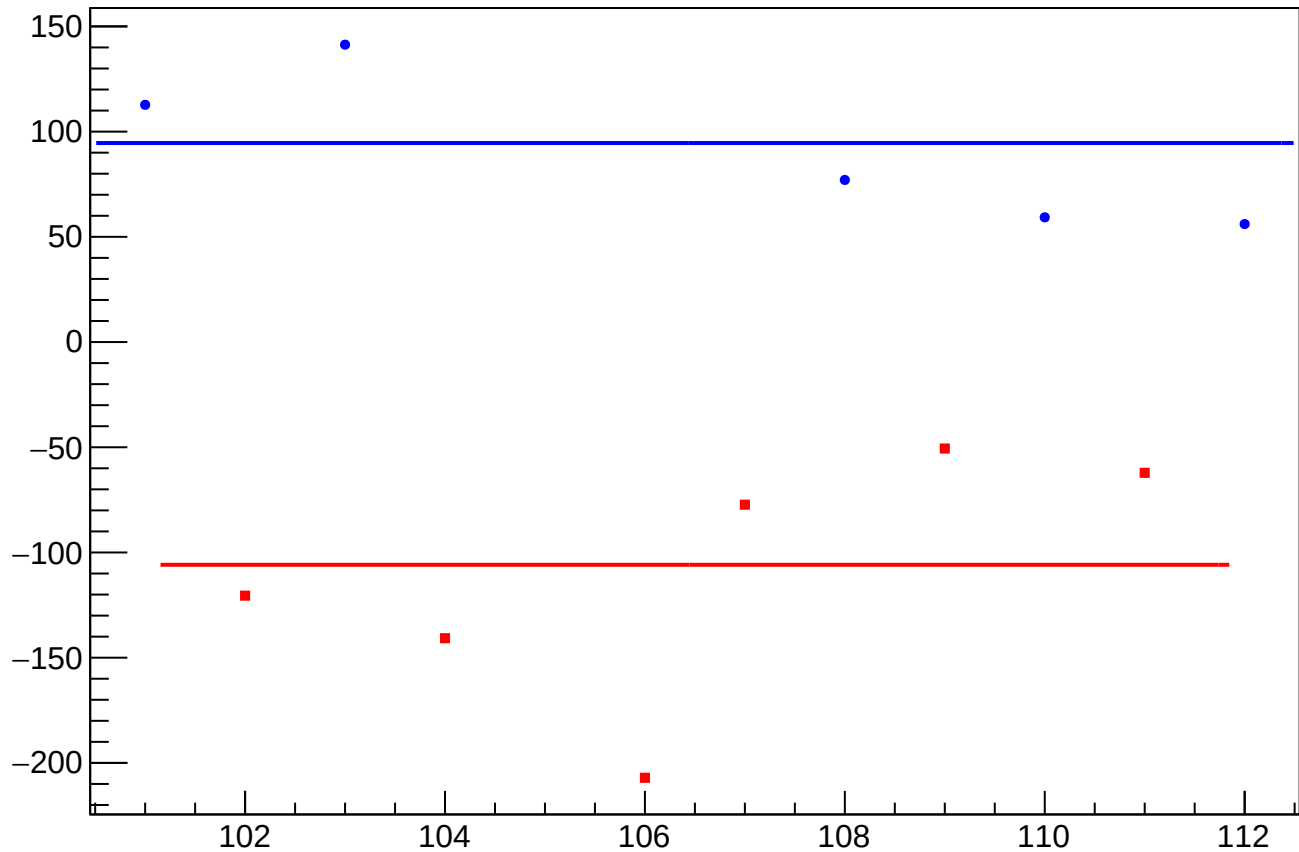
dit_sam5_coil3_err_mean vs Slug, Sign Corrected
