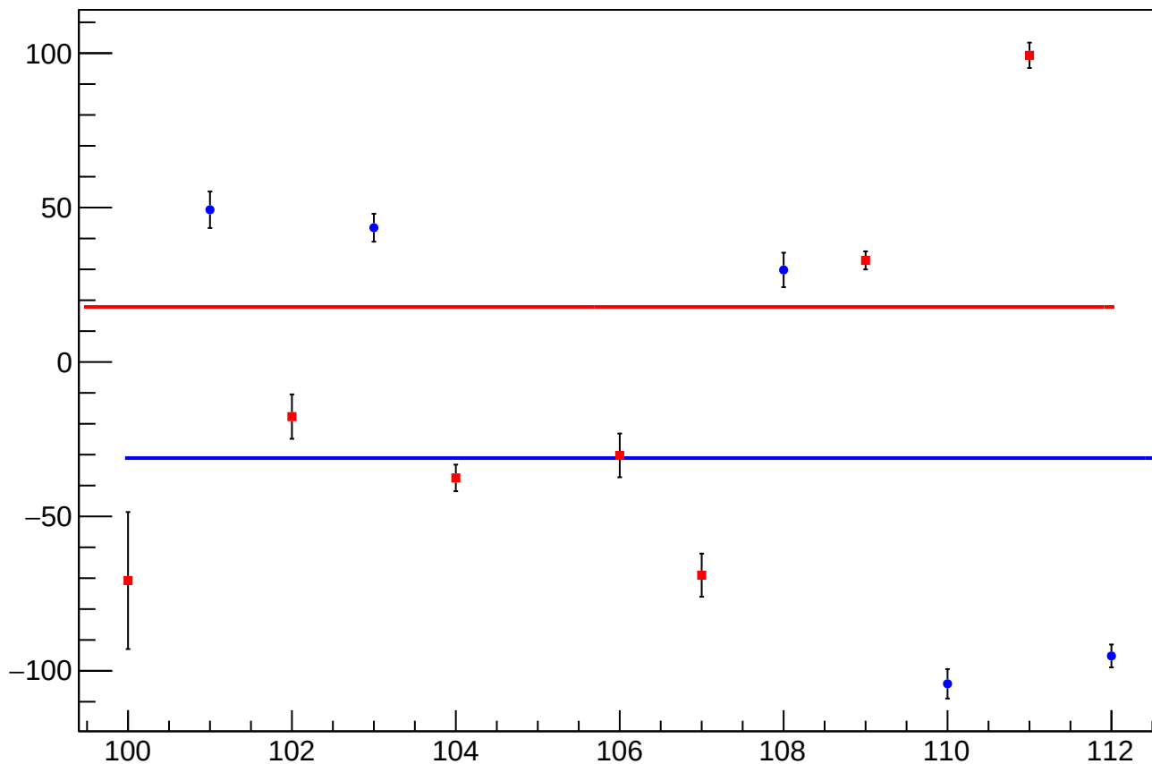
reg_asym_at2_dd_diff_bpm4aX_slope vs Slug, Sign Corrected
