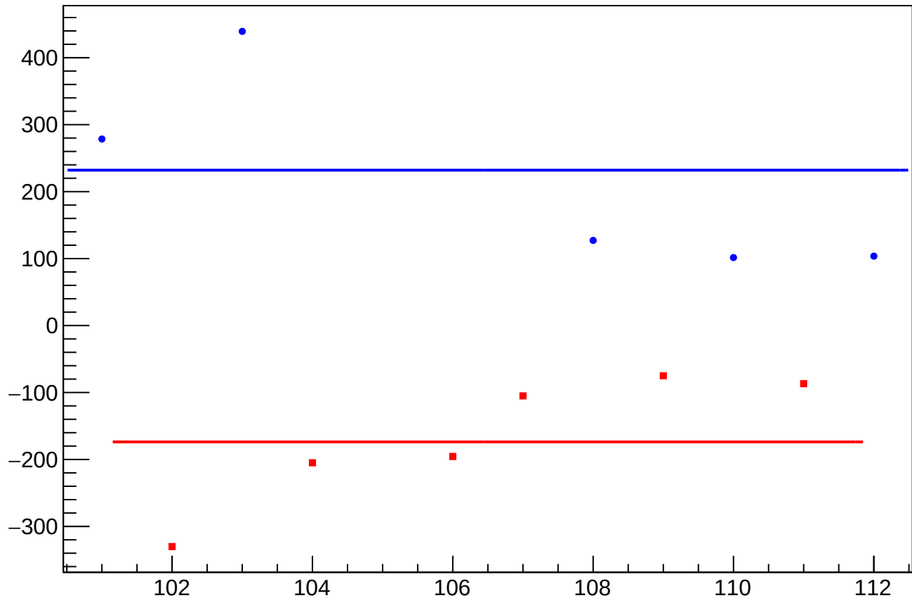
dit_sam1_coil6_err_mean vs Slug, Sign Corrected
