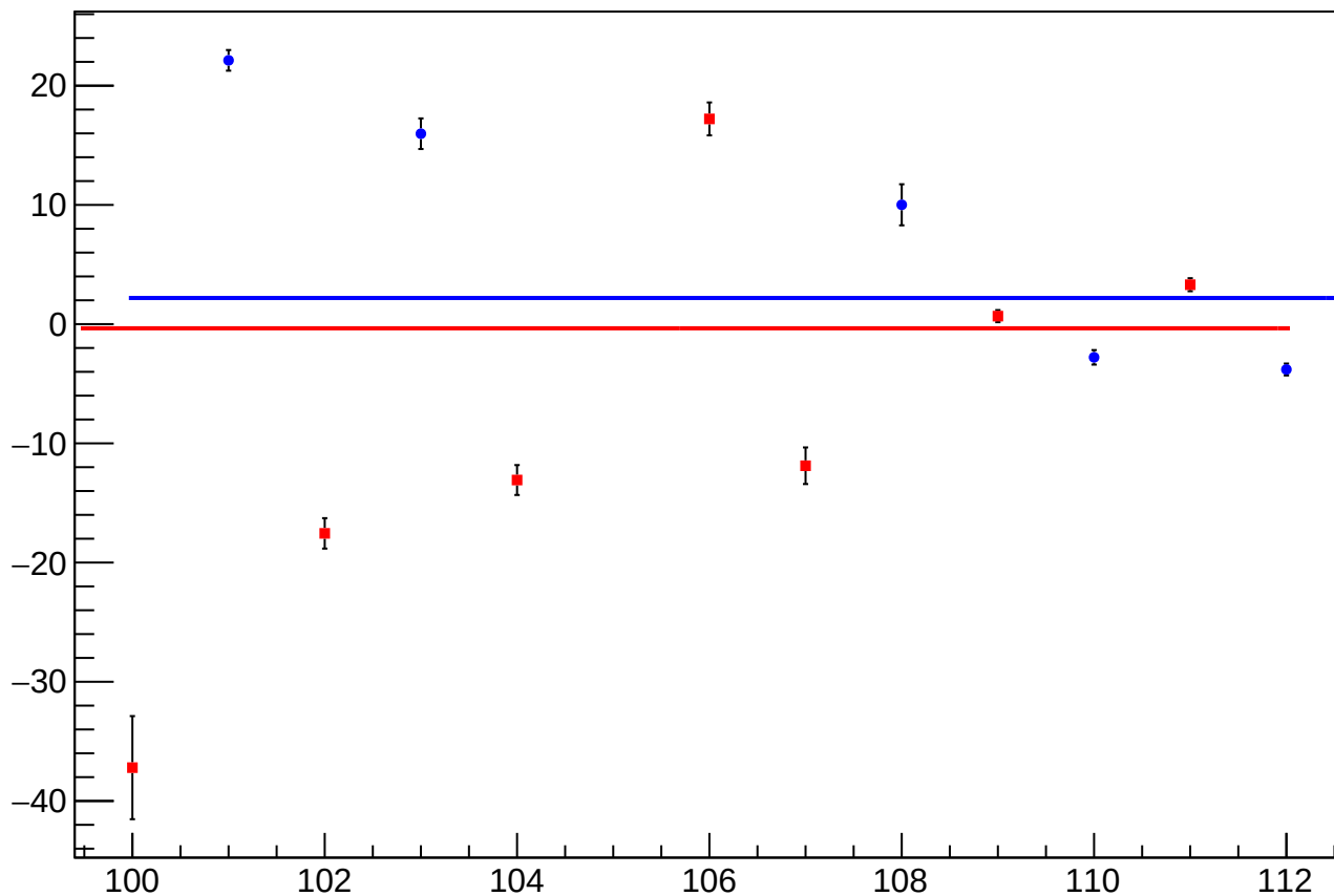
reg_asym_sam_15_37_dd_diff_bpm4aX_slope vs Slug, Sign Corrected
