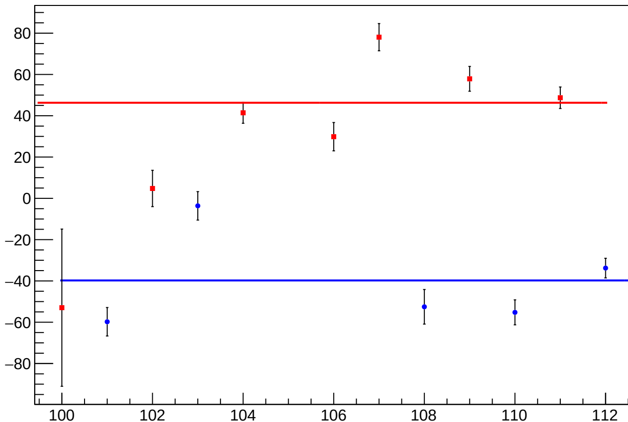
reg_asym_atr1l2_dd_diff_bpm4eY_slope vs Slug, Sign Corrected
