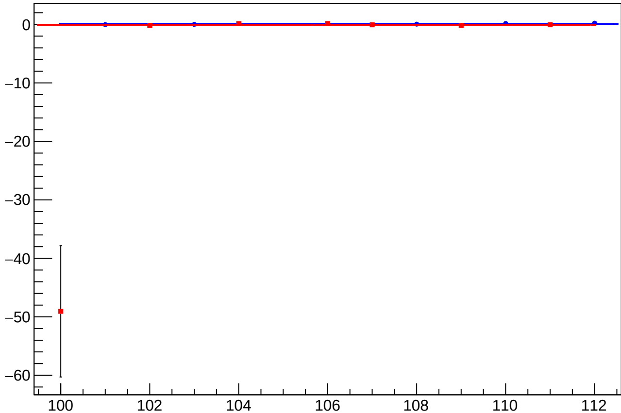
reg_asym_dsr_diff_bpm4aX_slope vs Slug, Sign Corrected
