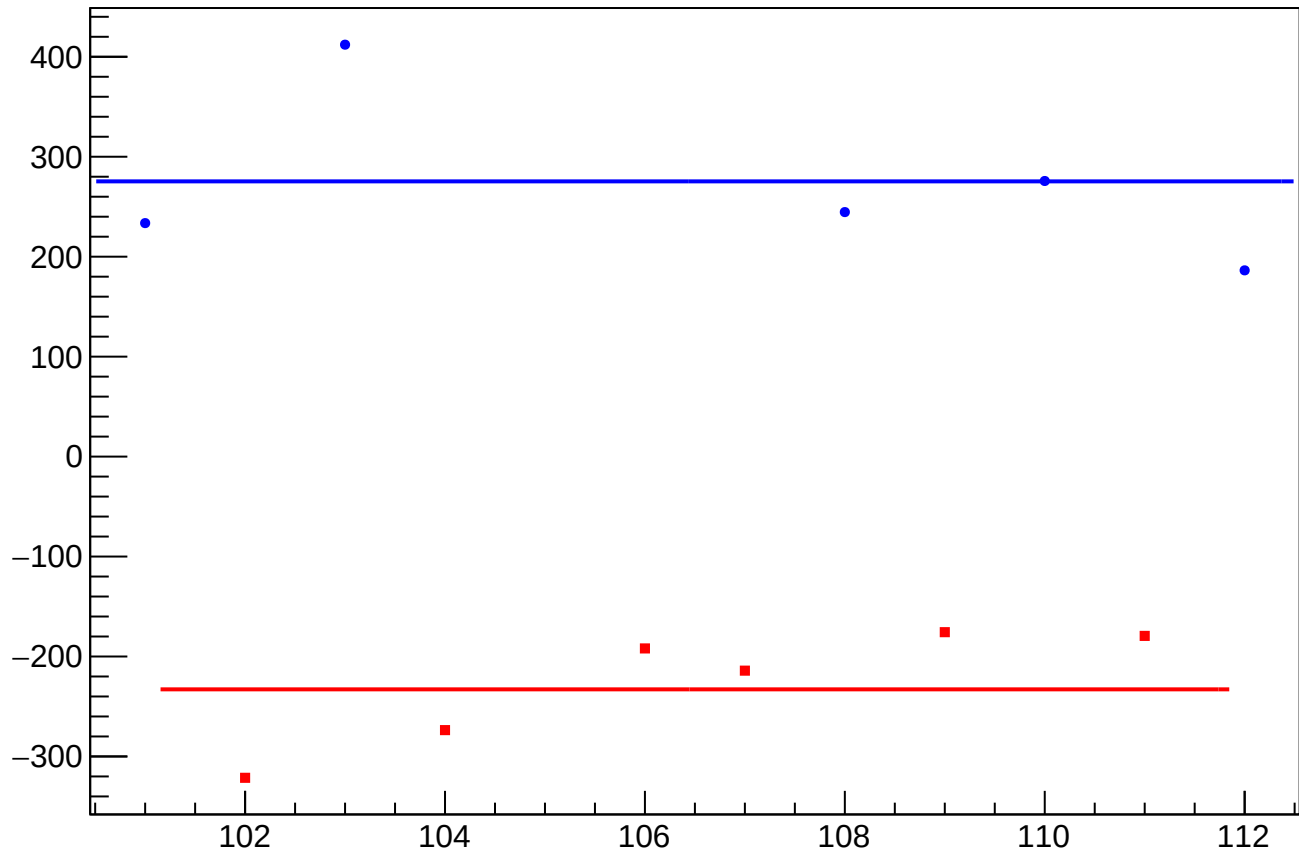
dit_sam6_coil7_err_mean vs Slug, Sign Corrected
