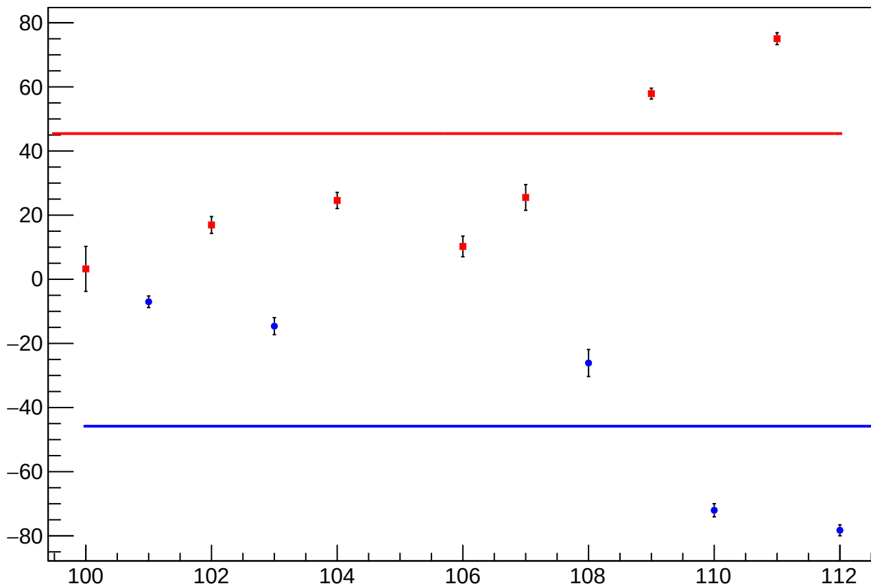
reg_asym_sam_48_avg_diff_bpm4eX_slope vs Slug, Sign Corrected
