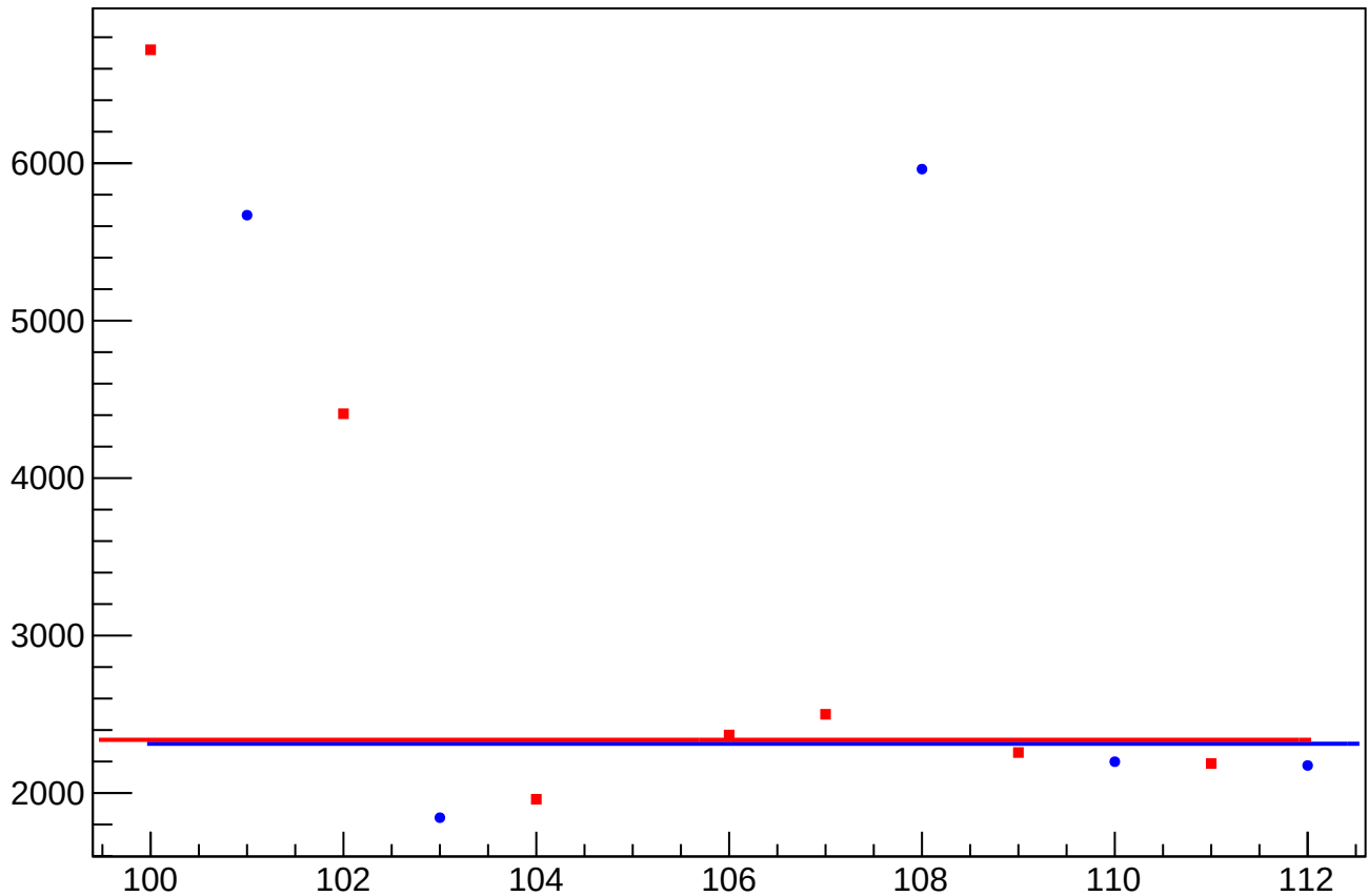
dit_asym_at1_avg_rms vs Slug, Sign Corrected
