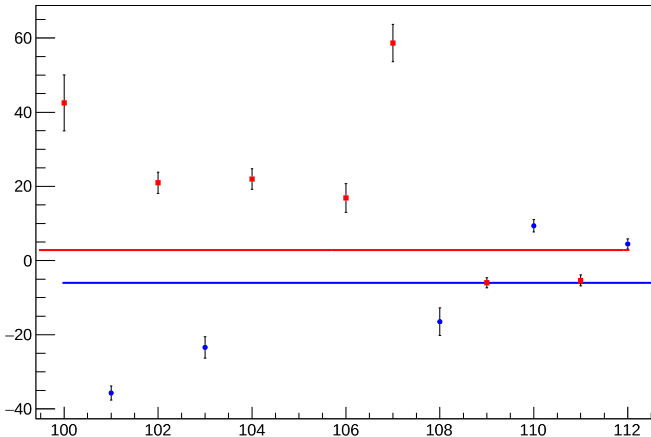
reg_asym_us_dd_diff_bpm4aX_slope vs Slug, Sign Corrected
