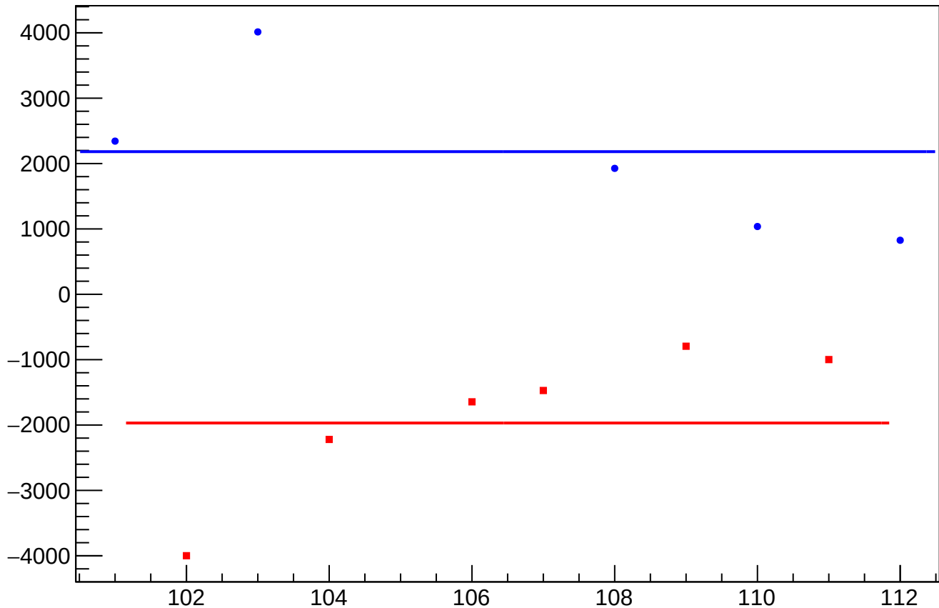
dit_sam2_coil1_err_mean vs Slug, Sign Corrected
