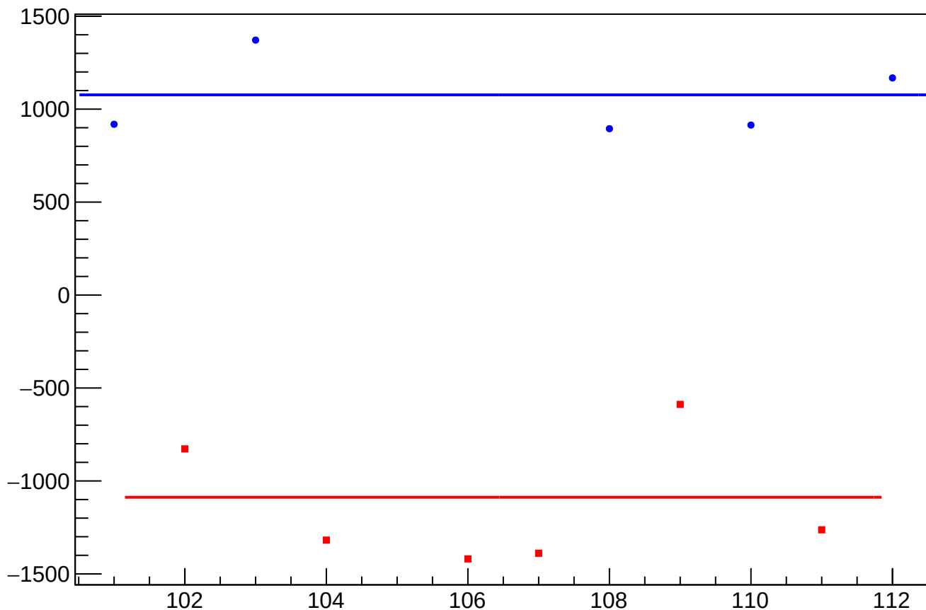
dit_atl1_coil6_Ndata_mean vs Slug, Sign Corrected
