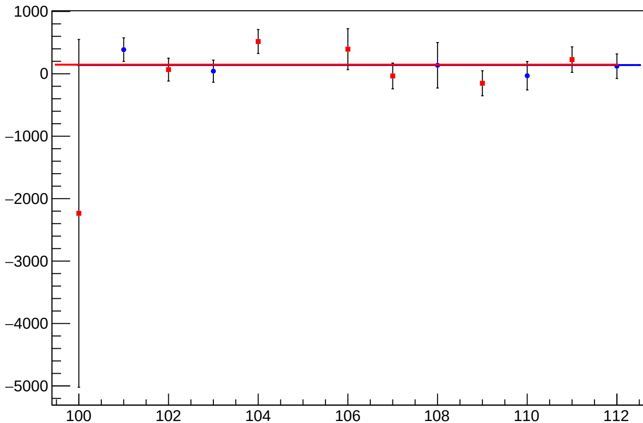
dit_asym_sam1_mean vs Slug, Sign Corrected
