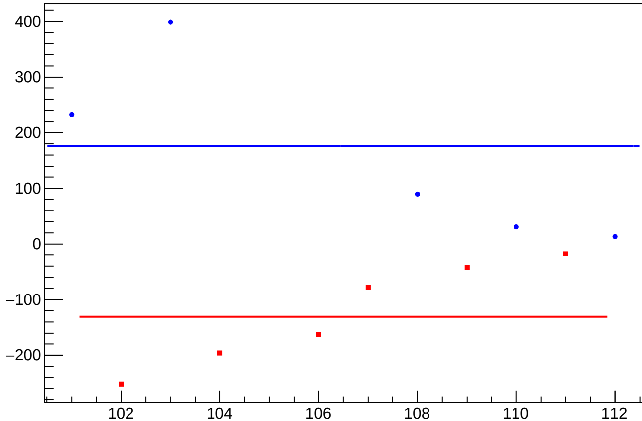
dit_sam8_coil6_err_mean vs Slug, Sign Corrected
