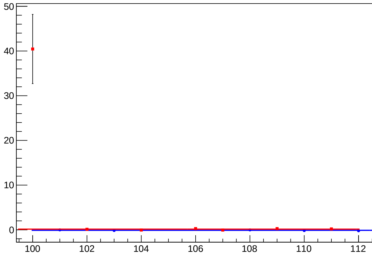
reg_asym_ds_dd_diff_bpm4aX_slope vs Slug, Sign Corrected
