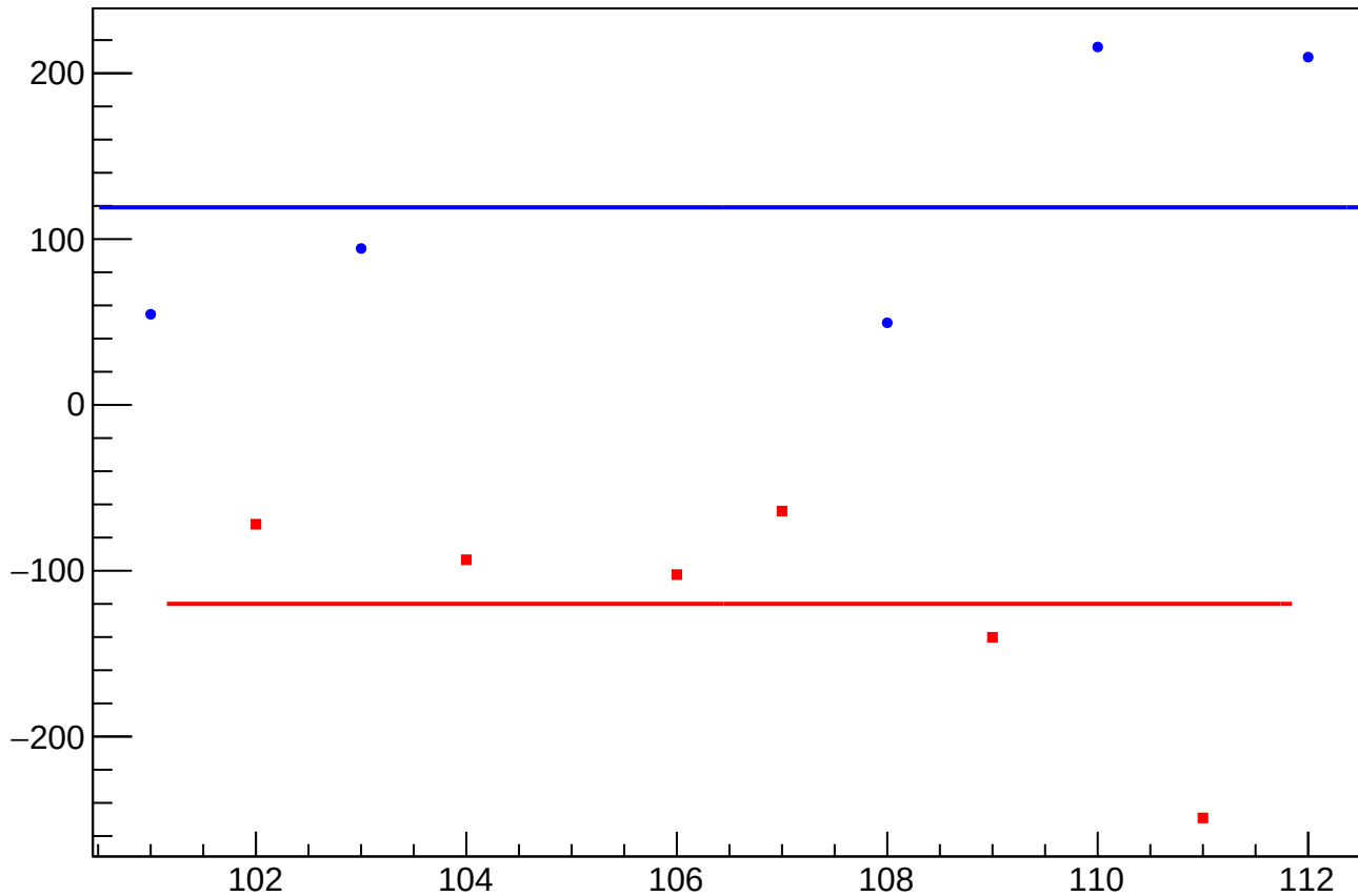
dit_4aX_coil7_mean vs Slug, Sign Corrected
