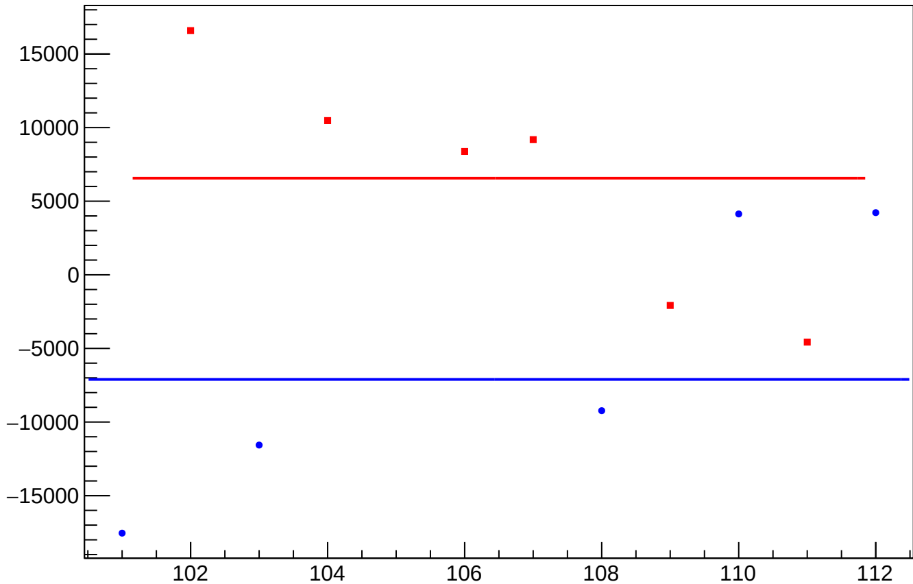
dit_atr2_coil6_mean vs Slug, Sign Corrected
