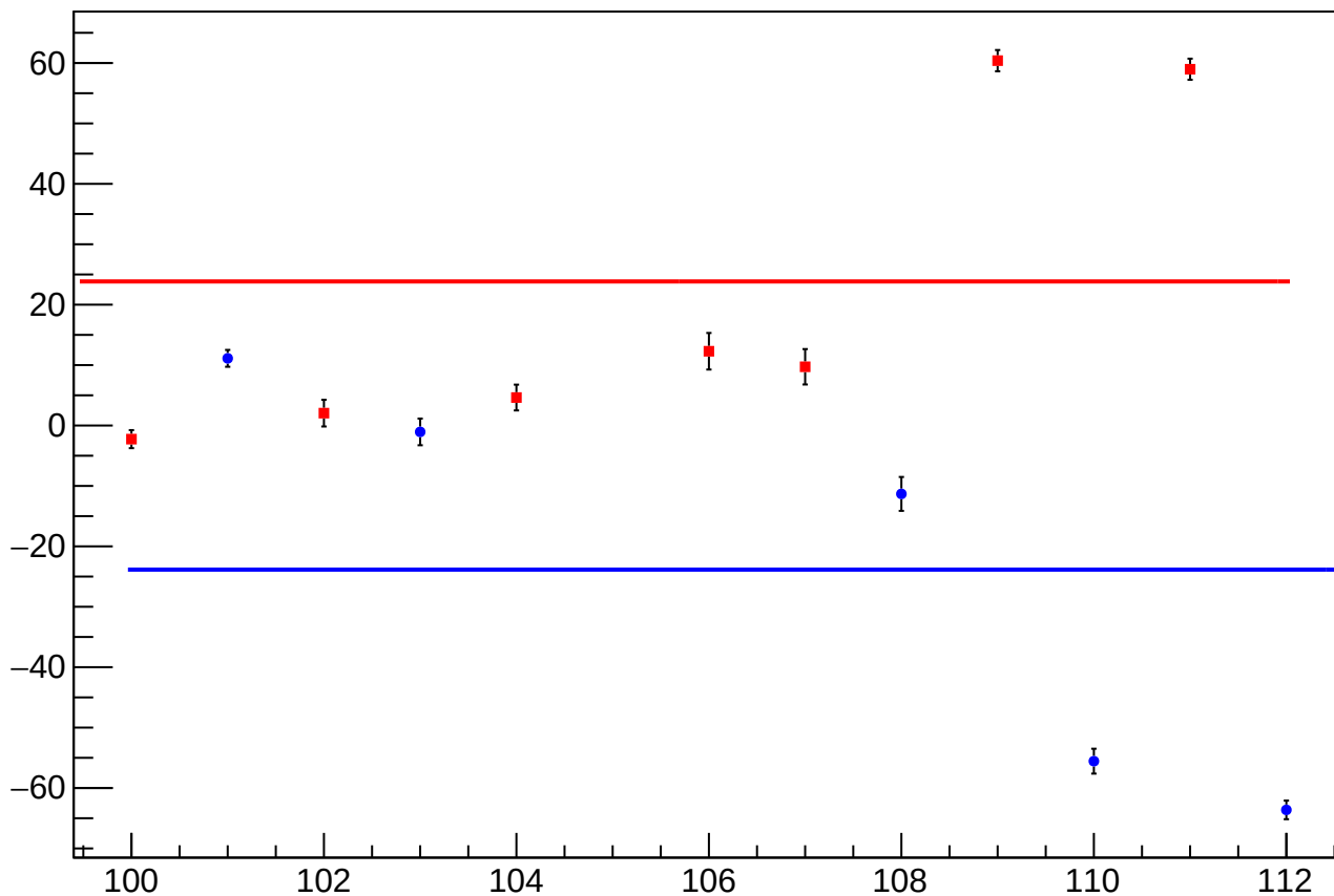
reg_asym_right_dd_diff_bpm4aX_slope vs Slug, Sign Corrected
