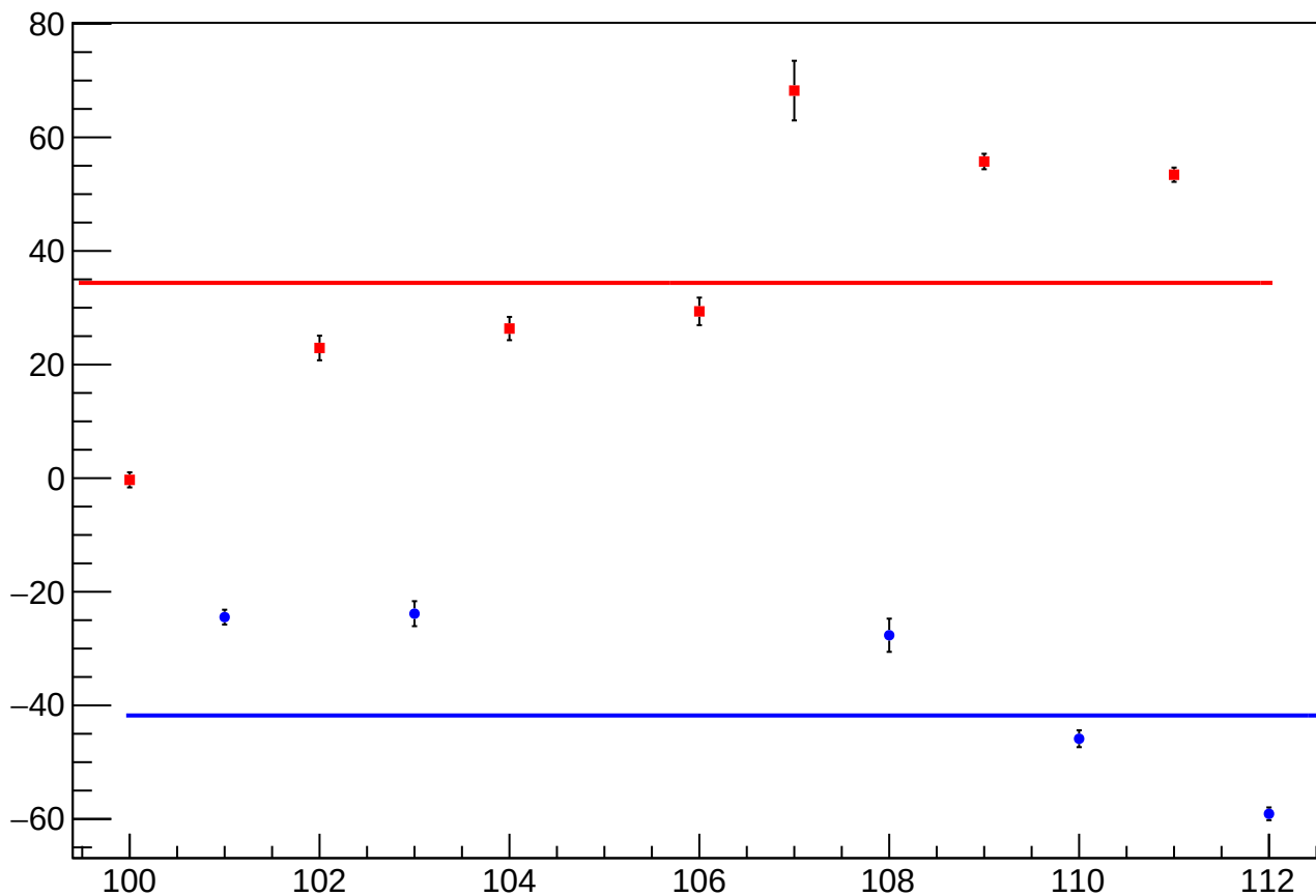
reg_asym_left_dd_diff_bpm4aX_slope vs Slug, Sign Corrected
