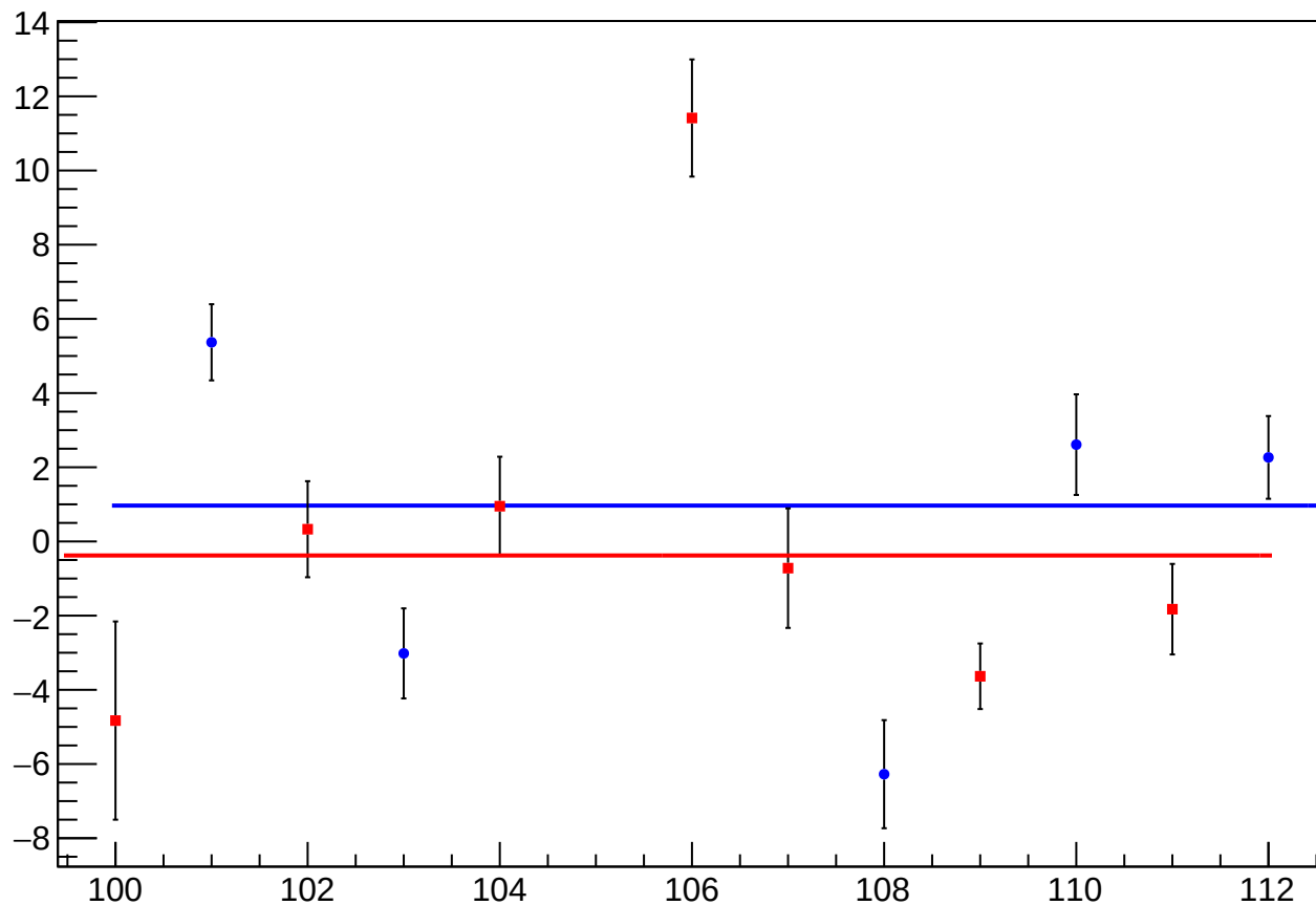
reg_asym_sam5_diff_bpm4aX_slope vs Slug, Sign Corrected
