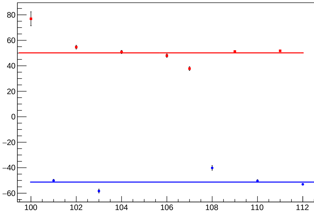
reg_asym_sam_37_dd_diff_bpm4aX_slope vs Slug, Sign Corrected
