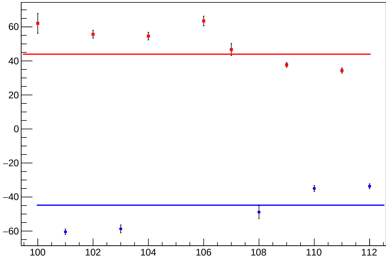
reg_asym_sam_48_dd_diff_bpm4aX_slope vs Slug, Sign Corrected
