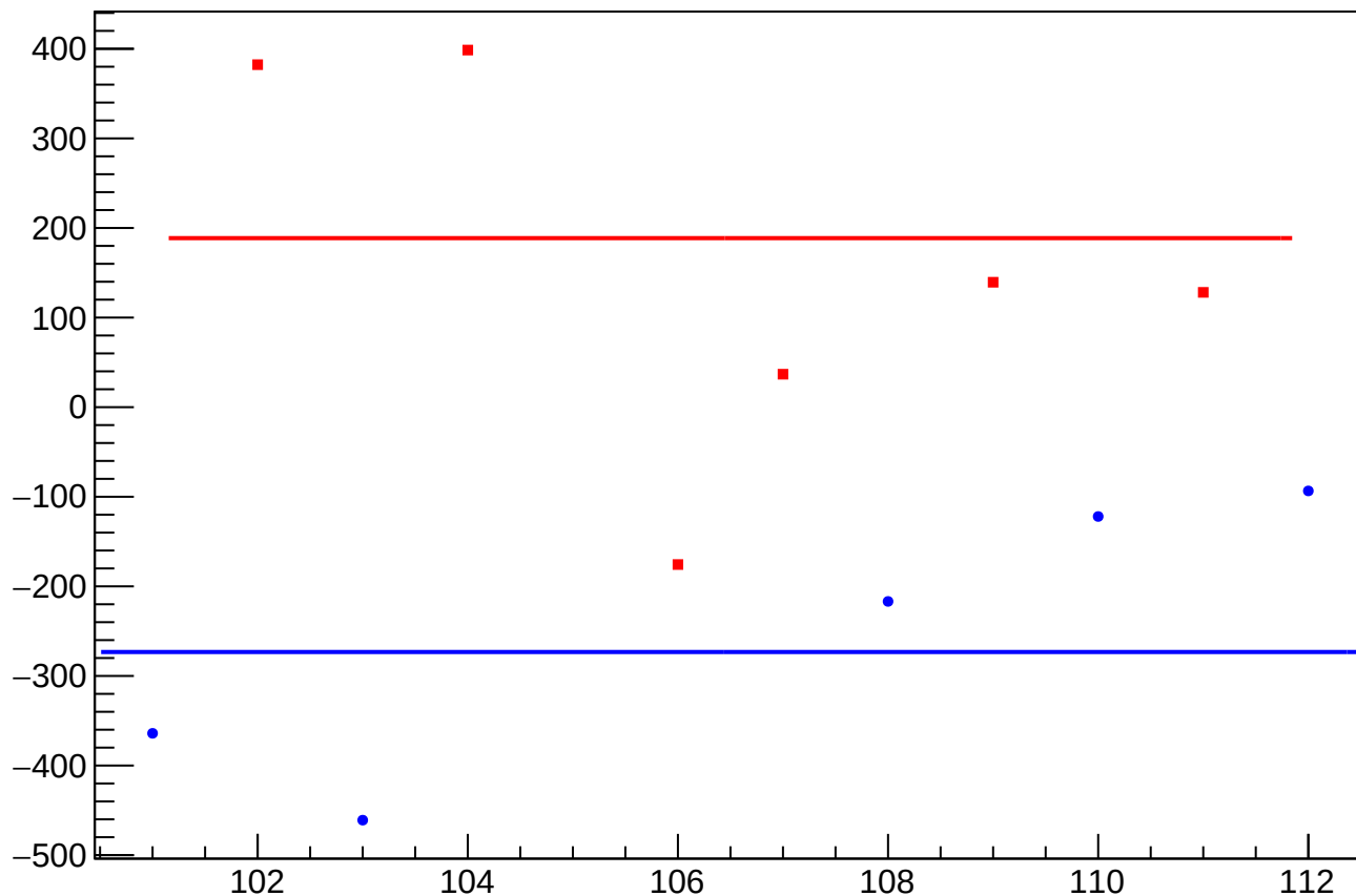
dit_sam1_coil3_mean vs Slug, Sign Corrected
