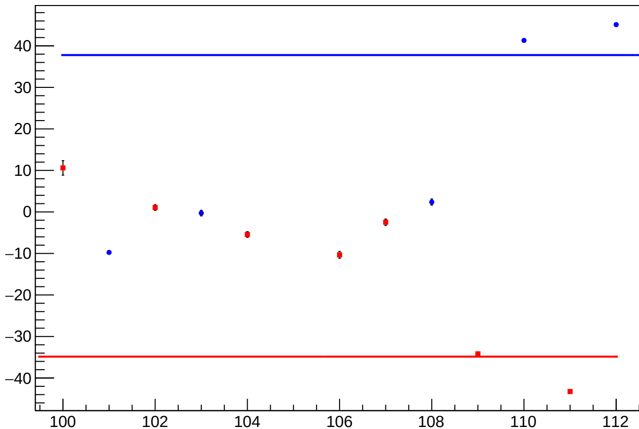
reg_asym_sam8_diff_bpm4aX_slope vs Slug, Sign Corrected
