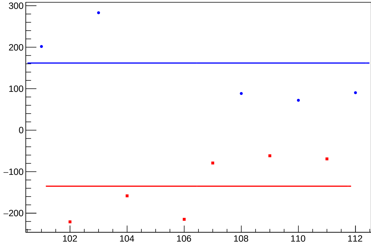
dit_sam5_coil6_err_mean vs Slug, Sign Corrected
