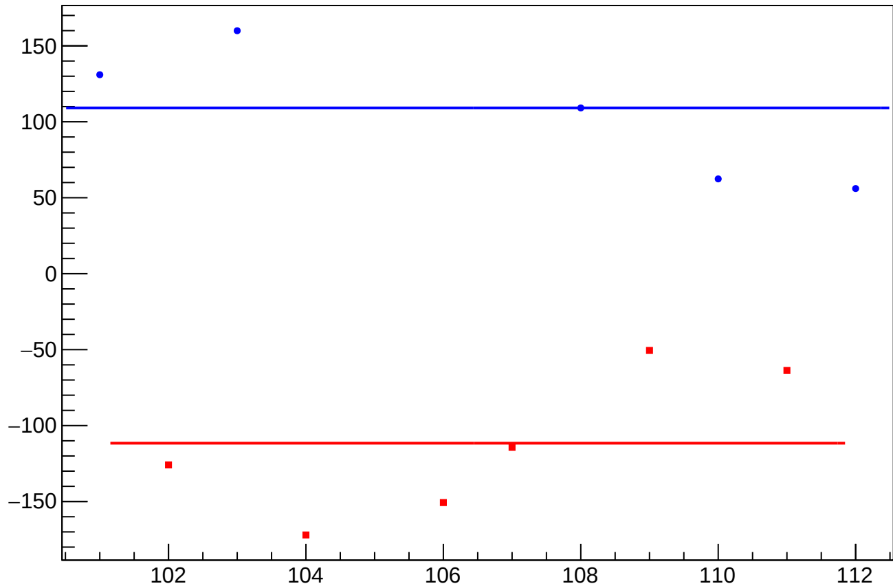
dit_sam6_coil3_err_mean vs Slug, Sign Corrected
