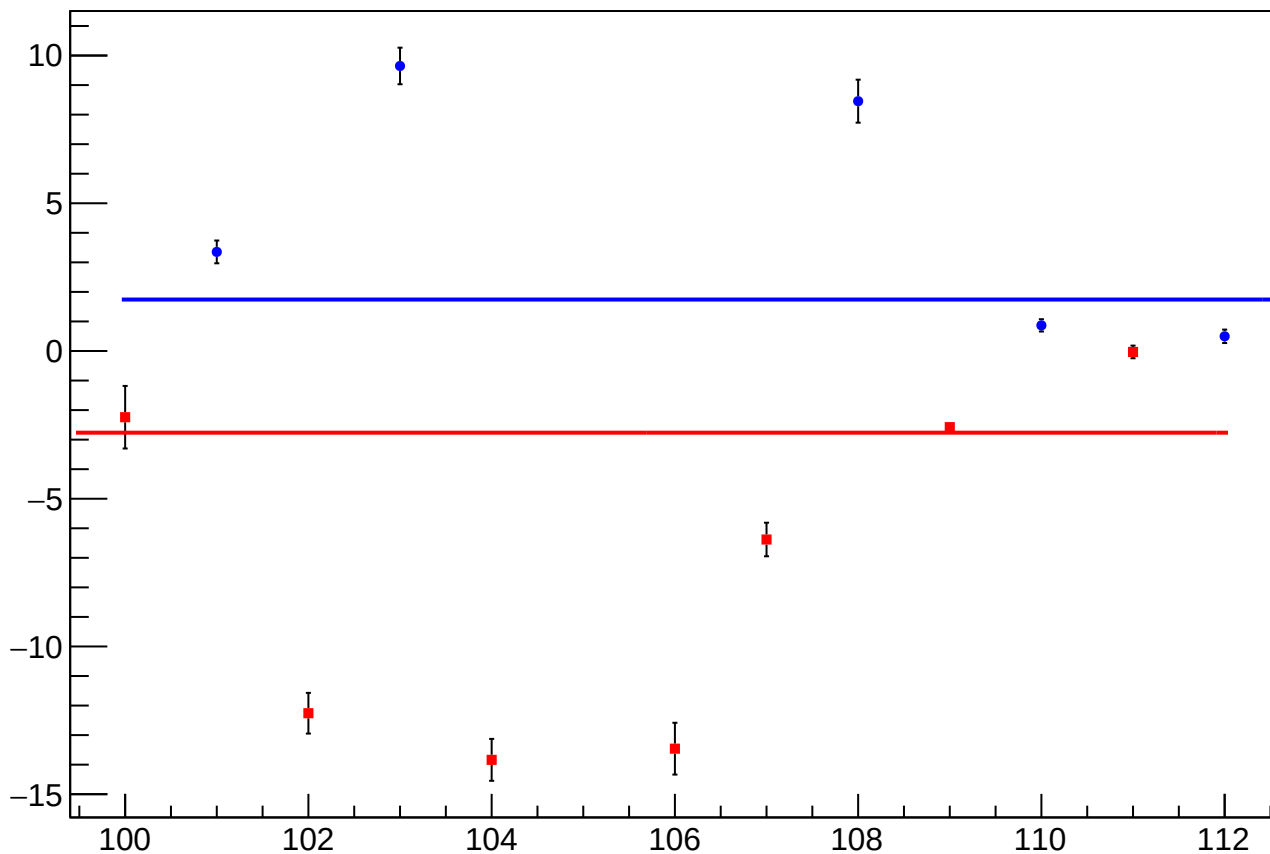
reg_asym_bcm_an_ds3_diff_bpm4aX_slope vs Slug, Sign Corrected
