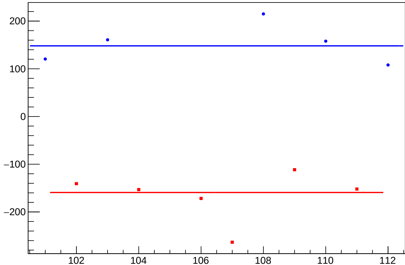
dit_sam6_coil4_err_mean vs Slug, Sign Corrected
