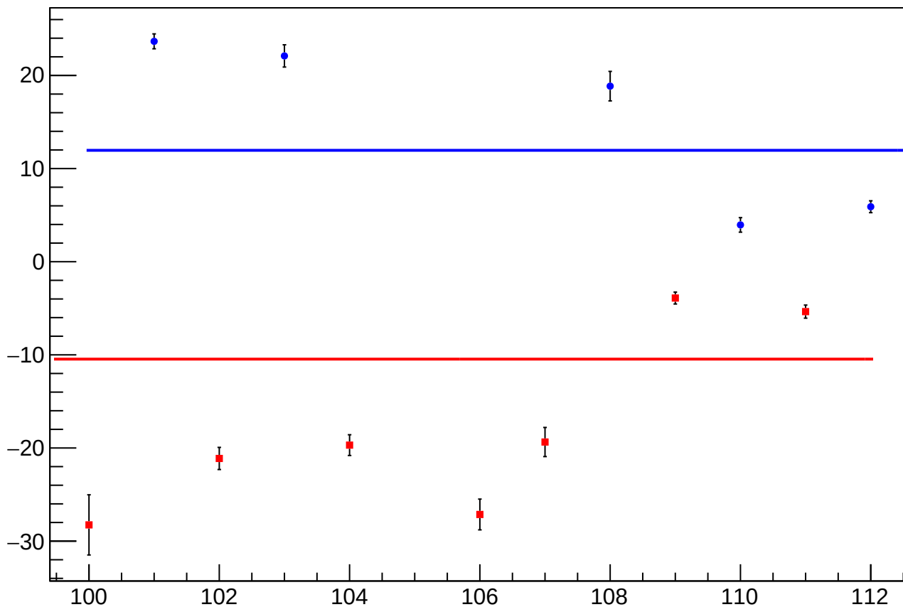
reg_asym_sam_1357_2468_dd_diff_bpm4aX_slope vs Slug, Sign Corrected
