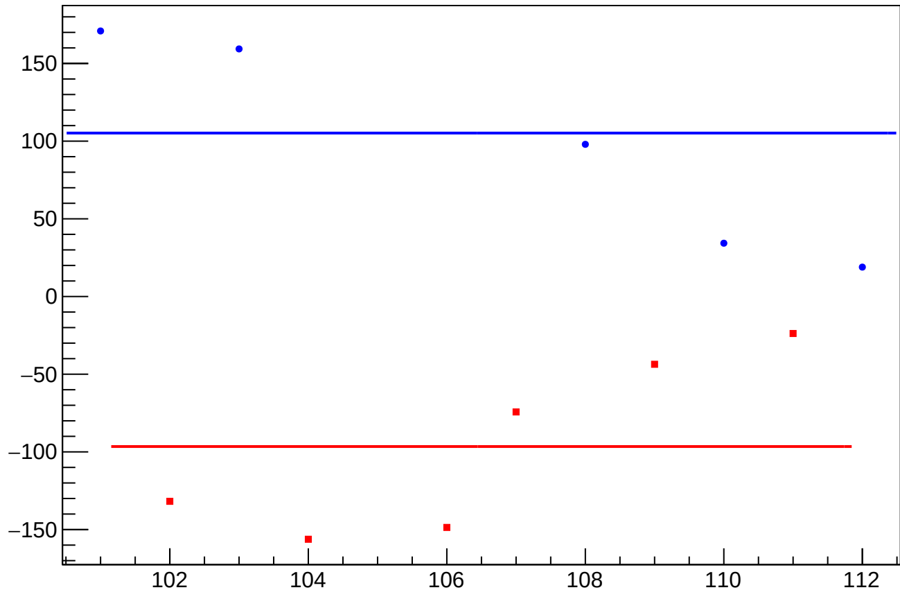
dit_sam8_coil3_err_mean vs Slug, Sign Corrected
