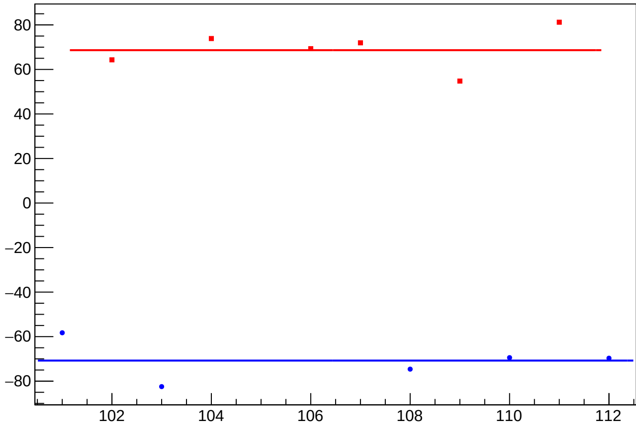
dit_11X12X_coil3_mean vs Slug, Sign Corrected
