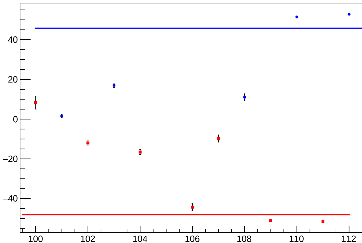
reg_asym_sam7_diff_bpm4aX_slope vs Slug, Sign Corrected
