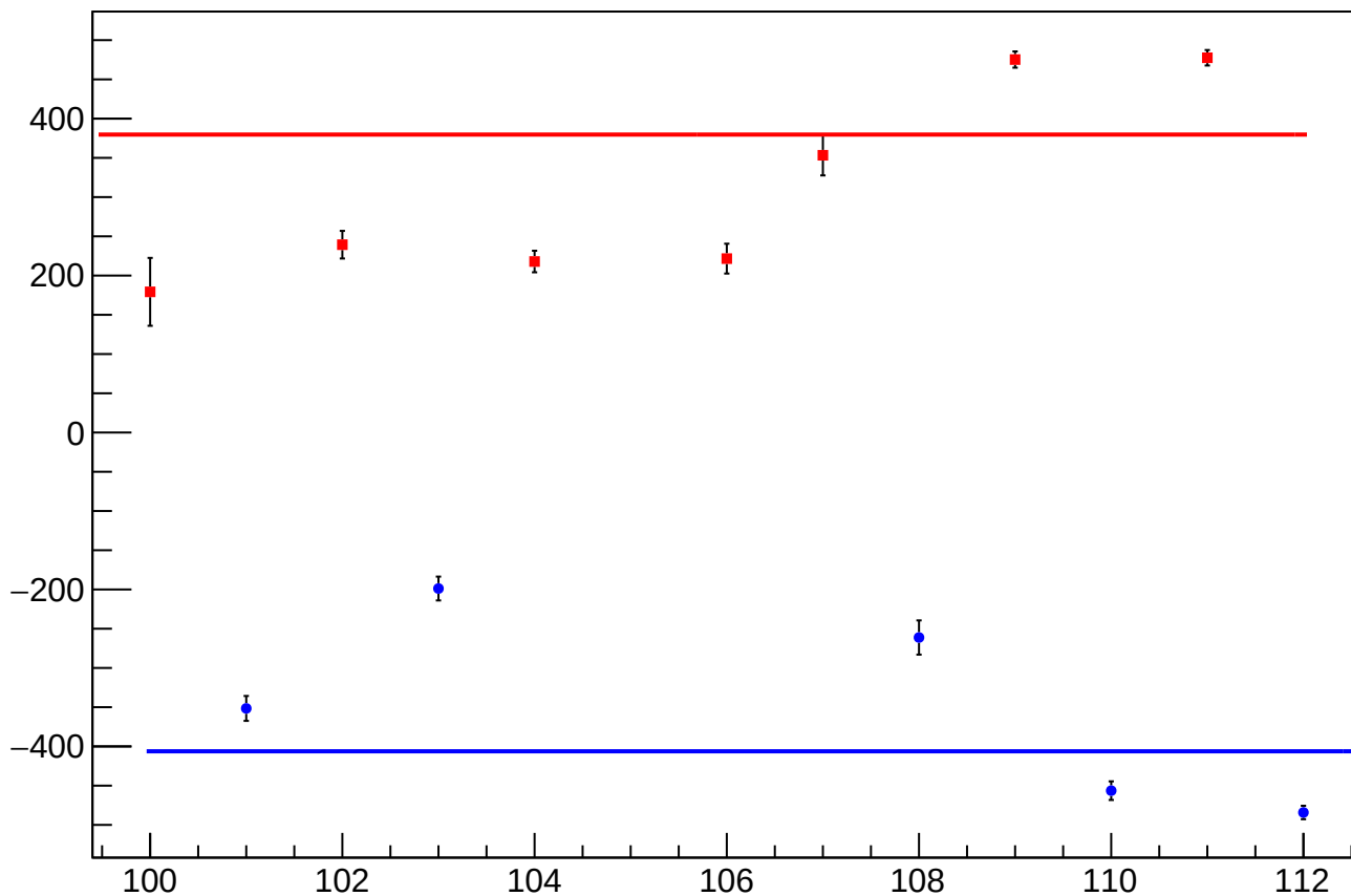
reg_asym_atl2_diff_bpm4aX_slope vs Slug, Sign Corrected
