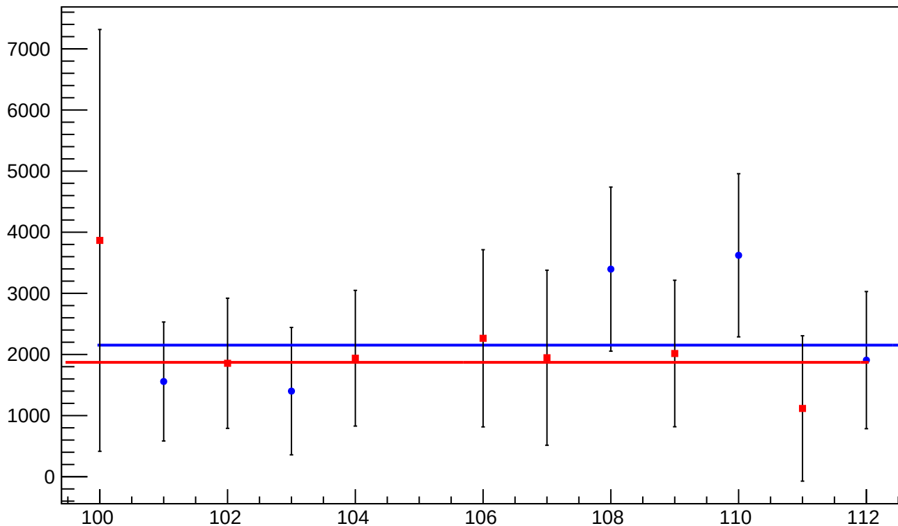
dit_asym_us_avg_mean vs Slug, Sign Corrected
