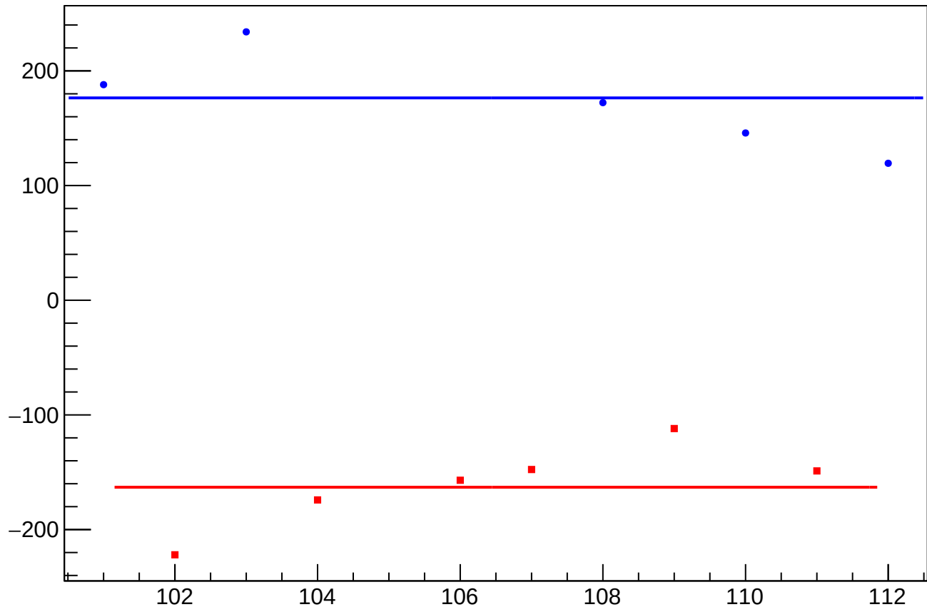
dit_sam6_coil1_err_mean vs Slug, Sign Corrected
