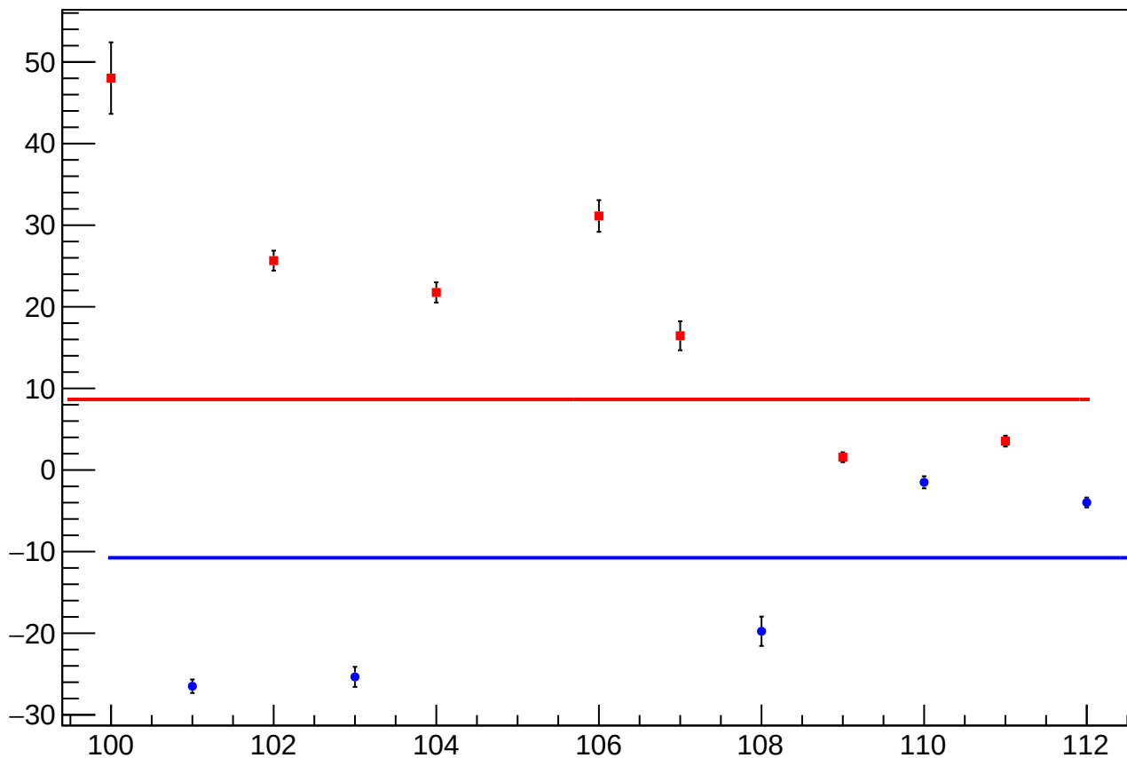
reg_asym_sam_1357_avg_diff_bpm4aX_slope vs Slug, Sign Corrected
