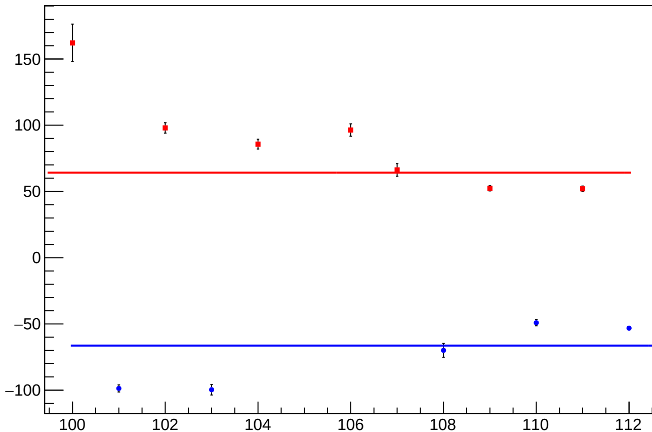
reg_asym_sam3_diff_bpm4aX_slope vs Slug, Sign Corrected
