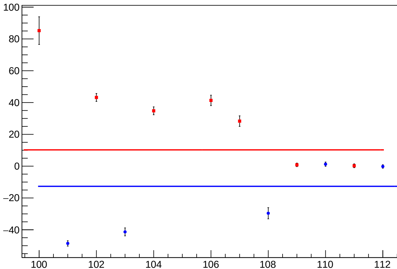
reg_asym_sam_37_avg_diff_bpm4aX_slope vs Slug, Sign Corrected
