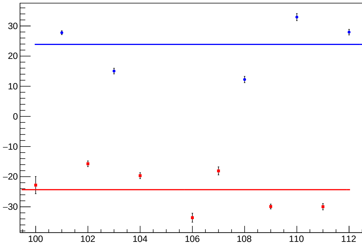
reg_asym_sam6_diff_bpm4aX_slope vs Slug, Sign Corrected
