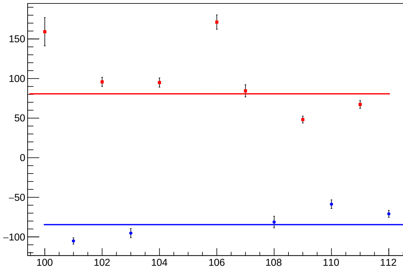
reg_asym_sam_26_dd_diff_bpm4aX_slope vs Slug, Sign Corrected
