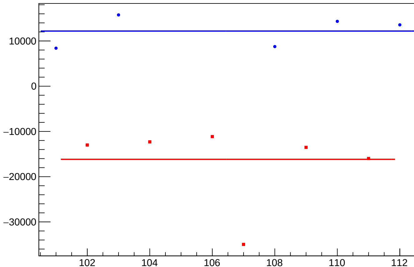
dit_usl_coil7_mean vs Slug, Sign Corrected
