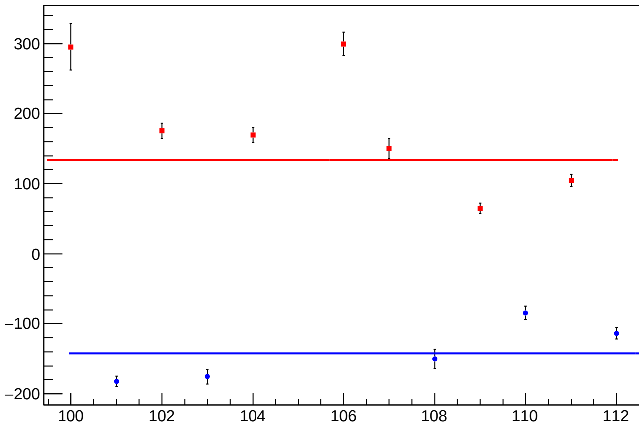
reg_asym_sam2_diff_bpm4aX_slope vs Slug, Sign Corrected
