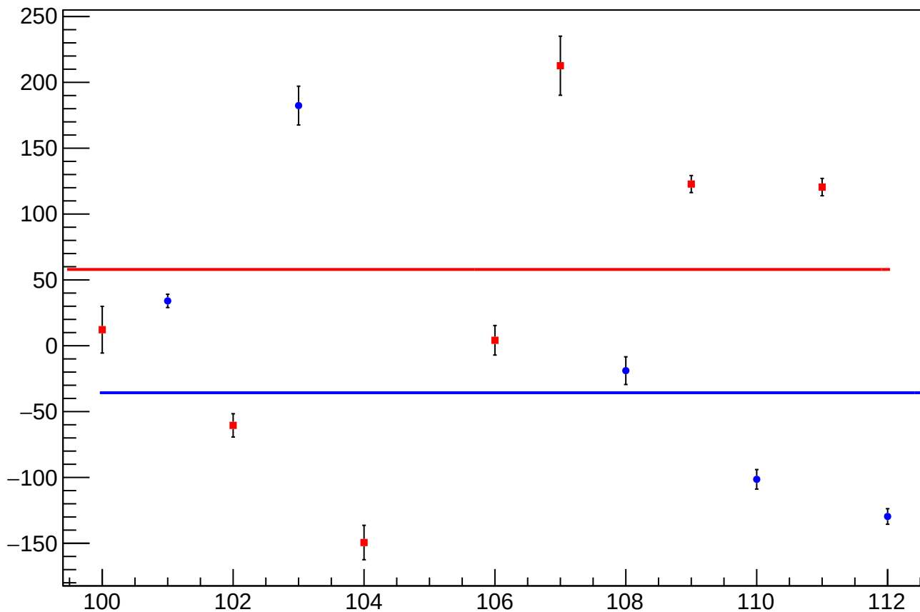
reg_asym_atl1_diff_bpm4aX_slope vs Slug, Sign Corrected
