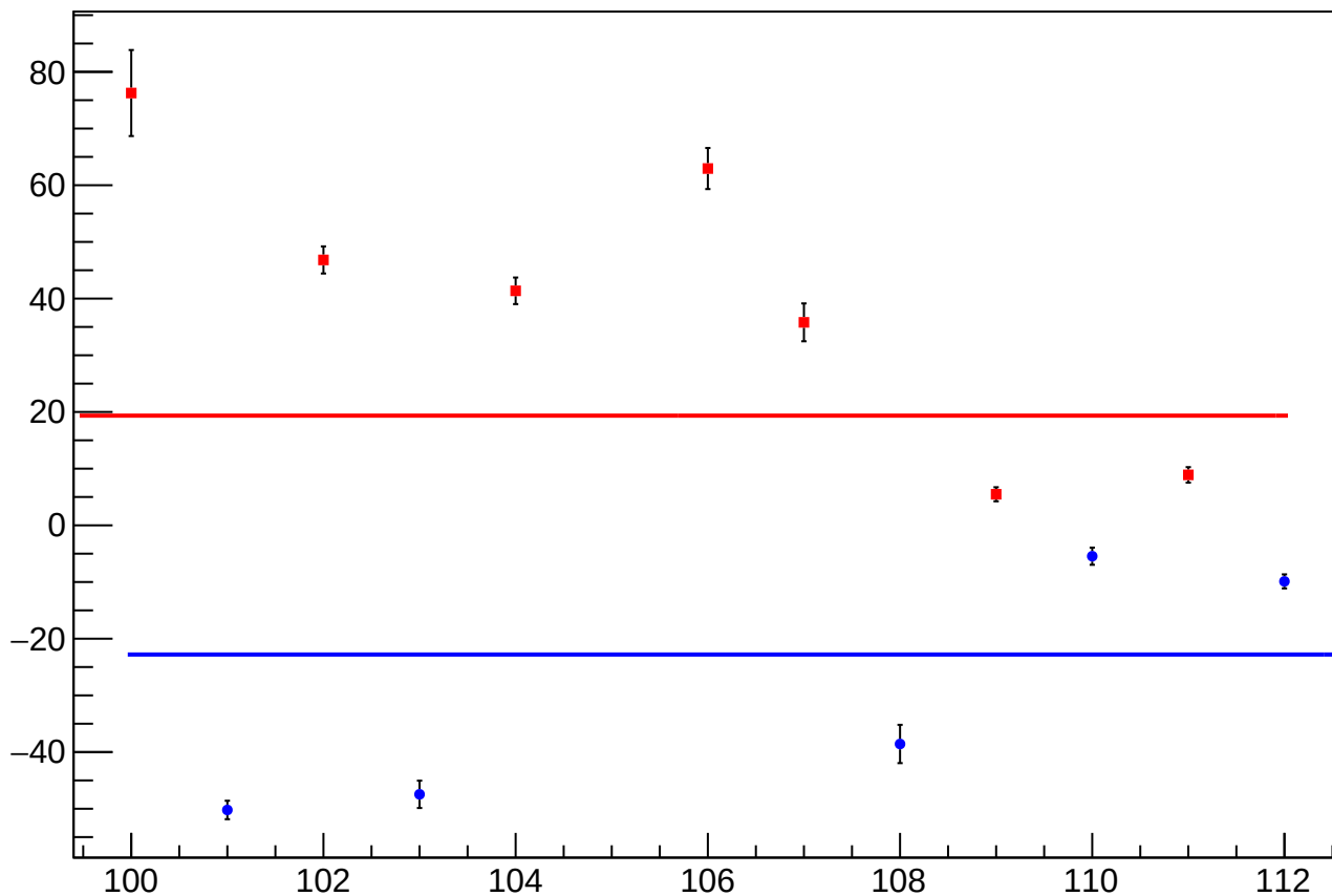
reg_asym_sam_12345678_avg_diff_bpm4aX_slope vs Slug, Sign Corrected
