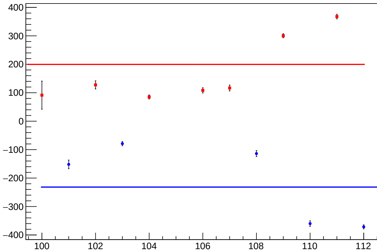
reg_asym_atr_avg_diff_bpm4aX_slope vs Slug, Sign Corrected
