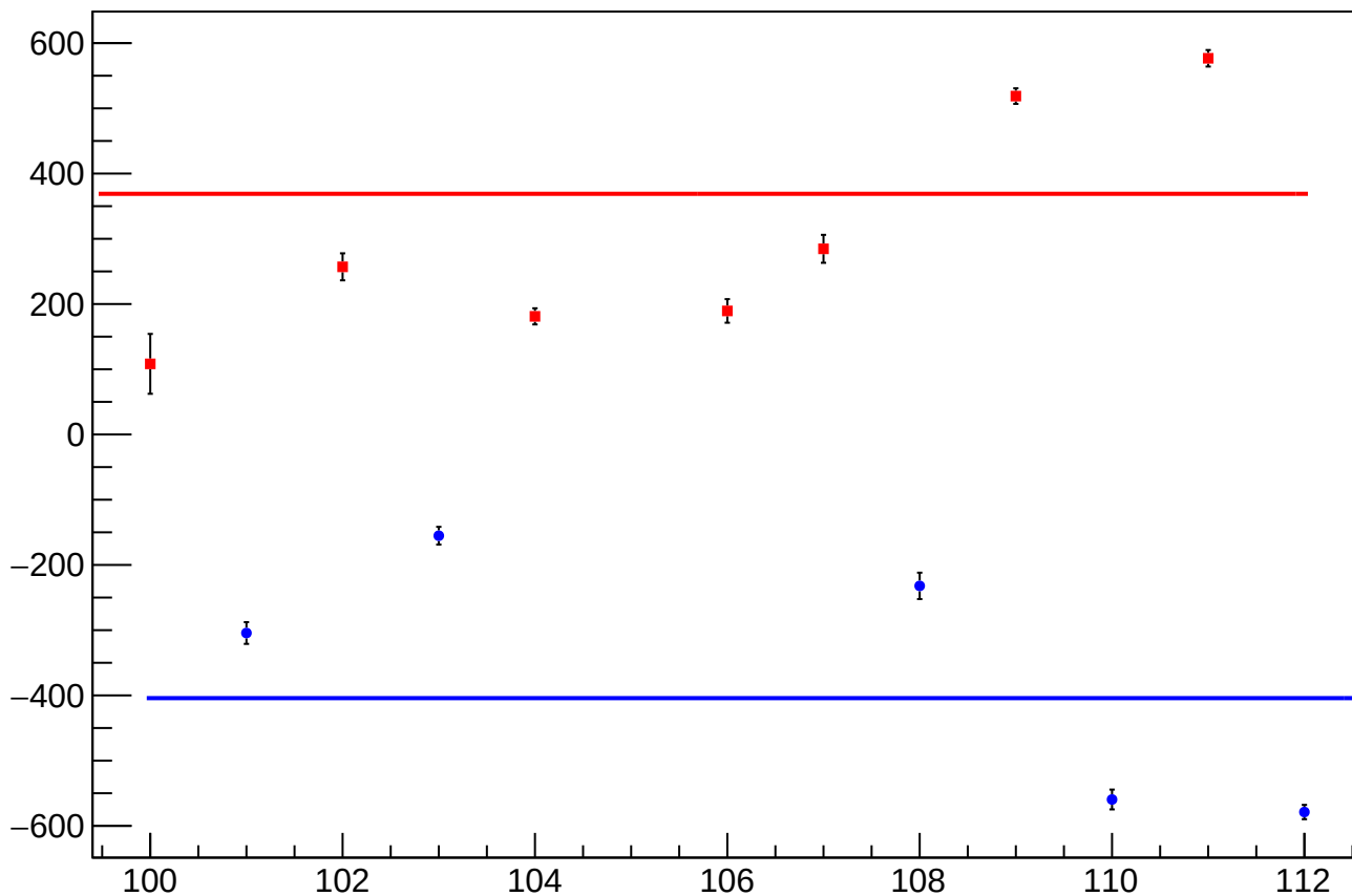
reg_asym_at2_avg_diff_bpm4aX_slope vs Slug, Sign Corrected
