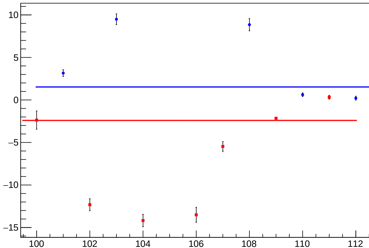
reg_asym_bcm_dg_ds_diff_bpm4aX_slope vs Slug, Sign Corrected
