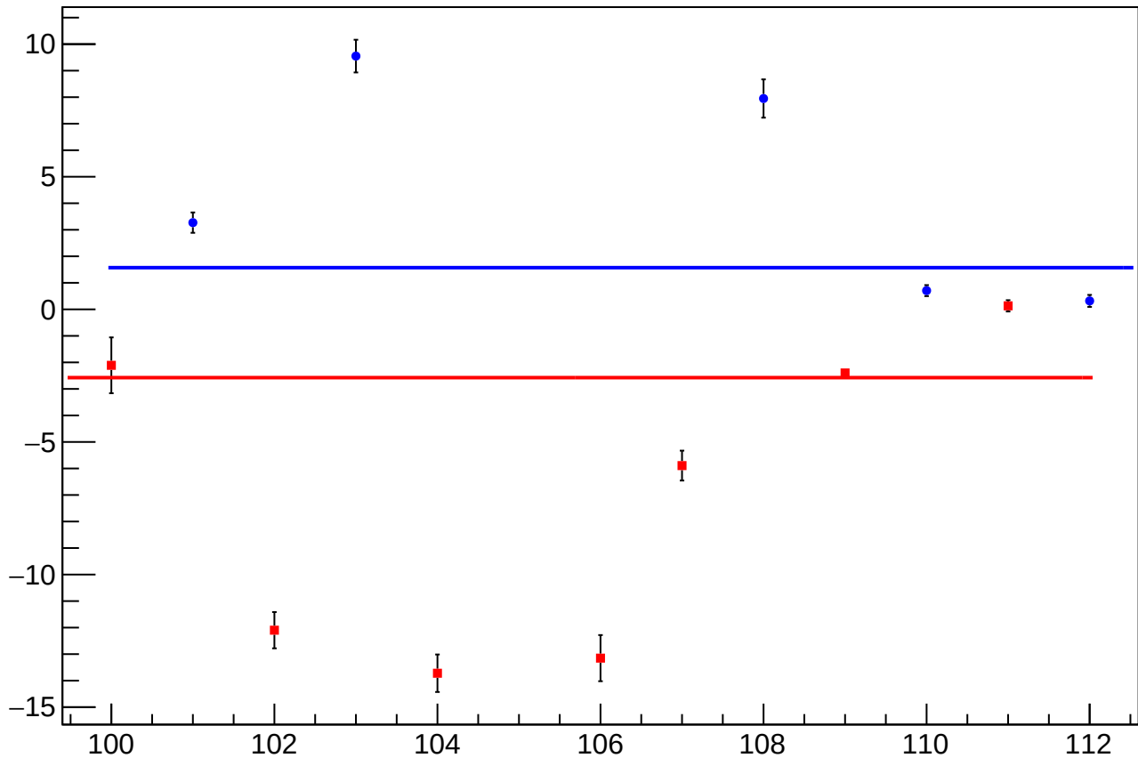
reg_asym_bcm_an_ds_diff_bpm4aX_slope vs Slug, Sign Corrected
