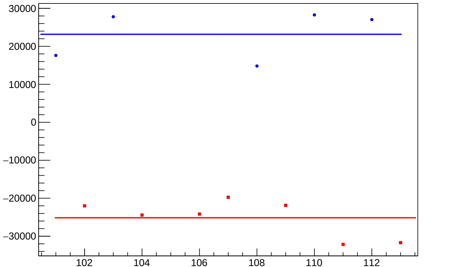
dit_usr_coil7_mean vs Slug, Sign Corrected
