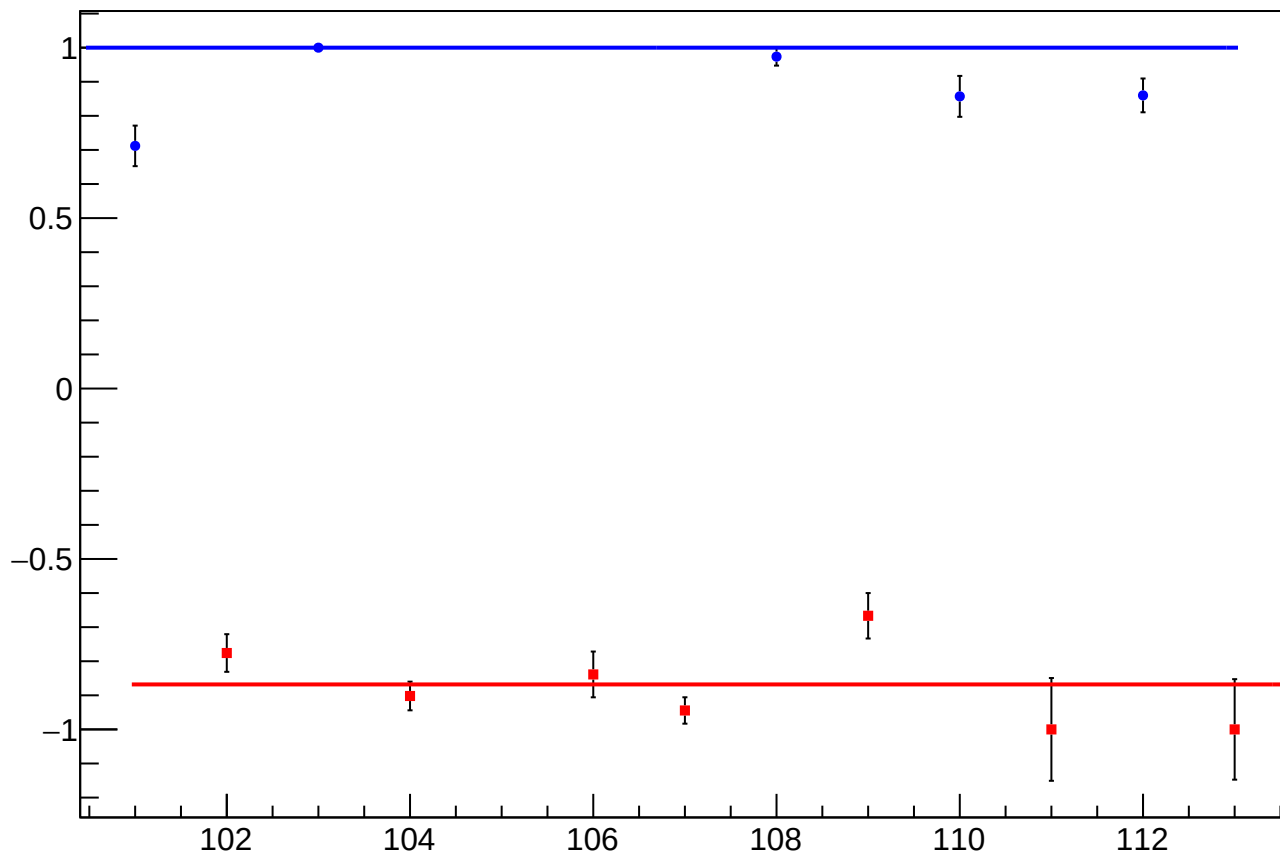
dit_flag_mean vs Slug, Sign Corrected
