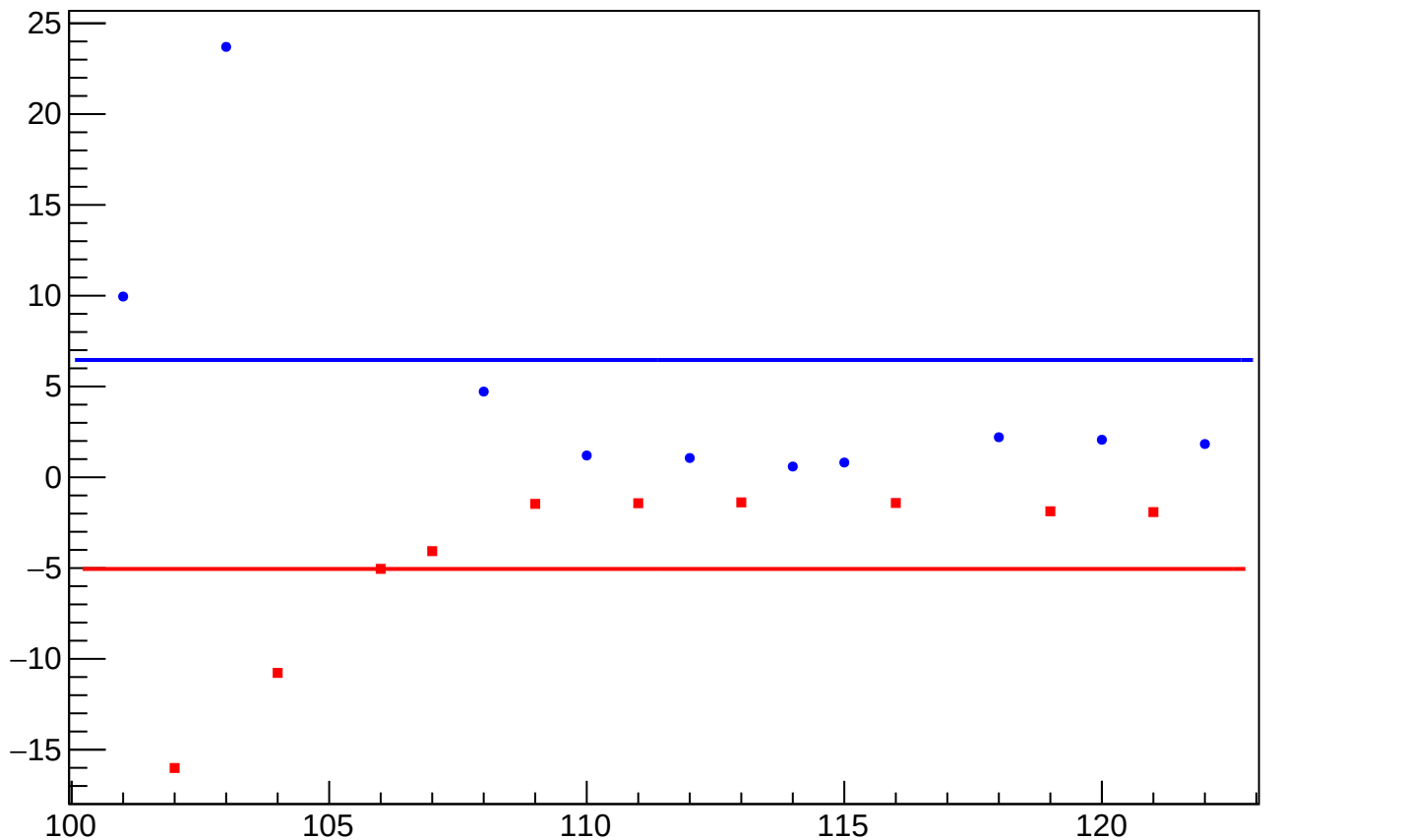
dit_4eX_coil6_err_mean vs Slug, Sign Corrected
