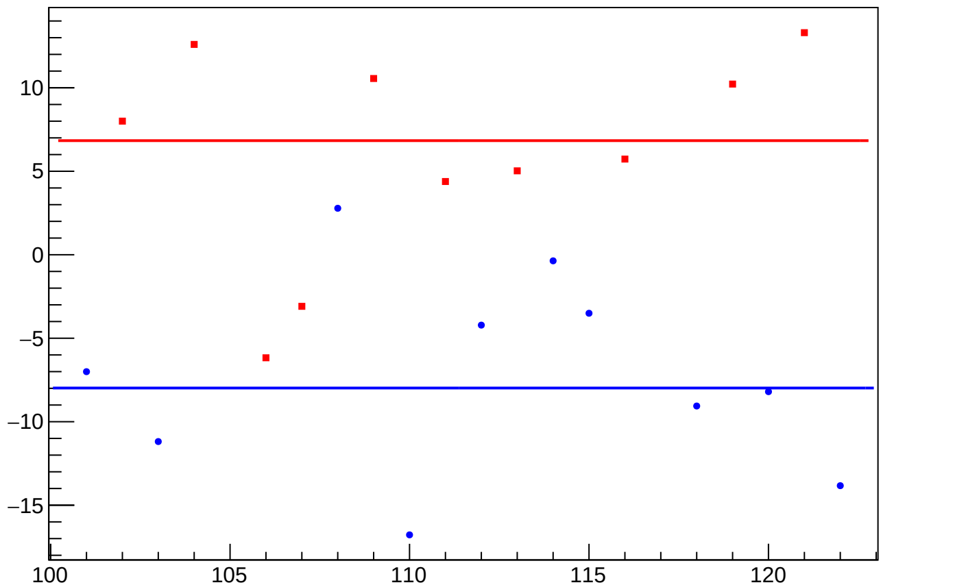
dit_4aY_coil7_mean vs Slug, Sign Corrected
