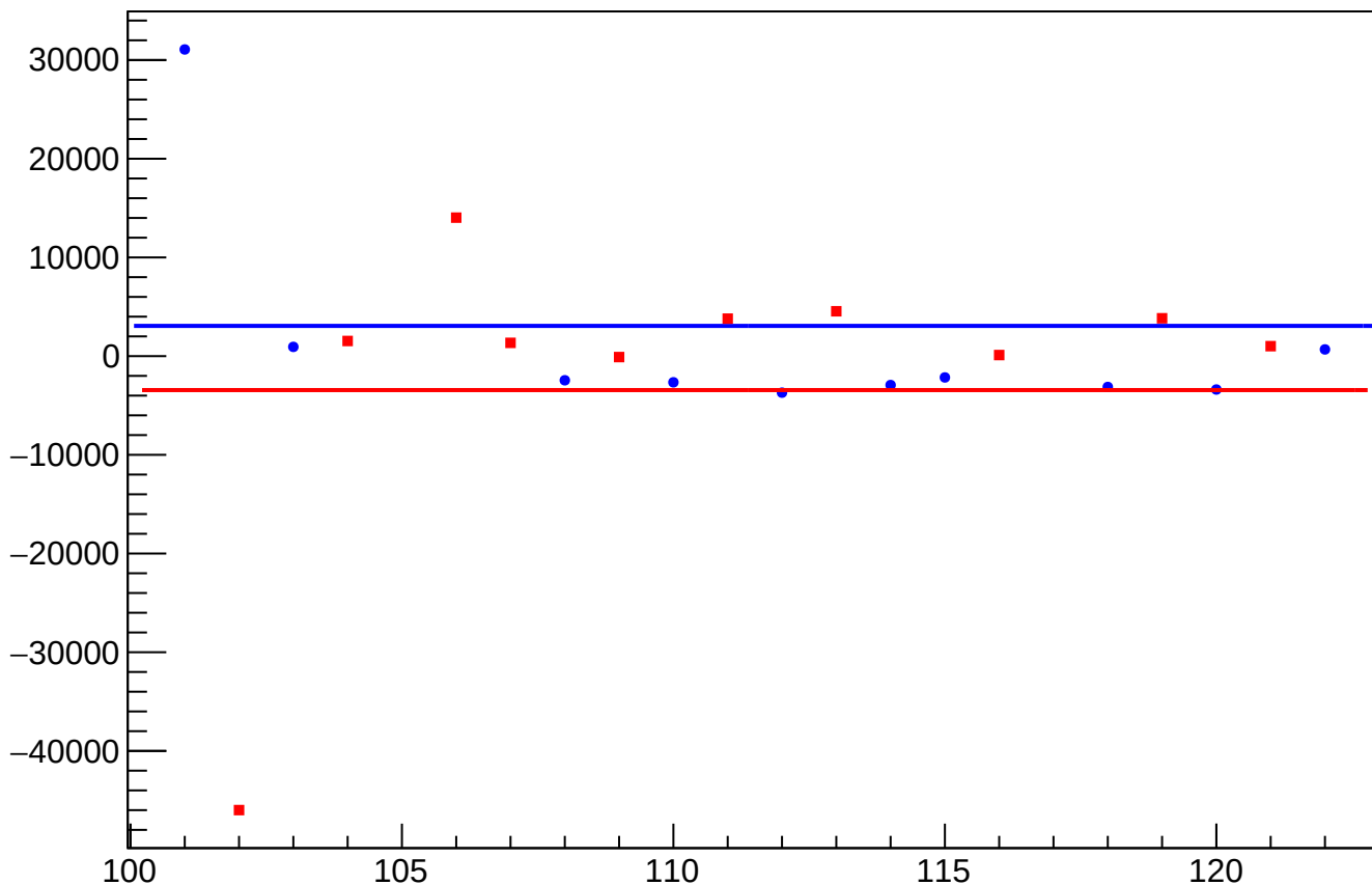
dit_atr1_coil7_mean vs Slug, Sign Corrected
