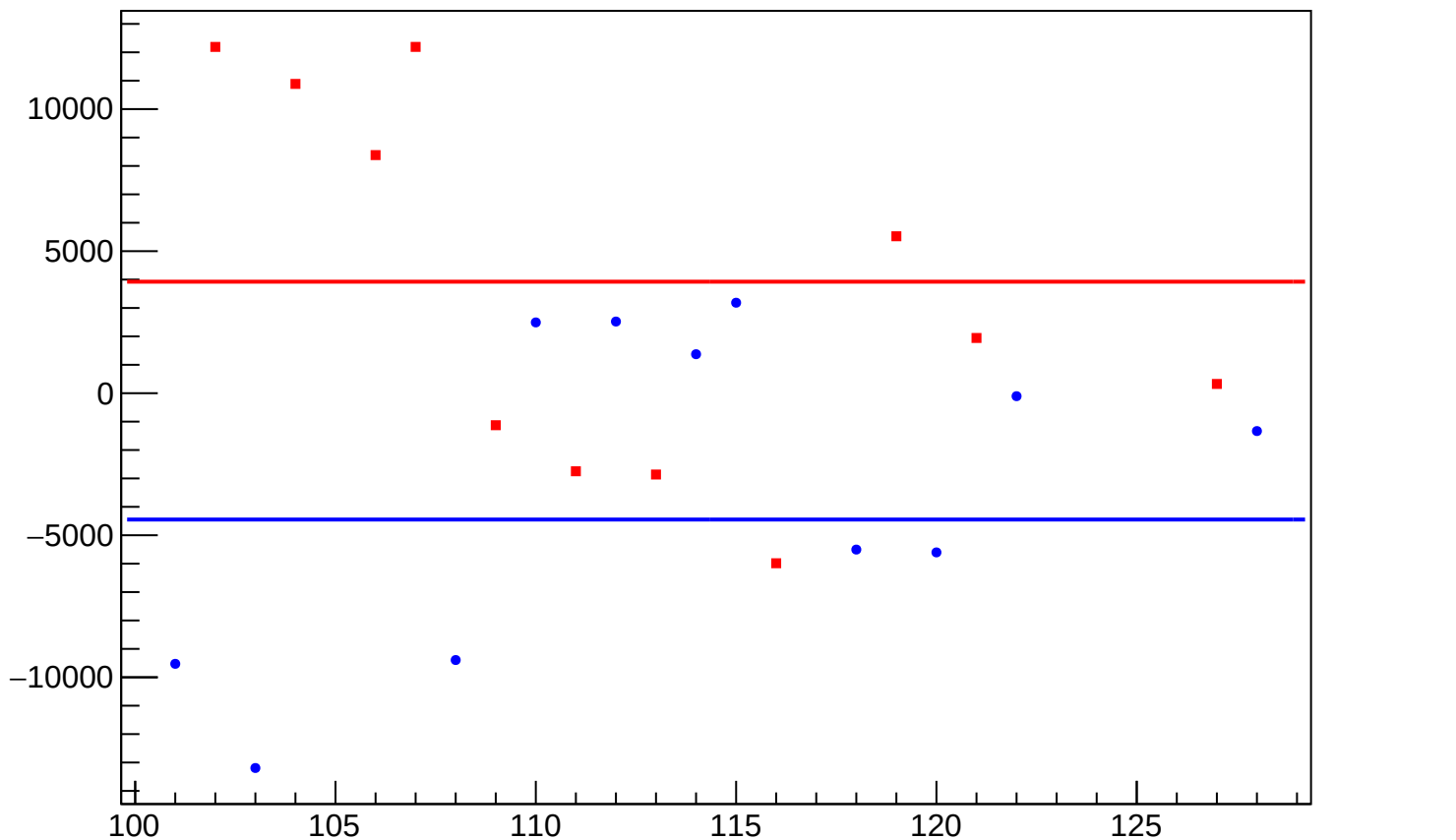
dit_atl2_coil6_mean vs Slug, Sign Corrected
