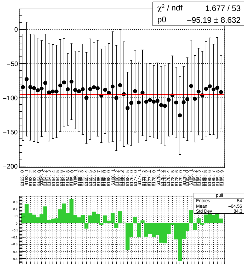
reg_asym_sam2_diff_bpm4aX_slope vs run
