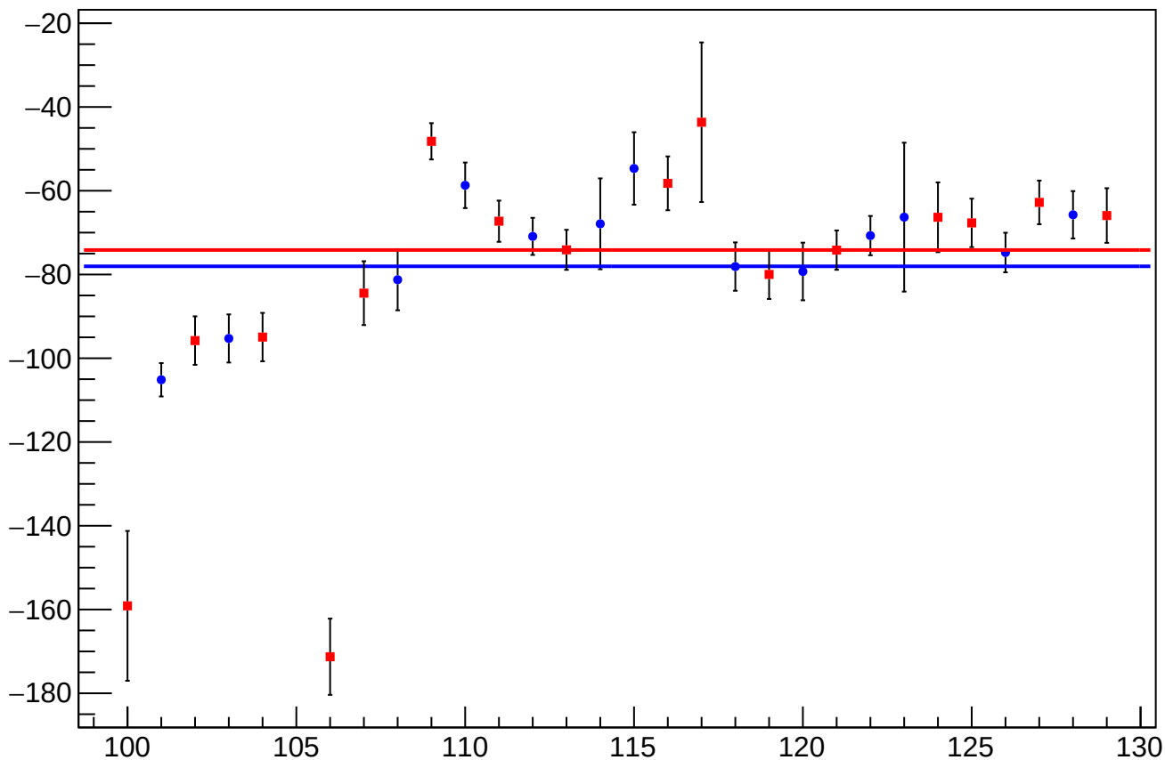
reg_asym_sam_26_dd_diff_bpm4aX_slope vs Slug
