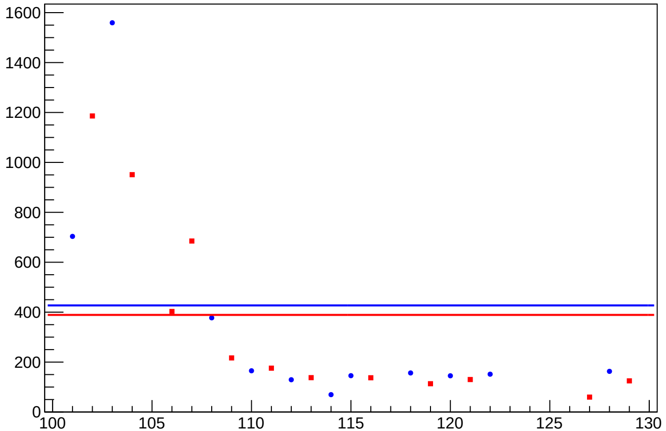
dit_usl_coil6_err_mean vs Slug
