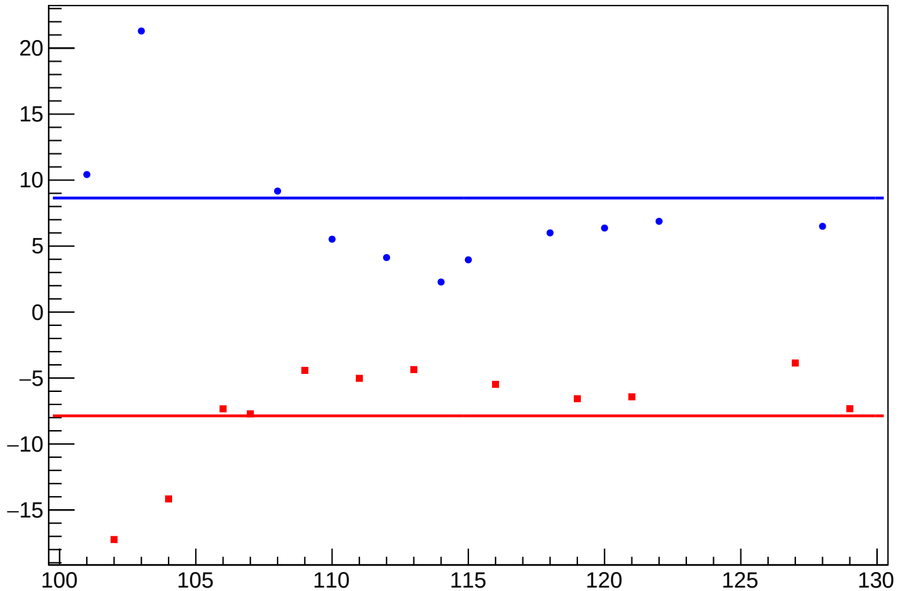
dit_4aX_coil7_err_mean vs Slug, Sign Corrected
