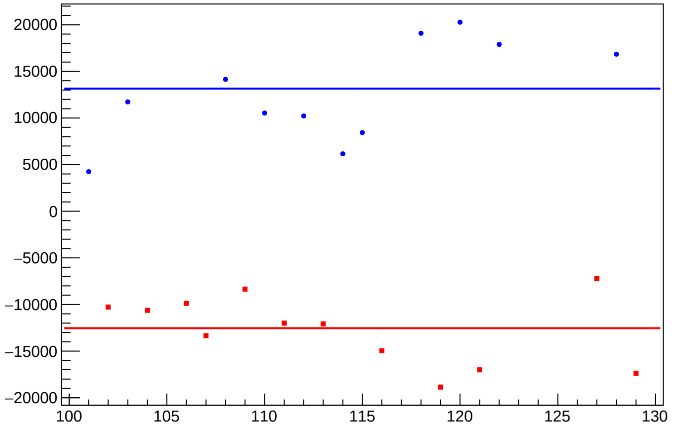
dit_atr1_coil1_mean vs Slug, Sign Corrected
