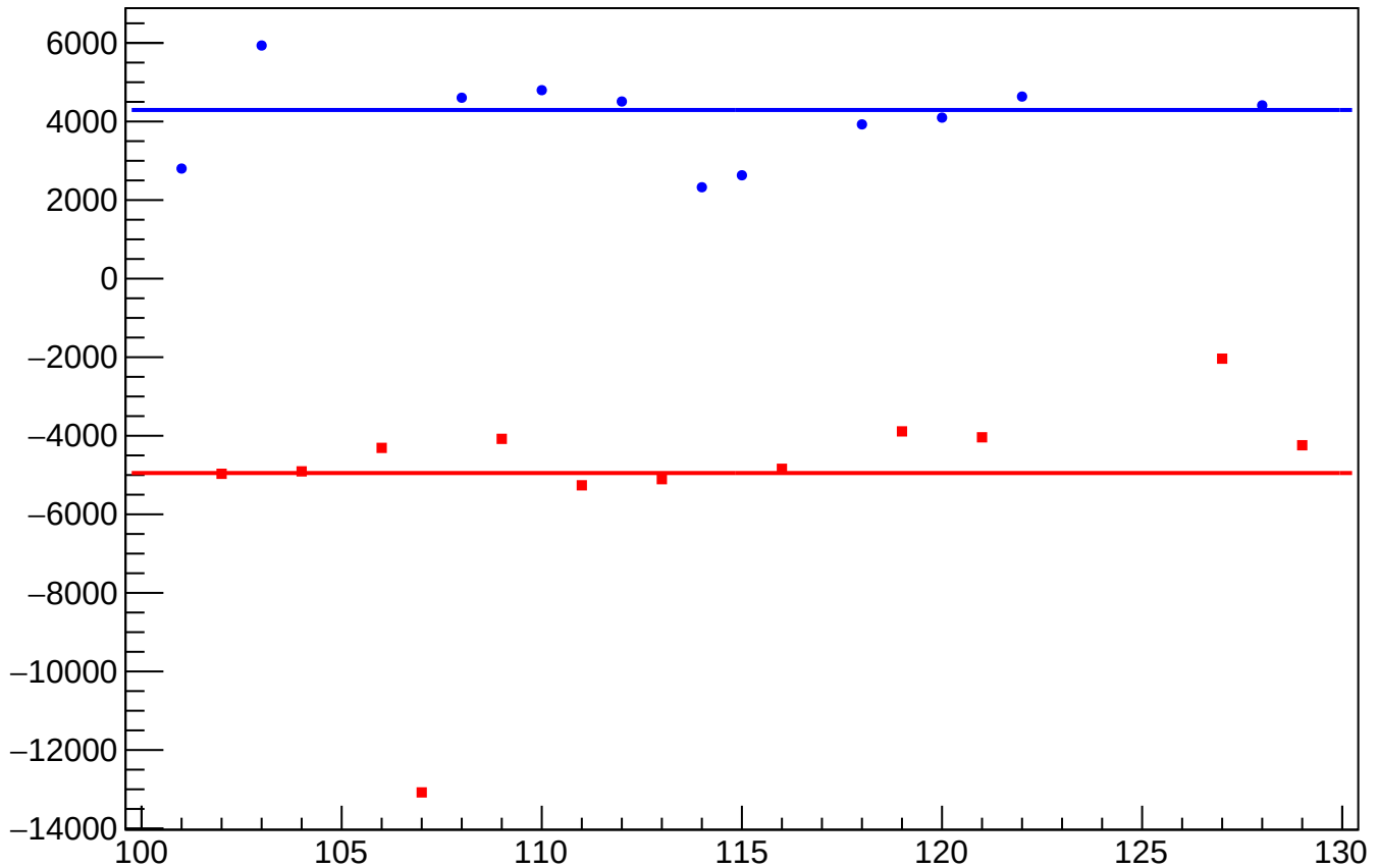
dit_usl_coil4_mean vs Slug, Sign Corrected
