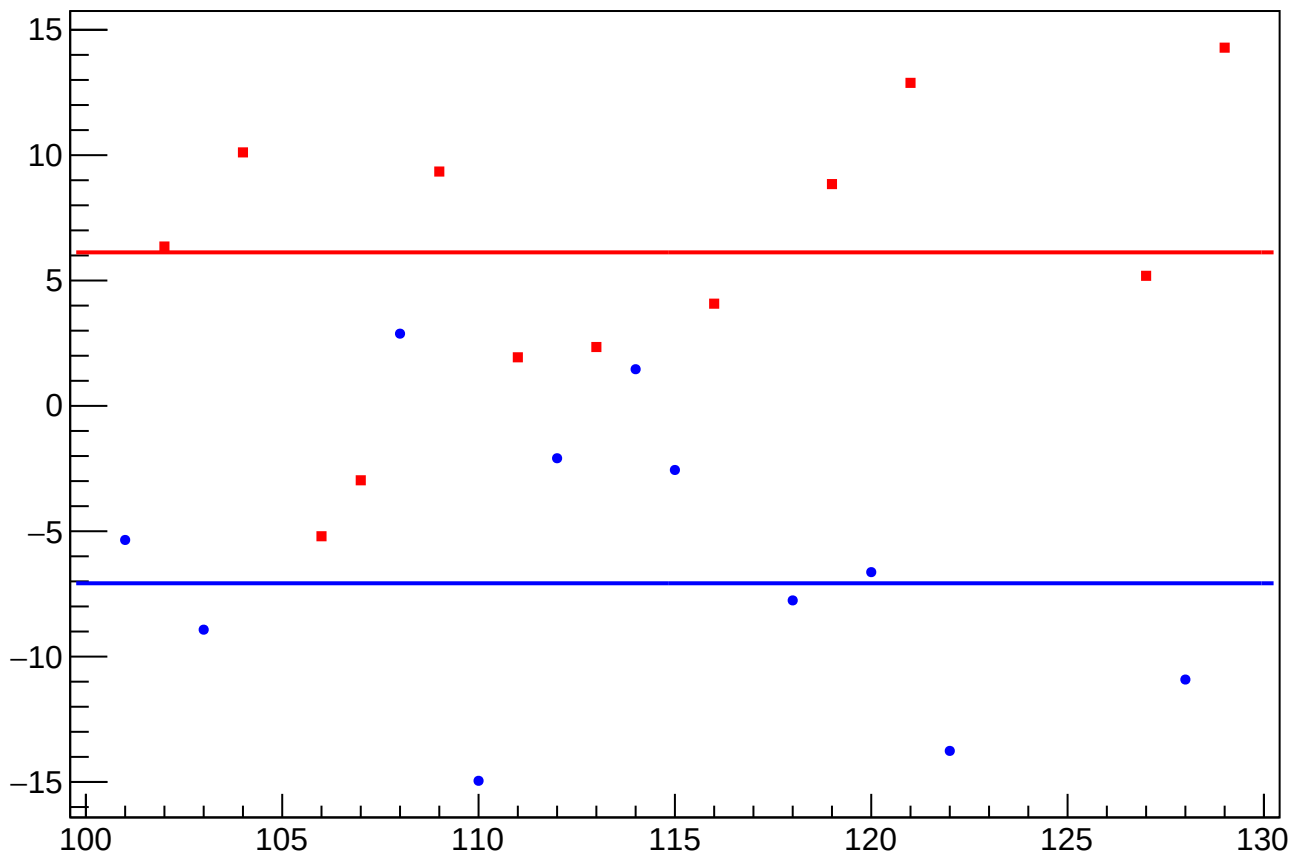
dit_4eY_coil7_mean vs Slug, Sign Corrected
