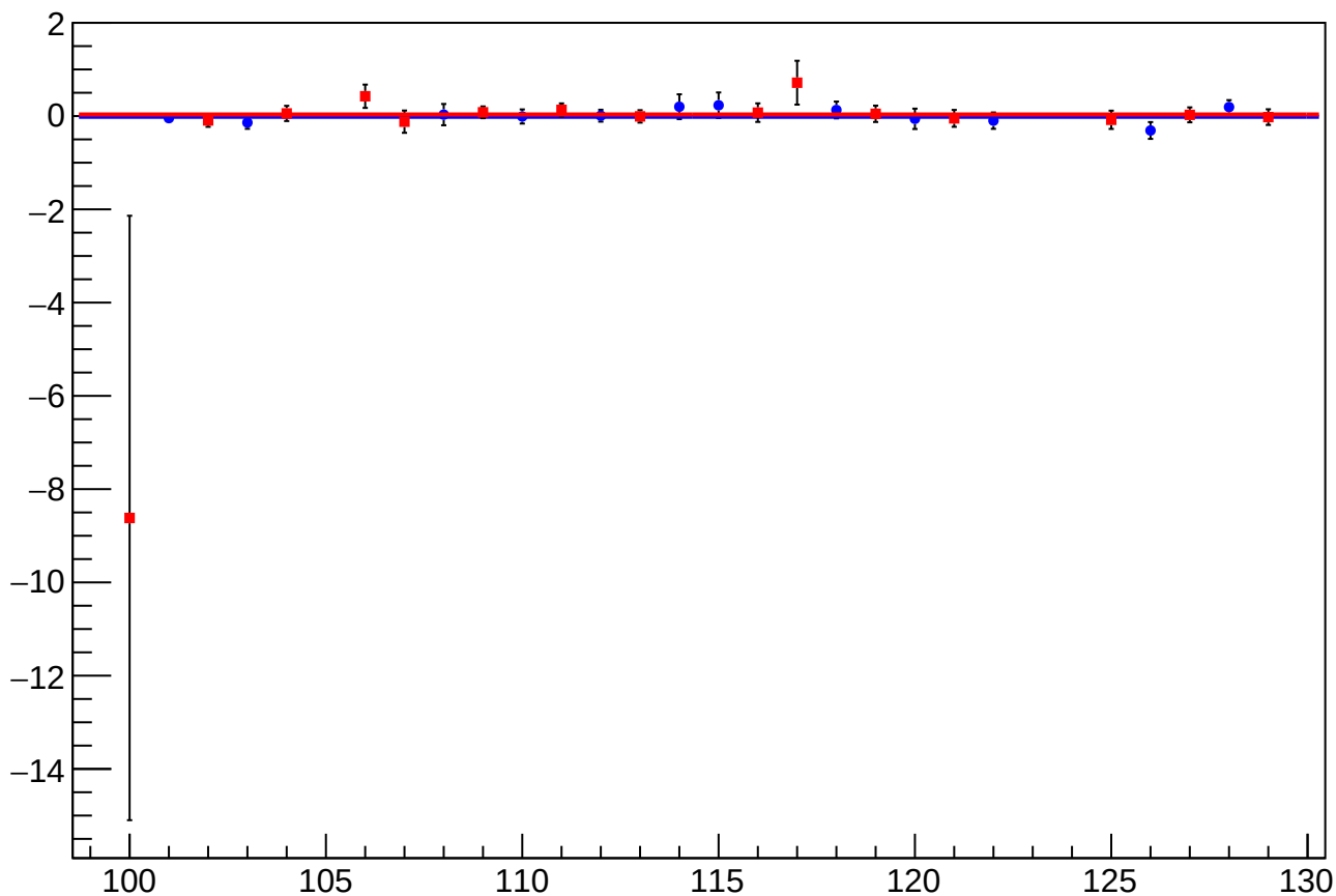
reg_asym_ds_avg_diff_bpm4aX_slope vs Slug, Sign Corrected
