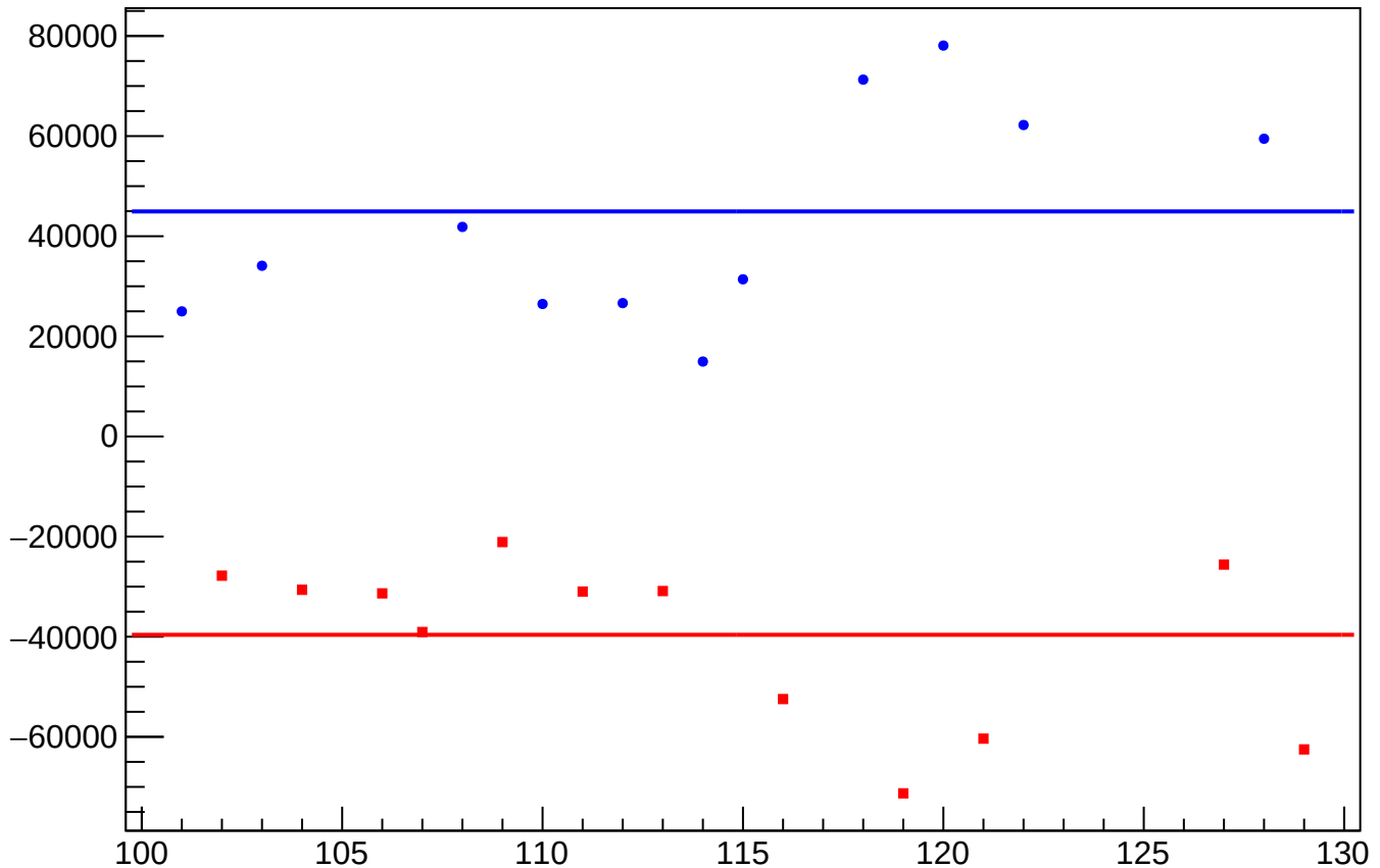
dit_sam4_coil1_mean vs Slug, Sign Corrected
