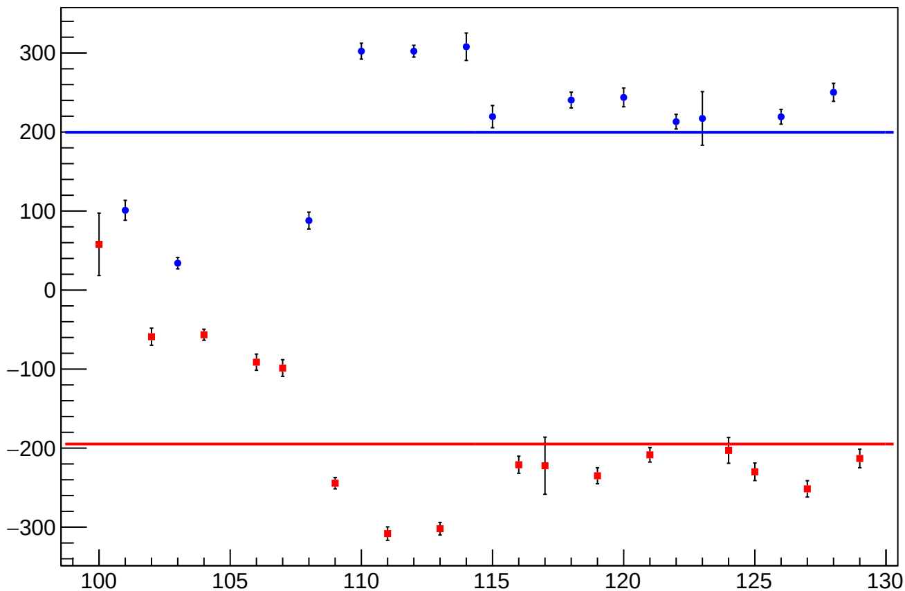
reg_asym_atr_dd_diff_bpm4aX_slope vs Slug, Sign Corrected
