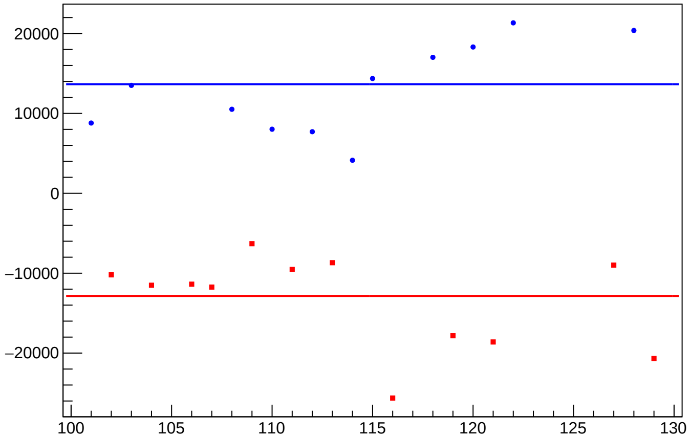
dit_sam6_coil4_mean vs Slug, Sign Corrected
