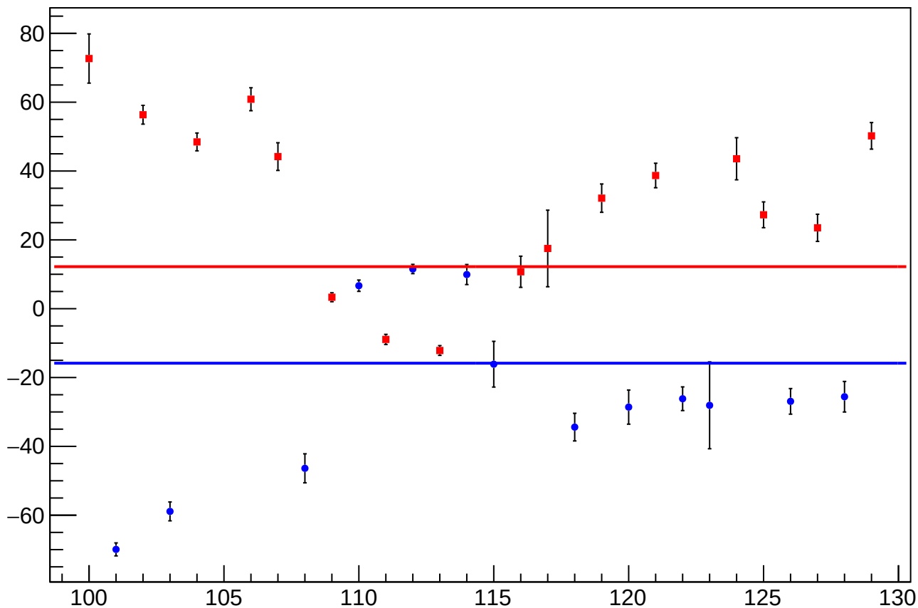
reg_asym_sam_48_avg_diff_bpm4aX_slope vs Slug, Sign Corrected
