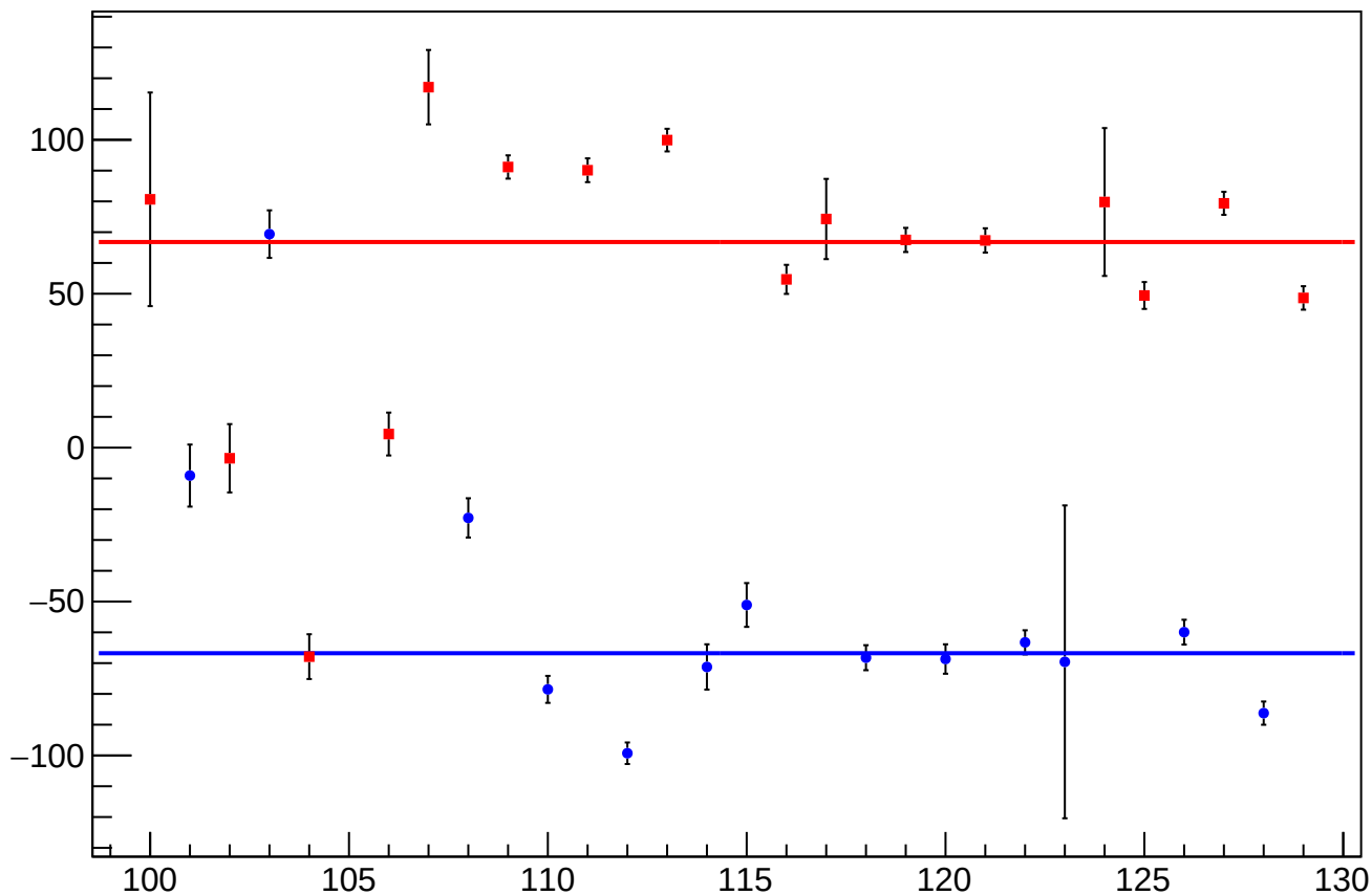
reg_asym_at1_avg_diff_bpm4aX_slope vs Slug, Sign Corrected
