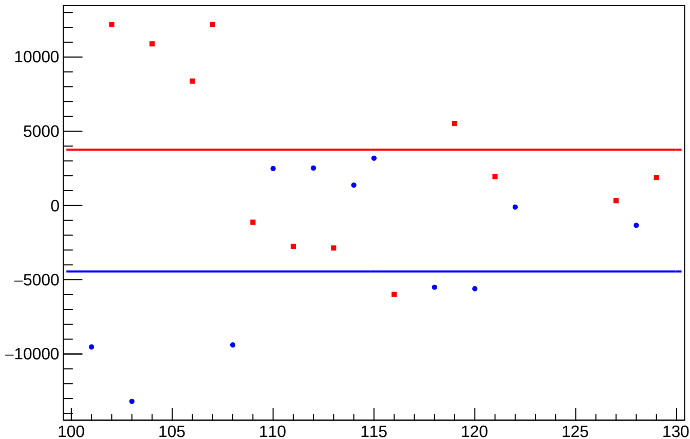
dit_atl2_coil6_mean vs Slug, Sign Corrected
