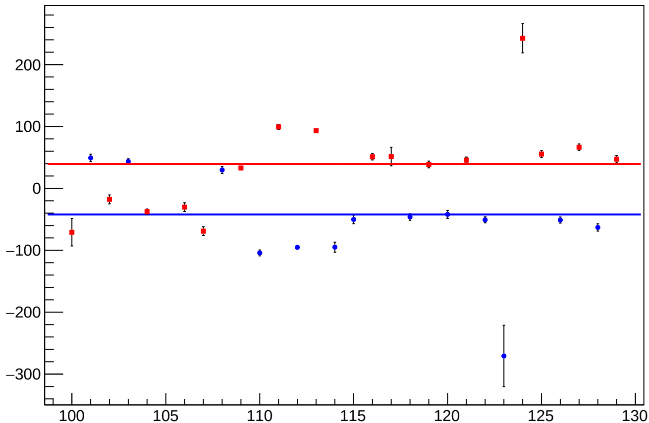
reg_asym_at2_dd_diff_bpm4aX_slope vs Slug, Sign Corrected
