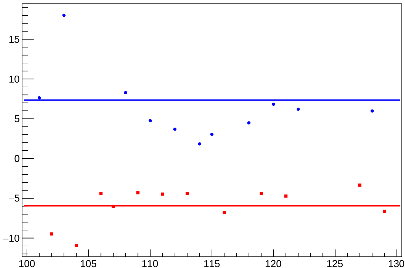
dit_11X12X_coil1_err_mean vs Slug, Sign Corrected
