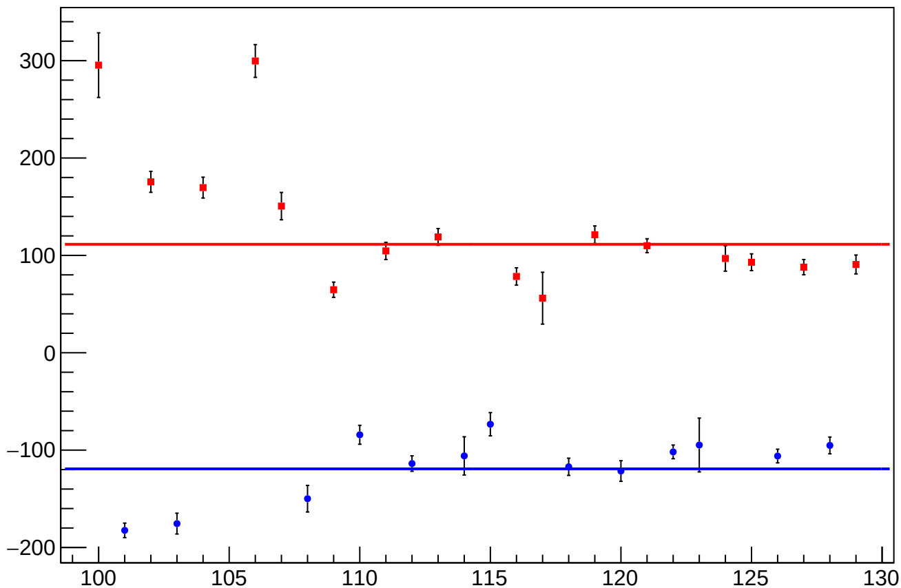
reg_asym_sam2_diff_bpm4aX_slope vs Slug, Sign Corrected
