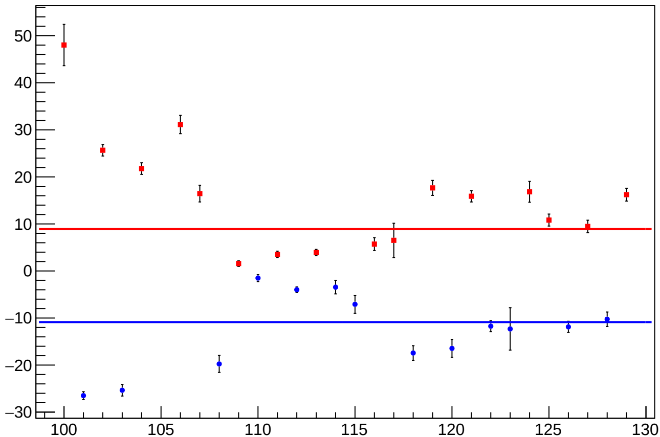
reg_asym_sam_1357_avg_diff_bpm4aX_slope vs Slug, Sign Corrected
