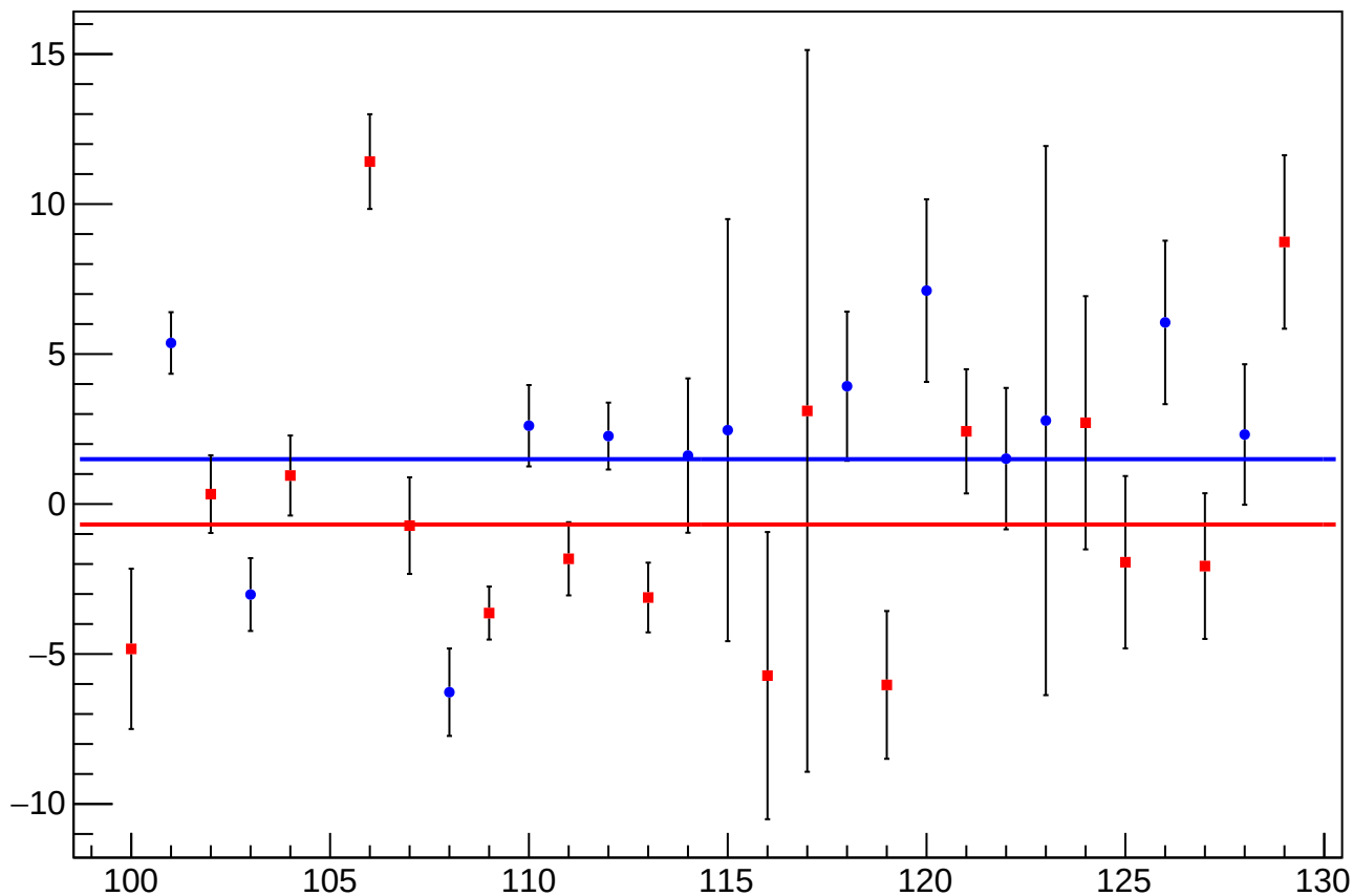
reg_asym_sam5_diff_bpm4aX_slope vs Slug, Sign Corrected
