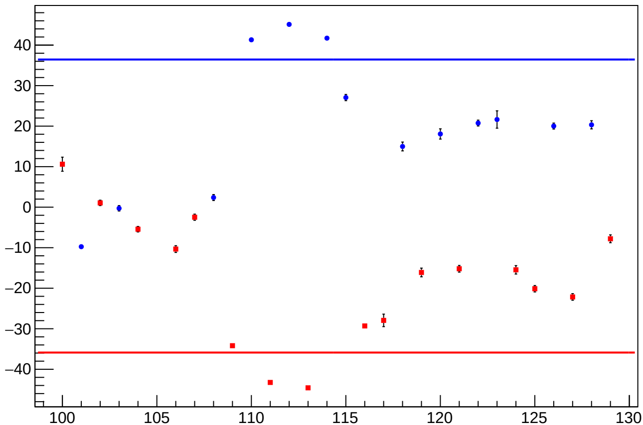
reg_asym_sam8_diff_bpm4aX_slope vs Slug, Sign Corrected
