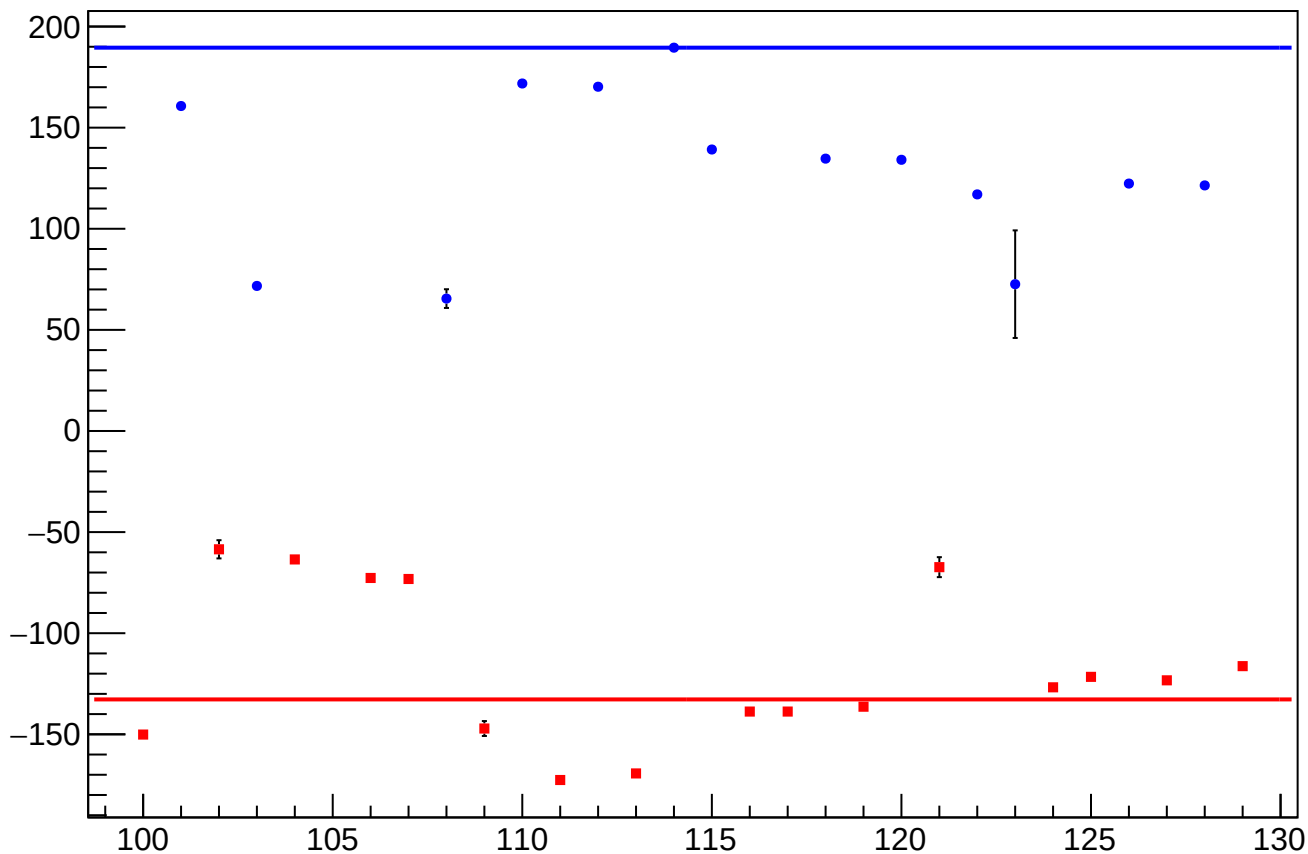
dit_atr2_4eY_slope vs Slug, Sign Corrected
