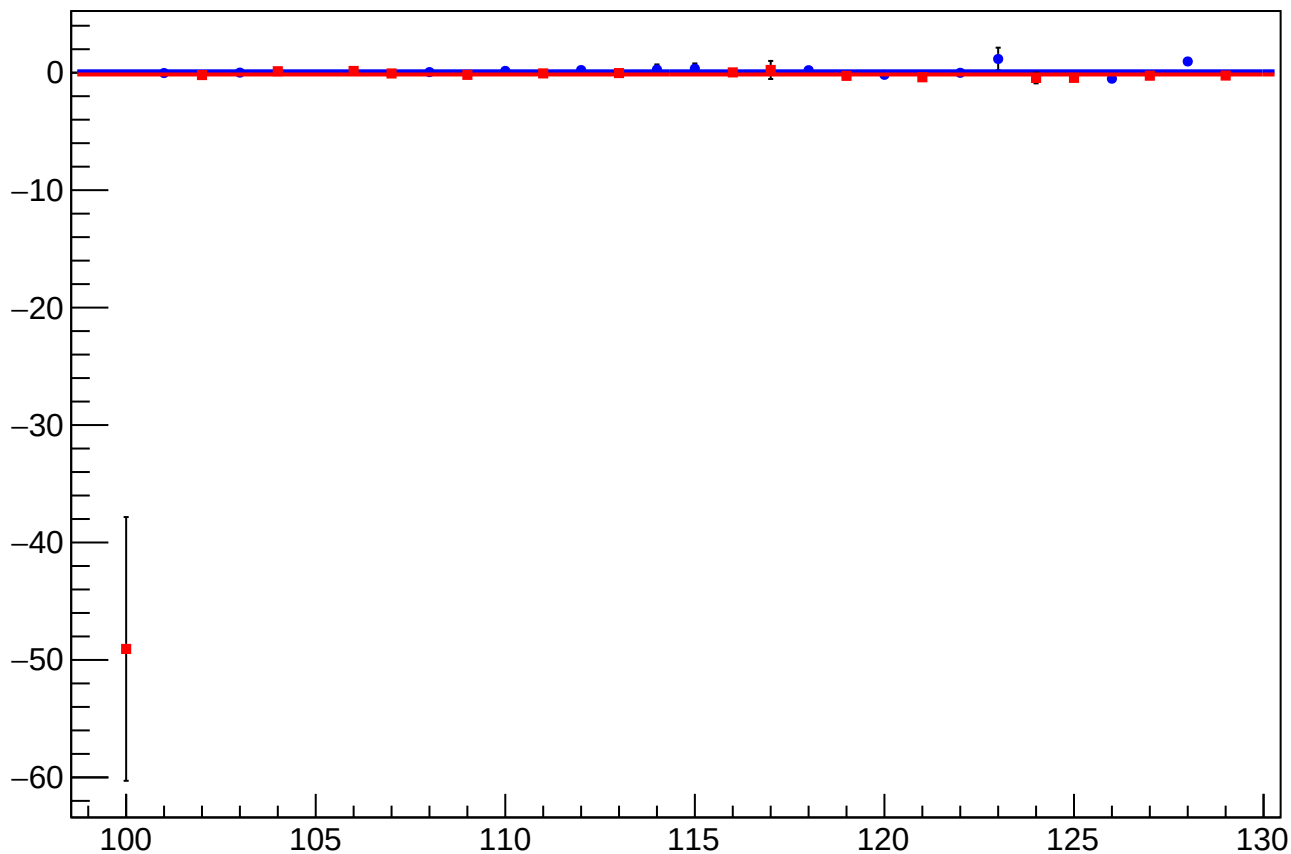
reg_asym_dsr_diff_bpm4aX_slope vs Slug, Sign Corrected
