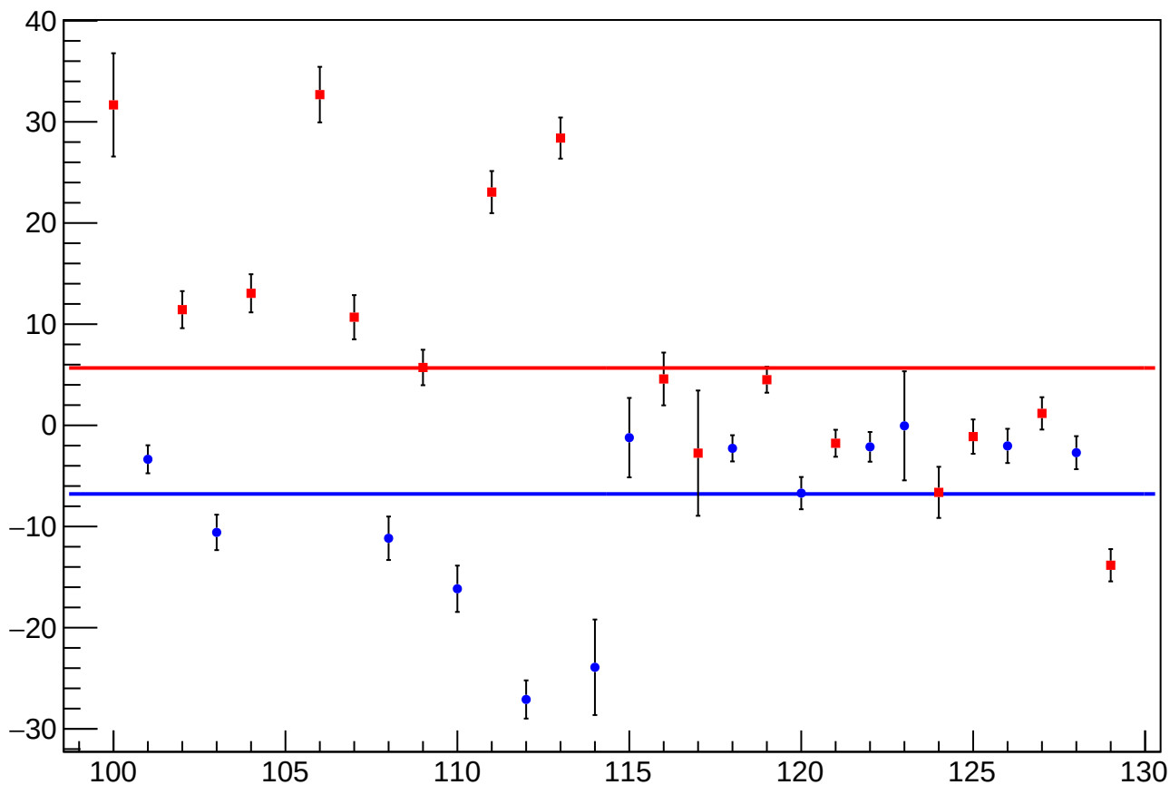
reg_asym_sam_26_48_dd_diff_bpm4aX_slope vs Slug, Sign Corrected
