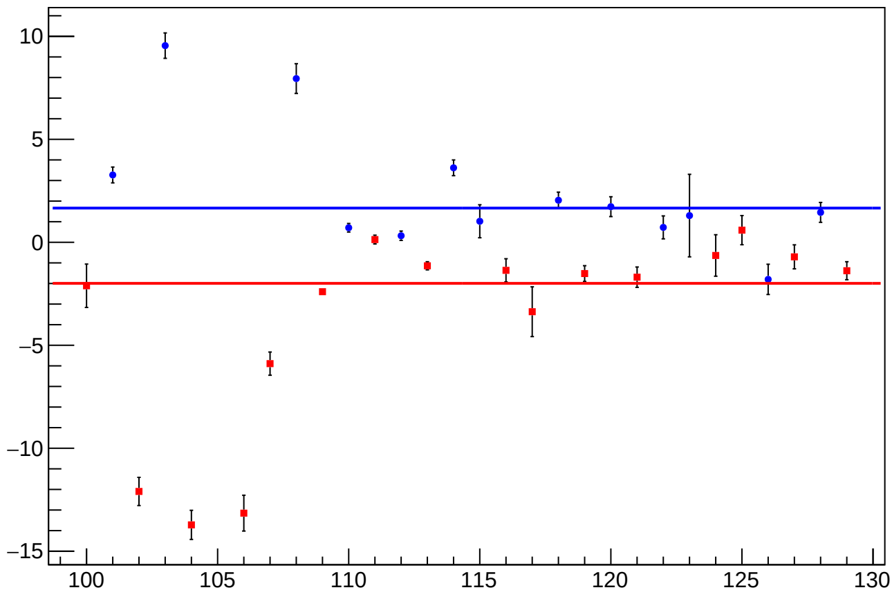
reg_asym_bcm_an_ds_diff_bpm4aX_slope vs Slug, Sign Corrected
