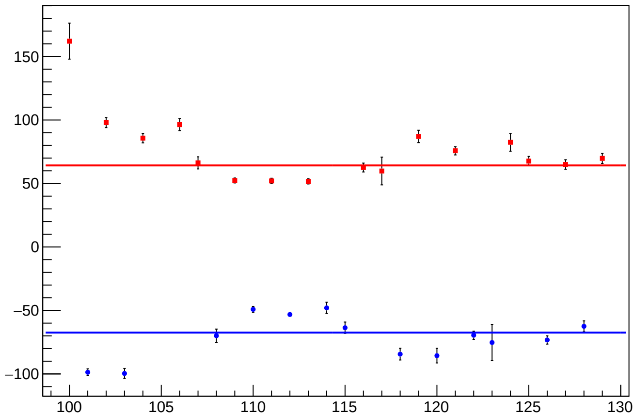
reg_asym_sam3_diff_bpm4aX_slope vs Slug, Sign Corrected
