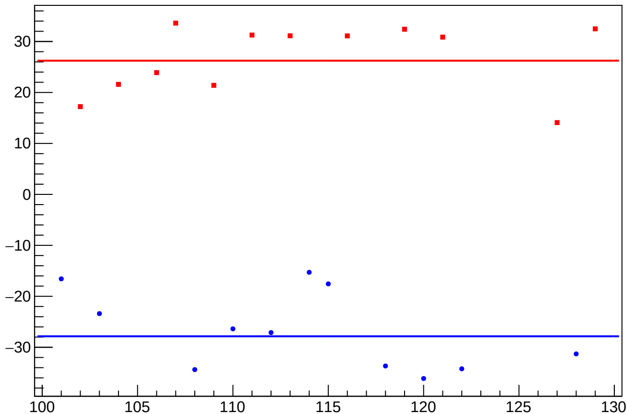
dit_4aX_coil3_mean vs Slug, Sign Corrected
