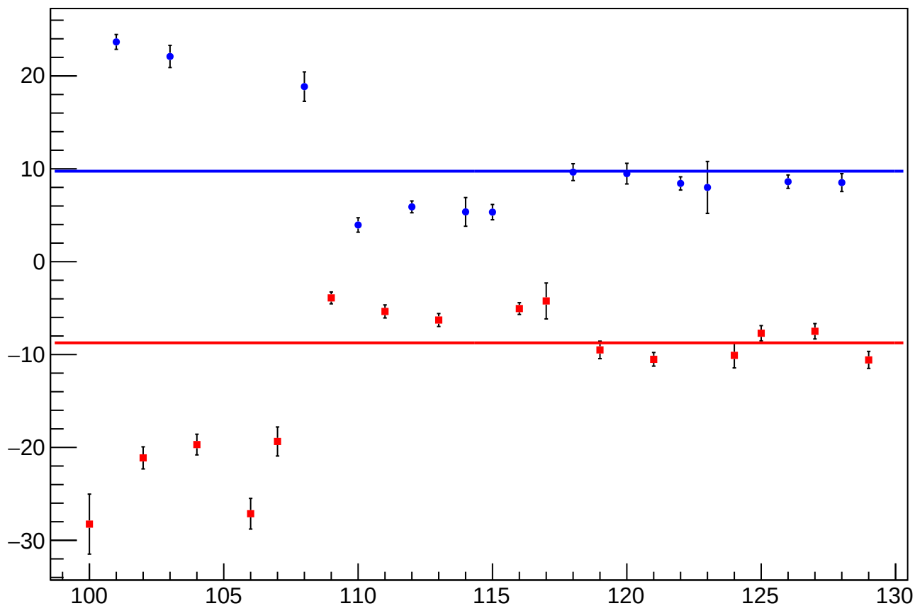
reg_asym_sam_1357_2468_dd_diff_bpm4aX_slope vs Slug, Sign Corrected
