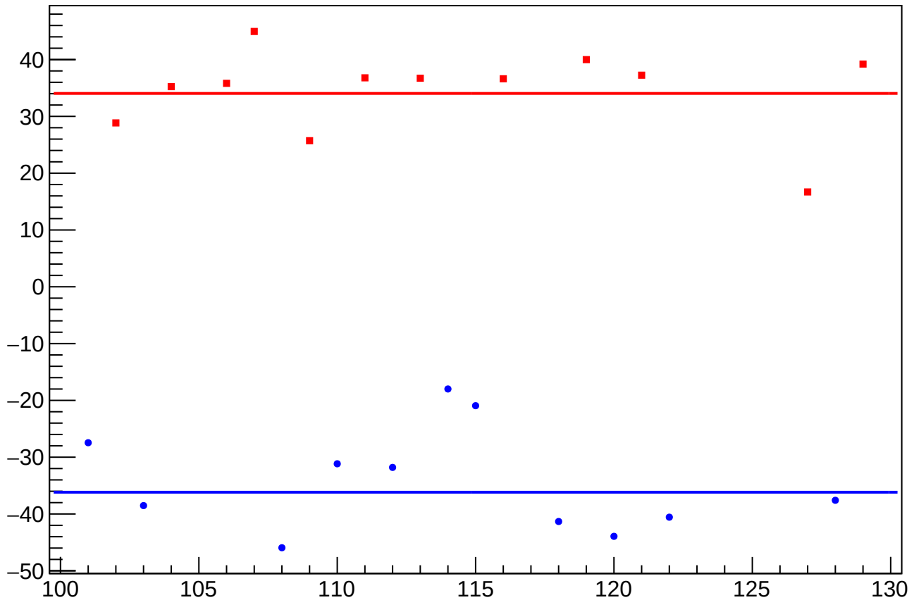
dit_4eX_coil3_mean vs Slug, Sign Corrected
