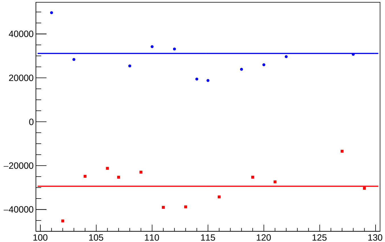
dit_atr2_coil4_mean vs Slug, Sign Corrected
