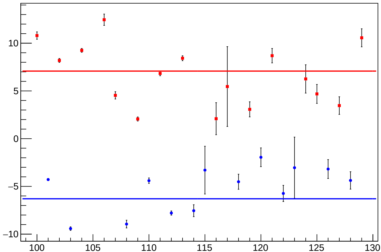
reg_asym_sam_15_avg_diff_bpm4aX_slope vs Slug, Sign Corrected
