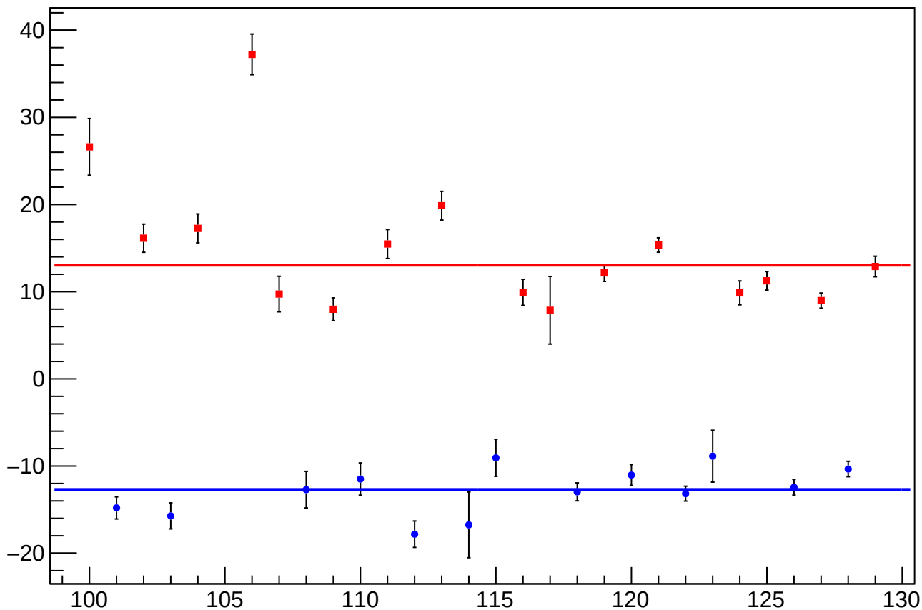
reg_asym_sam1_diff_bpm4aX_slope vs Slug, Sign Corrected
