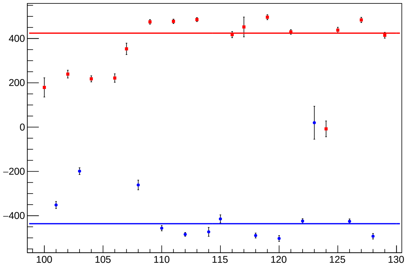
reg_asym_atl2_diff_bpm4aX_slope vs Slug, Sign Corrected
