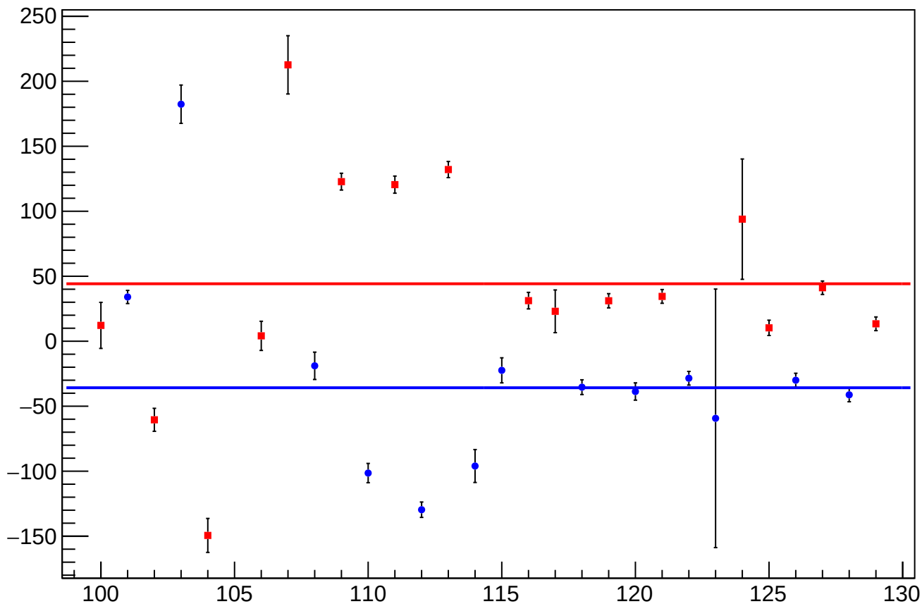
reg_asym_atl1_diff_bpm4aX_slope vs Slug, Sign Corrected
