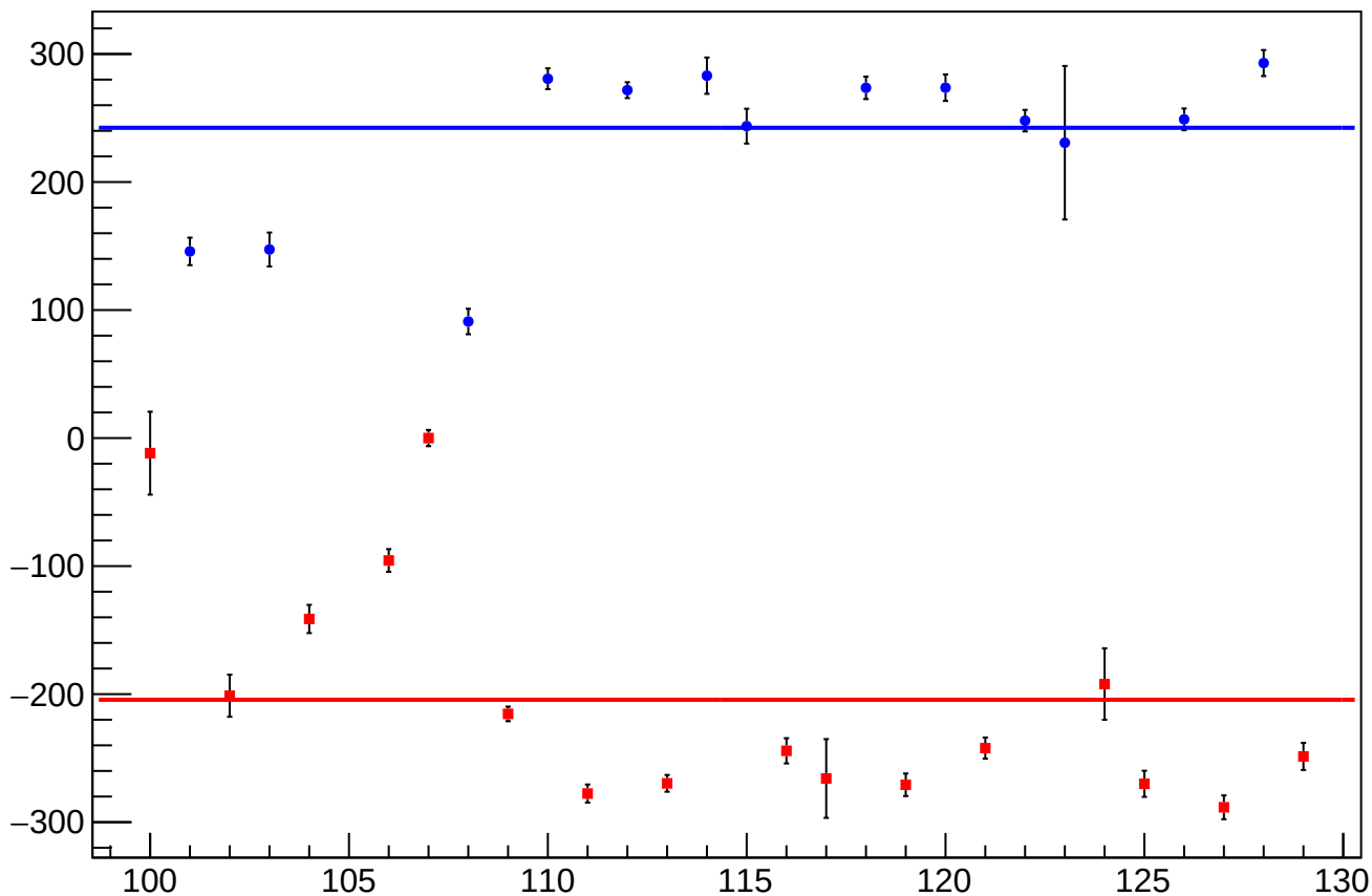
reg_asym_atl1r2_dd_diff_bpm4aX_slope vs Slug, Sign Corrected
