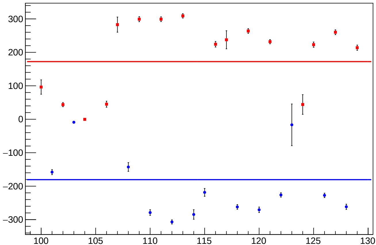
reg_asym_atl_avg_diff_bpm4aX_slope vs Slug, Sign Corrected
