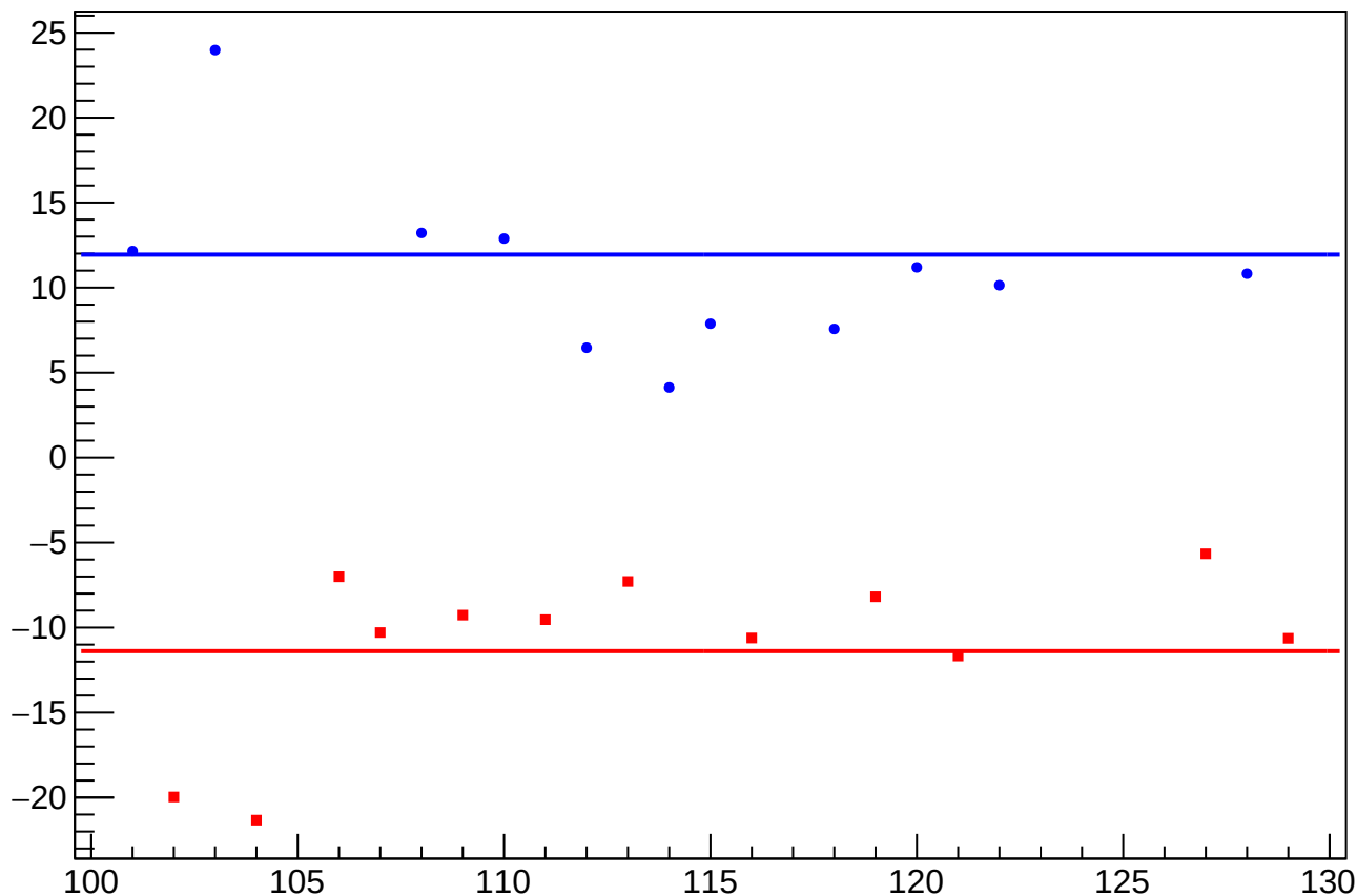
dit_11X12X_coil7_err_mean vs Slug, Sign Corrected
