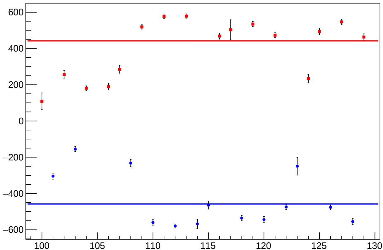
reg_asym_at2_avg_diff_bpm4aX_slope vs Slug, Sign Corrected
