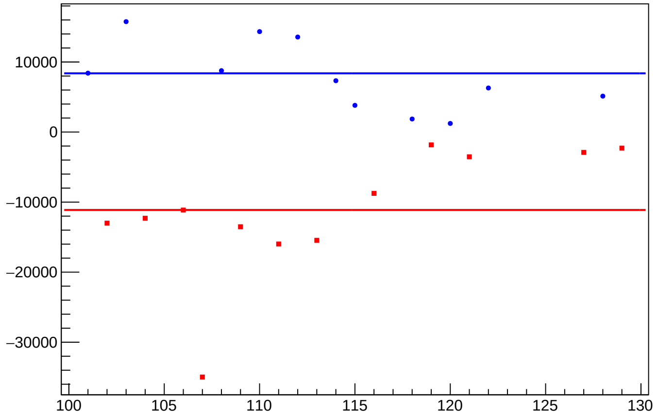
dit_usl_coil7_mean vs Slug, Sign Corrected
