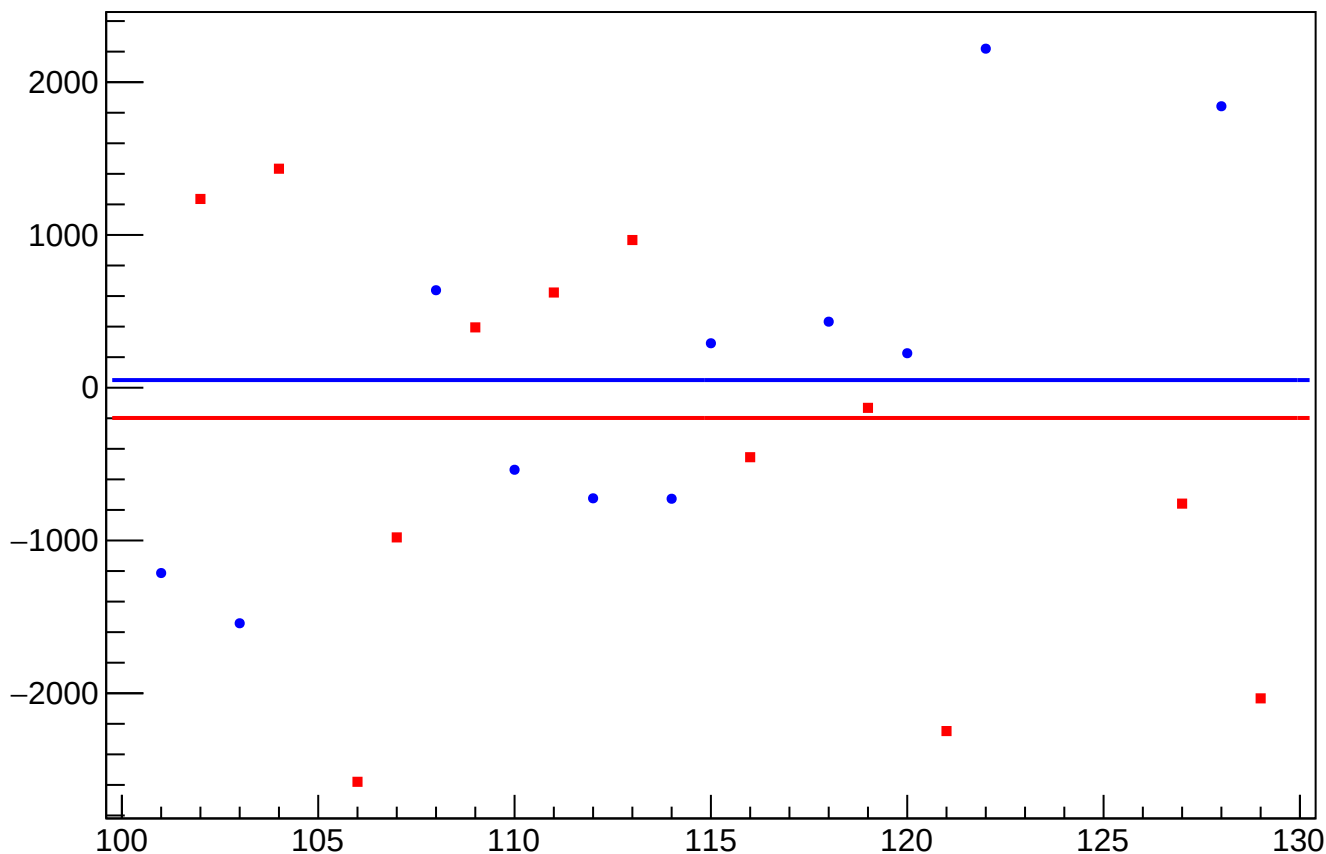
dit_sam5_coil1_mean vs Slug, Sign Corrected
