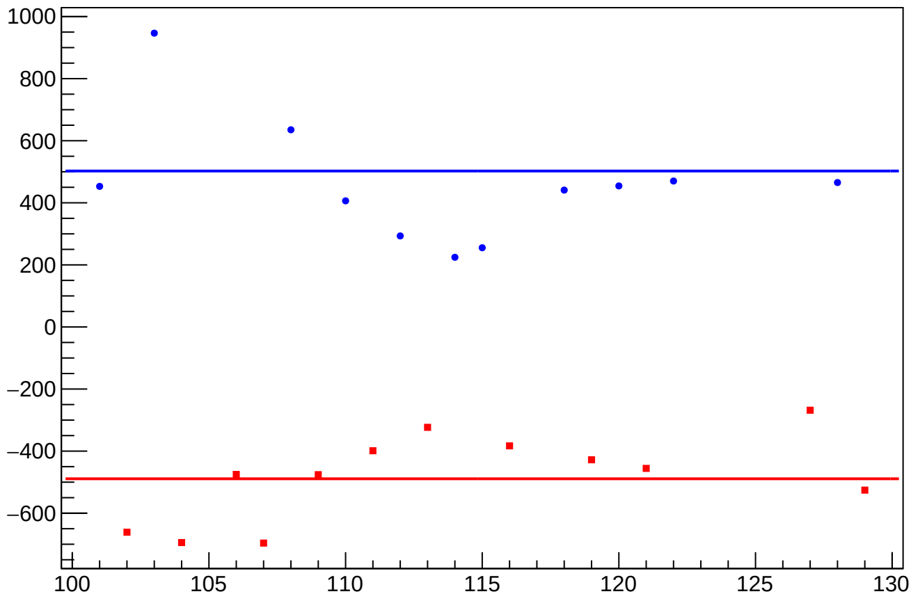
dit_usr_coil4_err_mean vs Slug, Sign Corrected
