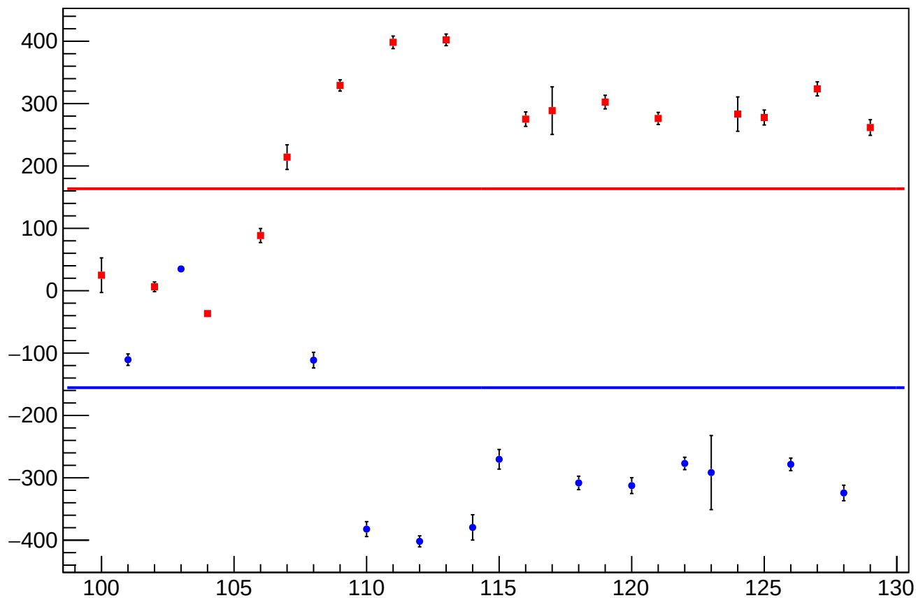
reg_asym_atl1r2_avg_diff_bpm4aX_slope vs Slug, Sign Corrected
