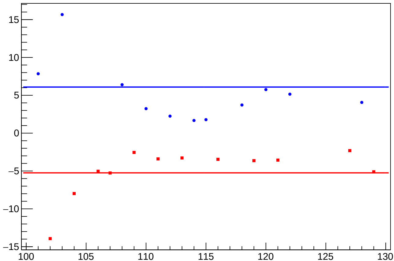
dit_4aX_coil1_err_mean vs Slug, Sign Corrected
