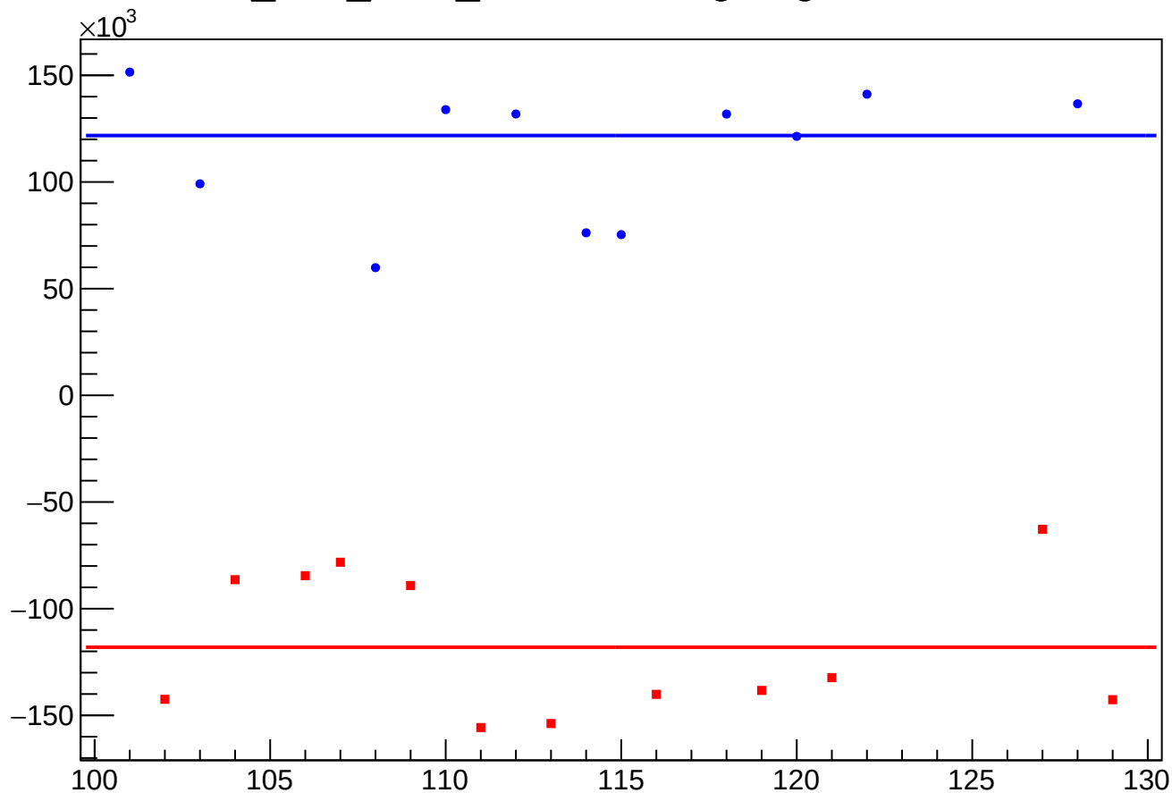
dit_atr2_coil7_mean vs Slug, Sign Corrected
