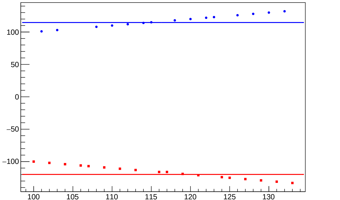
dit_slug_slope vs Slug, Sign Corrected
