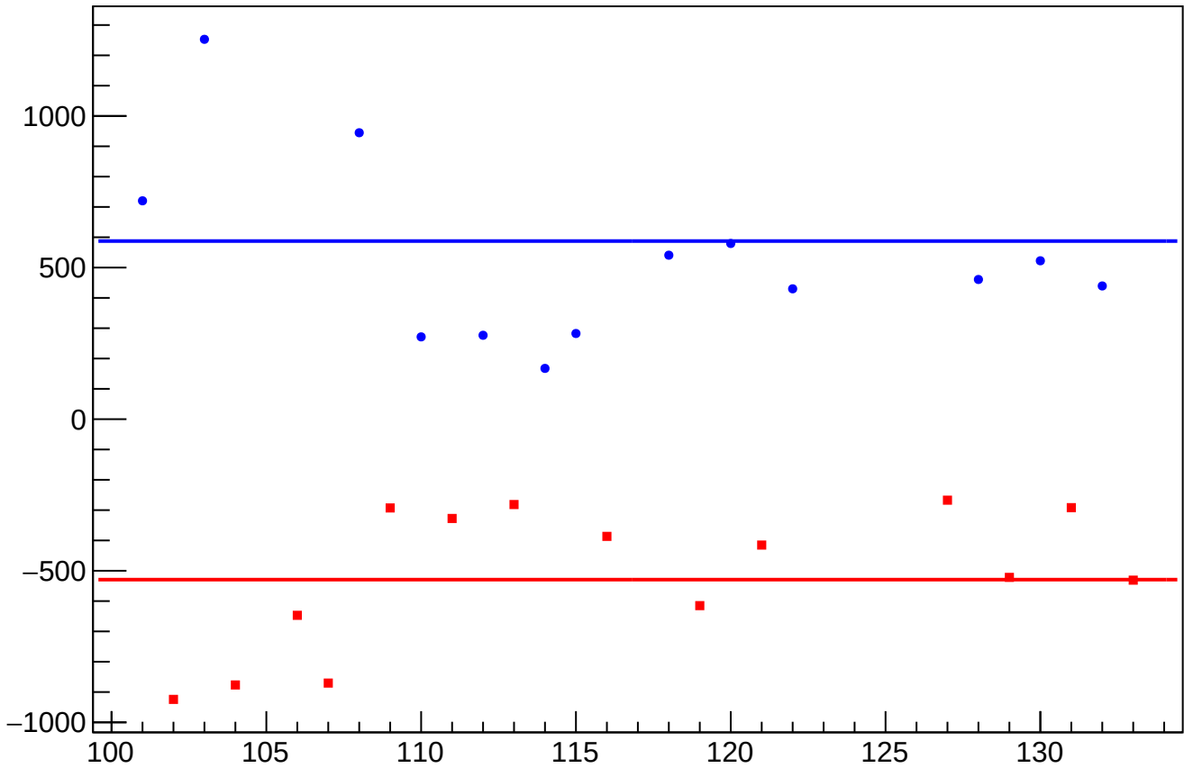
dit sam3 coil4 err mean vs Slug, Sign Corrected
