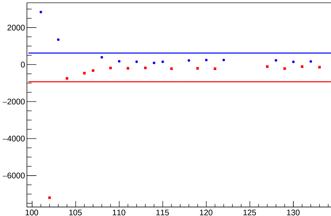
dit atr1 coil6 err_mean vs Slug, Sign Corrected
