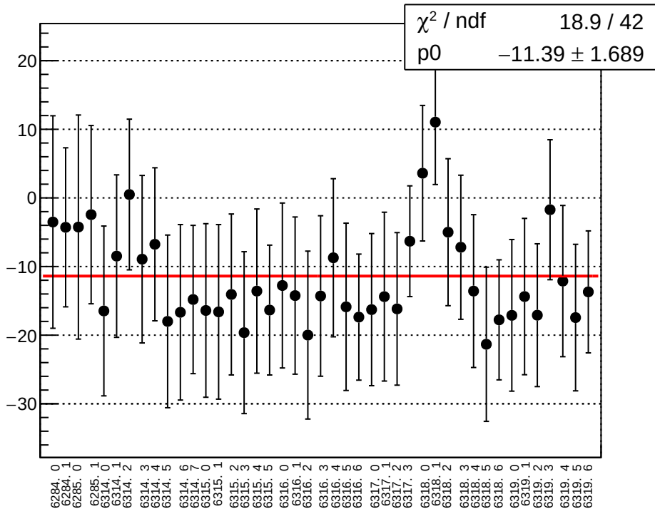
reg asym sam5 diff bpm4eX slope vs run
