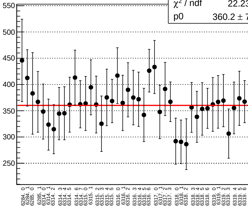
reg_asym_atl_dd_diff_bpm4aX_slope vs run
