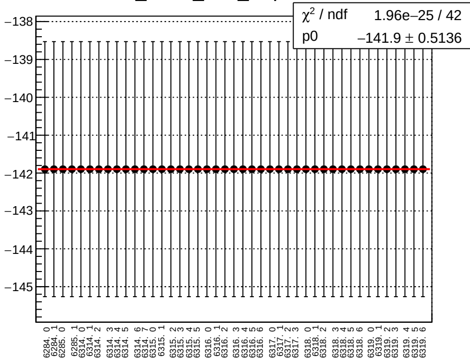
dit_sam7_4eX_slope vs run
