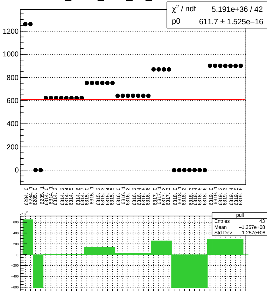
dit_sam3_coil7_err_mean vs run
