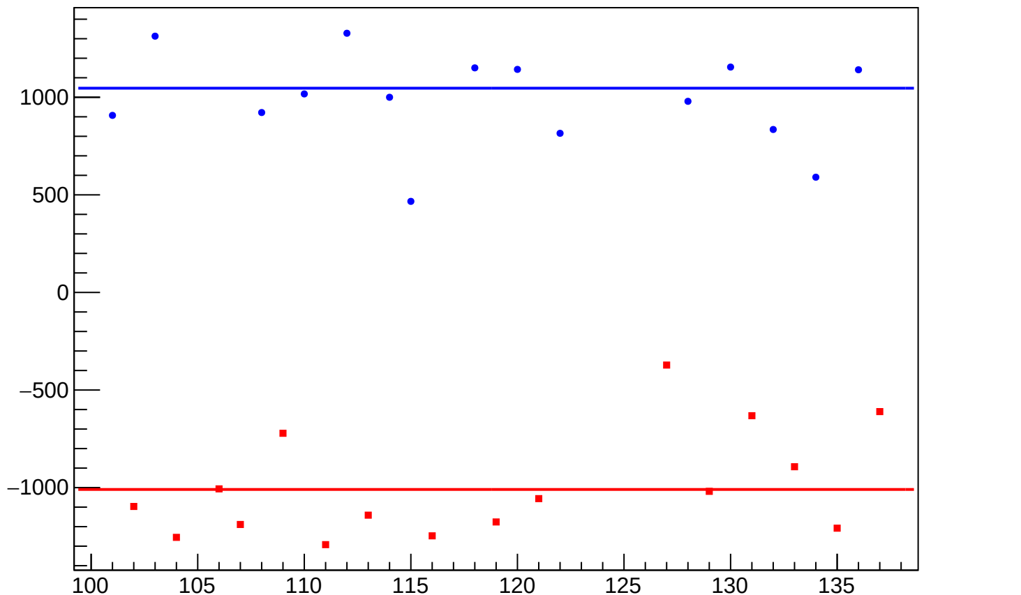
dit_11X12X_coil1_Ndata_mean vs Slug, Sign Corrected
