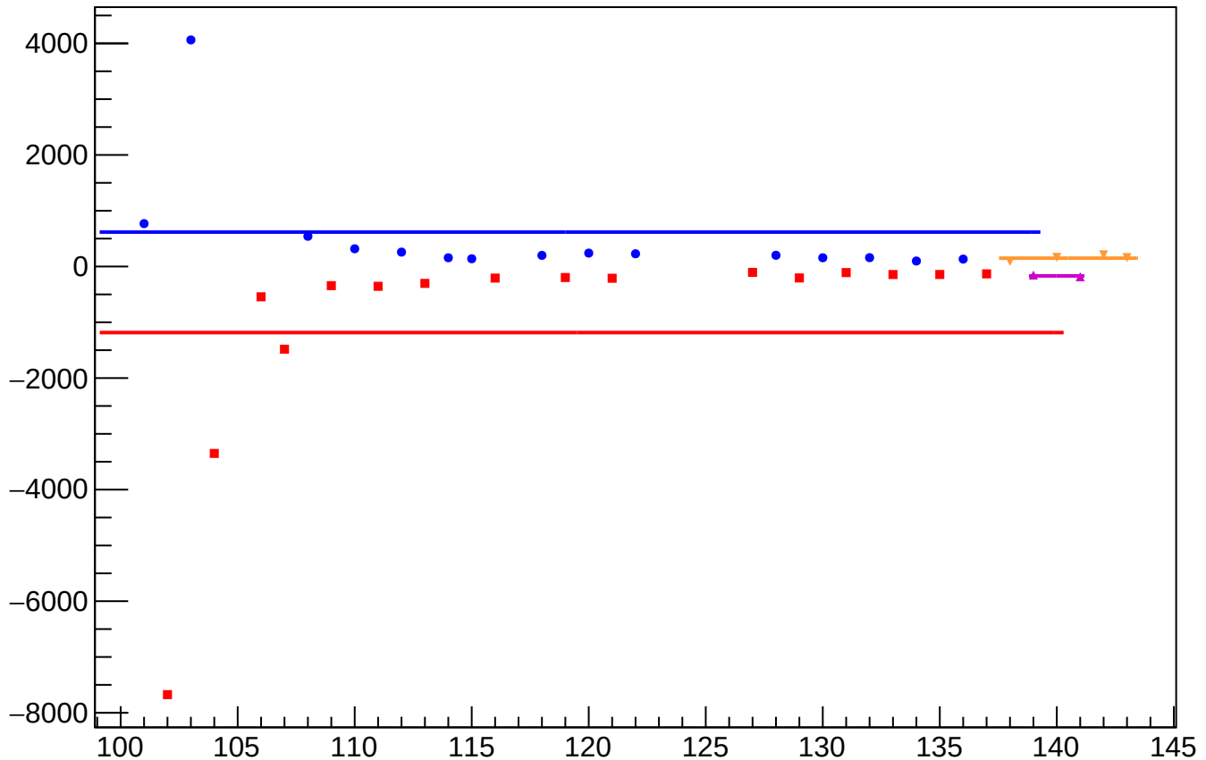
dit_atl1_coil6_err_mean vs Slug, Sign Corrected
