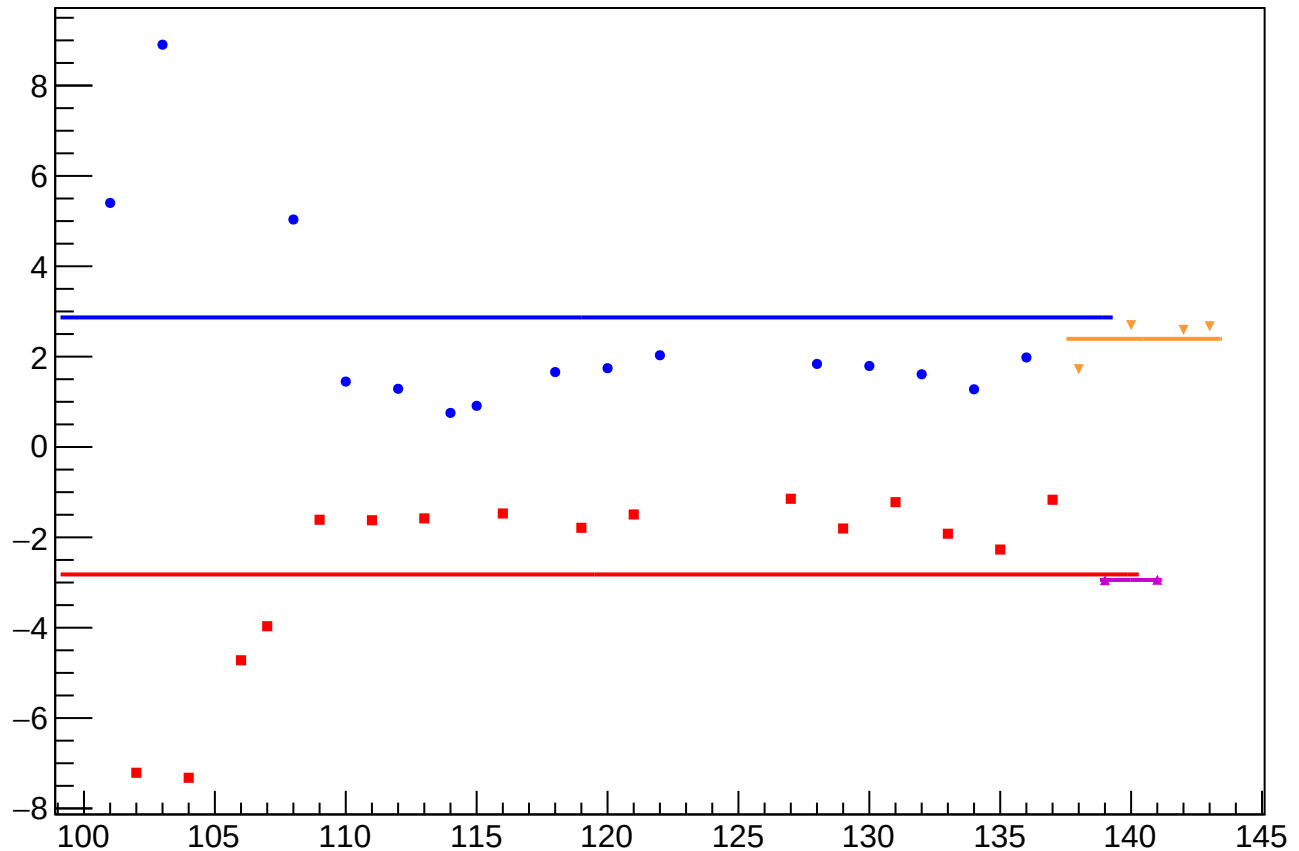
dit_4aX_coil3_err_mean vs Slug, Sign Corrected
