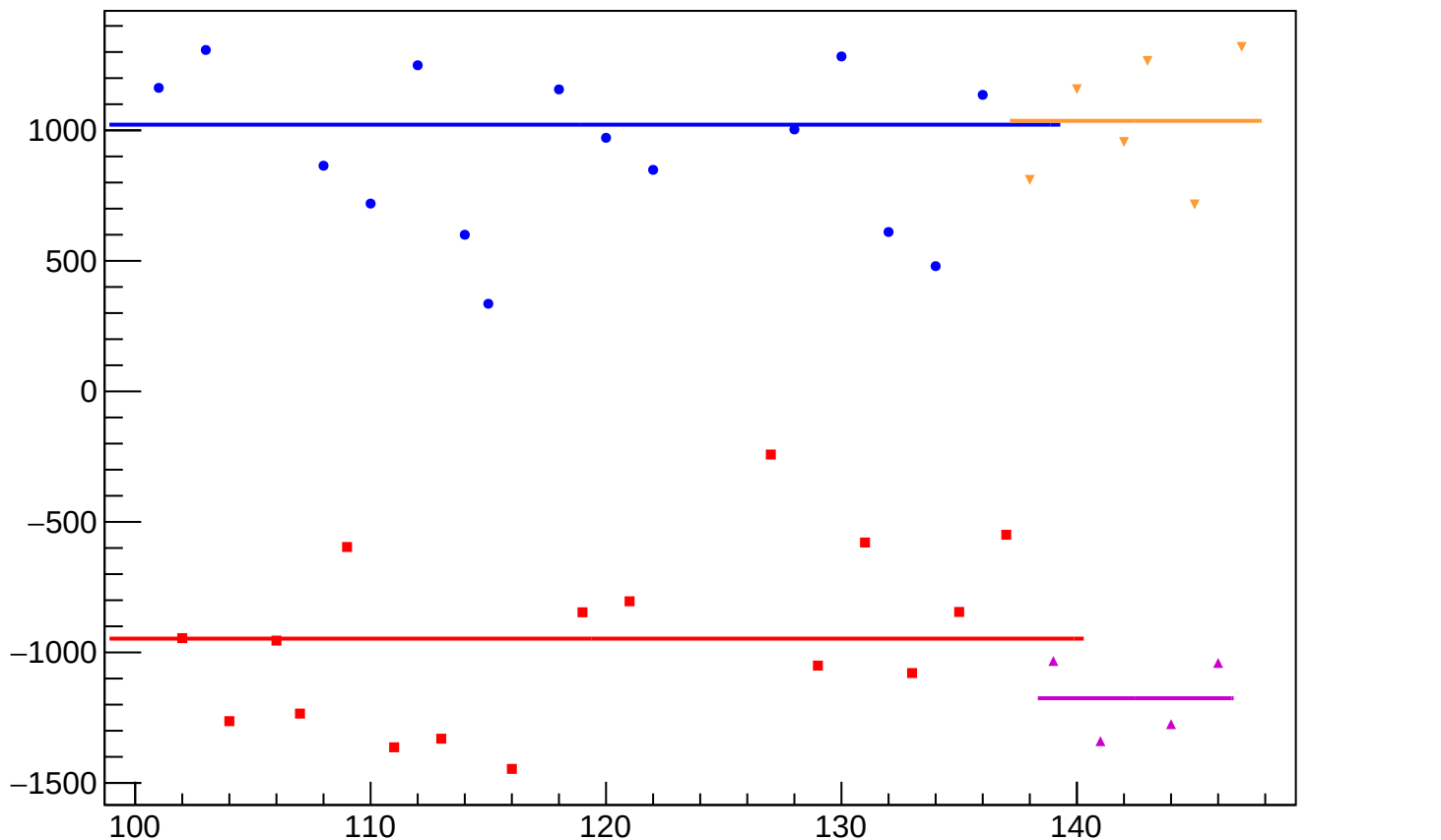
dit_sam7_coil7_Ndata_mean vs Slug, Sign Corrected
