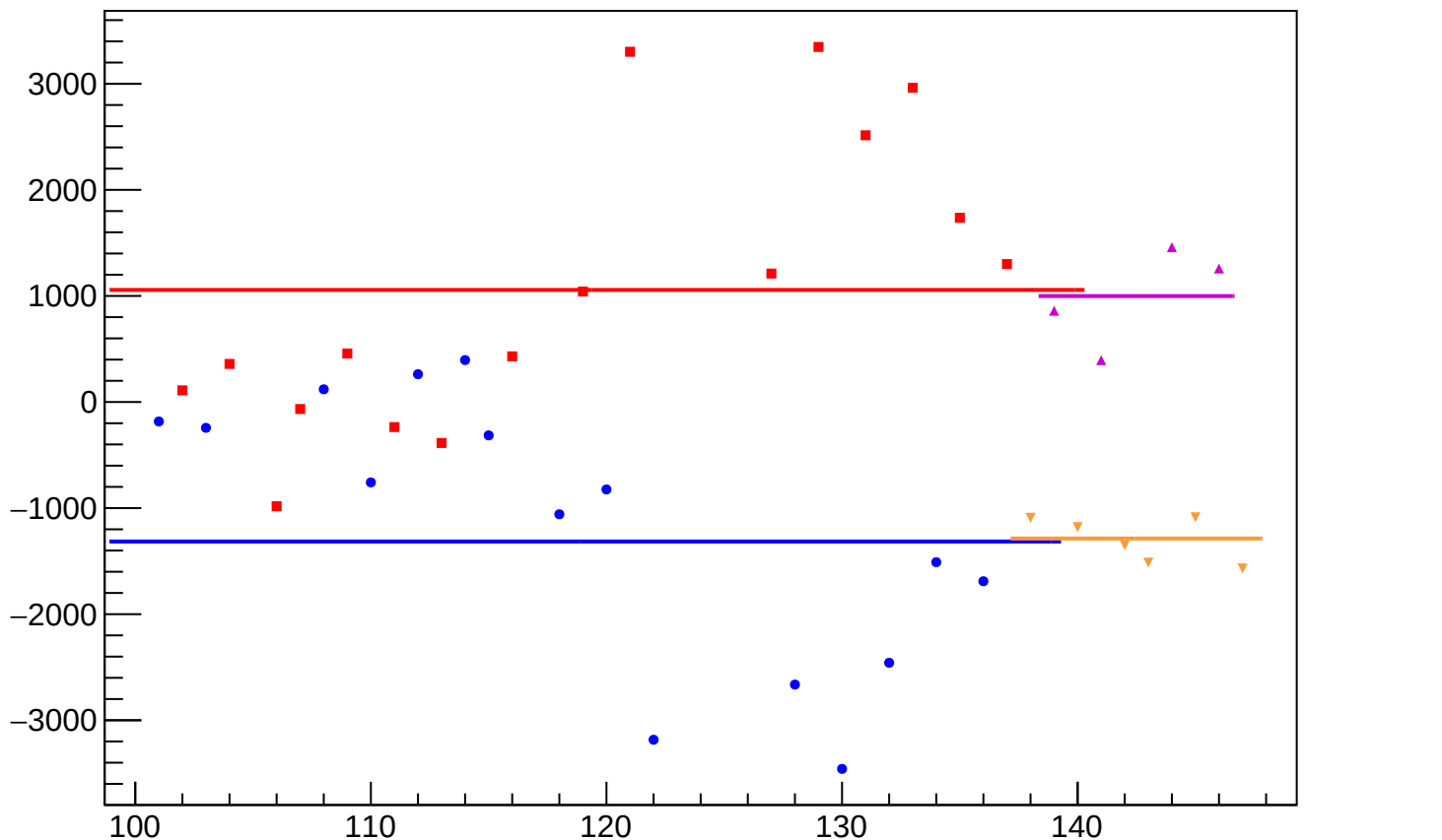
dit_sam5_coil7_mean vs Slug, Sign Corrected
