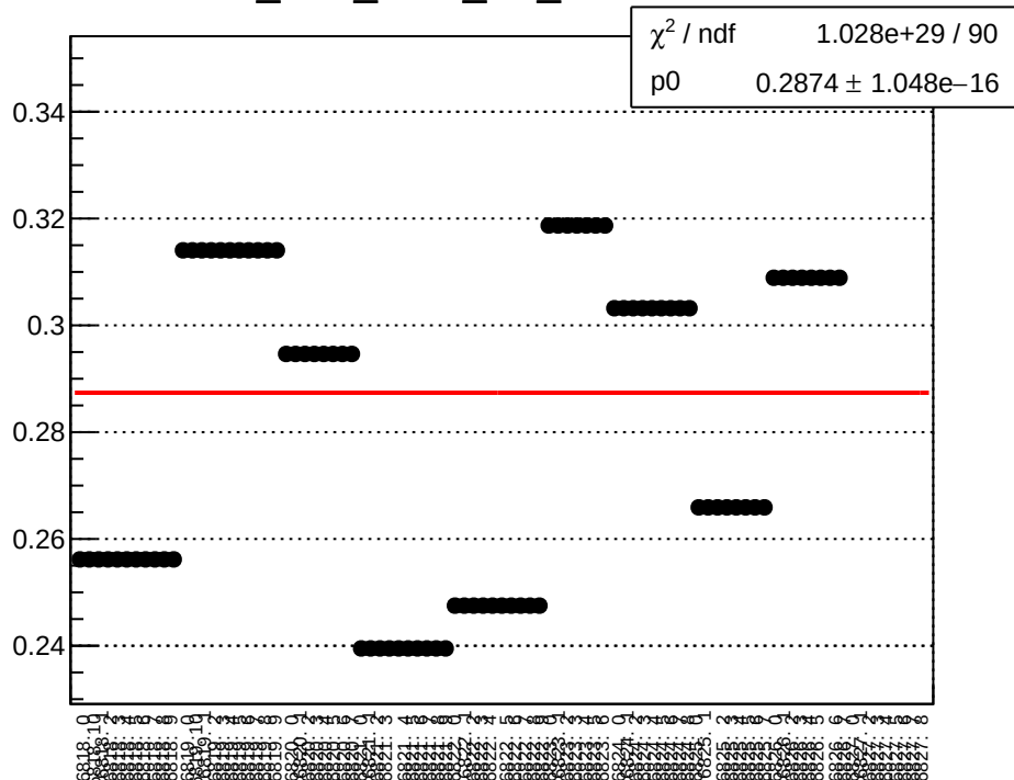
dit_4eY_coil6_err_mean vs run
