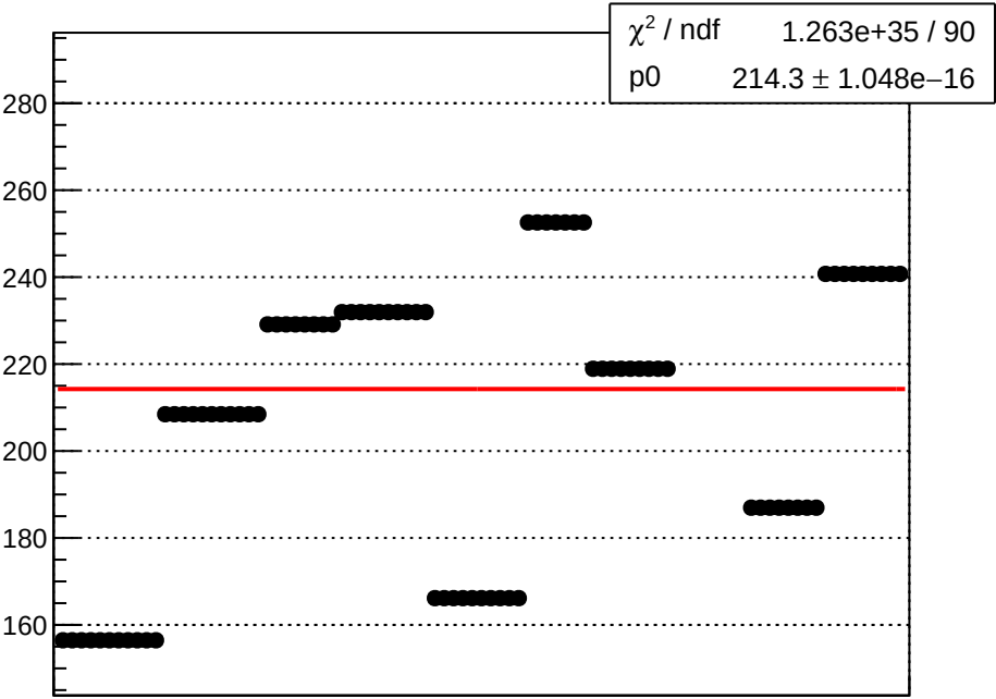
dit_sam5_coil7_err_mean vs run
