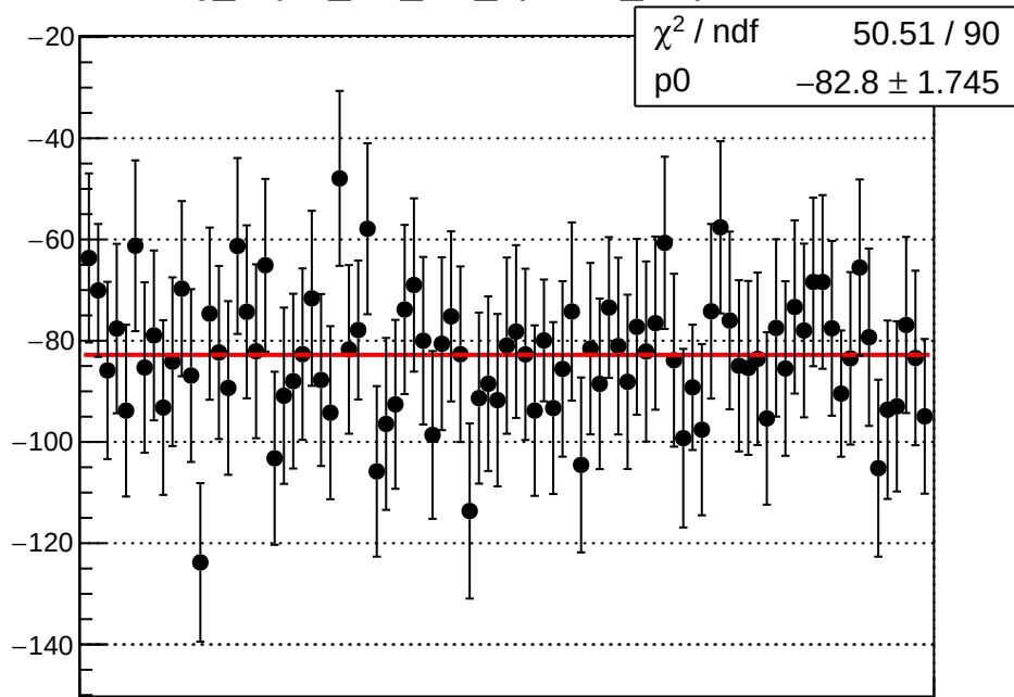
reg_asym_usl_diff_bpm1X_slope vs run
