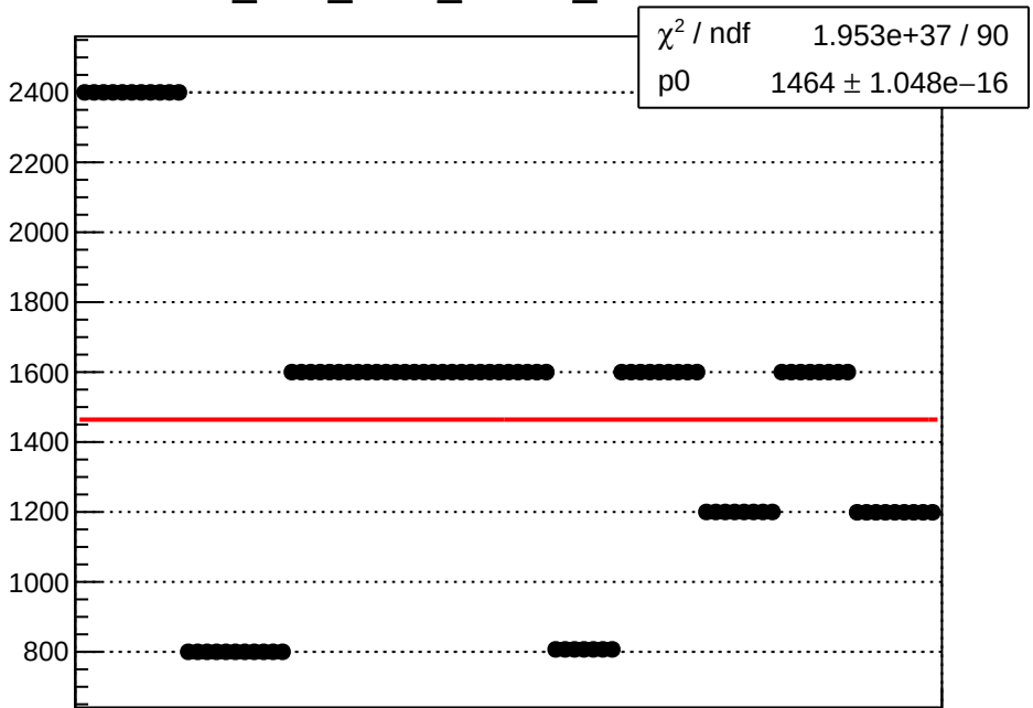
dit_atr1_coil7_Ndata_mean vs run
