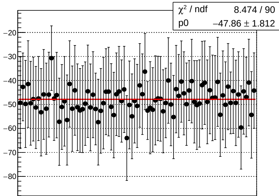
reg_asym_sam_26_dd_diff_bpm1X_slope vs run
