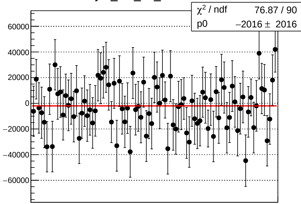
asym_at1_dd_mean vs run
