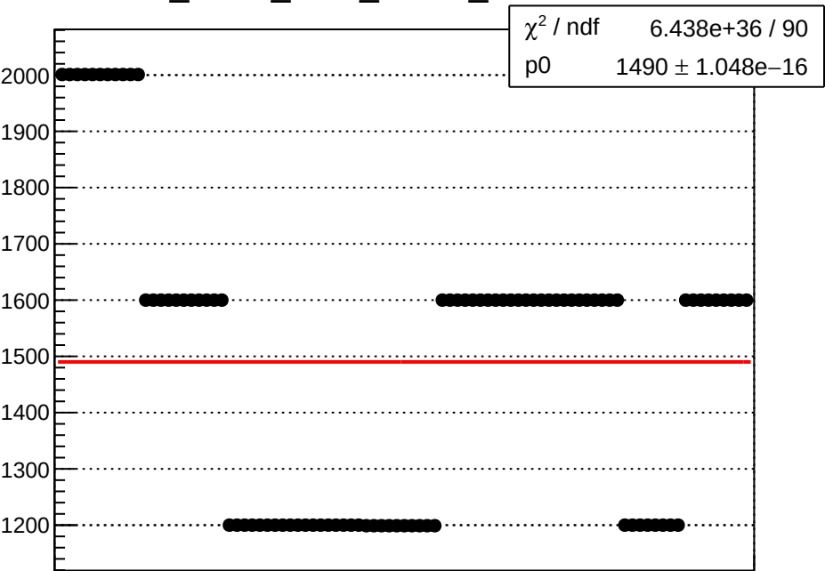
dit_sam4_coil1_Ndata_mean vs run
