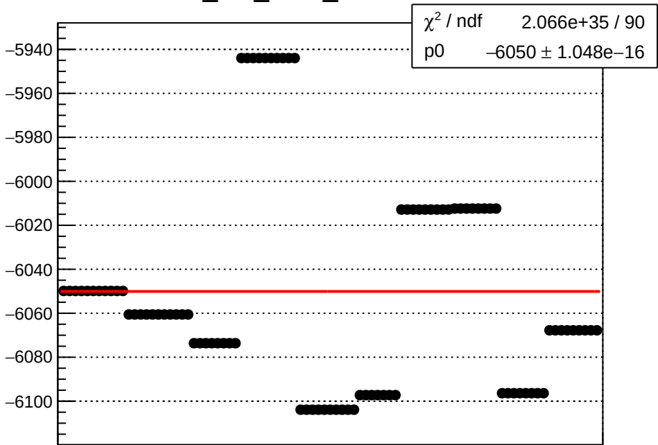
dit_usr_coil3_mean vs run
