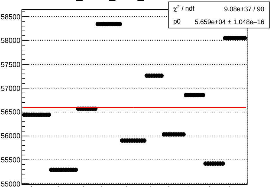
dit_sam3_coil1_mean vs run
