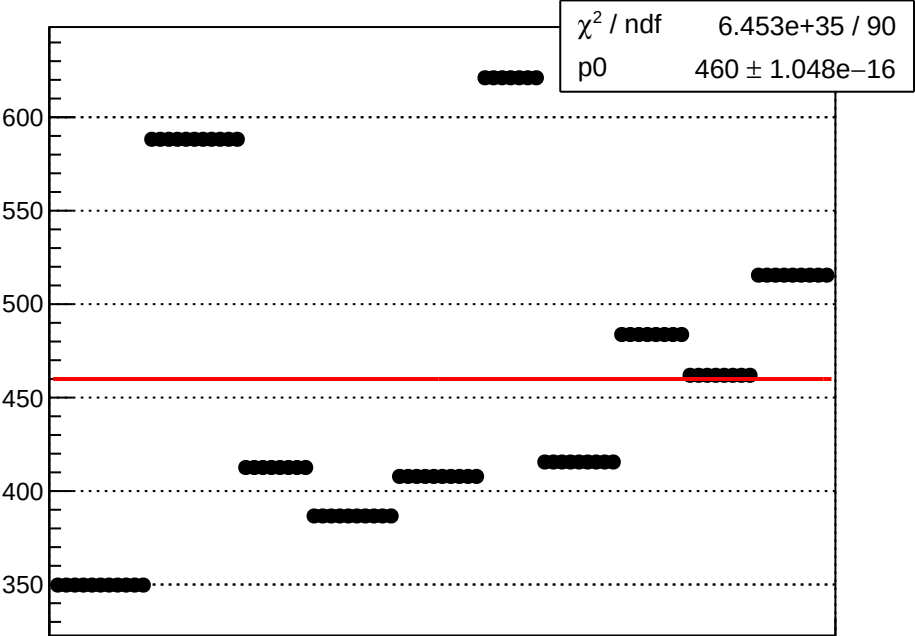
dit_atl1_coil7_err_mean vs run
