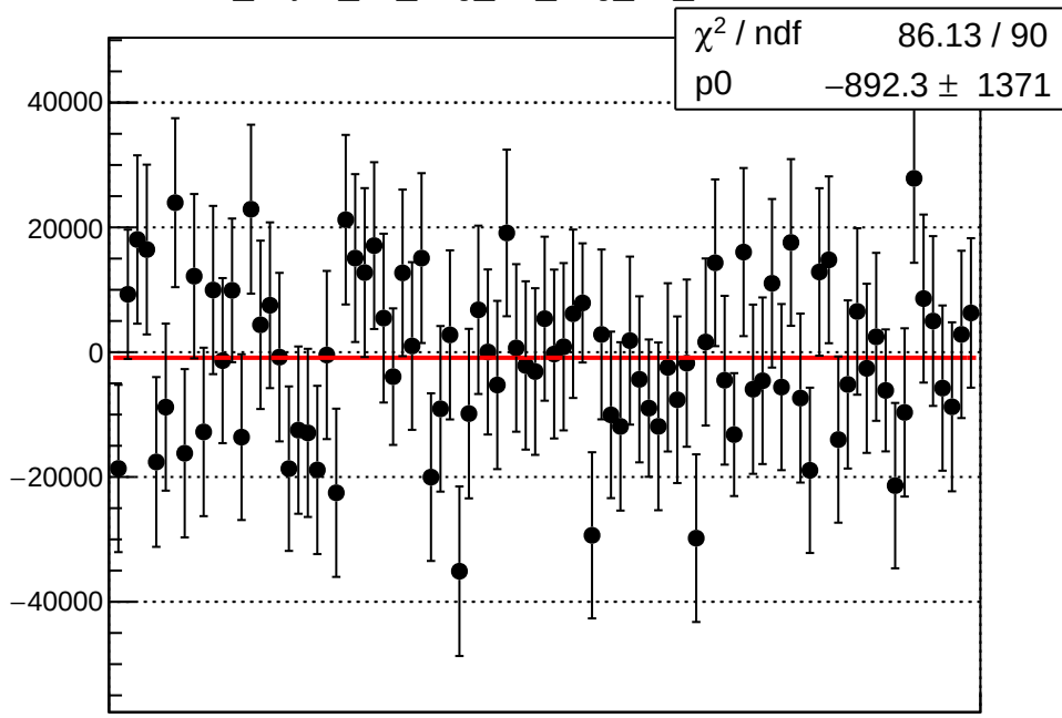
dit_asym_atl_avg_atr_avg_dd_mean vs run
