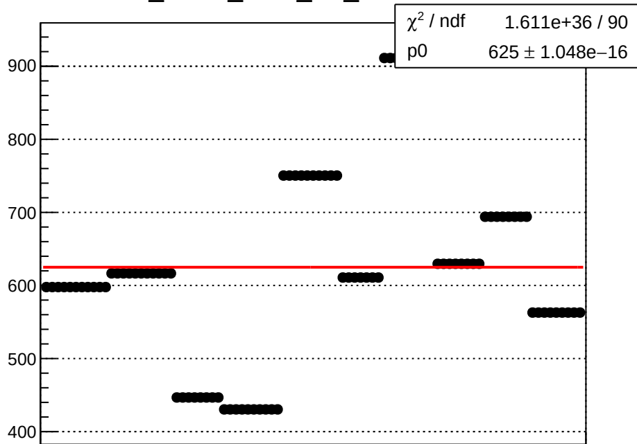
dit_sam4_coil4_err_mean vs run
