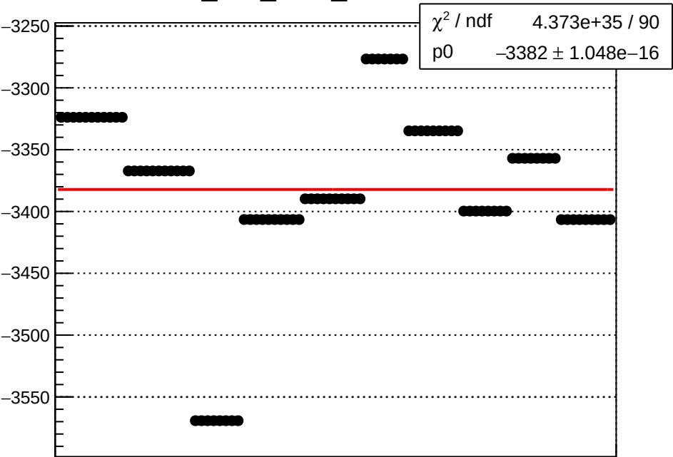
dit_atl1_coil3_mean vs run
