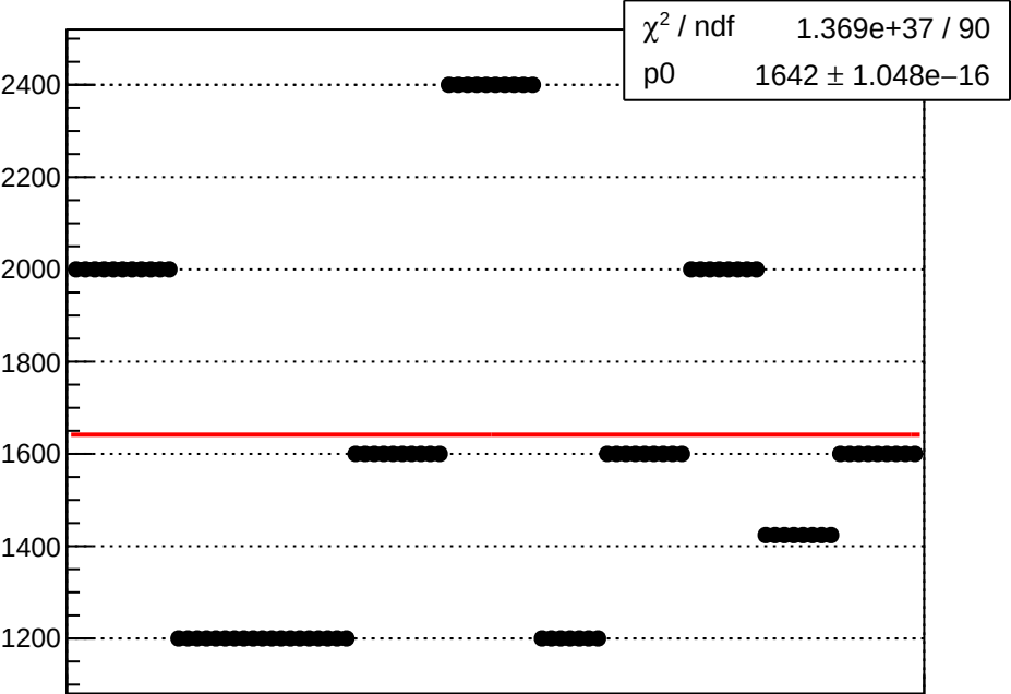
dit_sam6_coil3_Ndata_mean vs run
