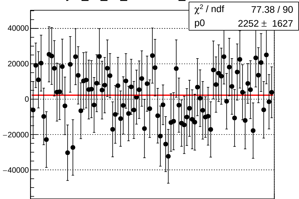
asym_us_dd_correction_mean vs run
