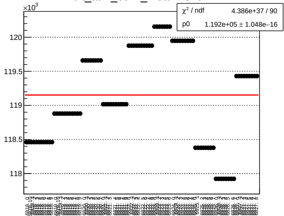
dit_atr2_coil7_mean vs run
