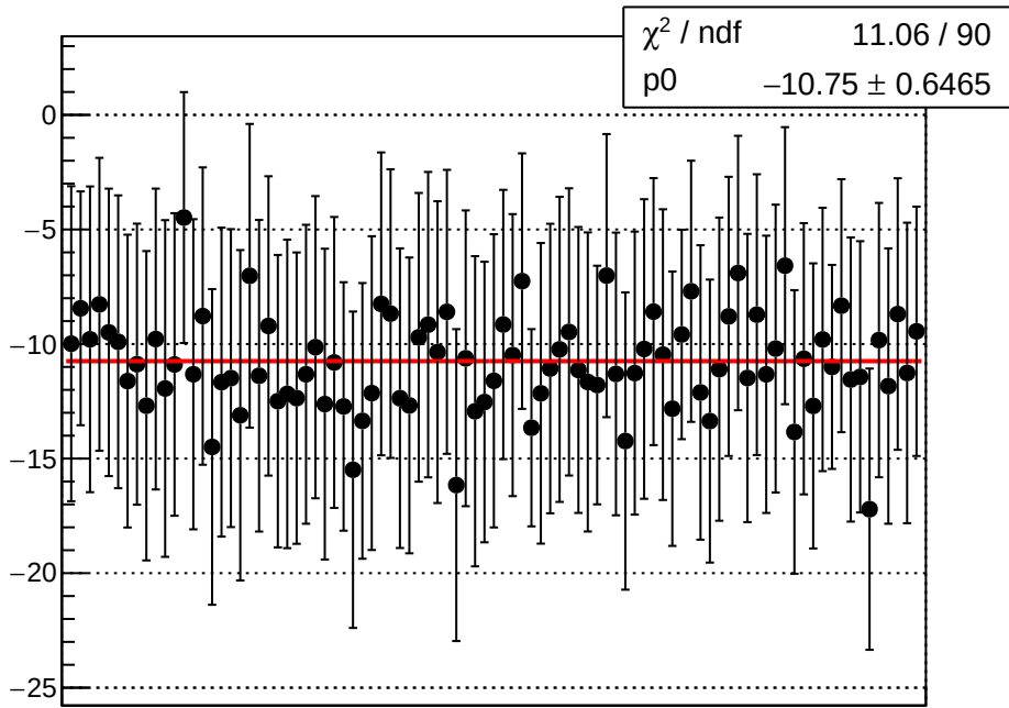
reg_asym_sam_15_dd_diff_bpm1X_slope vs run
