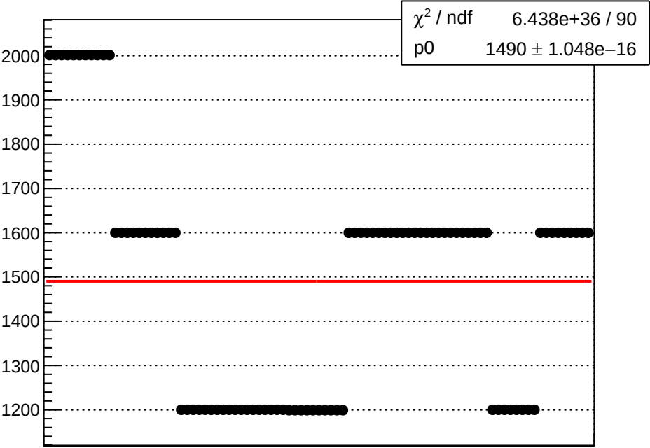
dit_sam7_coil1_Ndata_mean vs run
