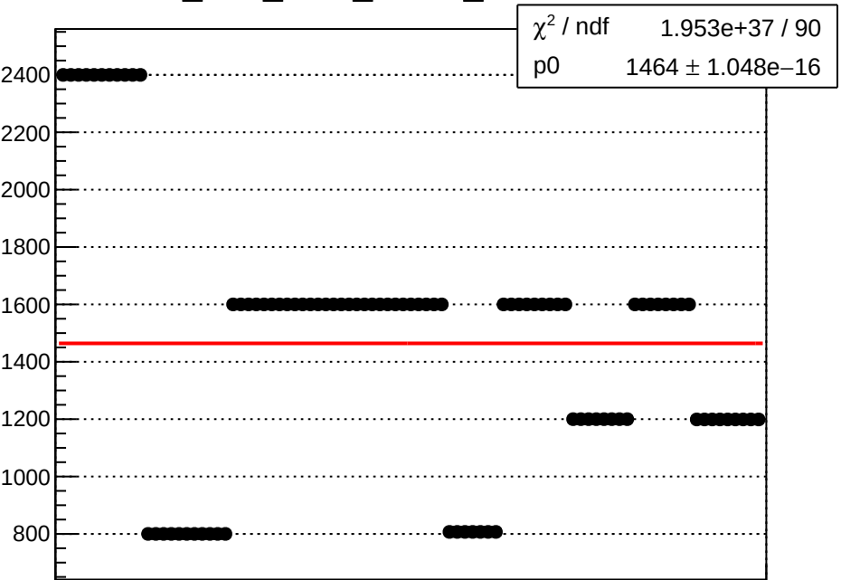
dit_4eX_coil7_Ndata_mean vs run
