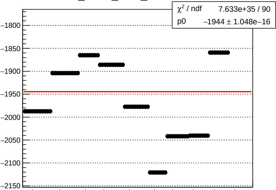
dit_sam6_coil6_mean vs run
