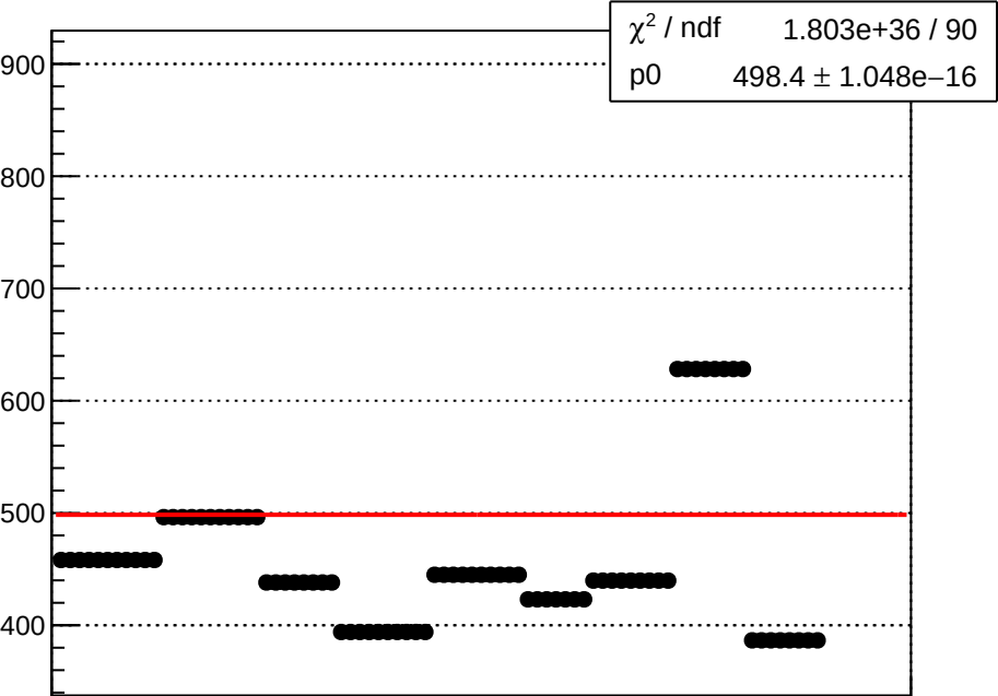
dit_atl2_coil6_err_mean vs run
