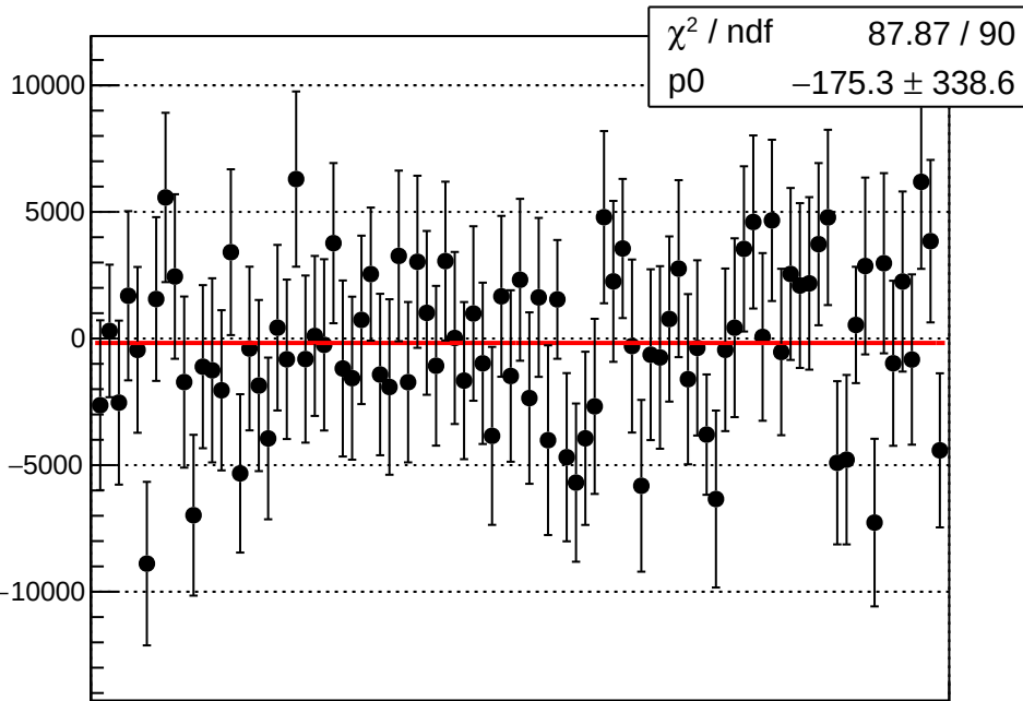
asym atl avg atr avg dd correction_mean vs run
