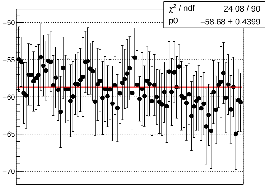
reg_asym_sam_15_dd_diff_bpm4aY_slope vs run
