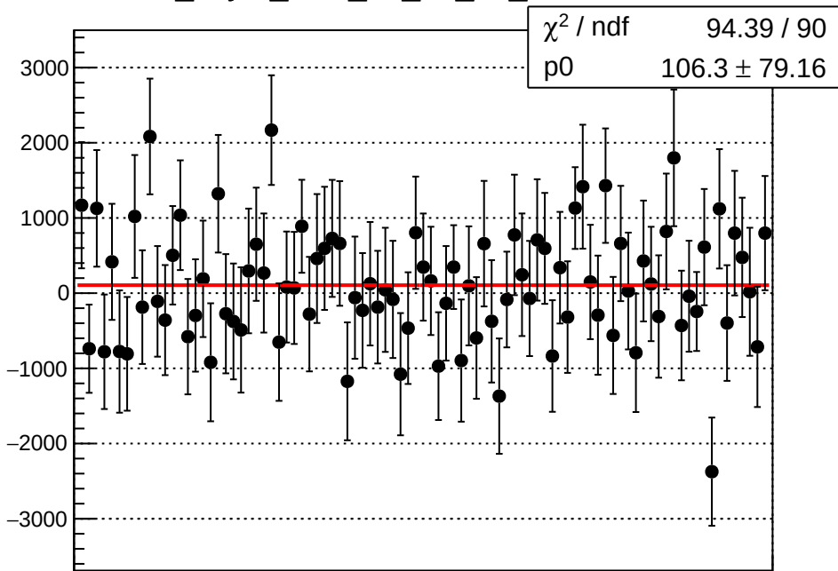
dit_asym_sam_15_26_dd_mean vs run
