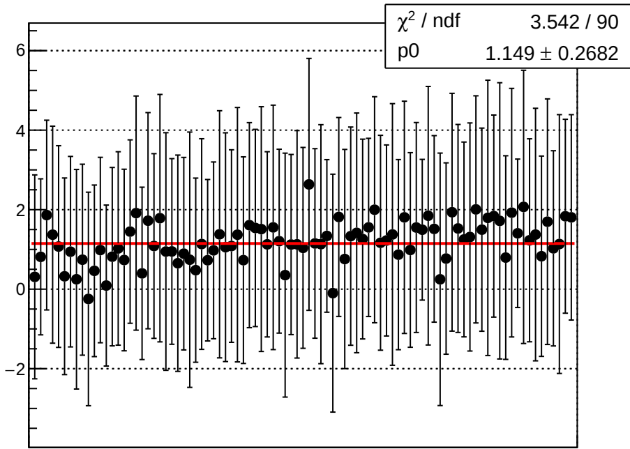
reg_asym_sam_1357_avg_diff_bpm4aY_slope vs run
