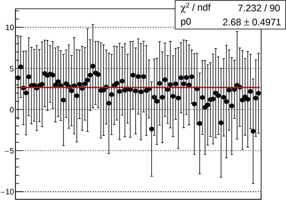
reg_asym_sam_3726_avg_diff_bpm4aY_slope vs run
