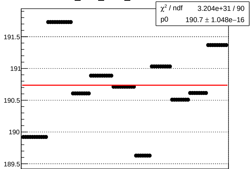
dit_4eY_coil4_mean vs run
