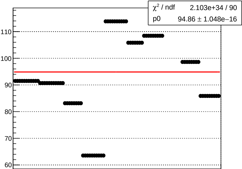
dit_sam8_coil4_err_mean vs run
