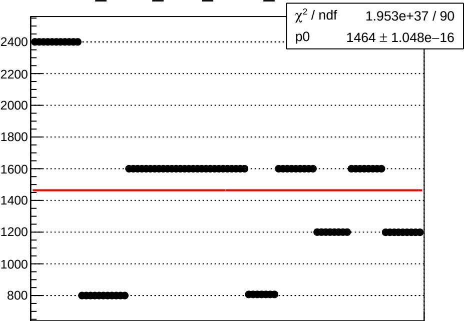
dit_sam4_coil7_Ndata_mean vs run
