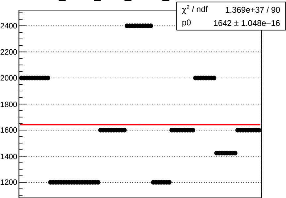
dit_sam8_coil3_Ndata_mean vs run
