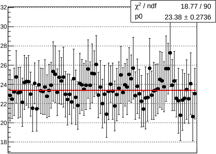
reg_asym_sam_37_dd_diff_bpm4eY_slope vs run
