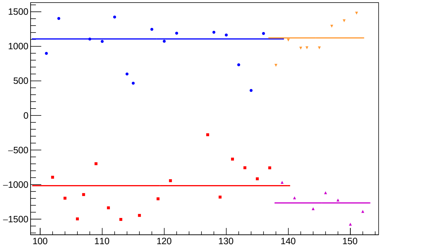
dit_atl2_coil4_Ndata_mean vs Slug, Sign Corrected
