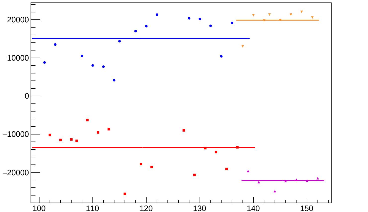
dit_sam6_coil4_mean vs Slug, Sign Corrected
