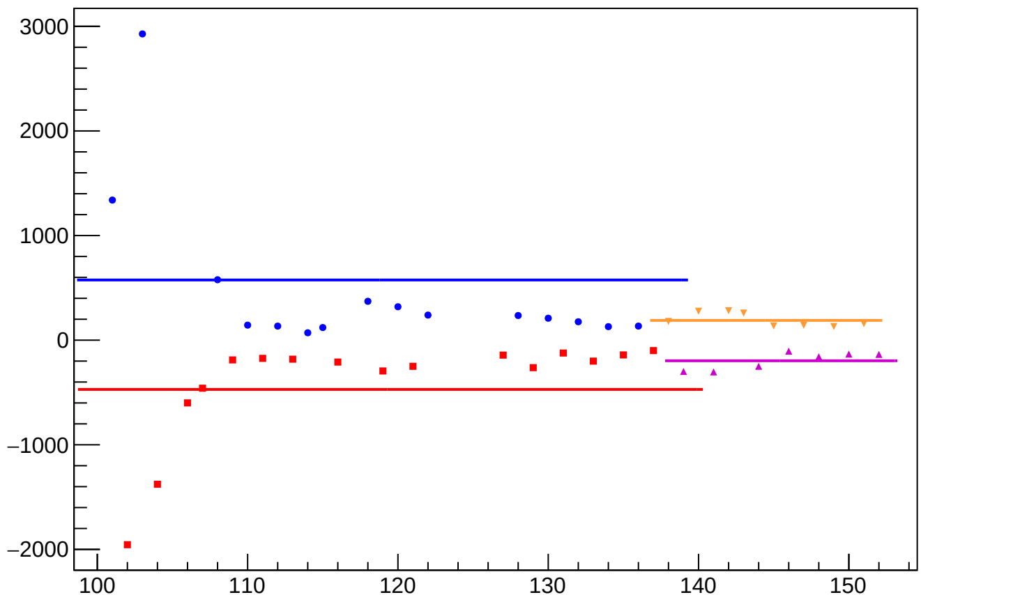
dit_sam3_coil6_err_mean vs Slug, Sign Corrected
