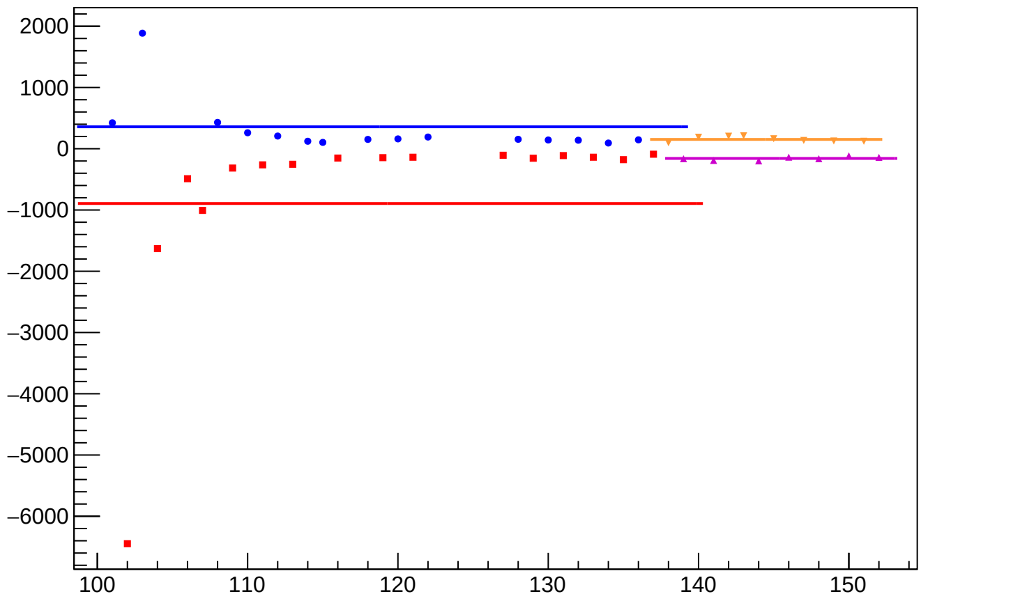
dit_atl1_coil3_err_mean vs Slug, Sign Corrected
