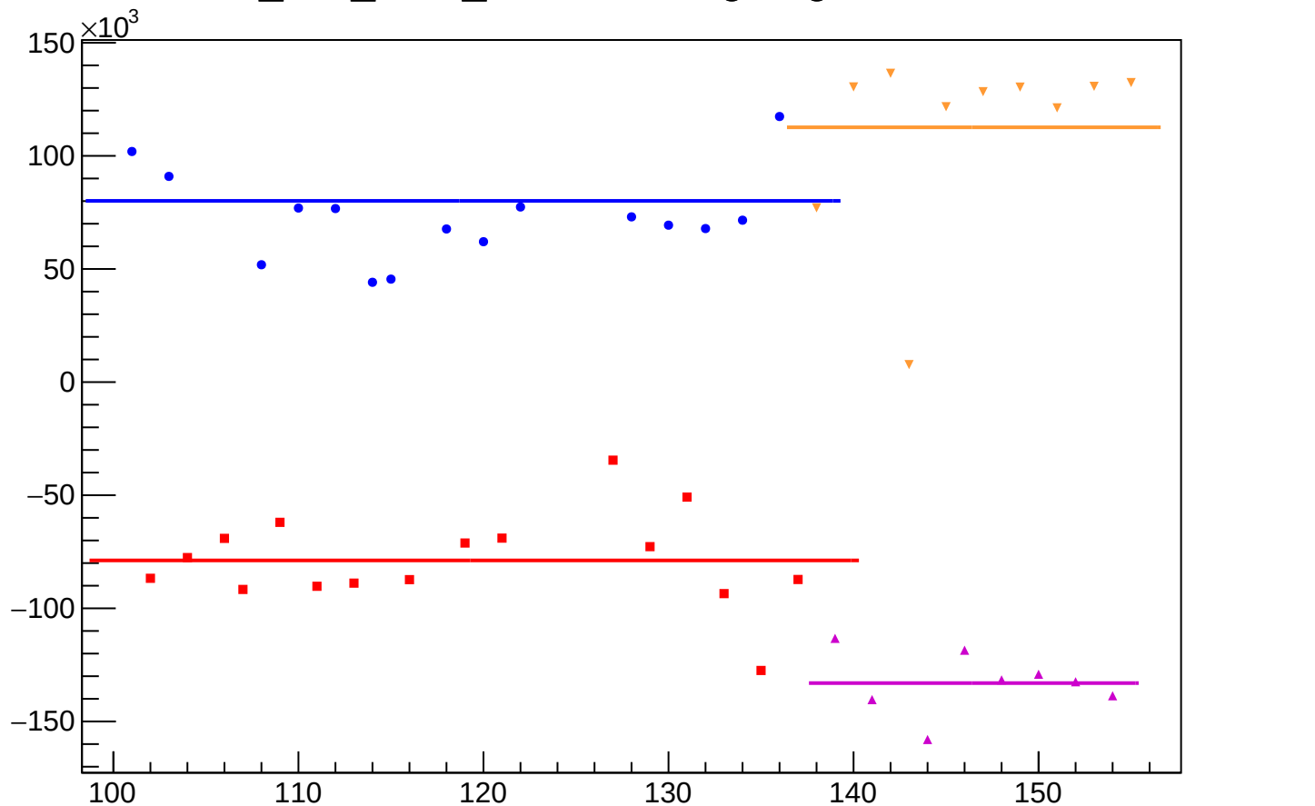
dit_atl2_coil7_mean vs Slug, Sign Corrected
