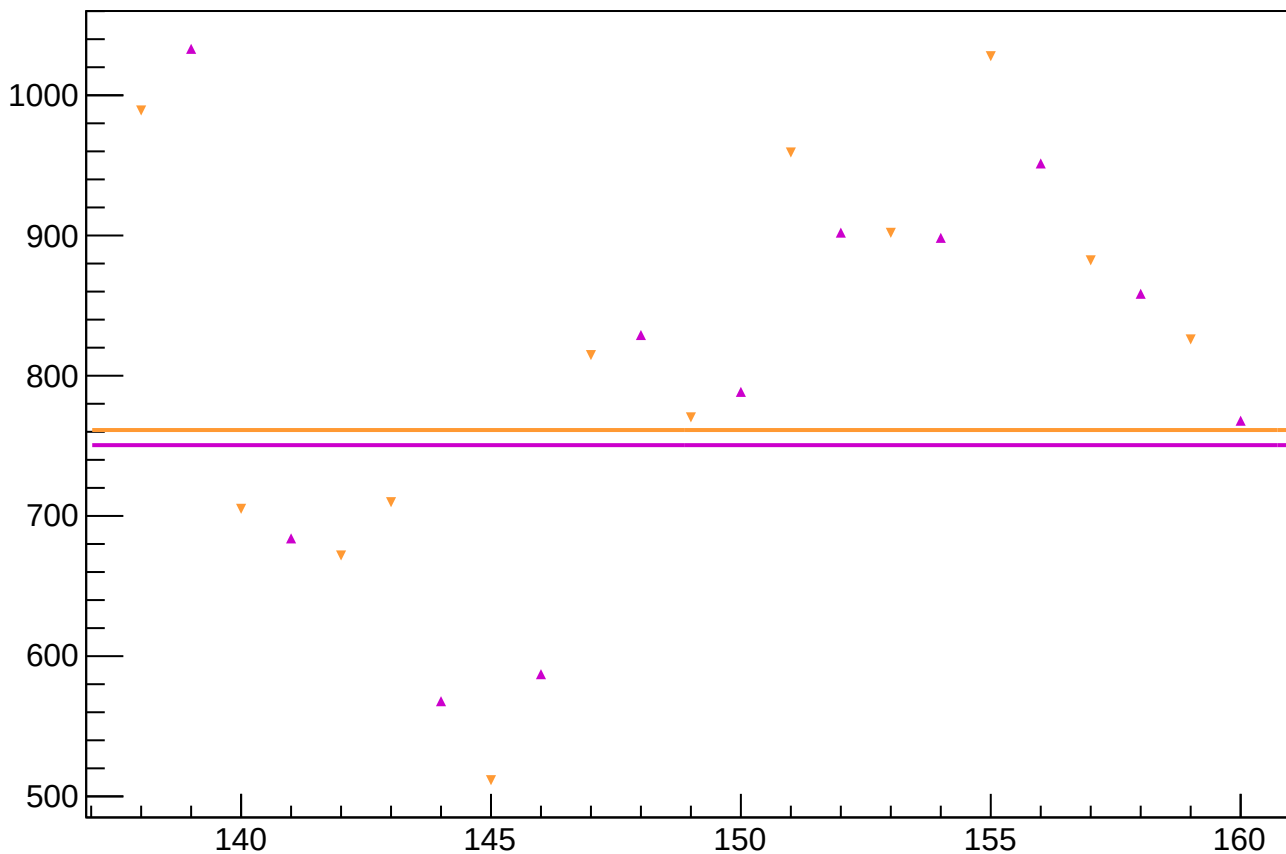
asym_sam_2468_avg_correction_rms vs Slug
