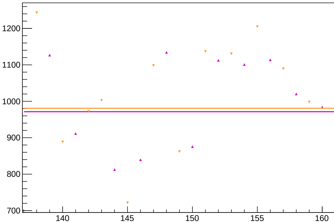
asym_sam_48_dd_rms vs Slug
