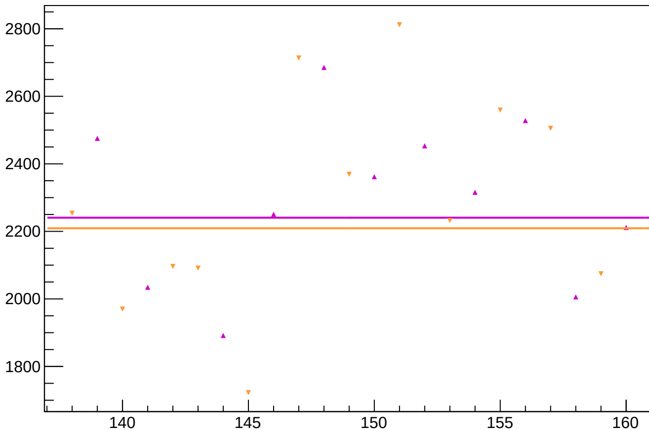
asym_sam2_correction_rms vs Slug
