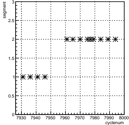
segment:cyclenum
