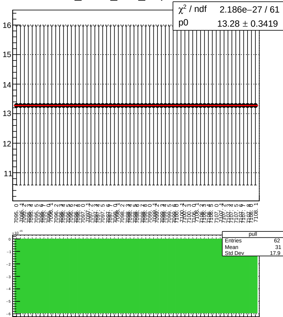
dit_sam5_4aX_slope vs run
