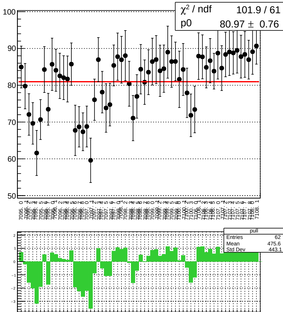
reg_asym_sam_1548_avg_diff_bpm4eY_slope vs run
