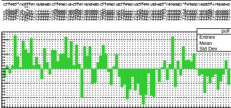
\chi^2 / \text{ndf} 113.1 p_0 -8.455 \pm 0.005
