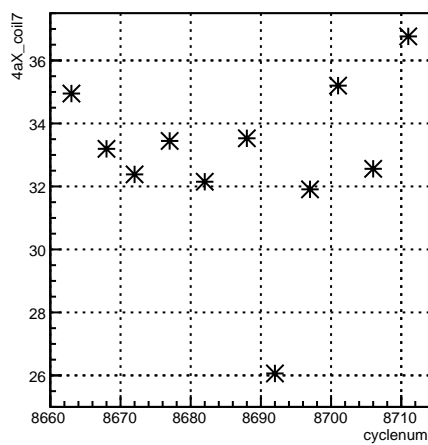
4aX_coil7:cyclenum
