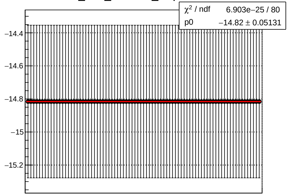
dit_atr1_11X12X_slope vs run
