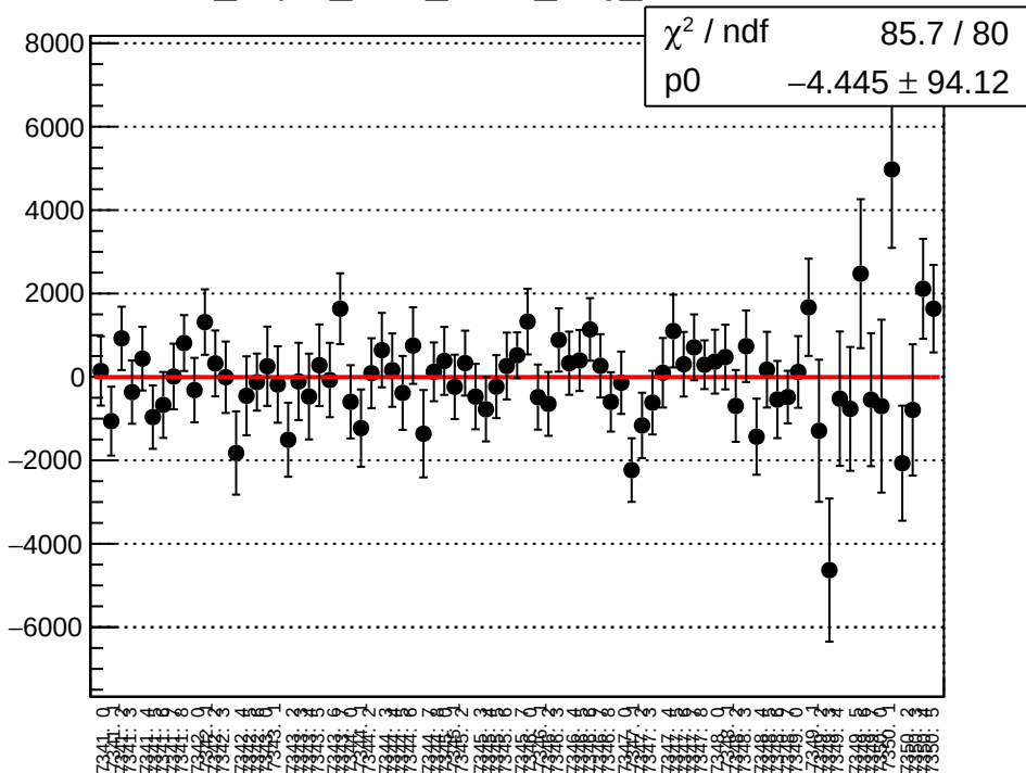
dit_asym_sam_1526_avg_g_mean vs run
