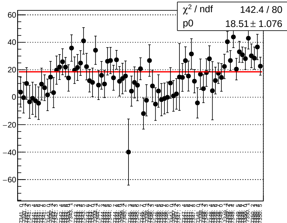
reg asym atl dd atr dd dd diff bpm1X slope vs run
