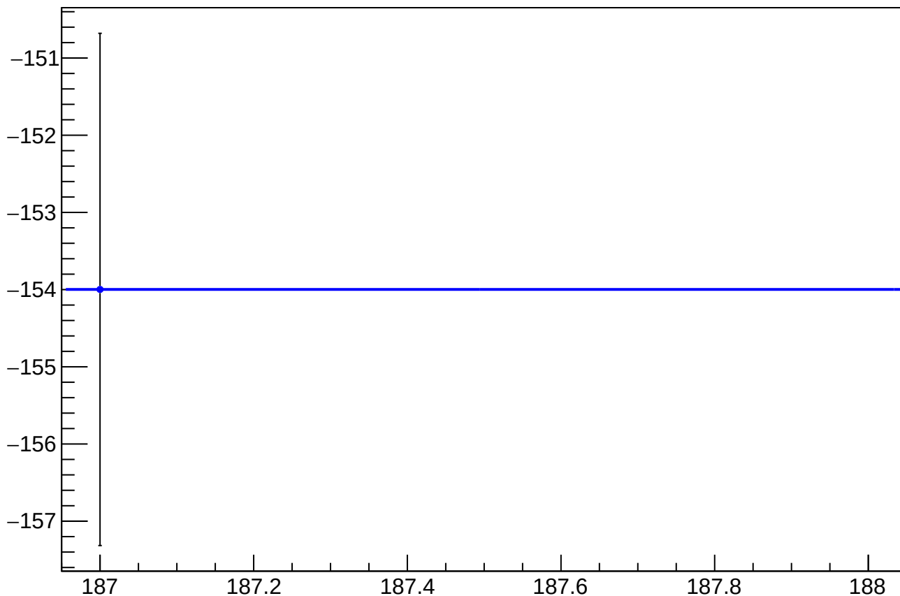
reg_asym_atr1_diff_bpm1X_slope vs Slug
