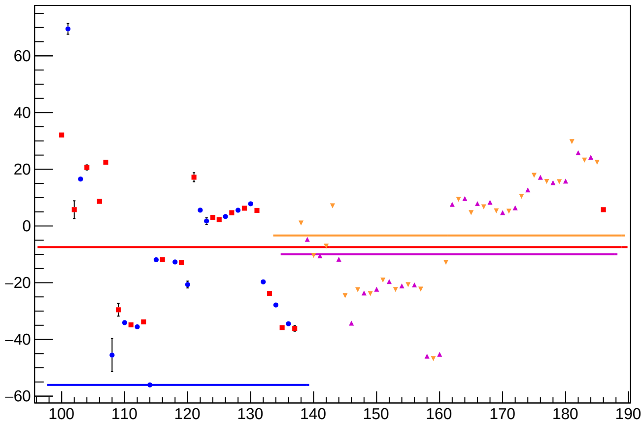
dit_atl2_4aY_slope vs Slug, Sign Corrected
