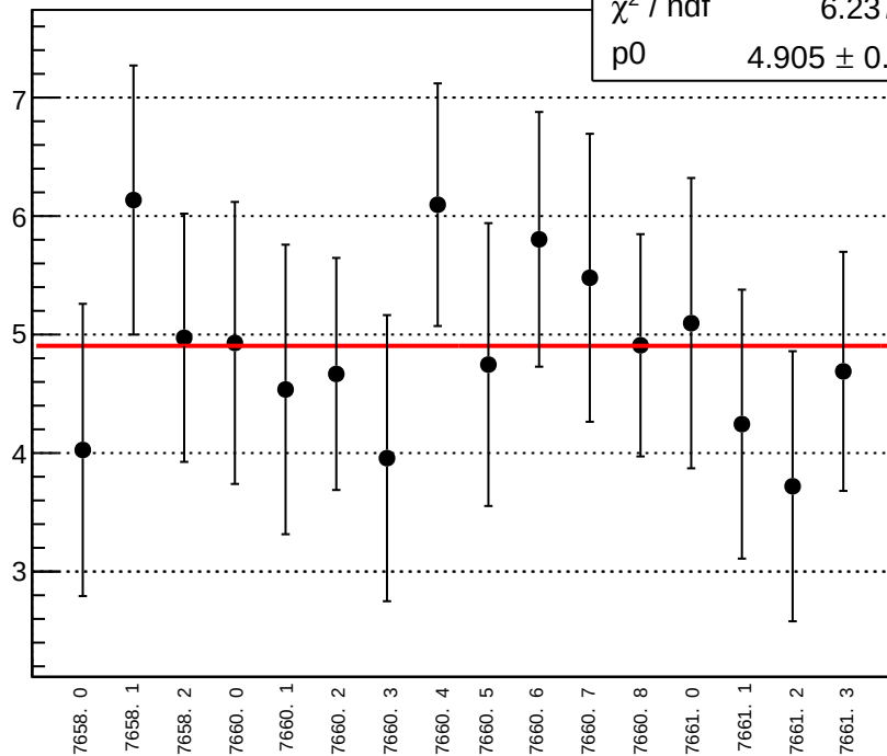
reg_asym_atl_dd_atr_dd_dd_diff_bpm12X_slope vs run
