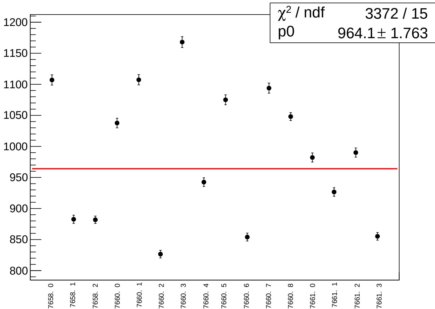
asym_sam_37_48_dd_correction_rms vs run
