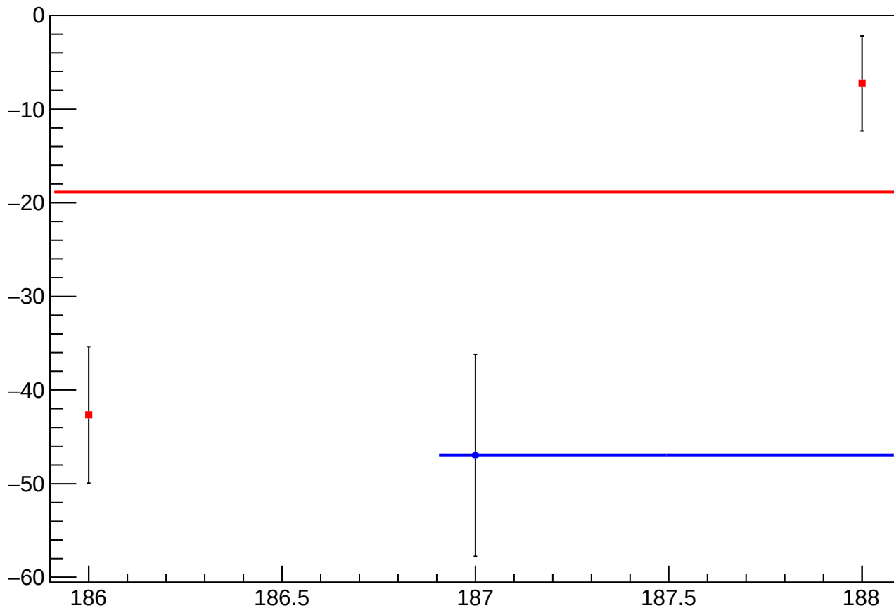
reg_asym_atr_dd_diff_bpm4eY_slope vs Slug, Sign Corrected
