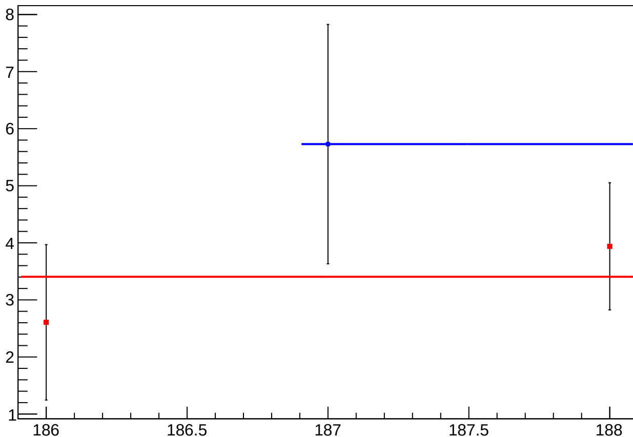
reg_asym_atl_dd_atr_dd_dd_diff_bpm1X_slope vs Slug, Sign Corrected
