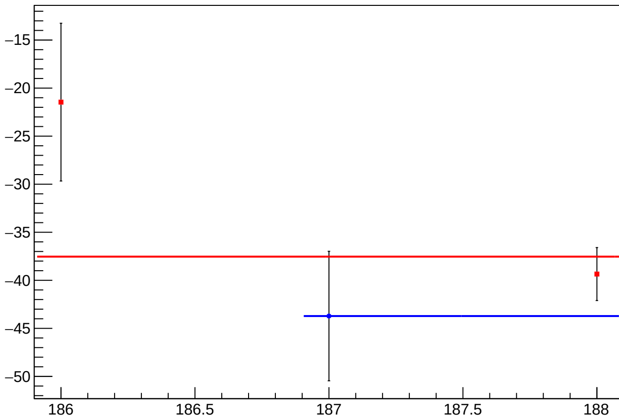
reg_asym_sam_26_dd_diff_bpm4aY_slope vs Slug, Sign Corrected
