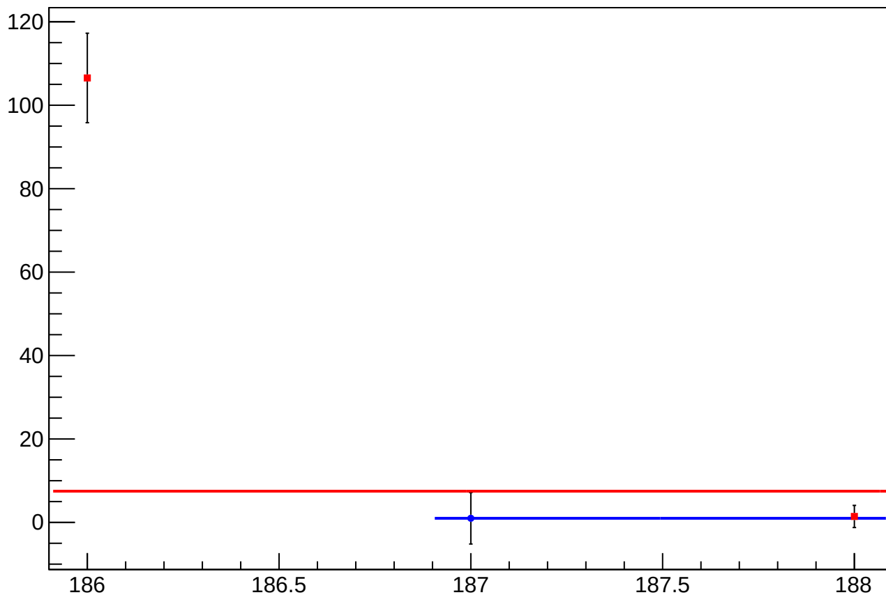
reg_asym_sam4_diff_bpm1X_slope vs Slug, Sign Corrected
