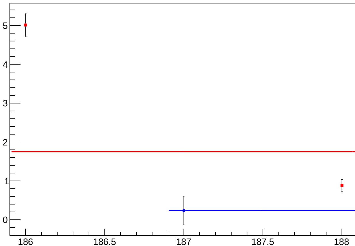
reg_asym_sam3_diff_bpm12X_slope vs Slug, Sign Corrected
