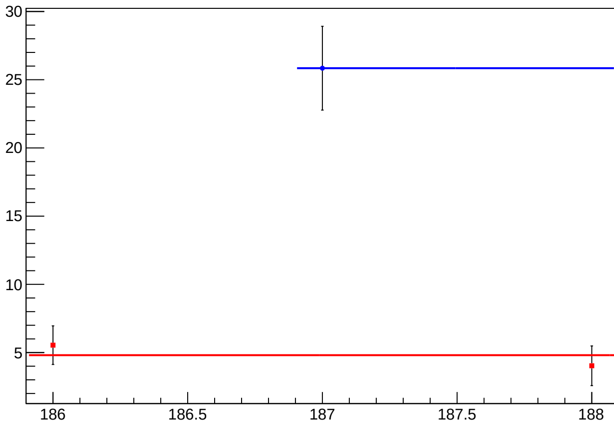
reg_asym_at1_avg_diff_bpm4aY_slope vs Slug, Sign Corrected
