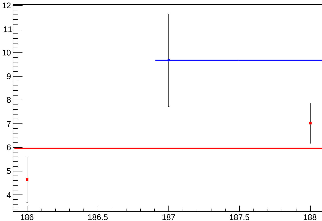
reg_asym_sam7_diff_bpm4aY_slope vs Slug, Sign Corrected
