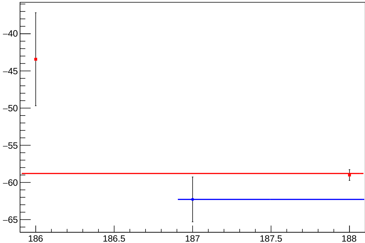
reg_asym_sam_15_dd_diff_bpm4aY_slope vs Slug, Sign Corrected
